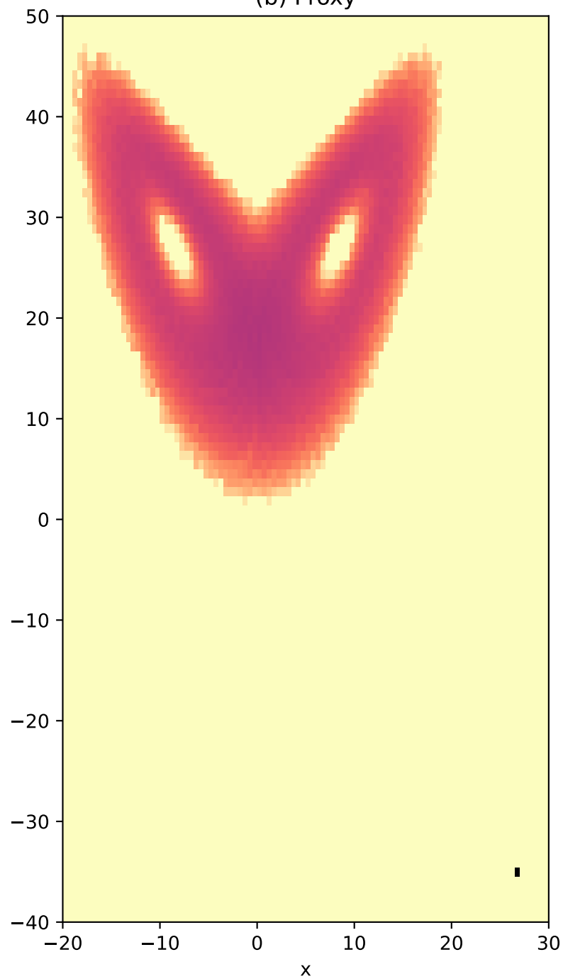
(b) Proxy
