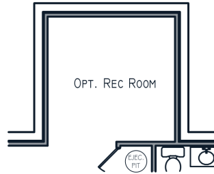
EXTENDED REC ROOM WITH OPTIONAL SUNROOM ABOVE
