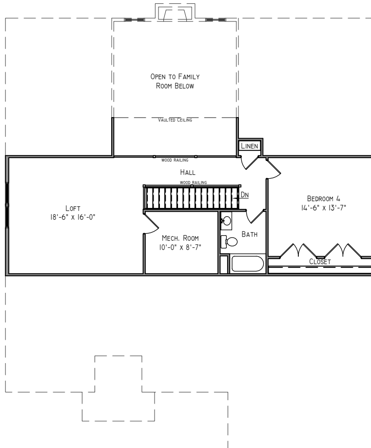
Optional Second Floor Plan
