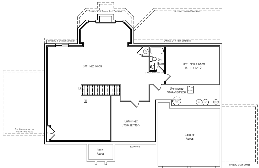
Extended Rec Room and Media Room w/ Optional 2'-0" Rear Extension and 4'-0" Family Room Extension Above
