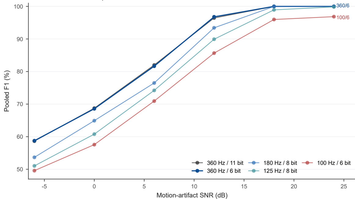
R-peak detection robustness under standardized motion artifact
