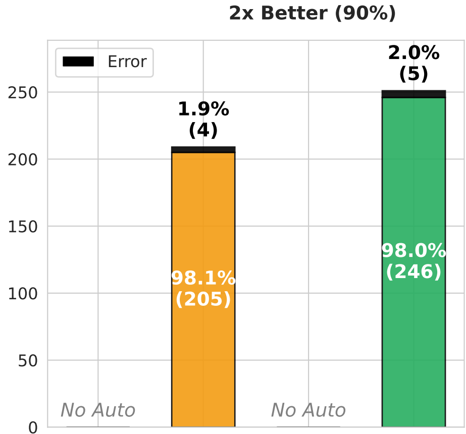
(I) Safety Profile (Actual Test Set Errors)
