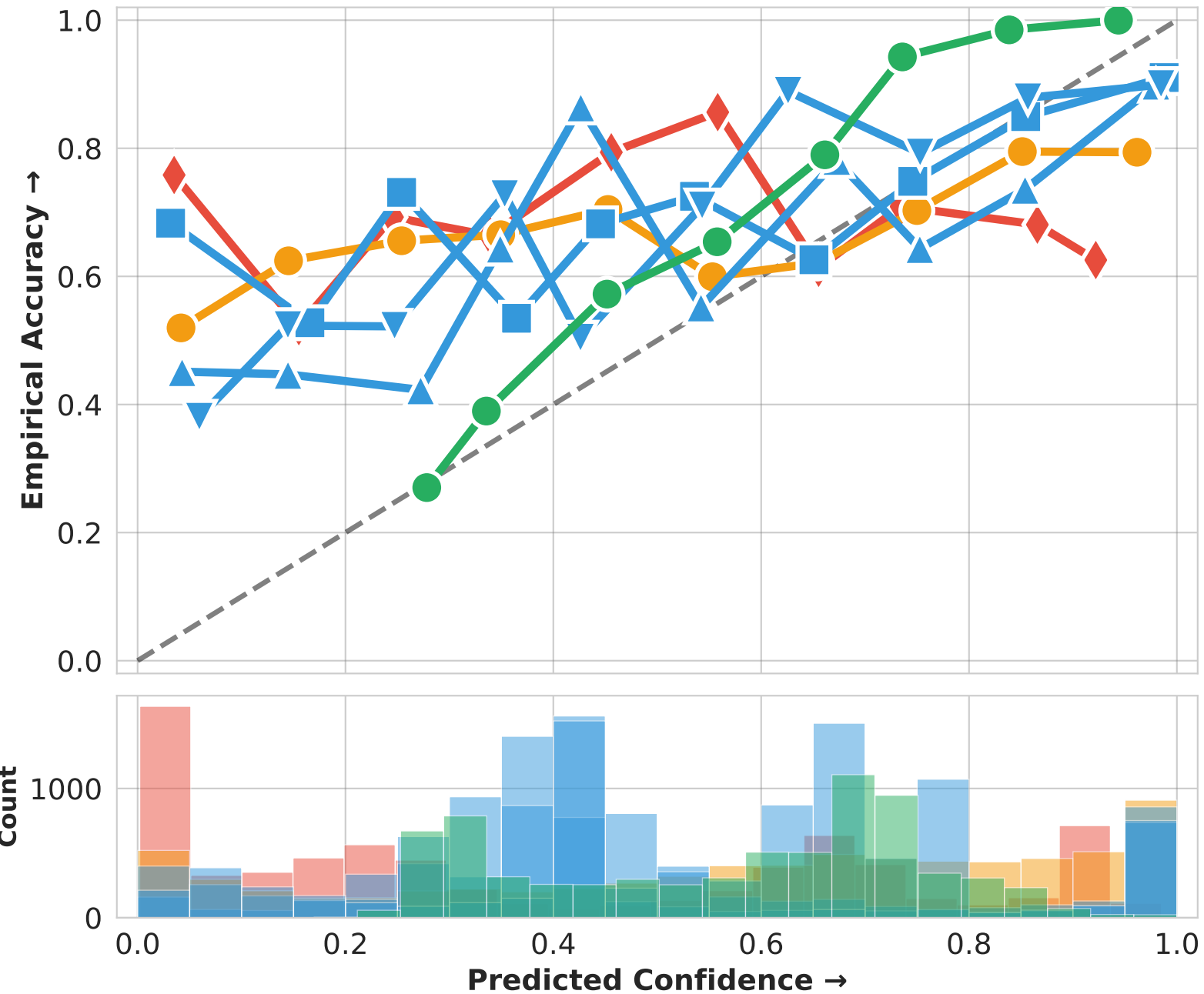
(A) Calibration vs. Discrimination Trade-off - CORAL-MCQA-Contextual (B) Calibration Reliability Diagram - CORAL-MCQA-Contextual
