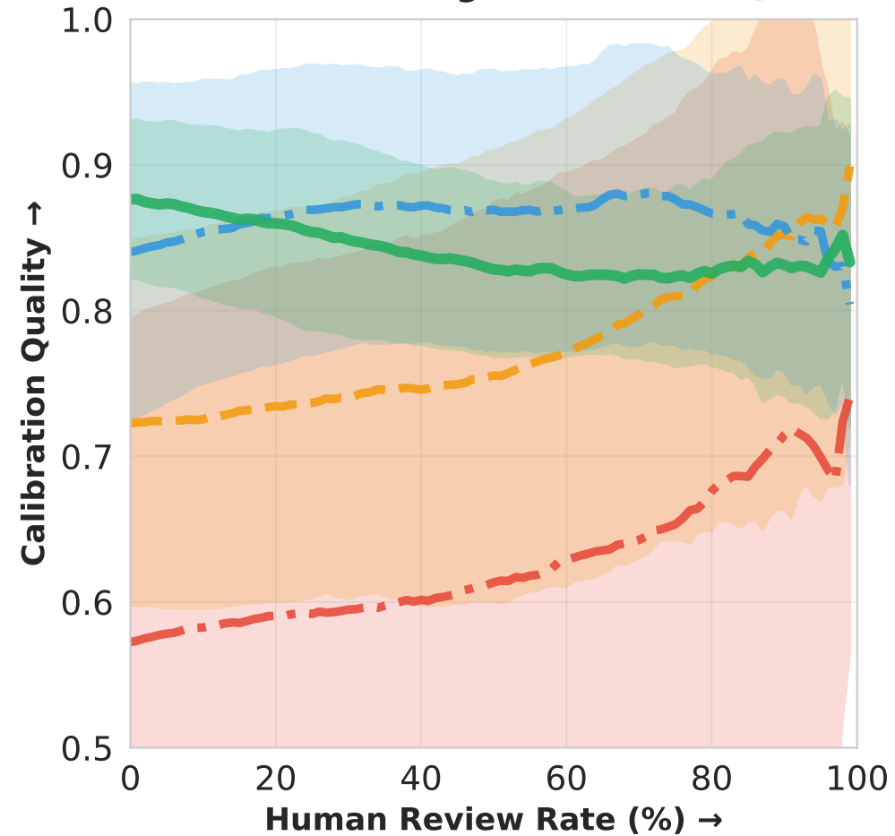
(E) Calibration Under Triage - CORAL-MCQA-Contextual
