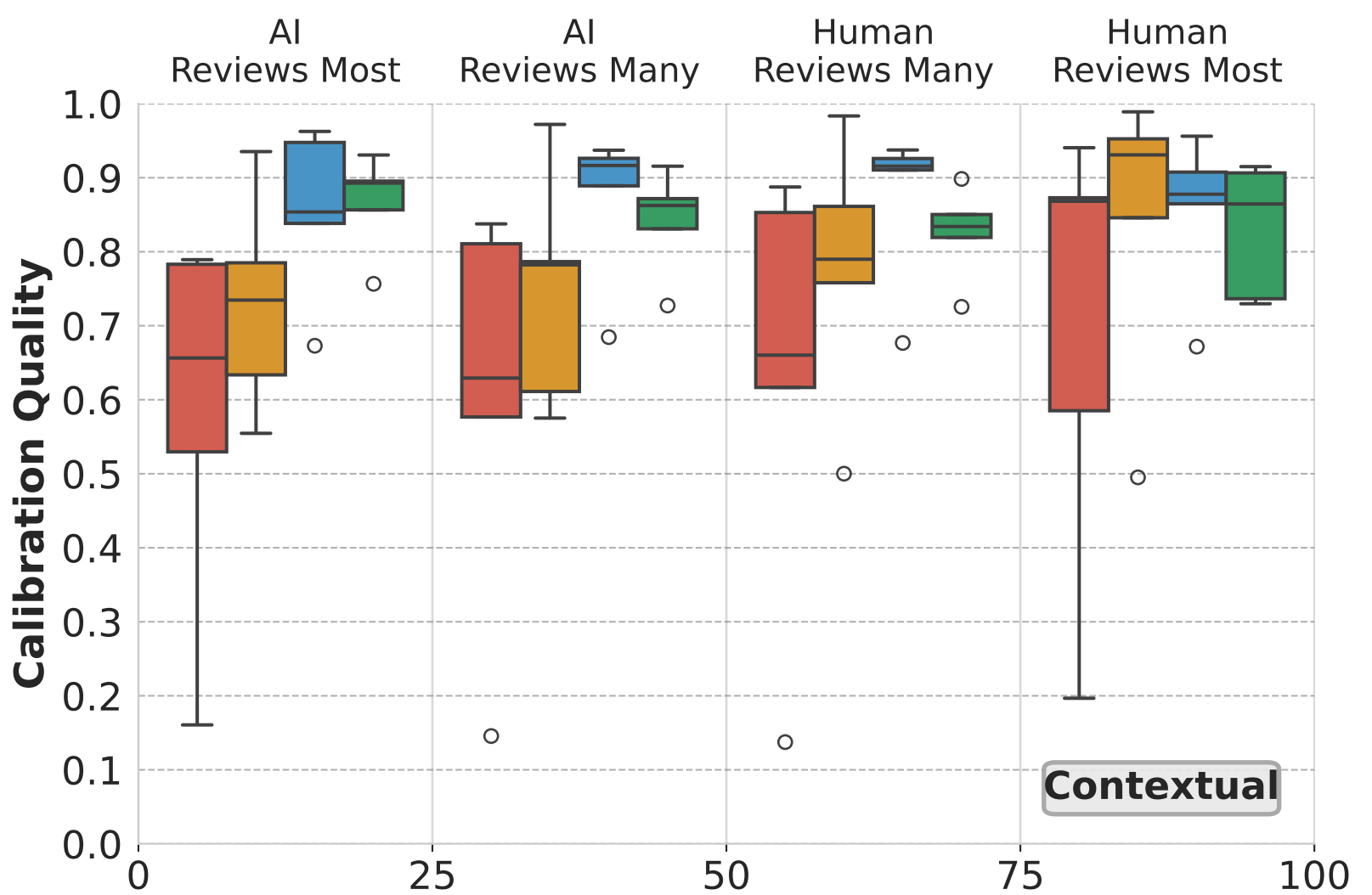
Calibration Quality Robustness across Models
