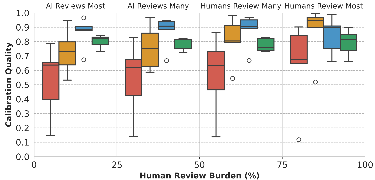
(G) Calibration Quality Robustness across Models - Inference
