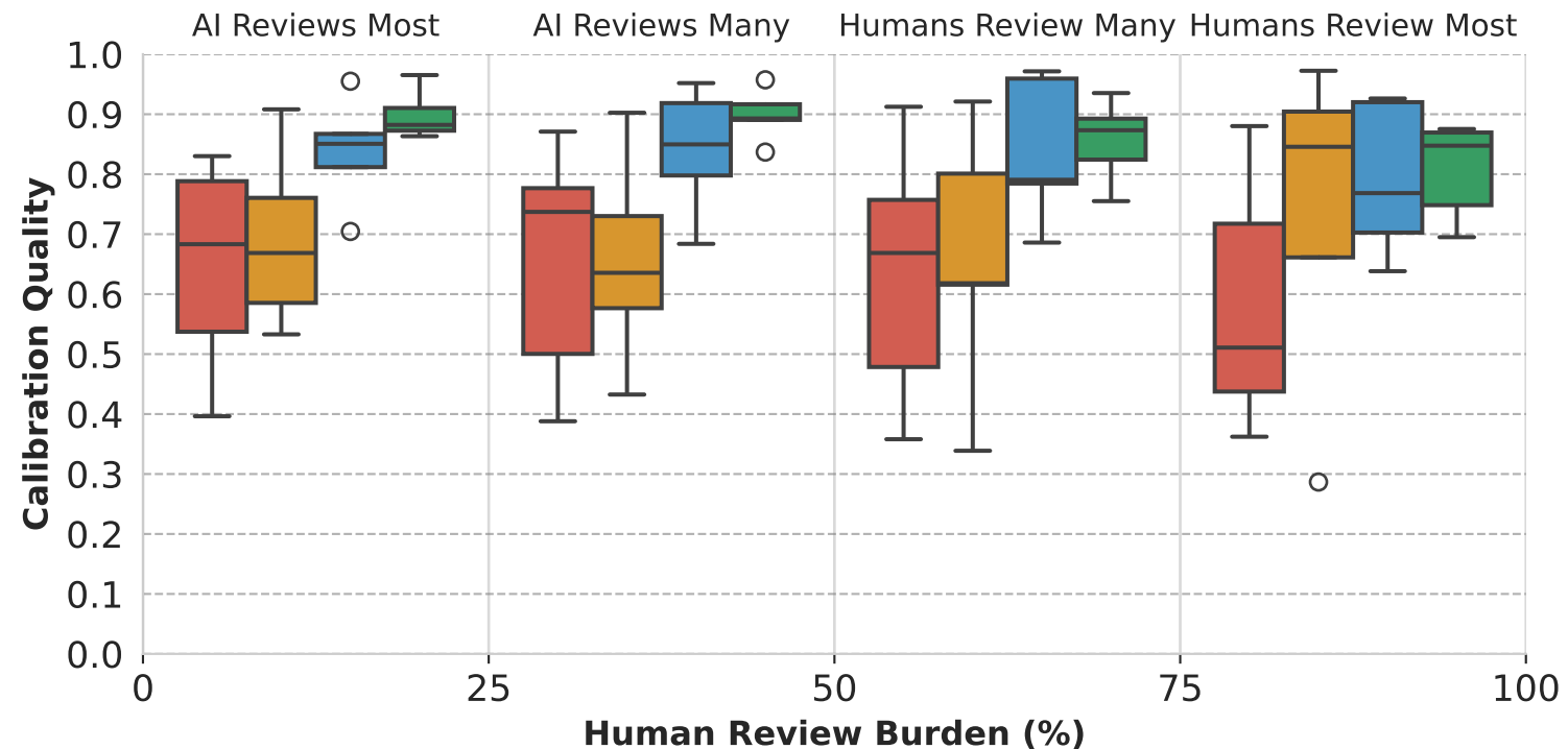
(G) Calibration Quality Robustness across Models - Synthesis
