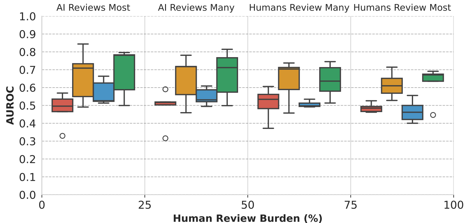
(F) AUROC Robustness across Models - Synthesis
