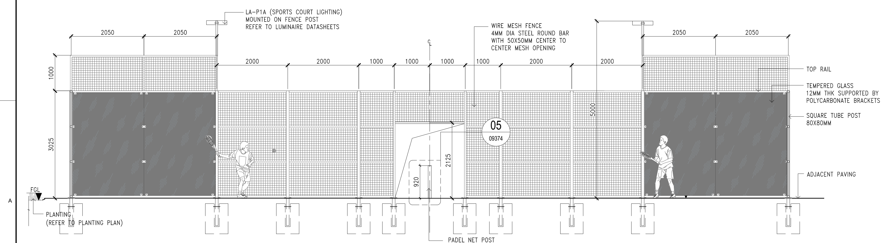
02 F07 - PADEL TENNIS FENCE DETAIL 09374 SPORTS HUB Scale 1:50
