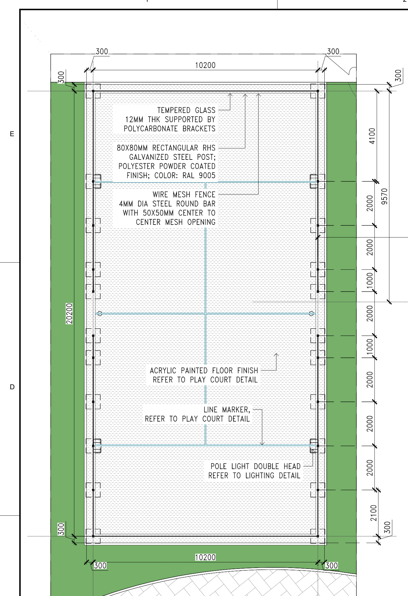
01 F07 - PADEL TENNIS FENCE DETAIL-PLAN 09374 SPORTS HUB Scale 1:100
