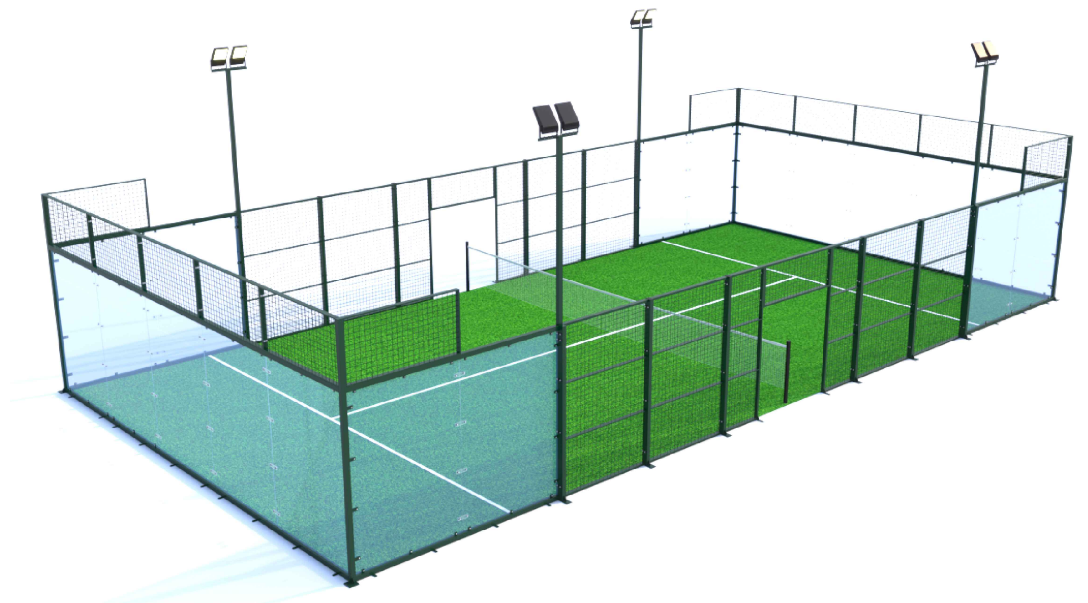
04 FE-19 - TYPICAL PADEL TENNIS DETAIL-REFERENCE IMAGE 09374 SPORTS HUB Scale 1:50
