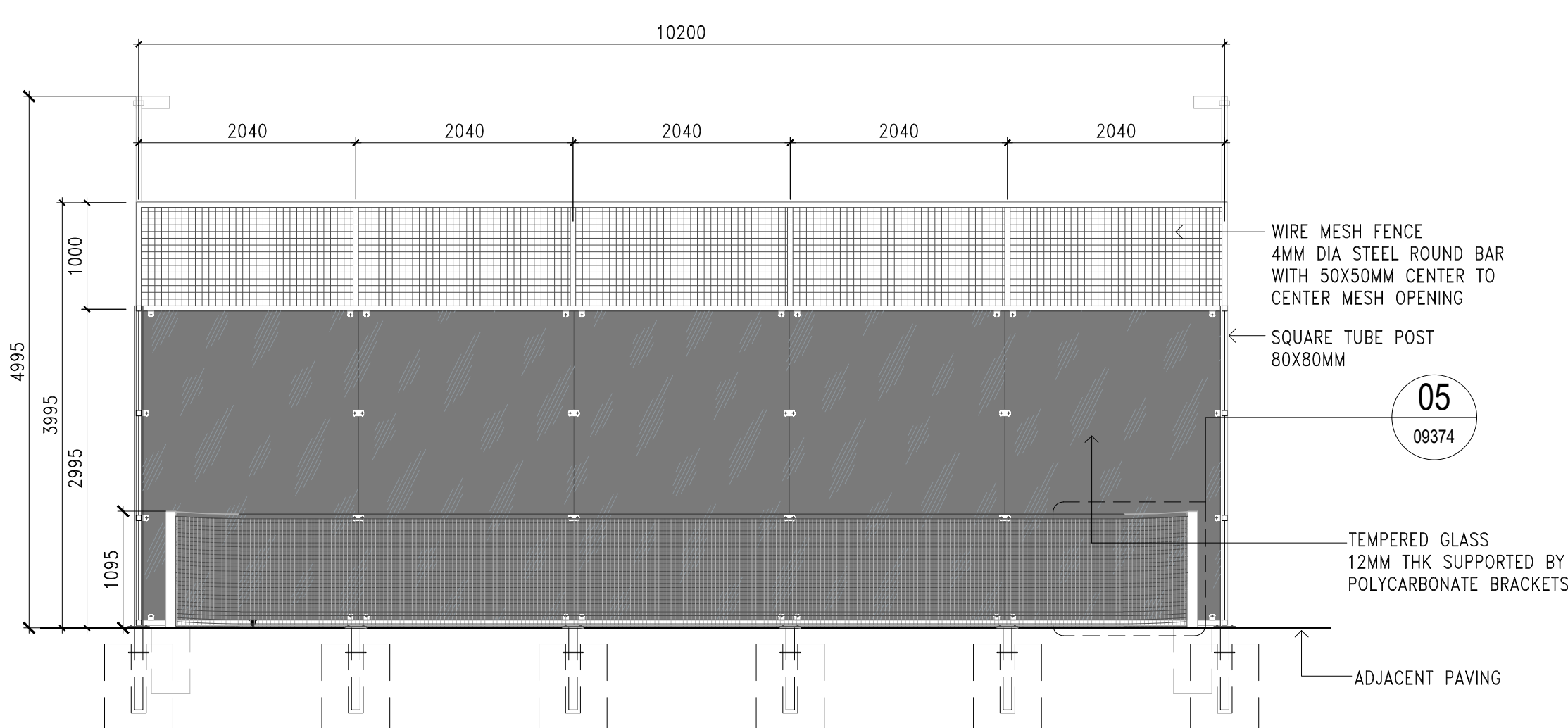
03 F07 - PADEL TENNIS FENCE DETAIL 09374 SPORTS HUB Scale 1:50
