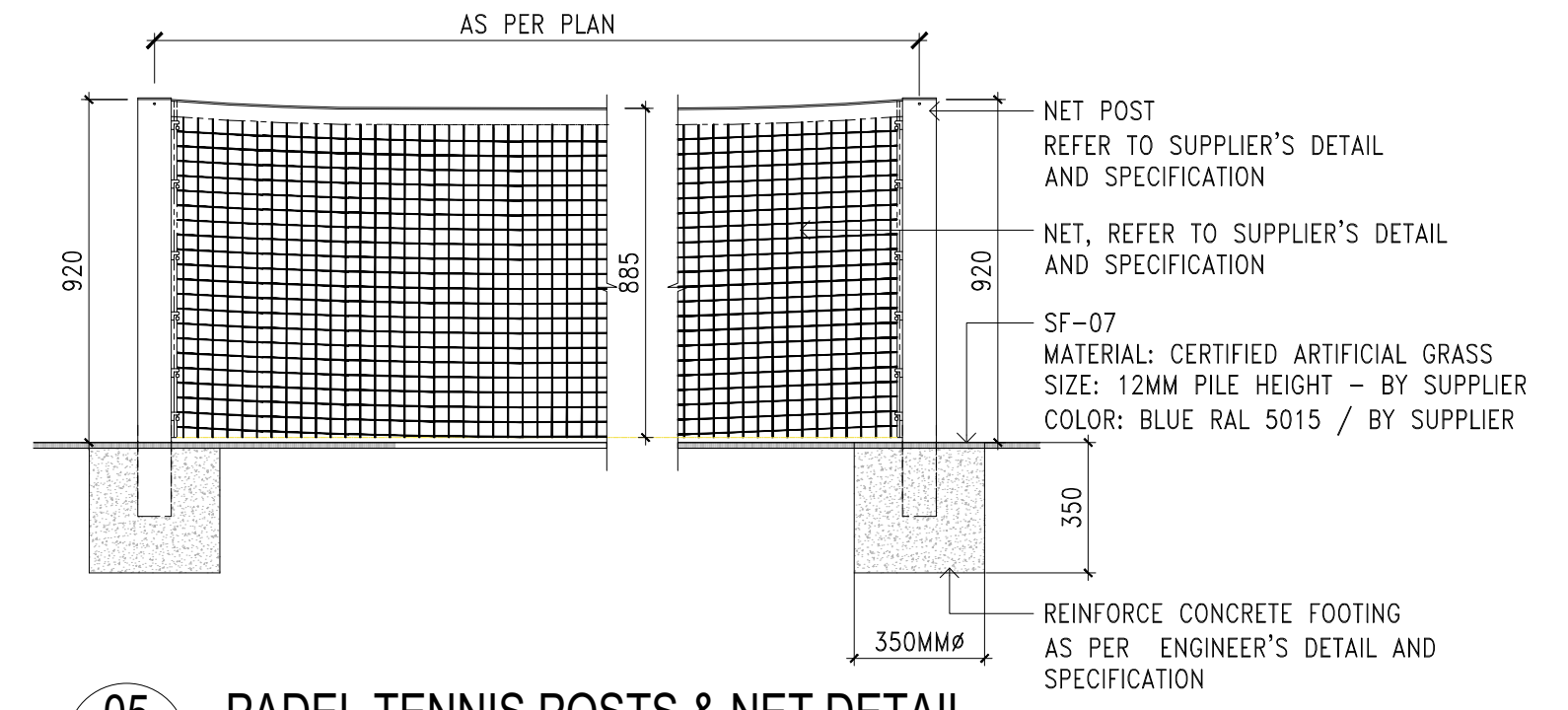
05 PADEL TENNIS POSTS & NET DETAIL 09374 Scale 1:20
