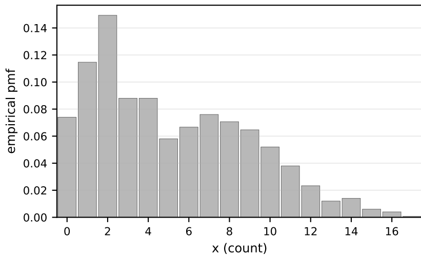
S3: 0.5 Pois(2)+0.5 Pois(8) N=1500 , V/M=2.80
