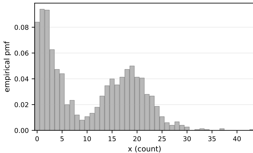
S4: 0.5 NB(2,0.4)+0.5 (CMP(3,0.5)+9) N=1500 , V/M=6.92
