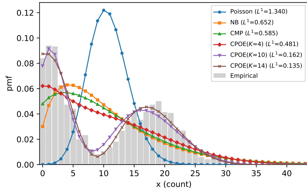
S4: empirical vs baselines vs CPOE( K=4,10,14 ; MoM)
