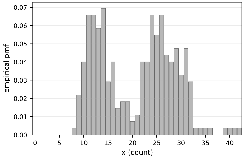
Insurance-smoker N=274 , V/M=2.85
