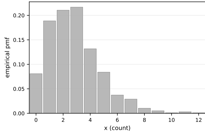
FIFA (World Cup goals) N=964 , V/M=1.32
