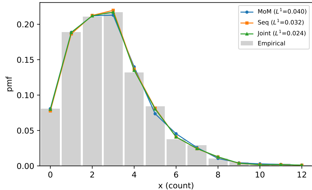
FIFA: 3 estimators at K=14
