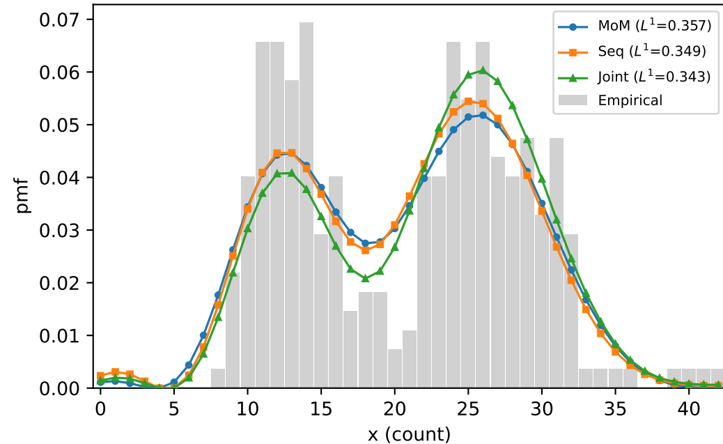
Insurance-smoker: 3 estimators at K=10
