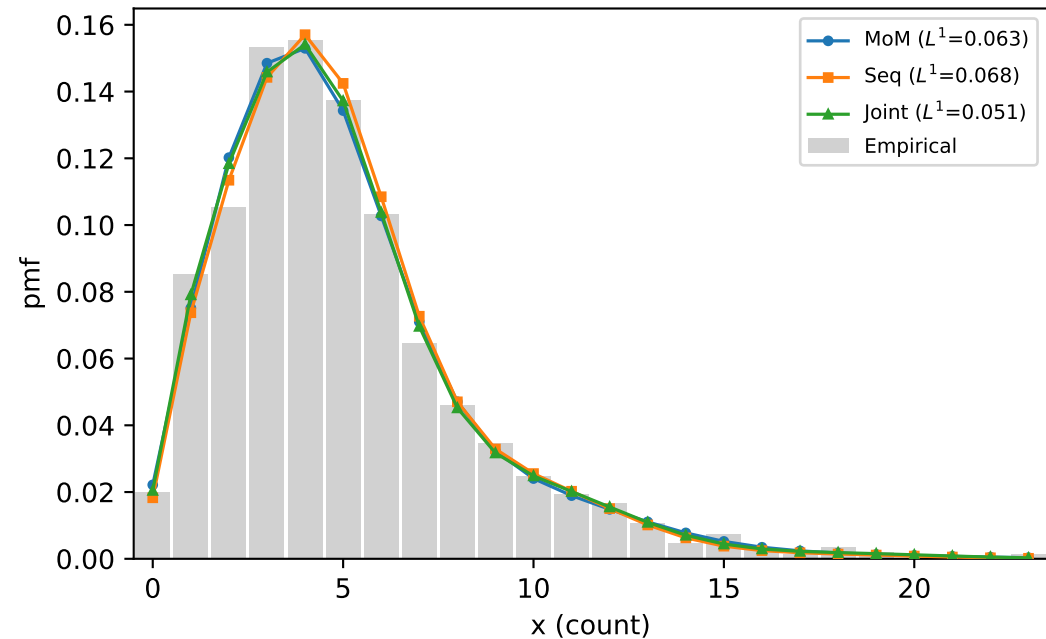
S2: 3 estimators at K=10
