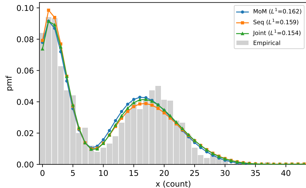
S4: 3 estimators at K=10
