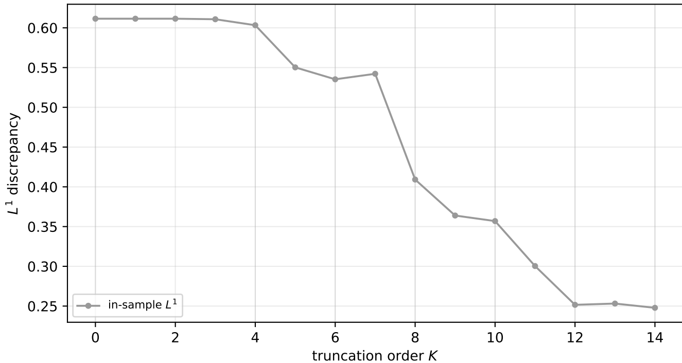
Insurance-smoker: in-sample L^1 vs K (MoM)
