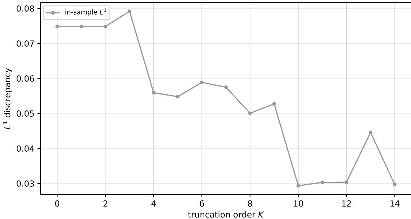
S1: in-sample L^1 vs K (MoM)
