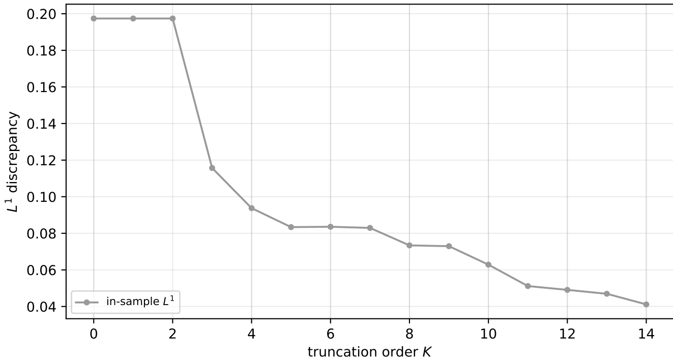
S2: in-sample L^1 vs K (MoM)
