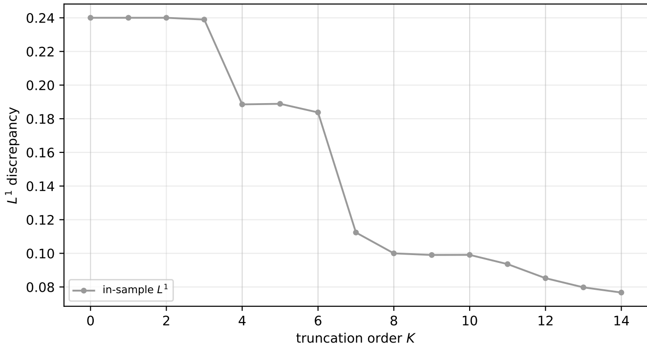
S3: in-sample L^1 vs K (MoM)
