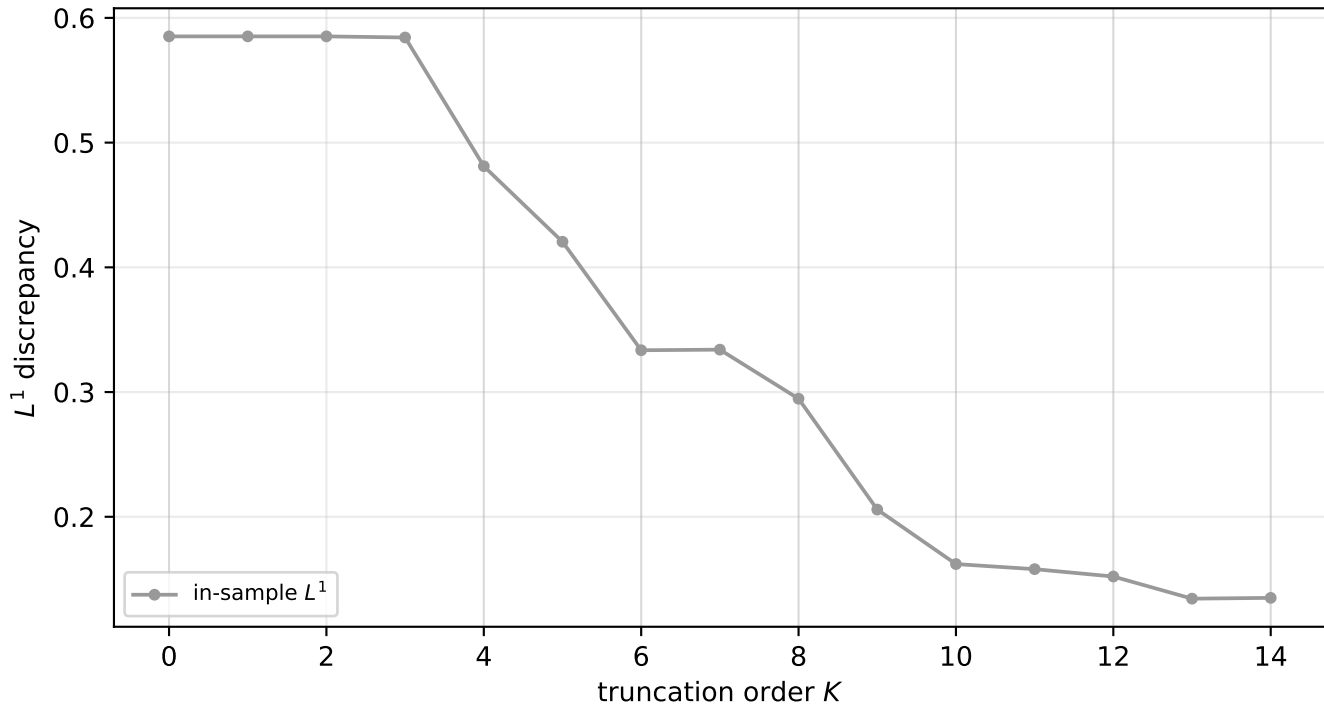
S4: in-sample L^1 vs K (MoM)
