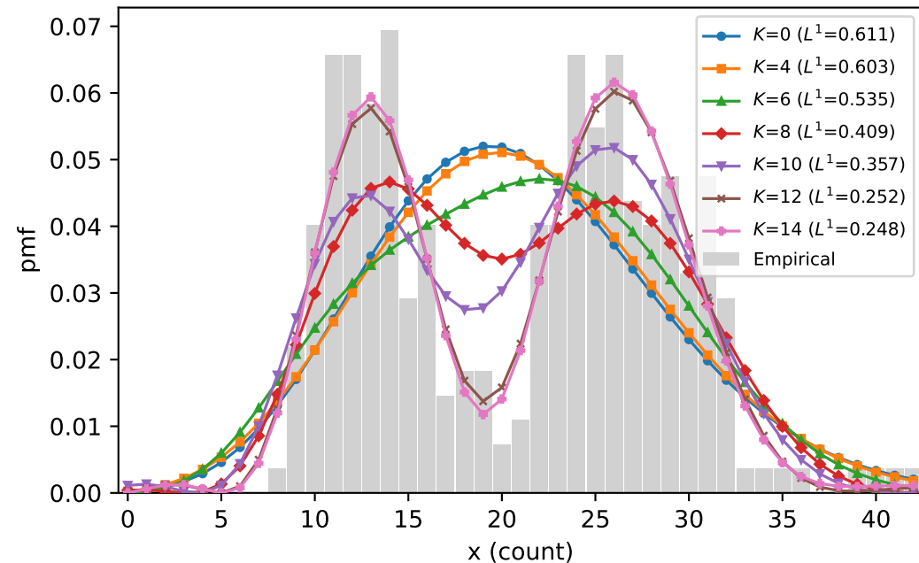
Insurance-smoker: empirical vs CPOE(MoM) pmf by K
