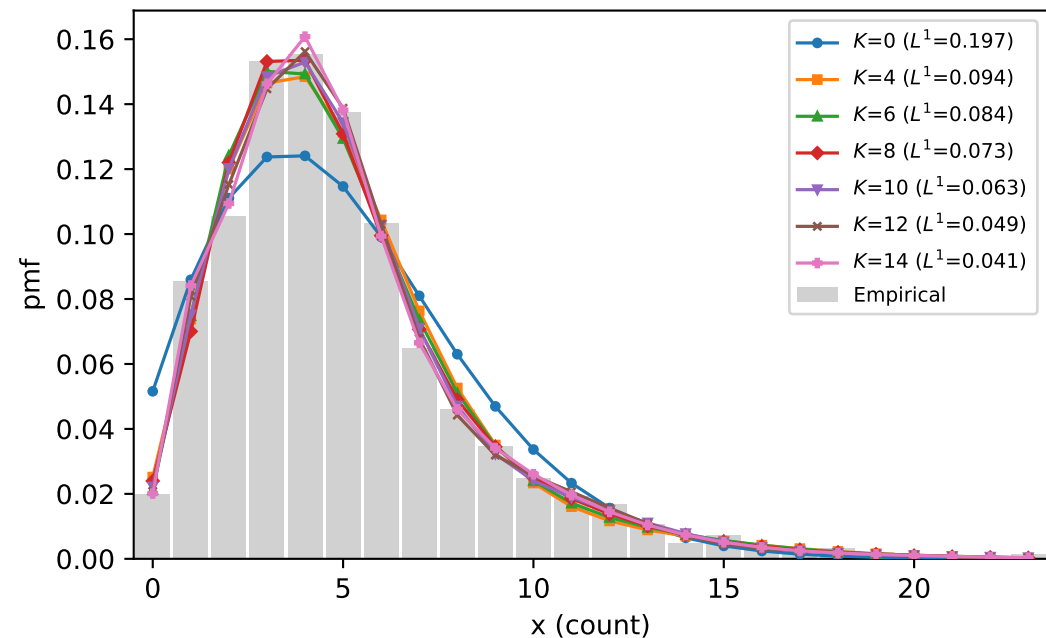
S2: empirical vs CPOE(MoM) pmf by K
