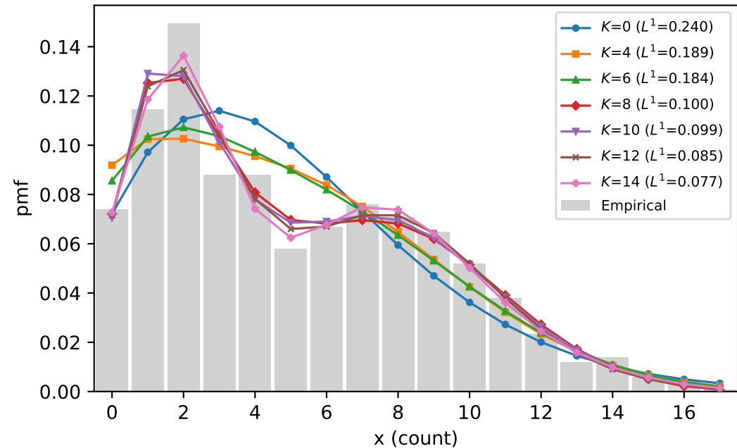
S3: empirical vs CPOE(MoM) pmf by K
