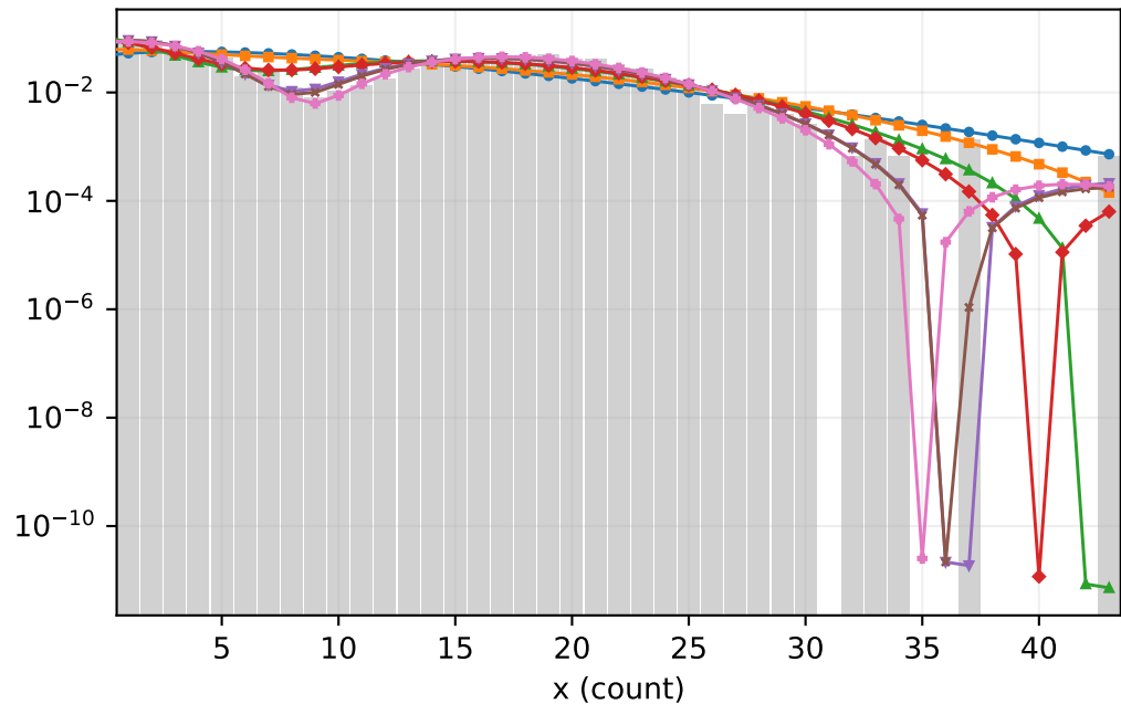
tail zoom (log-y)
