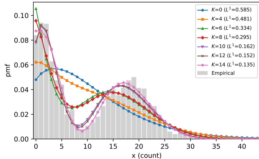
S4: empirical vs CPOE(MoM) pmf by K
