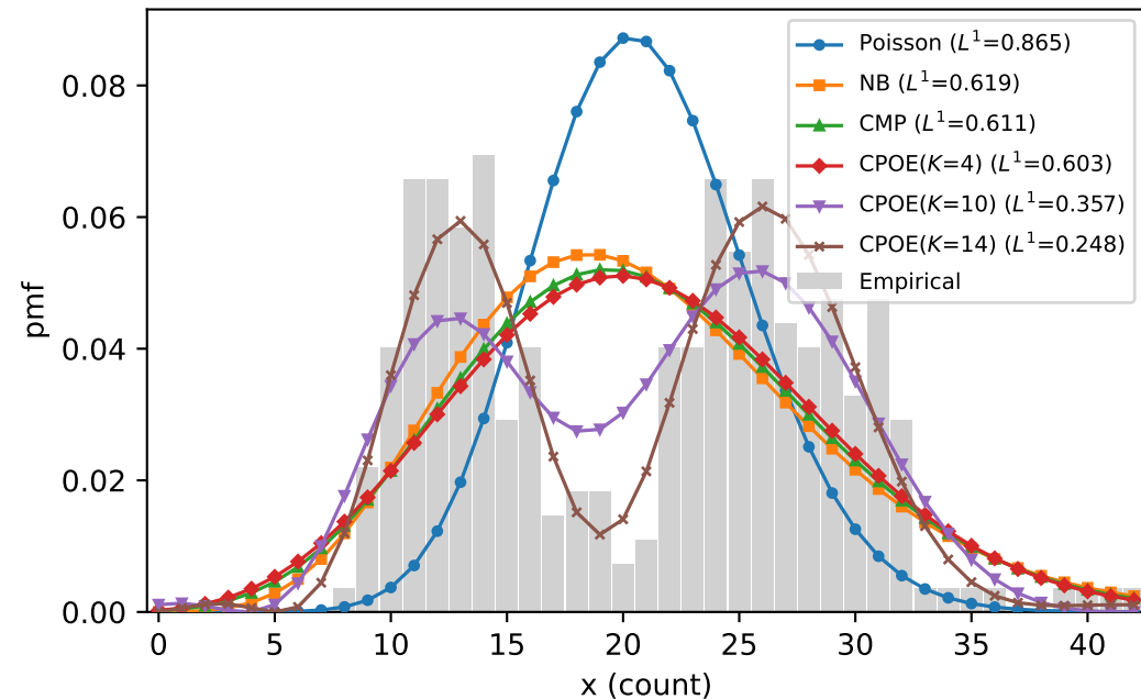
Insurance-smoker: empirical vs baselines vs CPOE( K=4,10,14 ; MoM)
