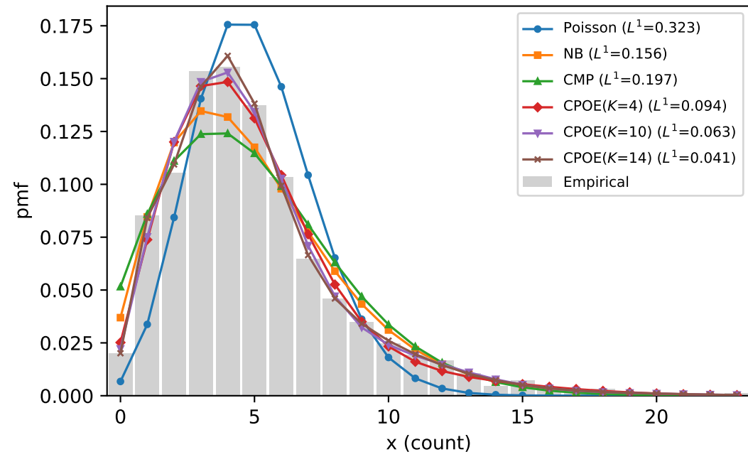
S2: empirical vs baselines vs CPOE( K=4,10,14 ; MoM)
