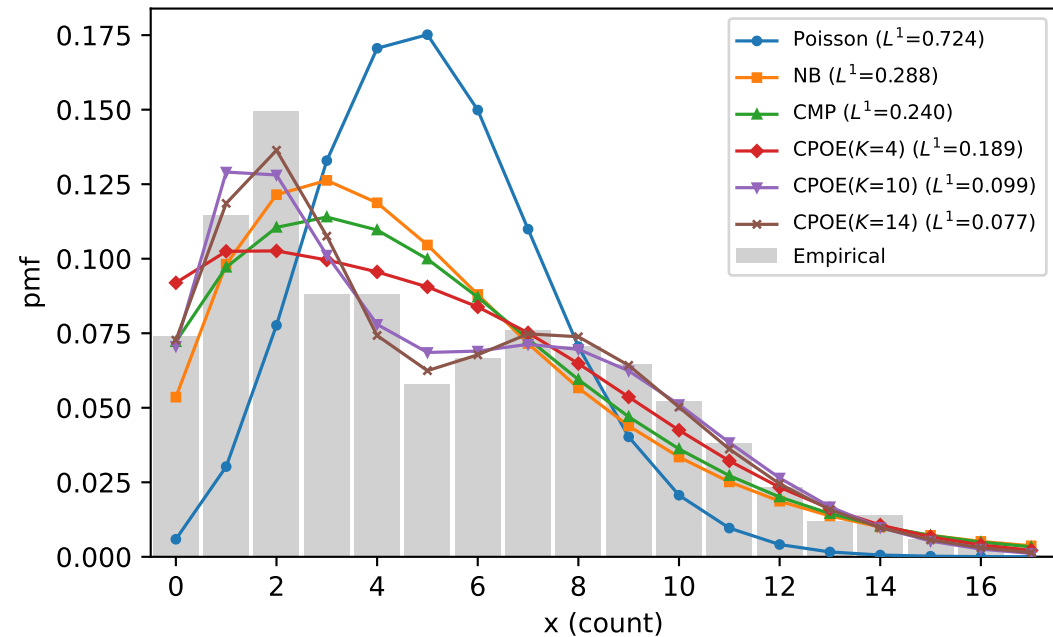
S3: empirical vs baselines vs CPOE( K=4,10,14 ; MoM)
