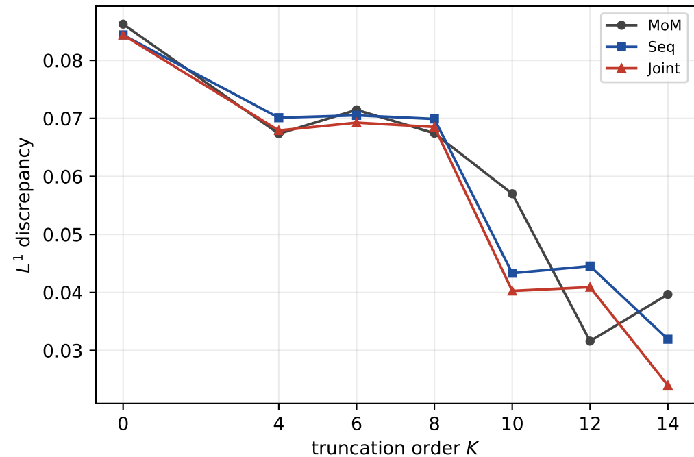
FIFA: L^1 vs K
