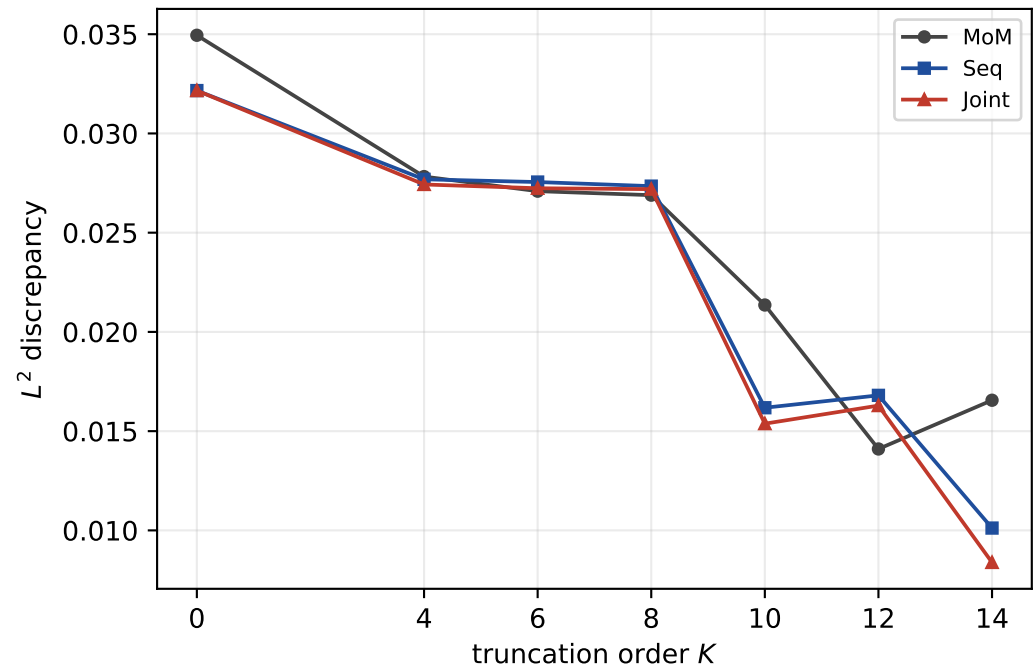
FIFA: unweighted L^2 vs K
