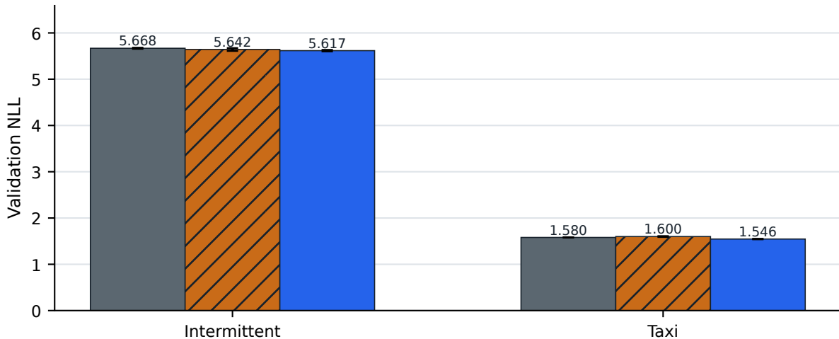
RMTPP-matched THP-matched TitanTPP Validation likelihood on completed e300 comparisons
