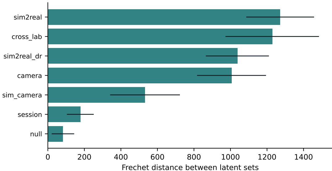
Distribution-shift rungs measured in one space (mean \pm sd)
