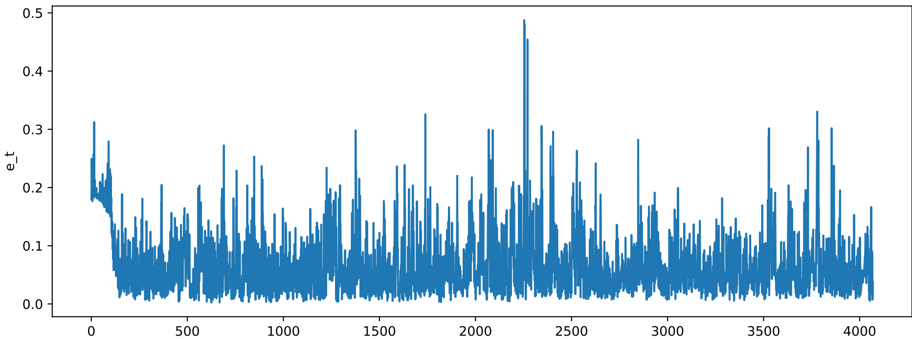
Translation Error
