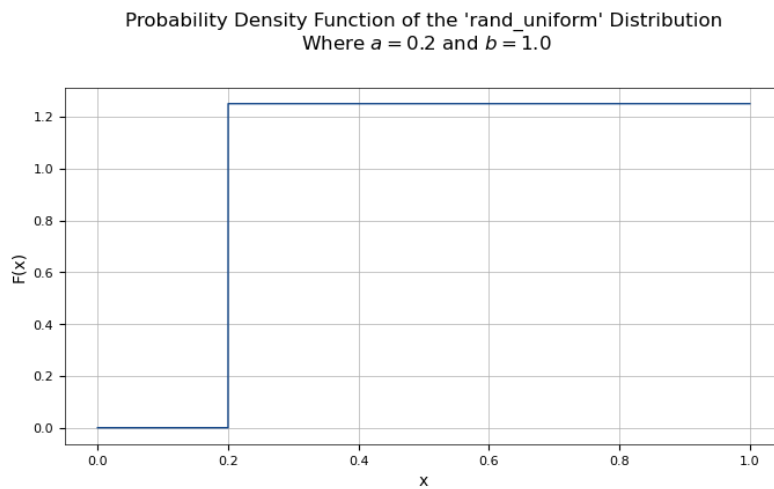
Figure 1: The Plot of the Uniform PDF where a = 0.2 and b = 1.0 in the Real Interval [0.0, 1.0]
