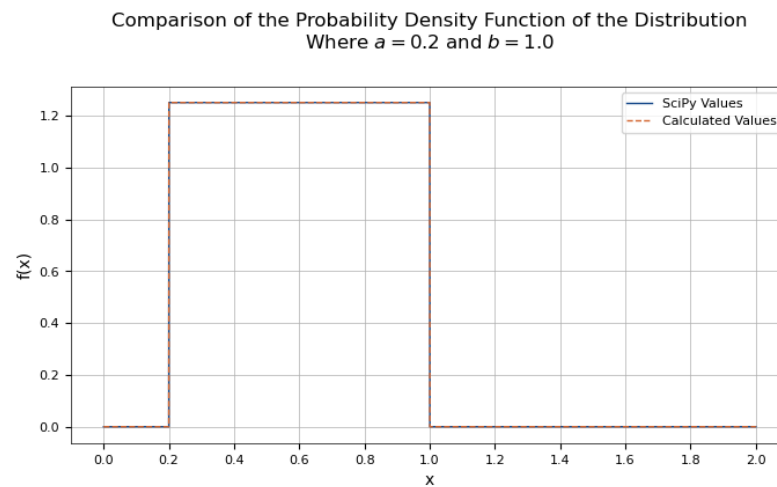
Figure 5: Comparison of the PDF Output from the SciPy library and Direct Calculation for the Uniform Distribution
