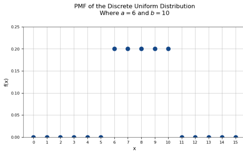
Figure 7: Plot of the Probability Mass Function for the Discrete Uniform Distribution
