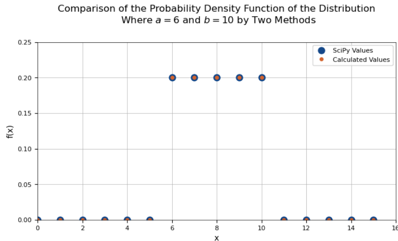
Figure 9: Comparison of the PMF Output from the SciPy library and Direct Calculation for the Discrete Uniform Distribution
