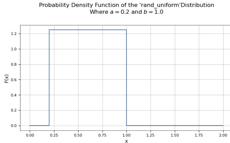
Figure 2: The Plot of the Uniform PDF where a = 0.2 and b = 1.0 in the Real Interval [0.0, 2.0] Showing the Characteristic Rectangular Shape
