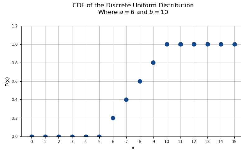
Figure 8: Plot of the Cumulative Distribution Function for the Discrete Uniform Distribution
