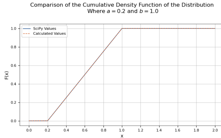
Figure 6: Comparison of the CDF Output from the SciPy library and Direct Calculation for the Uniform Distribution
