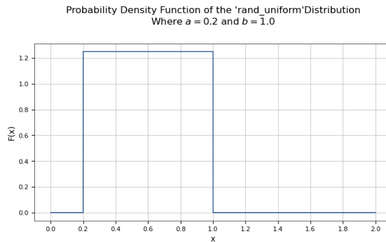
Figure 3: The Plot of the Uniform PDF where a = 0.2 and b = 1.0 in the Real Interval [0.0, 2.0] Using Revised Tick Markers
