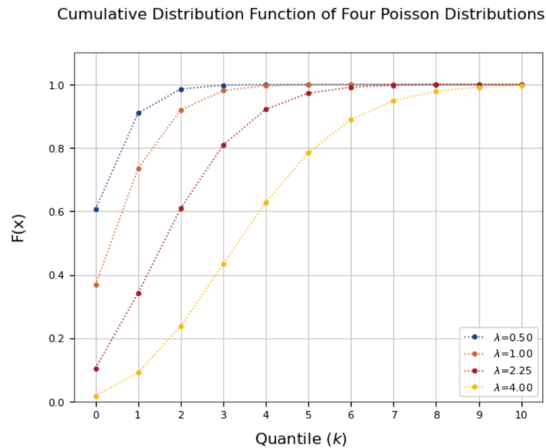
Figure 4: Plot of the CDF Values of the Quantiles for Four Poisson Distributions
