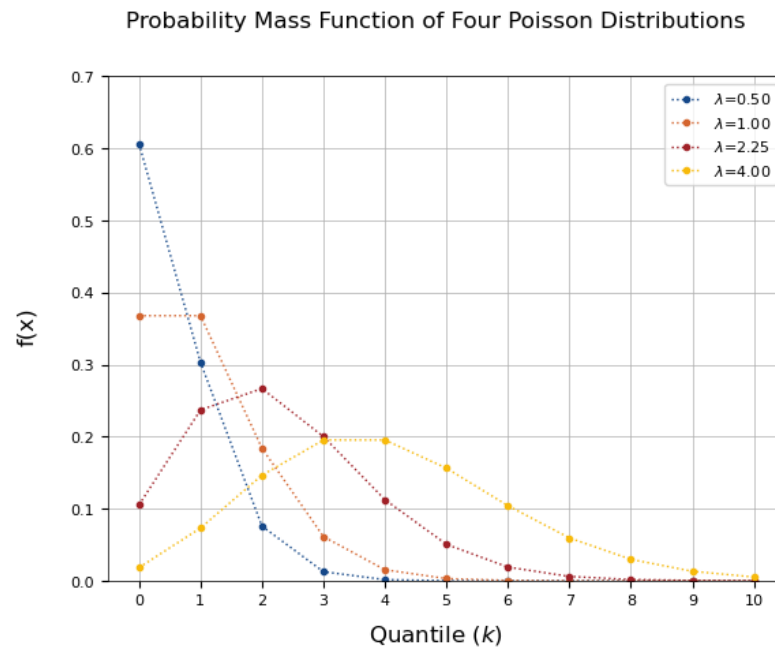
Figure 3: Plot of the PMF Values of the Quantiles for Four Poisson Distributions
