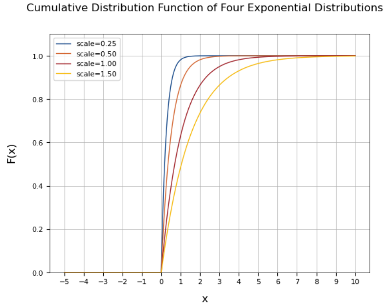
Figure 7: Plot of the CDF Values of Different Scales for Four Standard Exponential Distributions
