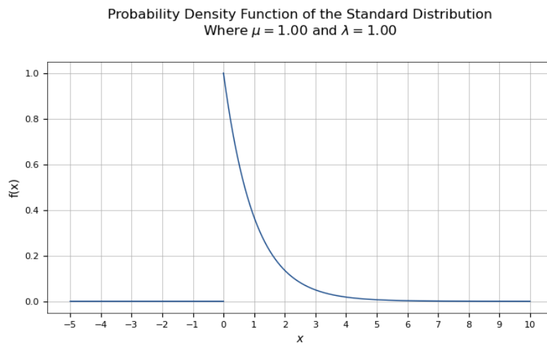
Figure 3: A Plot of the Standard Exponential PDF where \mu = 1 and \lambda = 1 in the Real Interval [-5.0, 10.0] , Showing the Expected Discontinuity
