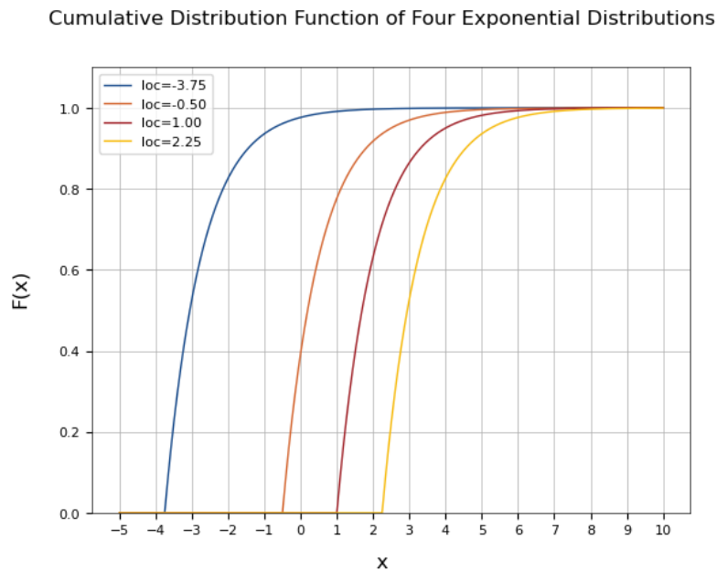
Figure 5: Plot of the CDF Values of the Locations for Four Standard Exponential Distributions
