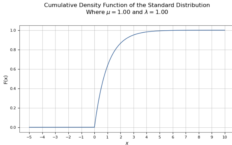
Figure 2: The Plot of the Standard Exponential CDF where \mu = 1 and \lambda = 1 in the Real Interval [-5.0, 10.0]
