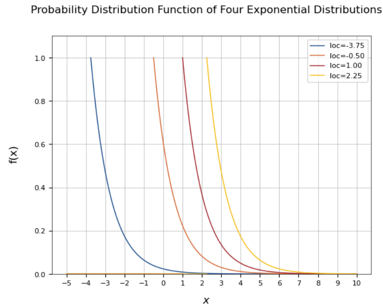
Figure 4: Plot of the PDF Values of the Locations for Four Standard Exponential Distributions
