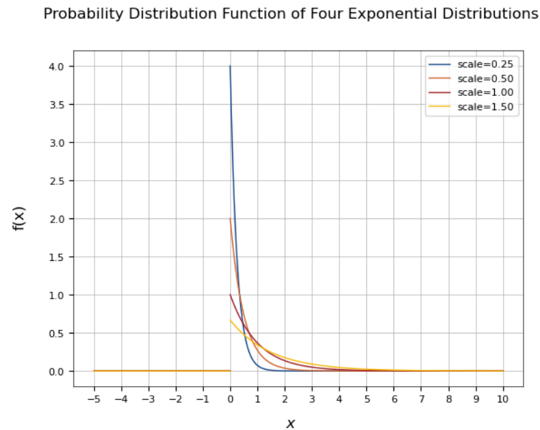
Figure 6: Plot of the PDF Values of Different Scales for Four Standard Exponential Distributions
