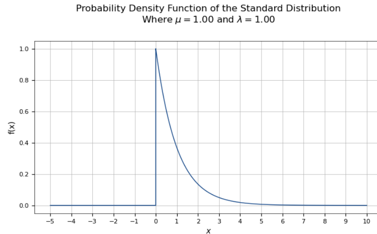
Figure 1: A Quick Plot of the Standard Exponential PDF where \mu = 1 and \lambda = 1 in the Real Interval [-5.0, 10.0]
