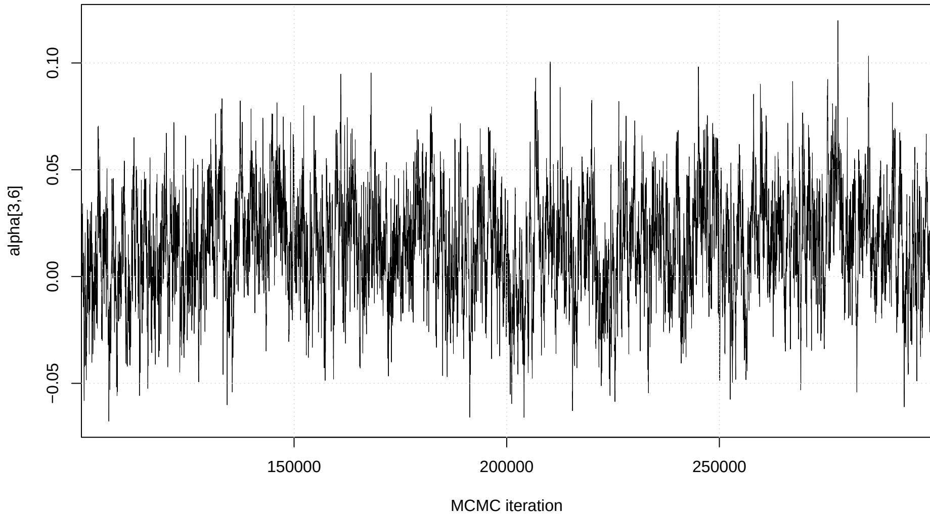
Trace plot: alpha[3,6]
