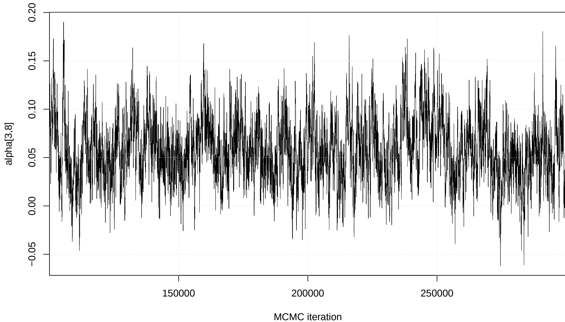
Trace plot: alpha[3,8]
