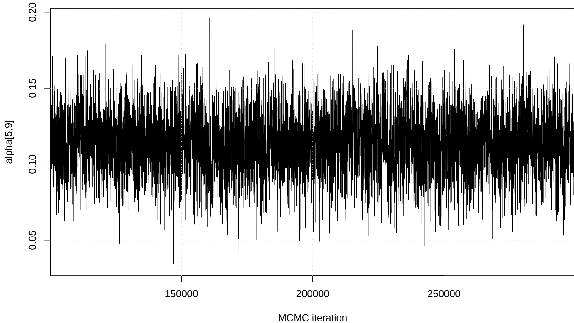
Trace plot: alpha[5,9]
