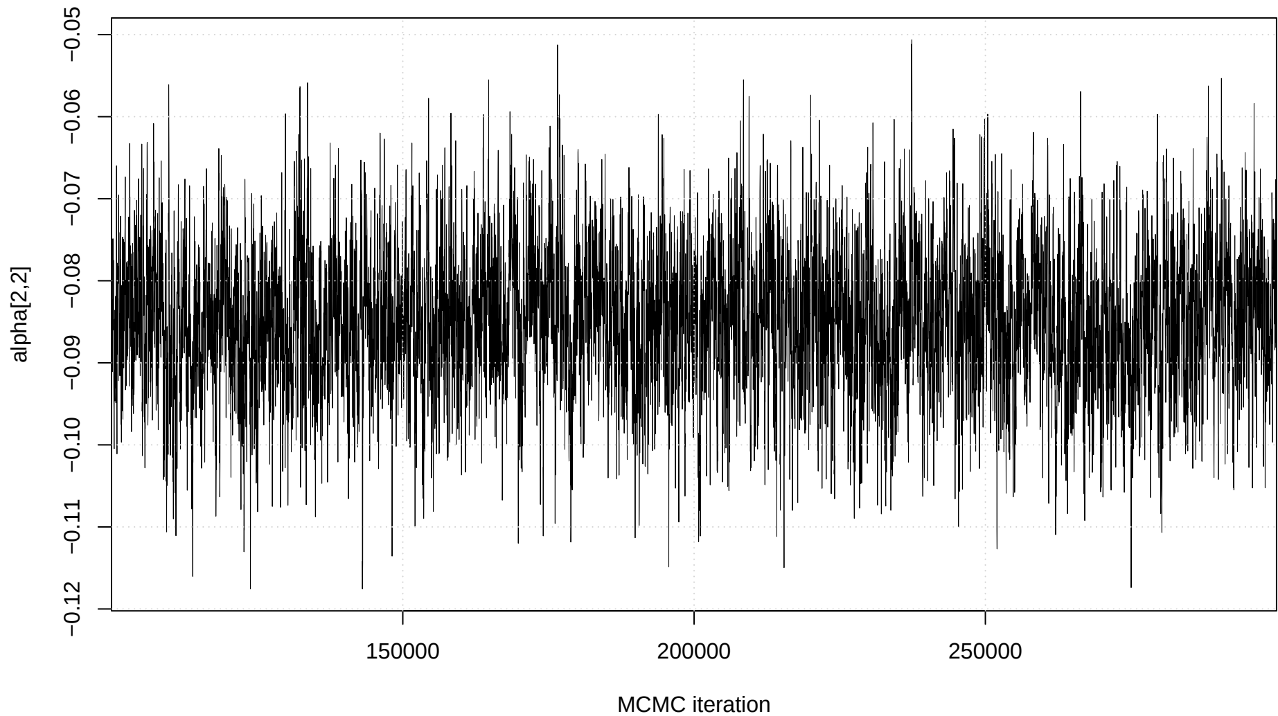
Trace plot: alpha[2,2]
