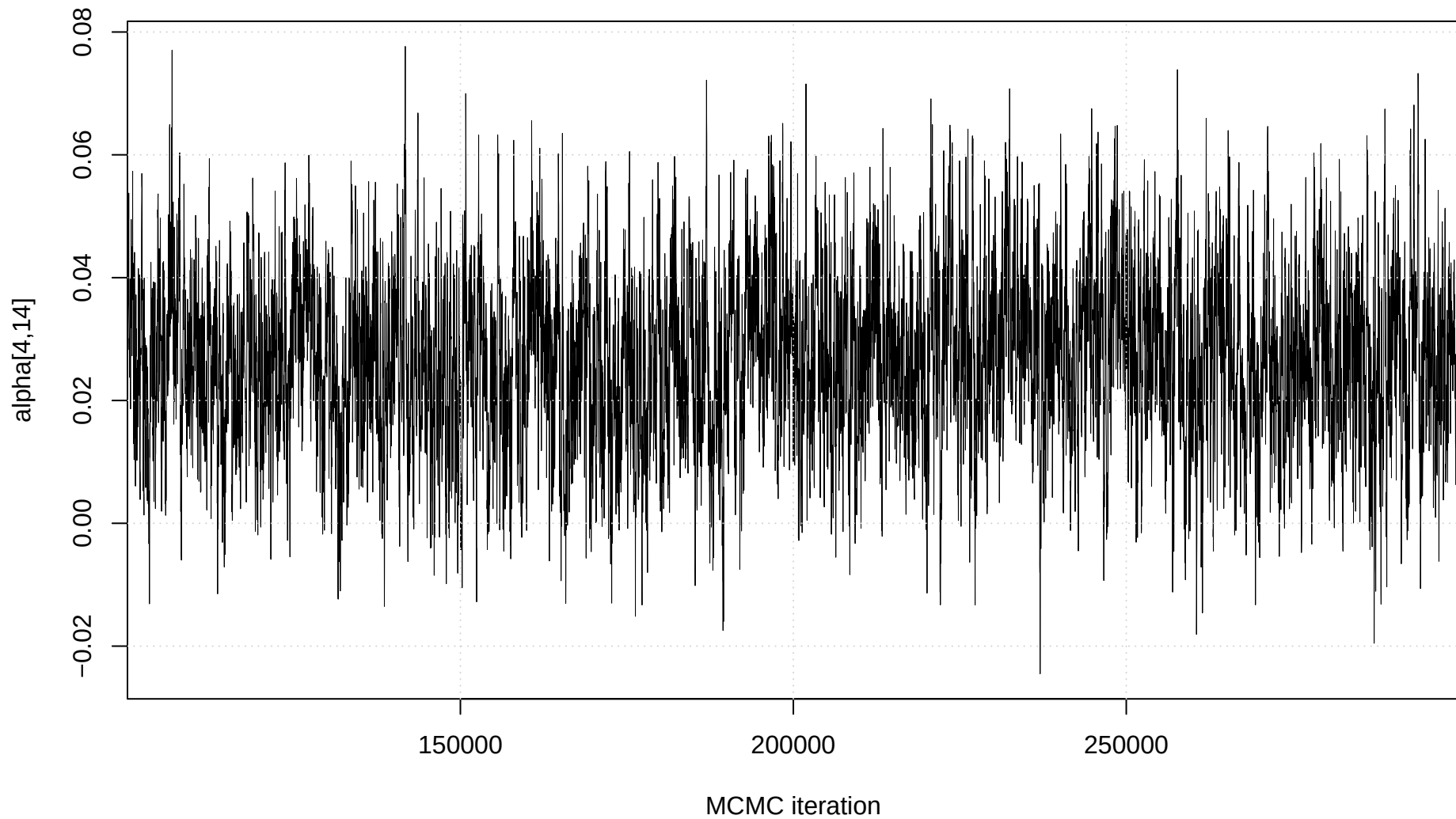
Trace plot: alpha[4,14]
