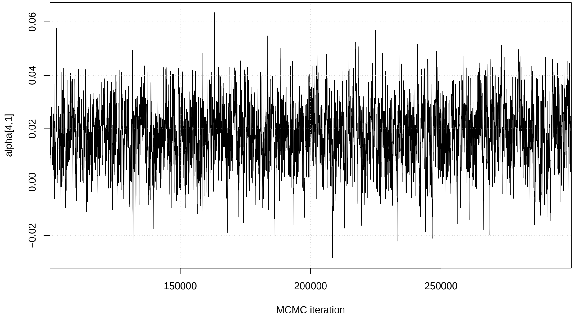
Trace plot: alpha[4,1]
