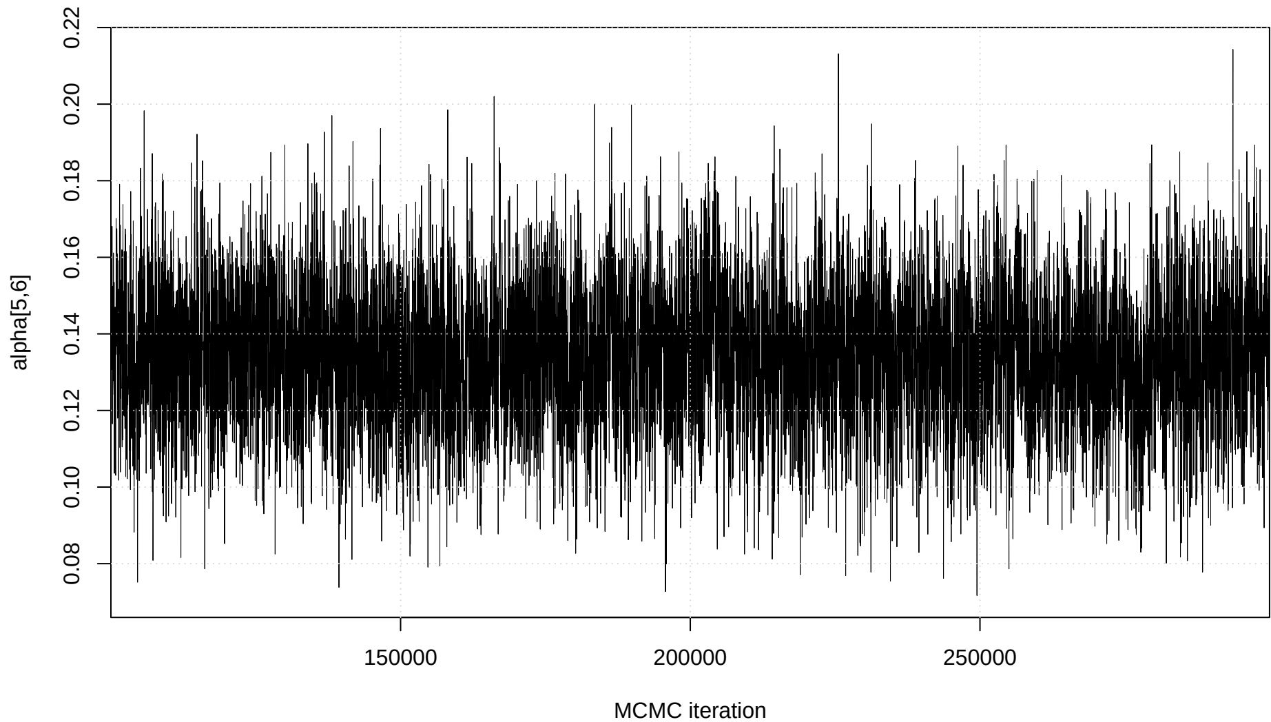
Trace plot: alpha[5,6]
