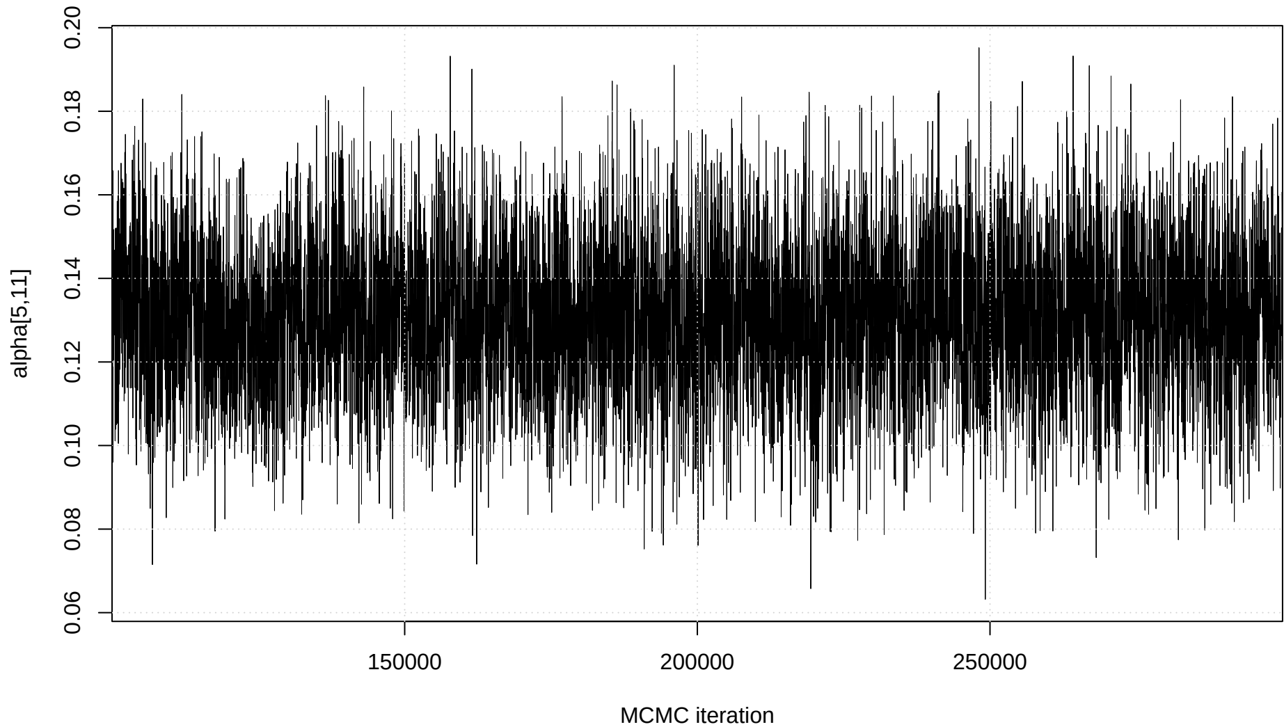
Trace plot: alpha[5,11]
