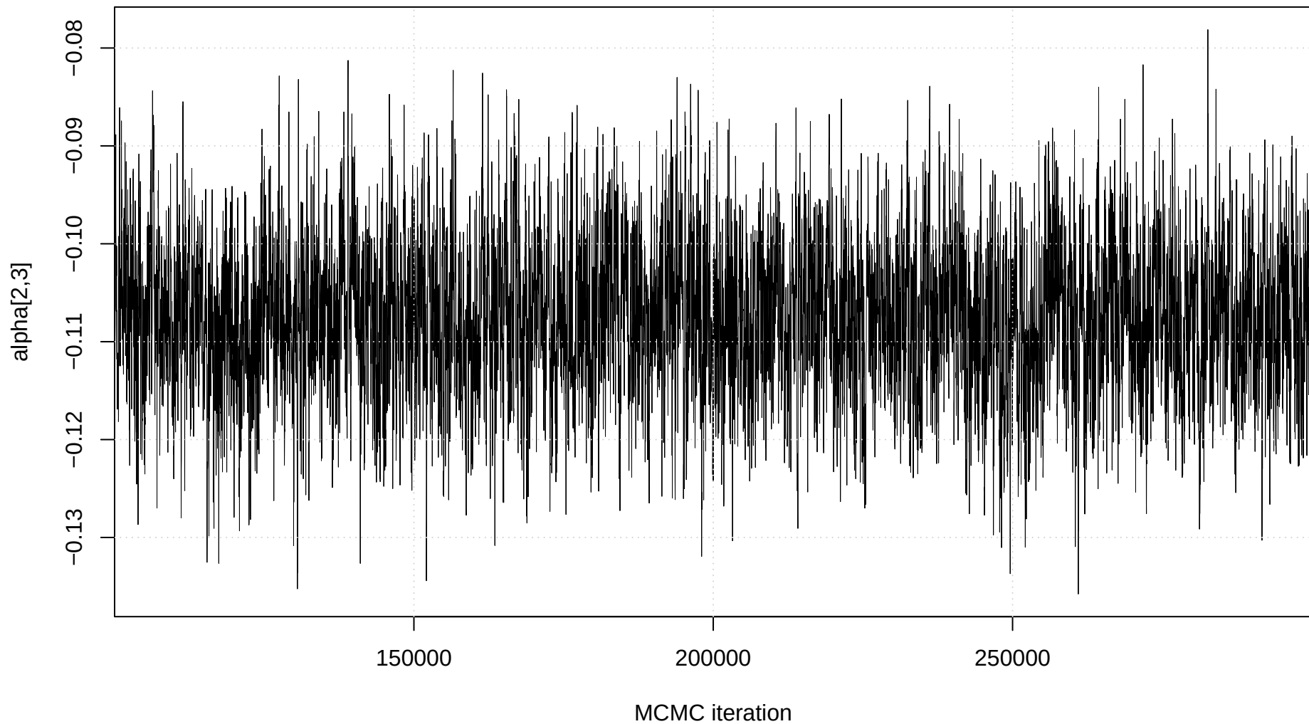
Trace plot: alpha[2,3]
