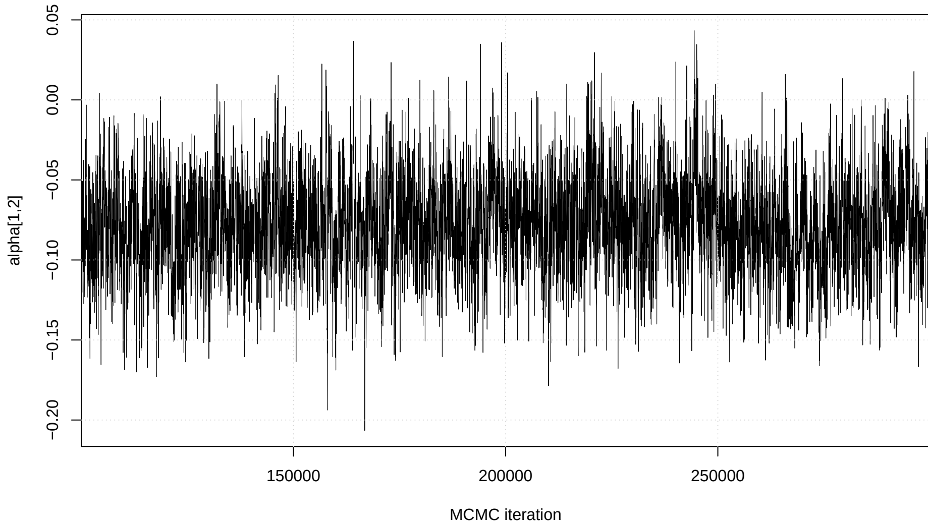
Trace plot: alpha[1,2]
