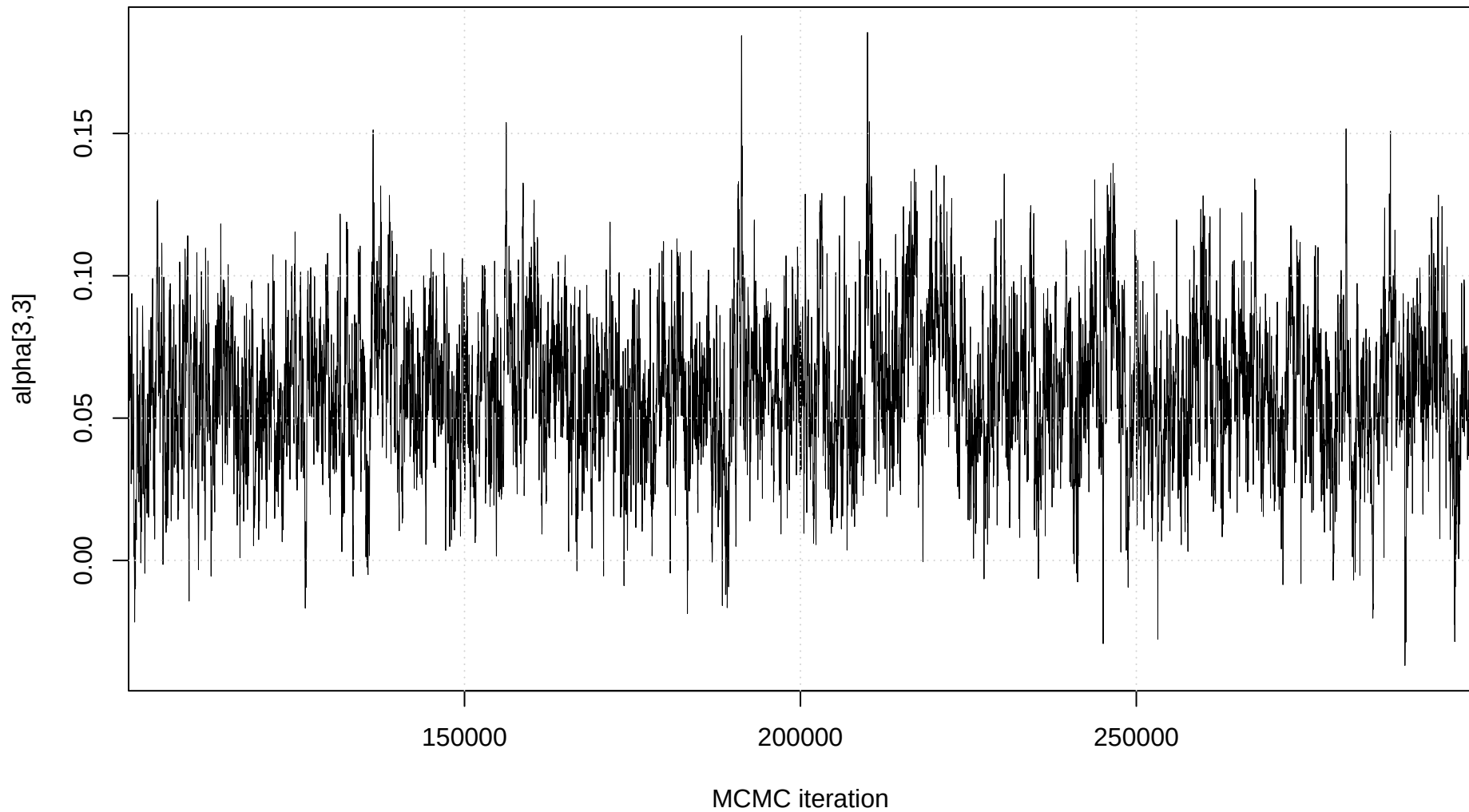
Trace plot: alpha[3,3]
