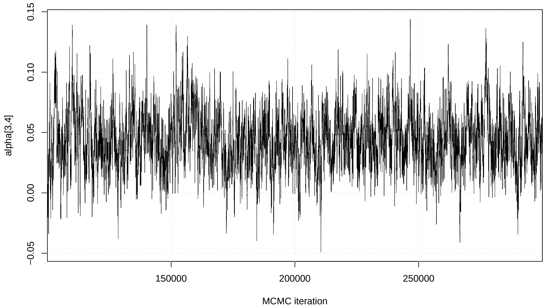
Trace plot: alpha[3,4]
