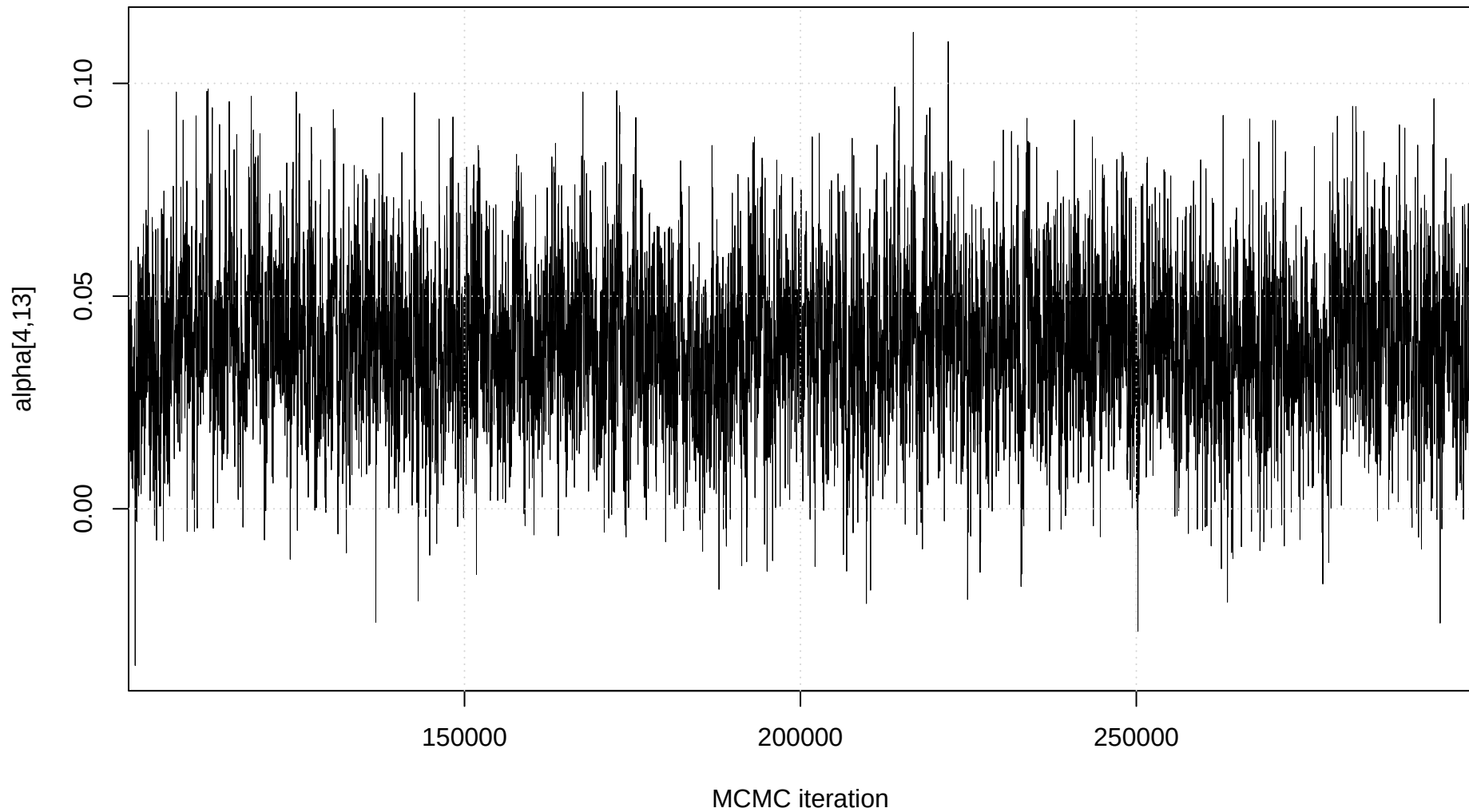
Trace plot: alpha[4,13]
