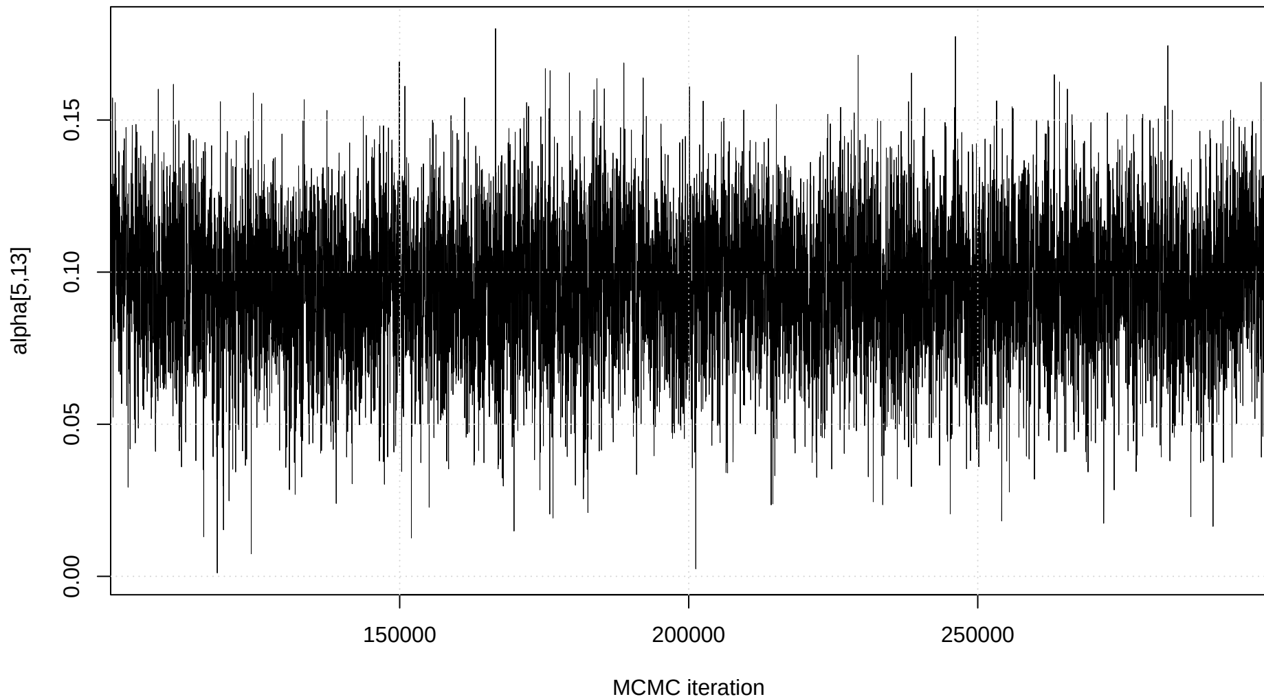
Trace plot: alpha[5,13]
