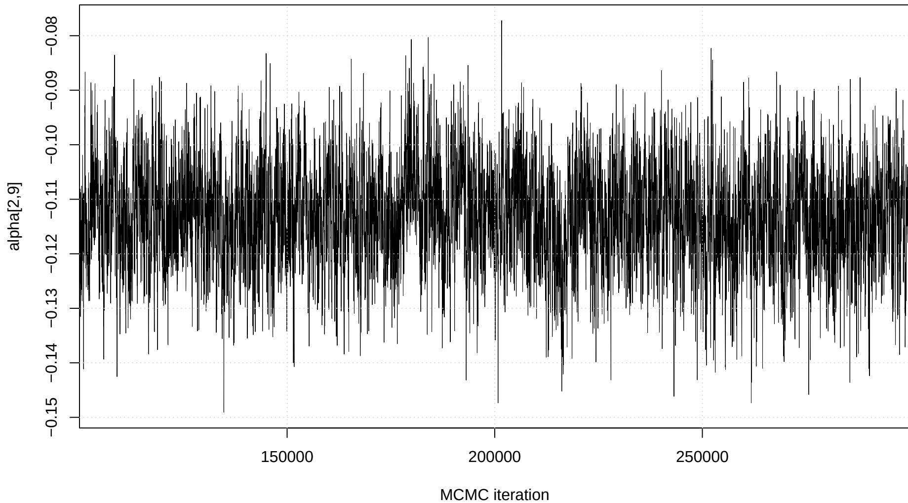
Trace plot: alpha[2,9]
