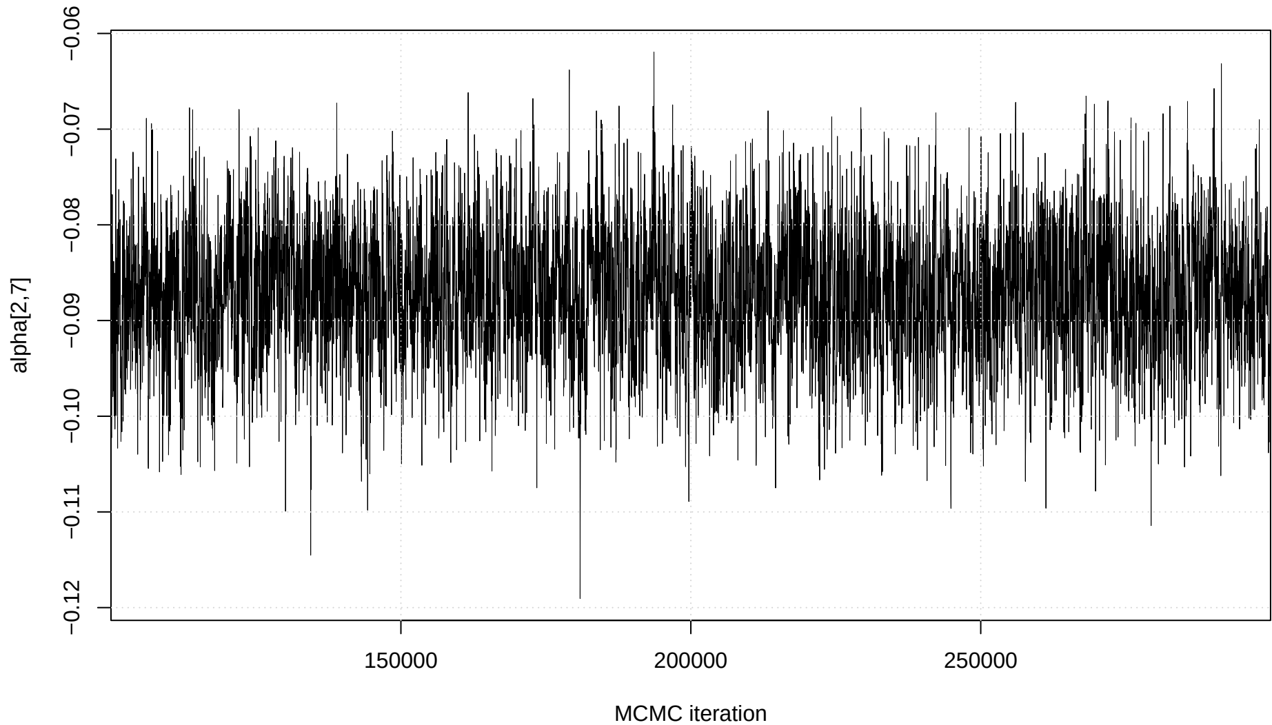
Trace plot: alpha[2,7]
