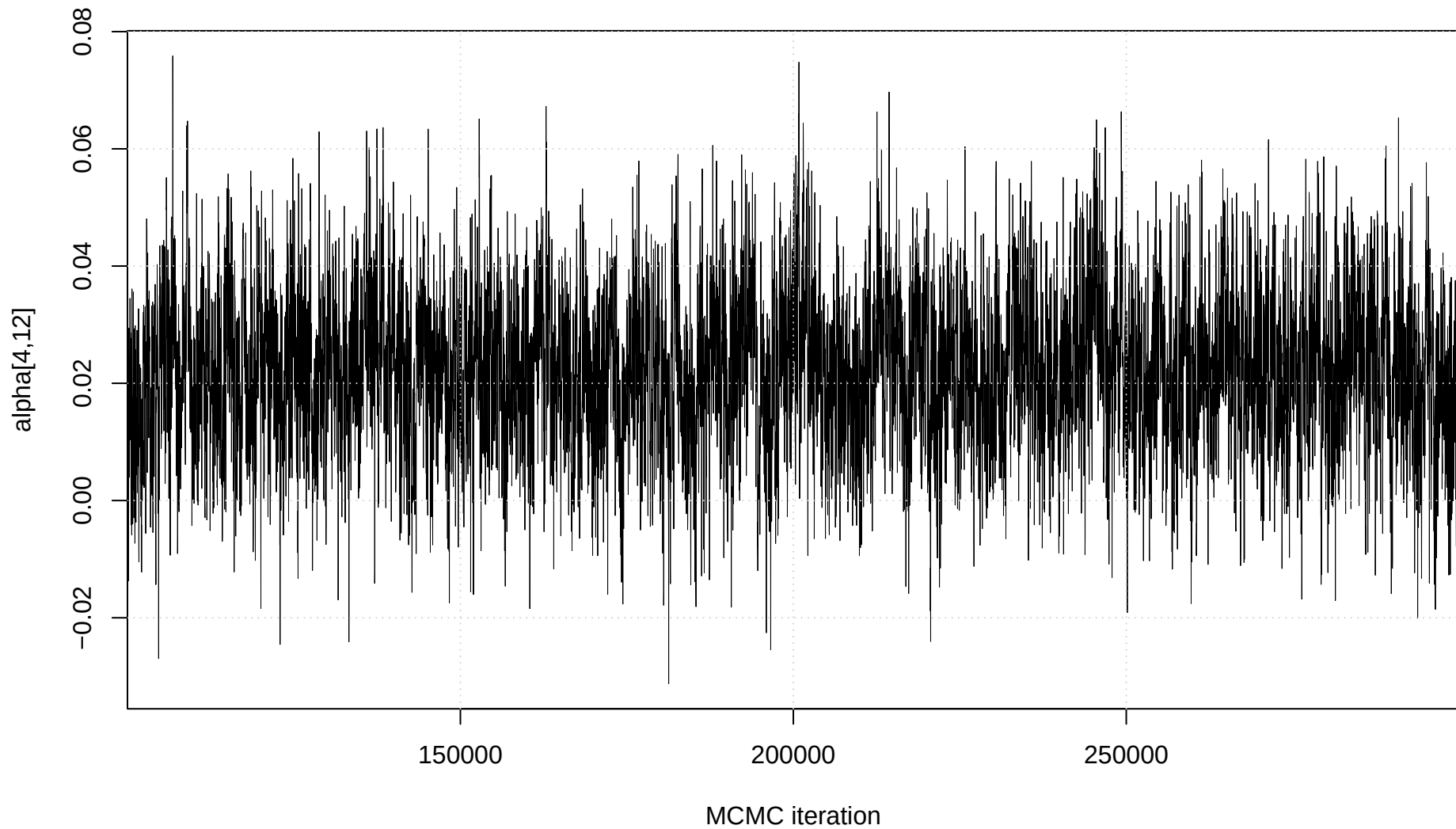
Trace plot: alpha[4,12]
