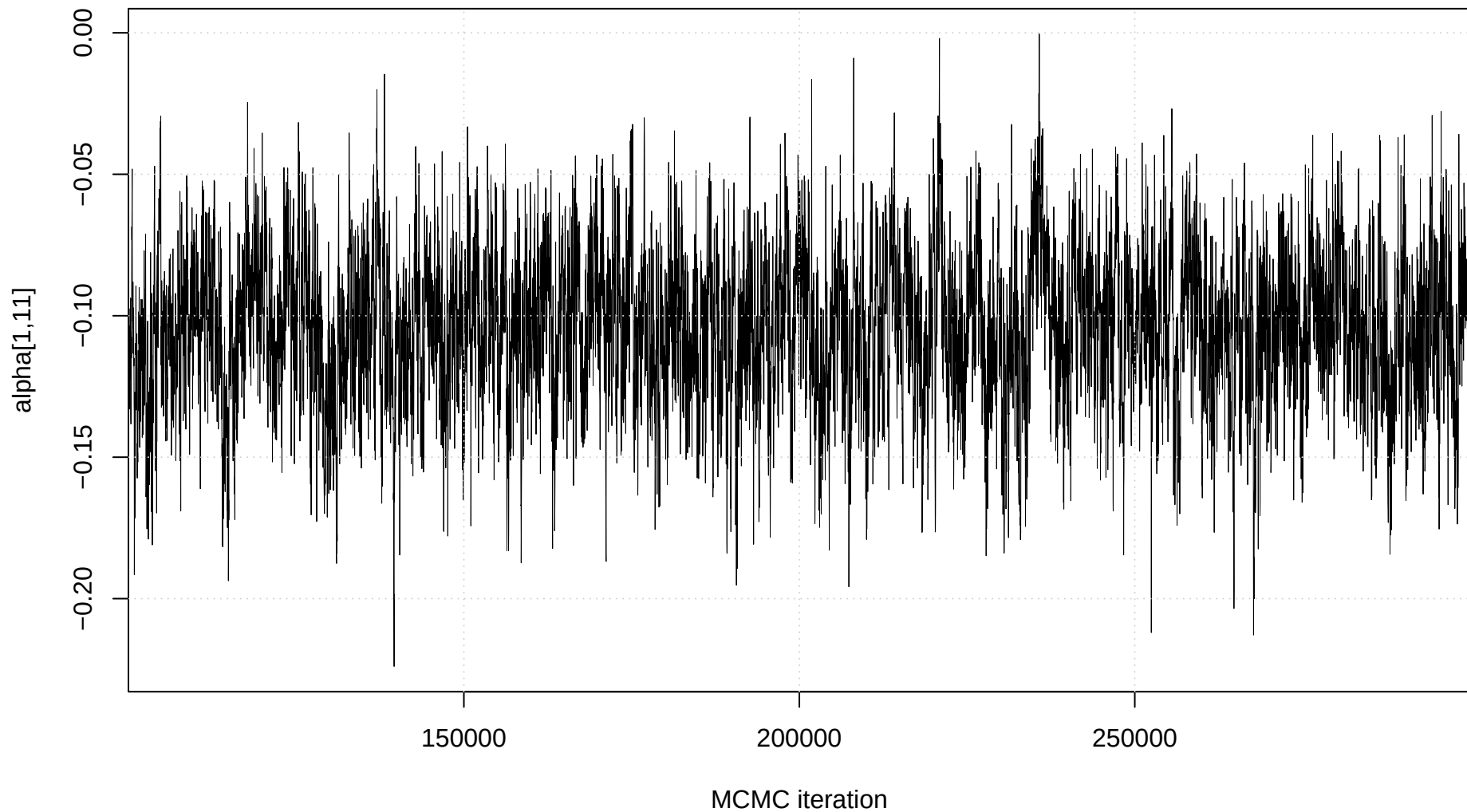
Trace plot: alpha[1,11]
