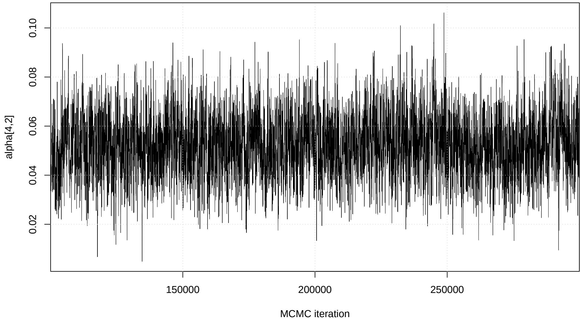
Trace plot: alpha[4,2]
