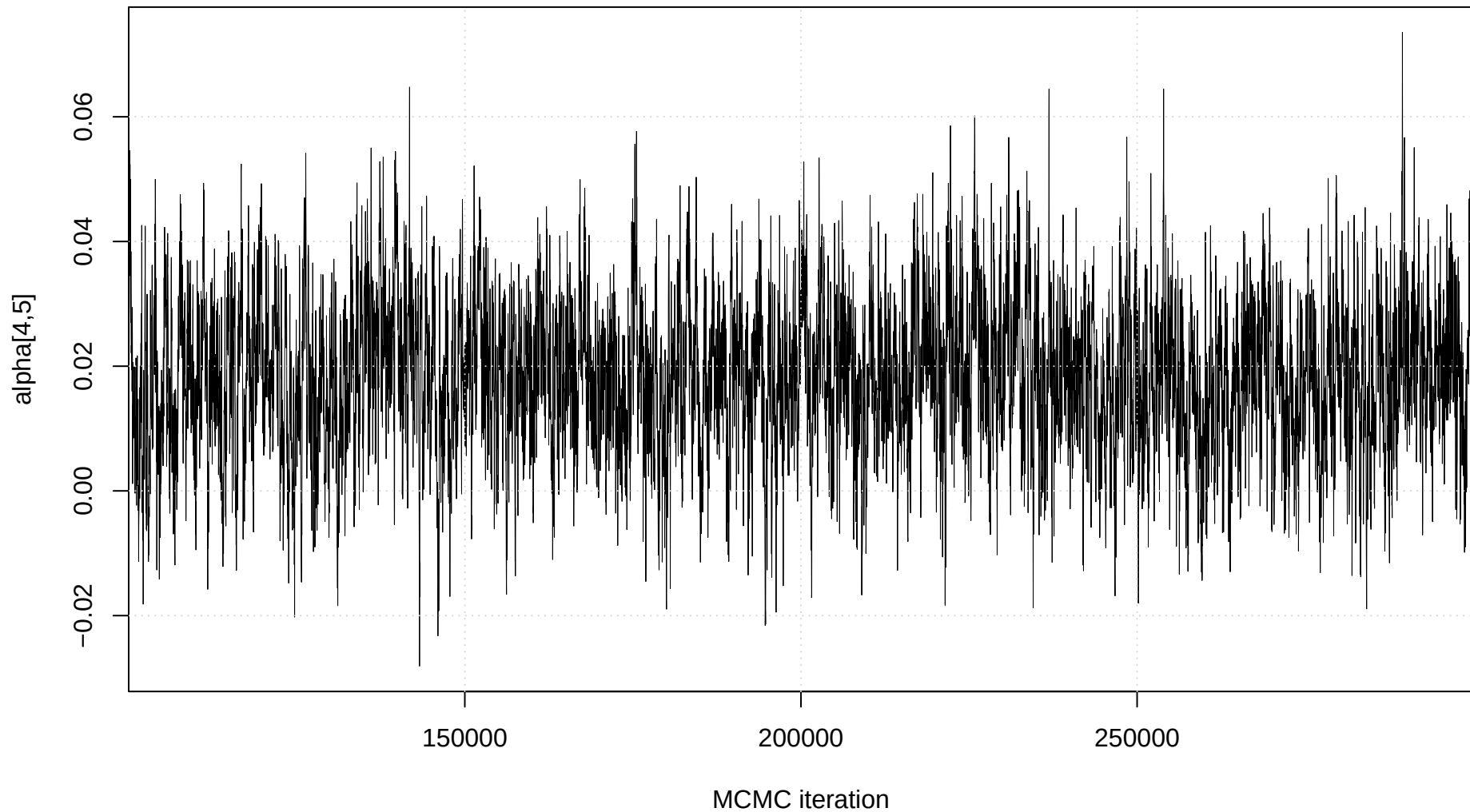
Trace plot: alpha[4,5]
