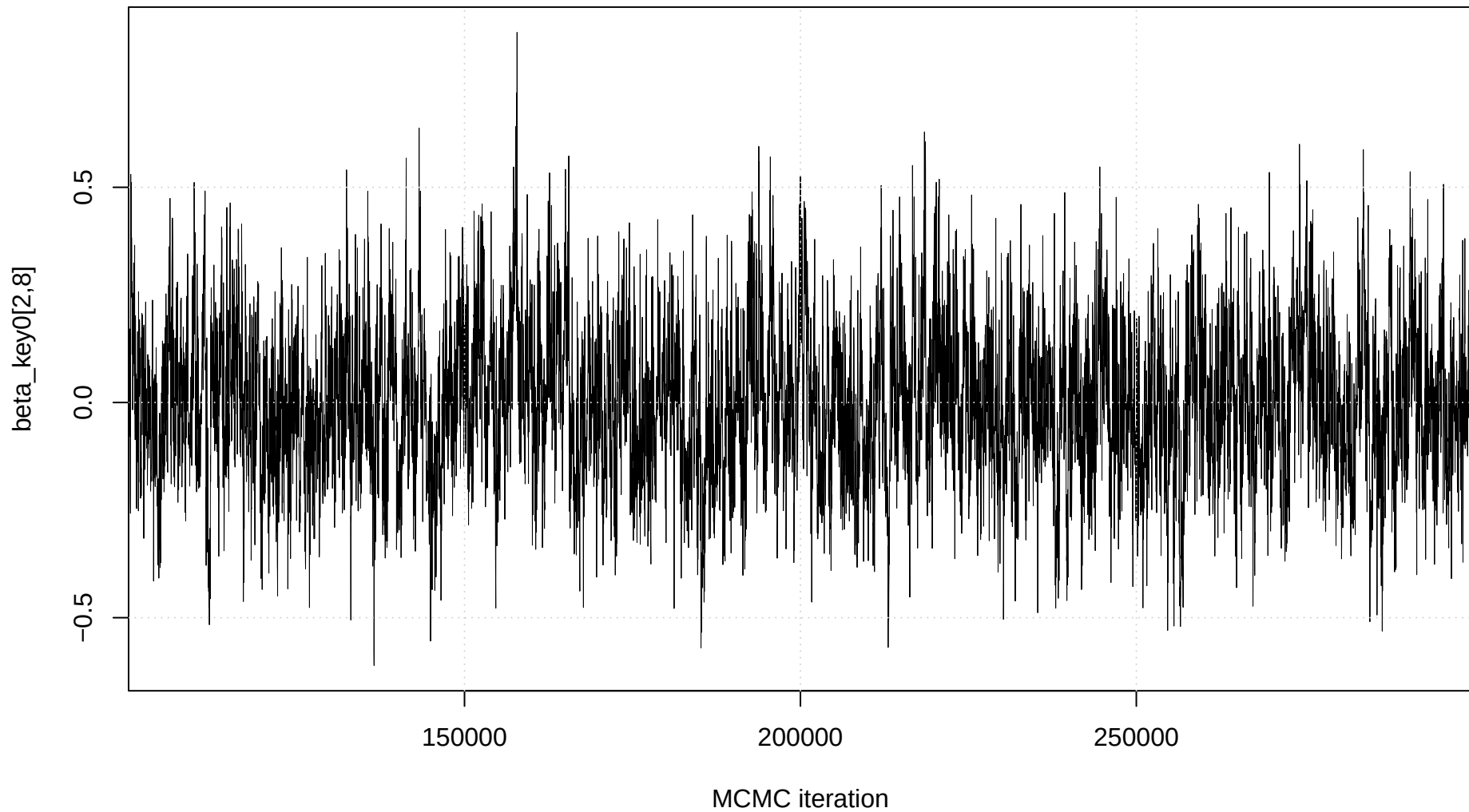
Trace plot: beta_key0[2,8]
