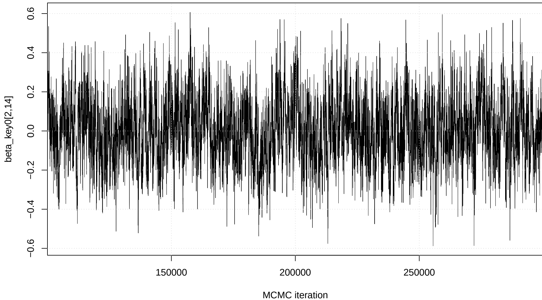
Trace plot: beta_key0[2,14]
