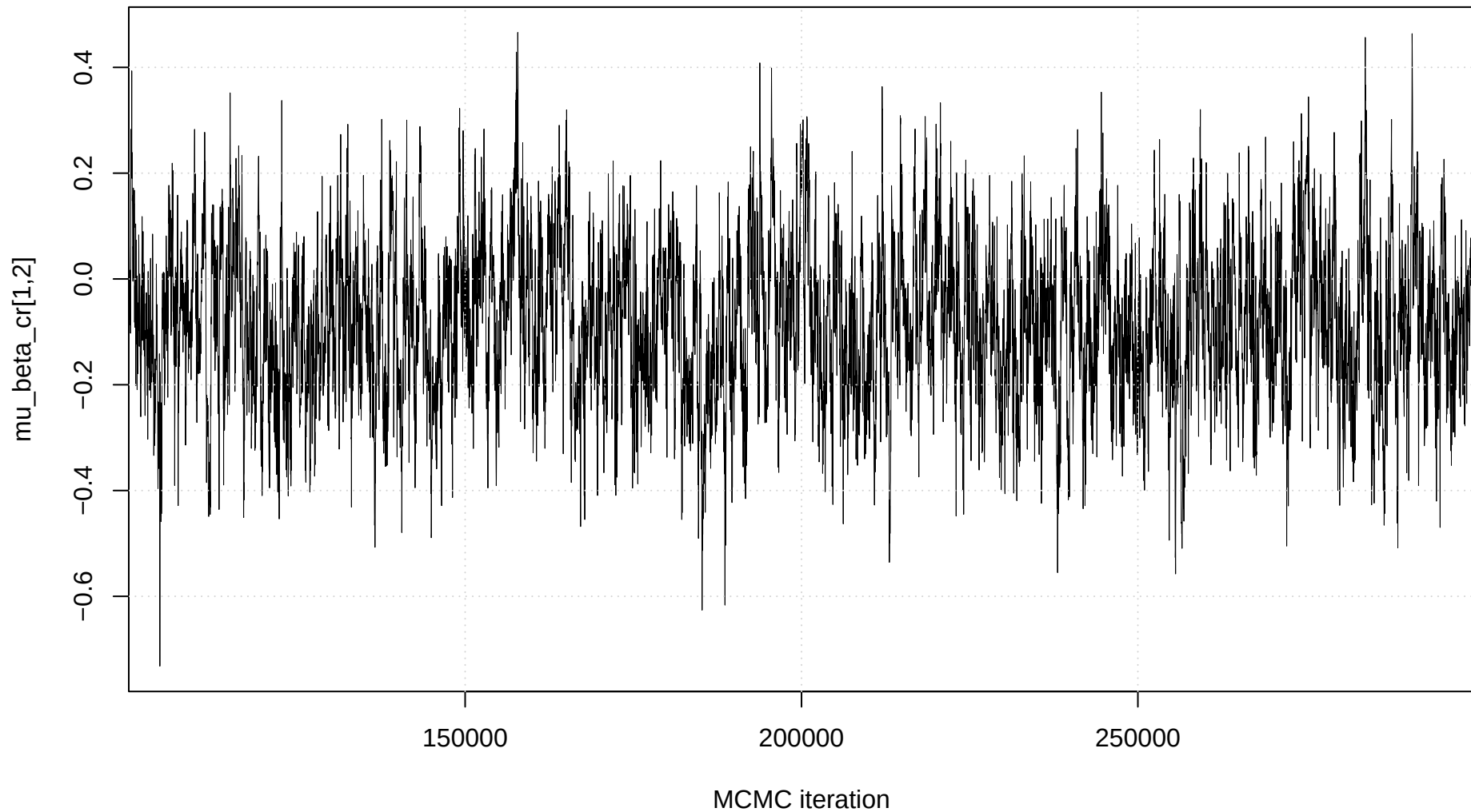
Trace plot: mu_beta_cr[1,2]
