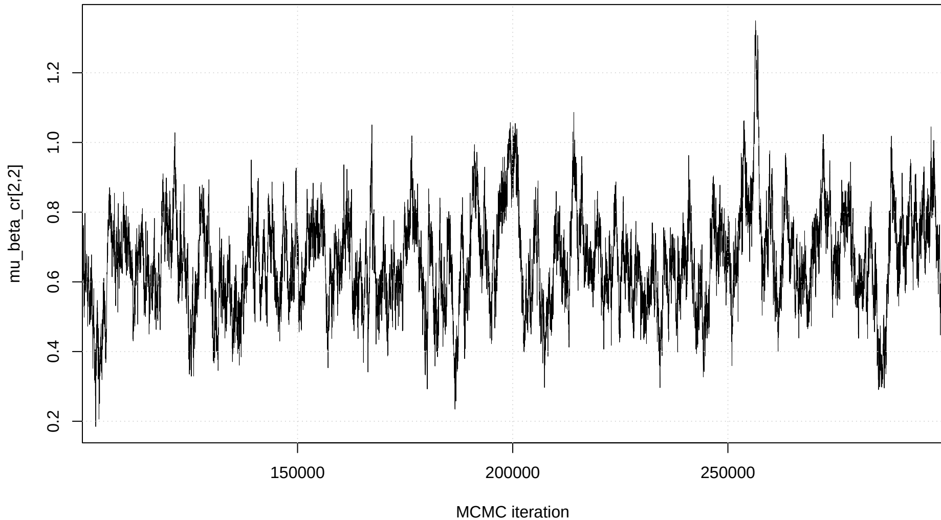
Trace plot: mu_beta_cr[2,2]
