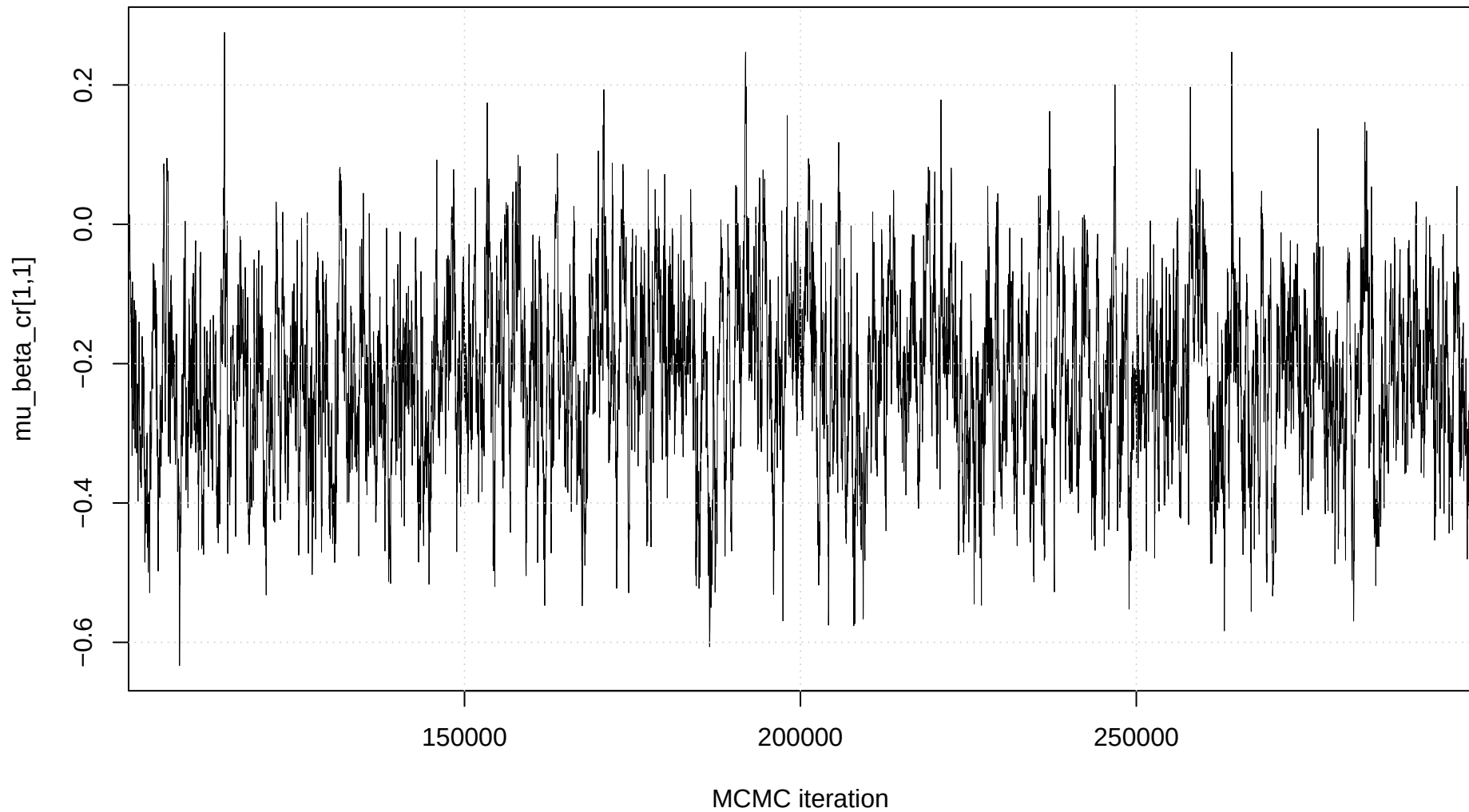
Trace plot: mu_beta_cr[1,1]
