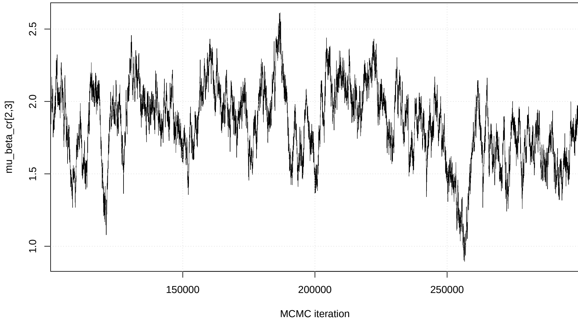
Trace plot: mu_beta_cr[2,3]
