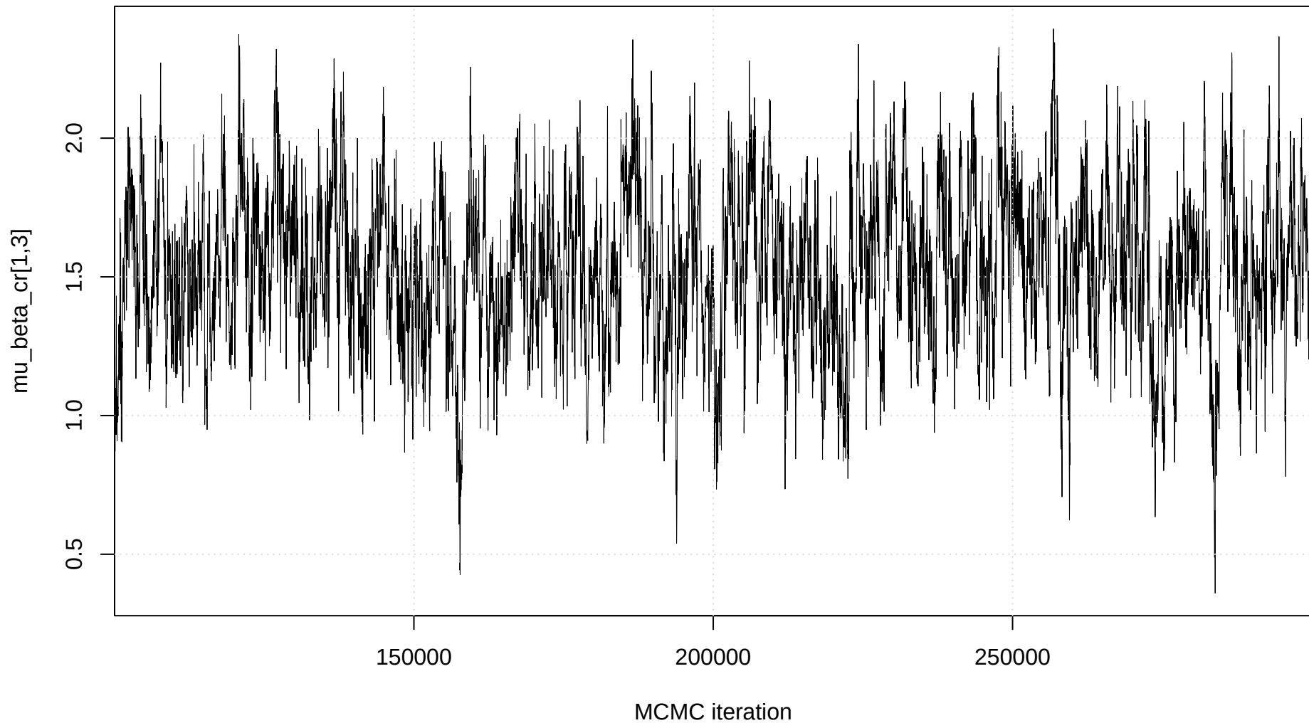
Trace plot: mu_beta_cr[1,3]
