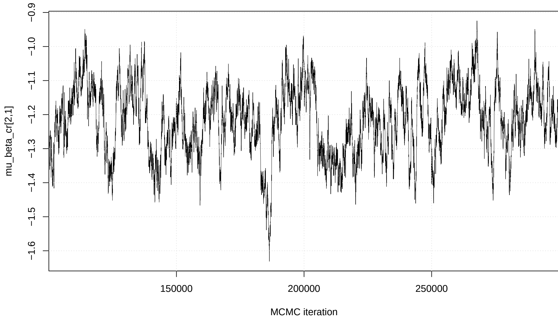
Trace plot: mu_beta_cr[2,1]
