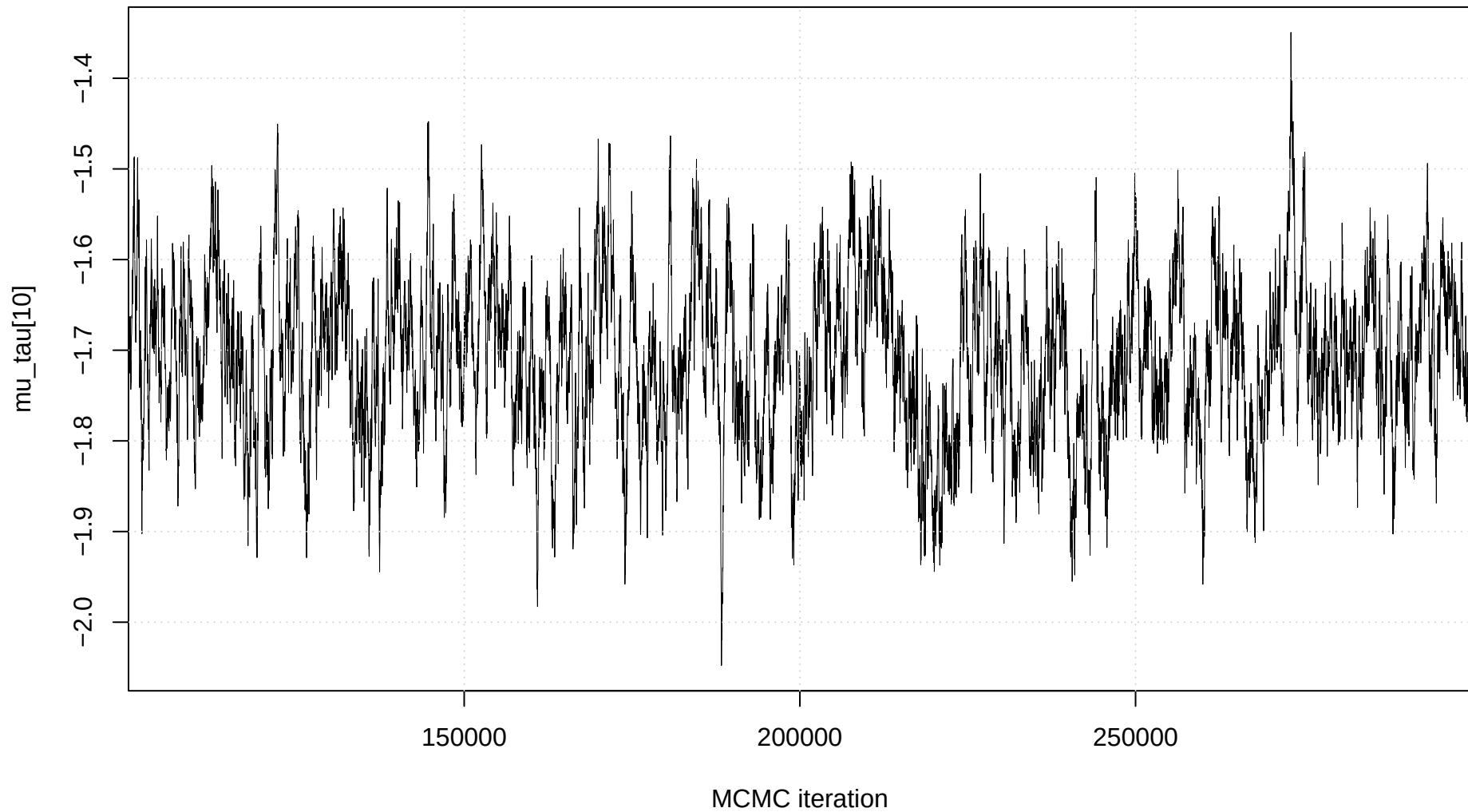
Trace plot: \mu_{\text{tau}}[10]
