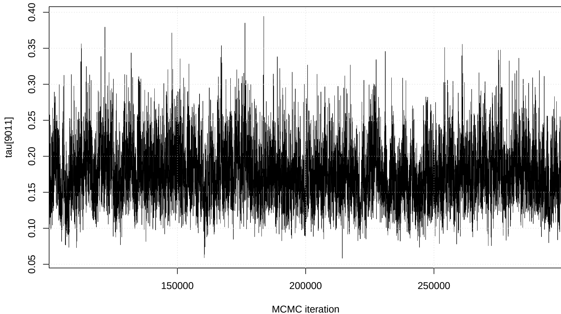
Trace plot: tau[9011]
