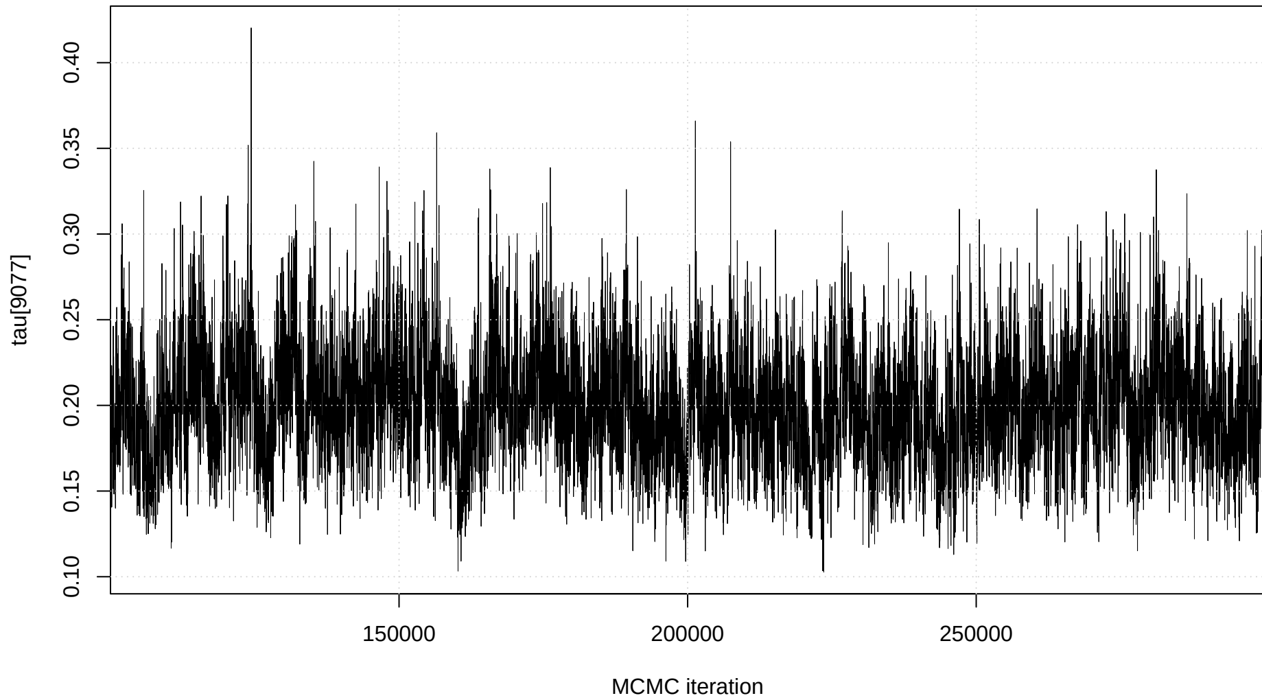
Trace plot: tau[9077]
