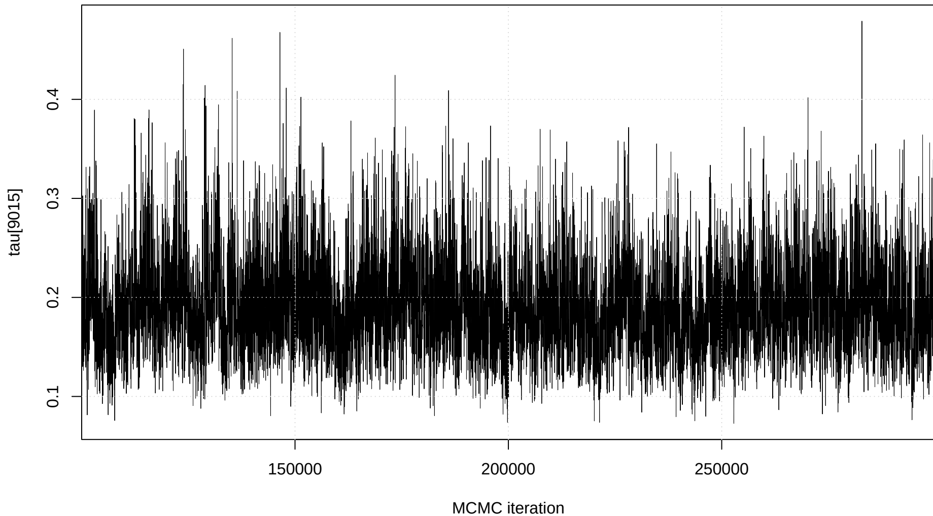
Trace plot: tau[9015]
