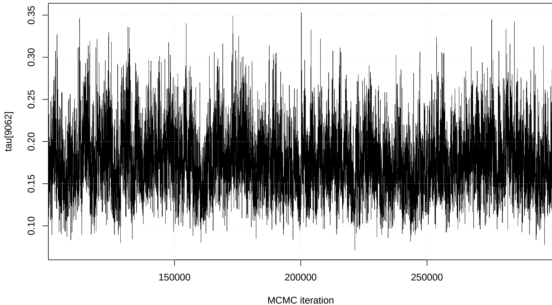
Trace plot: tau[9062]
