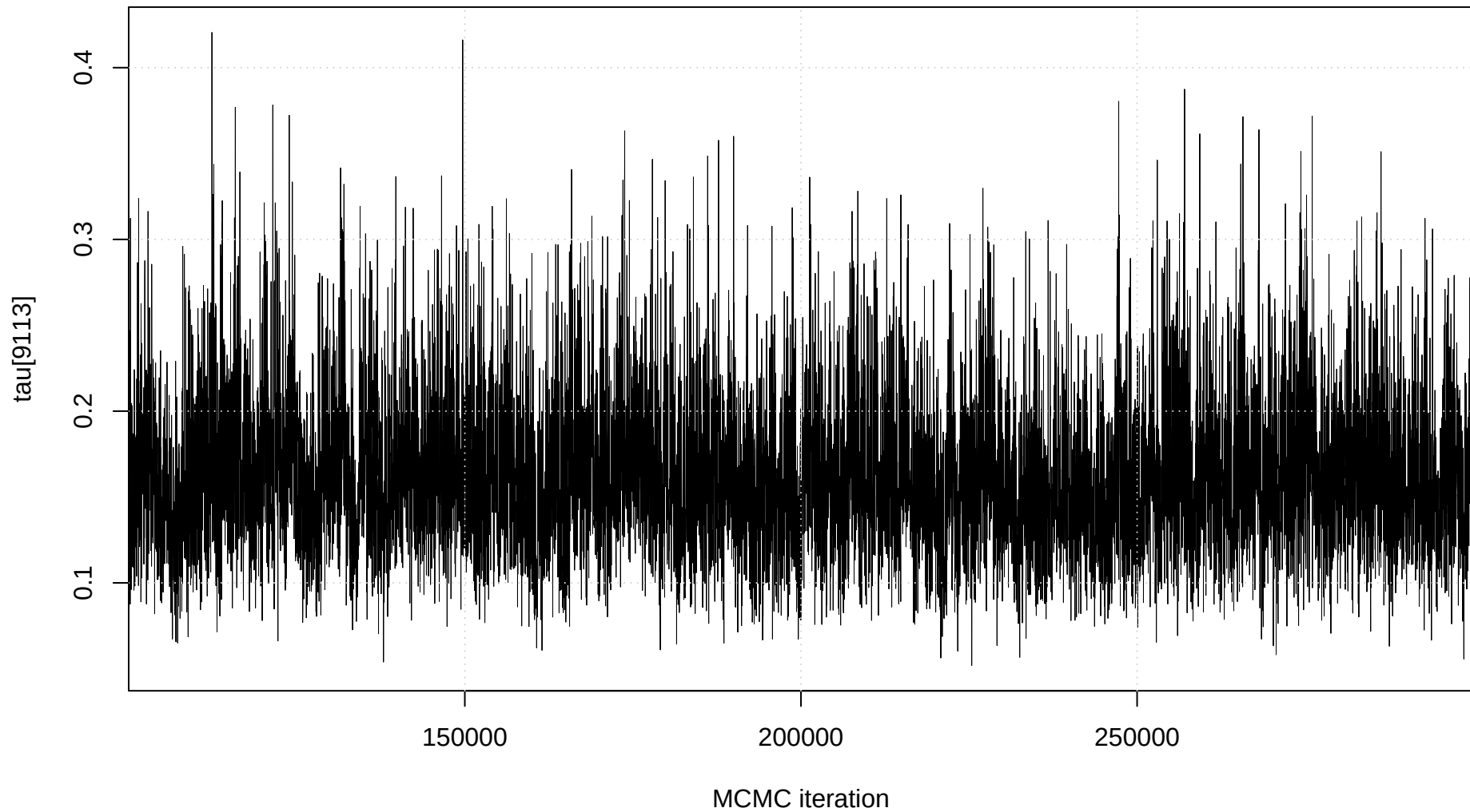
Trace plot: tau[9113]
