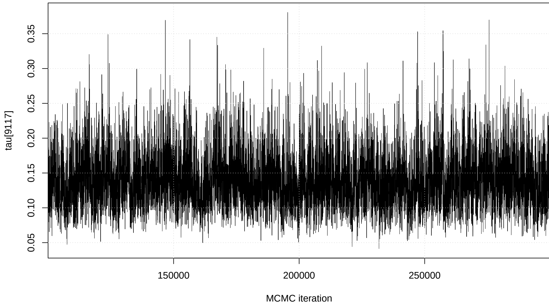
Trace plot: tau[9117]
