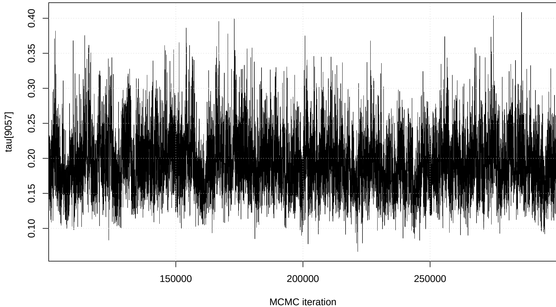
Trace plot: tau[9057]
