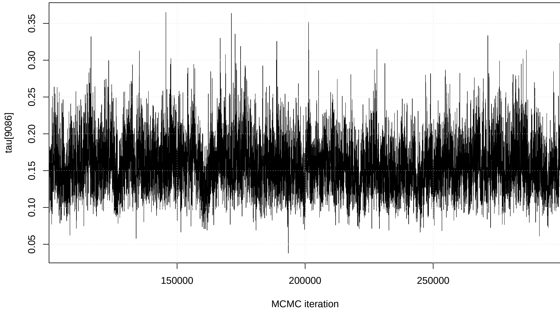
Trace plot: tau[9086]
