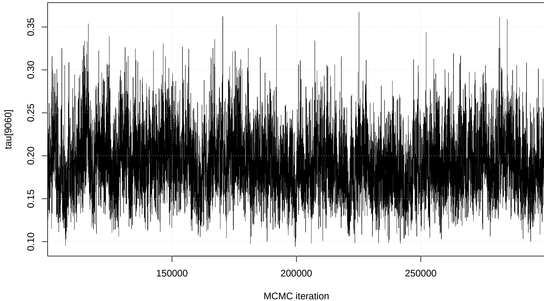
Trace plot: tau[9060]
