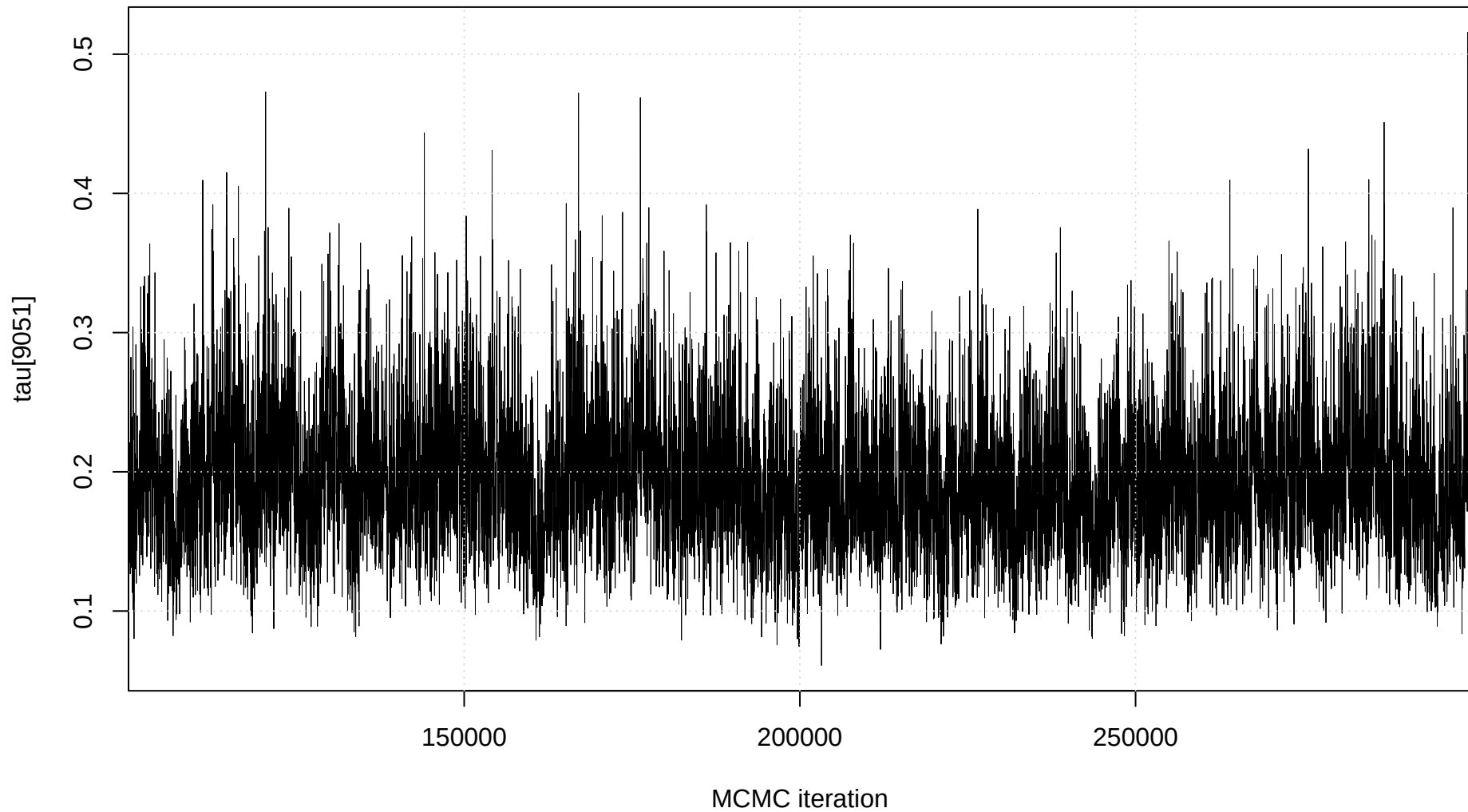
Trace plot: tau[9051]
