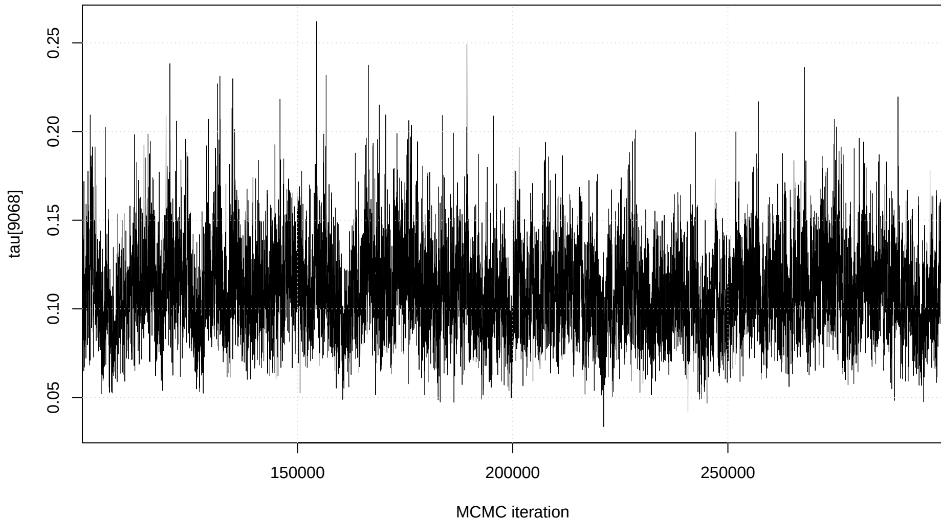
Trace plot: tau[9068]
