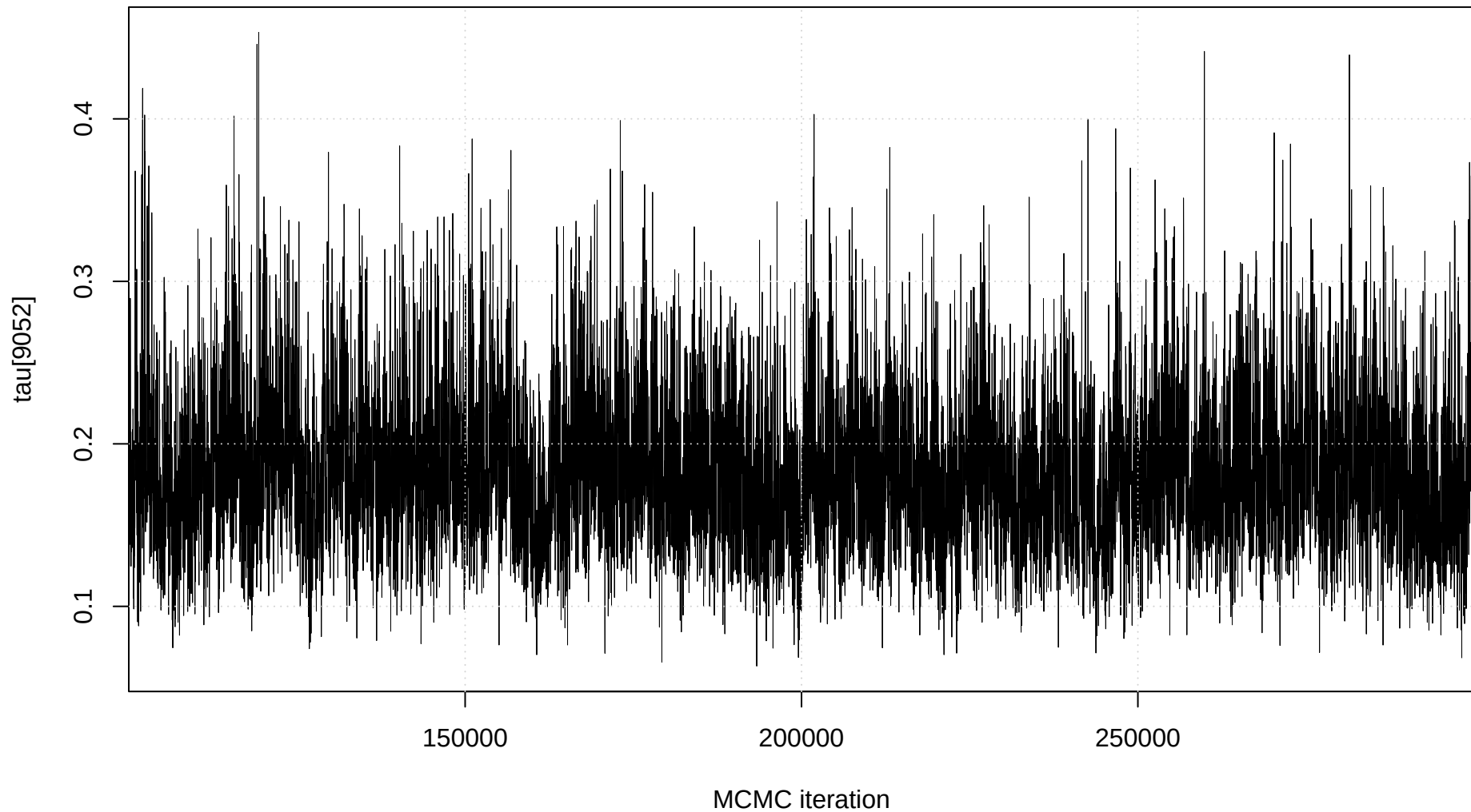
Trace plot: tau[9052]
