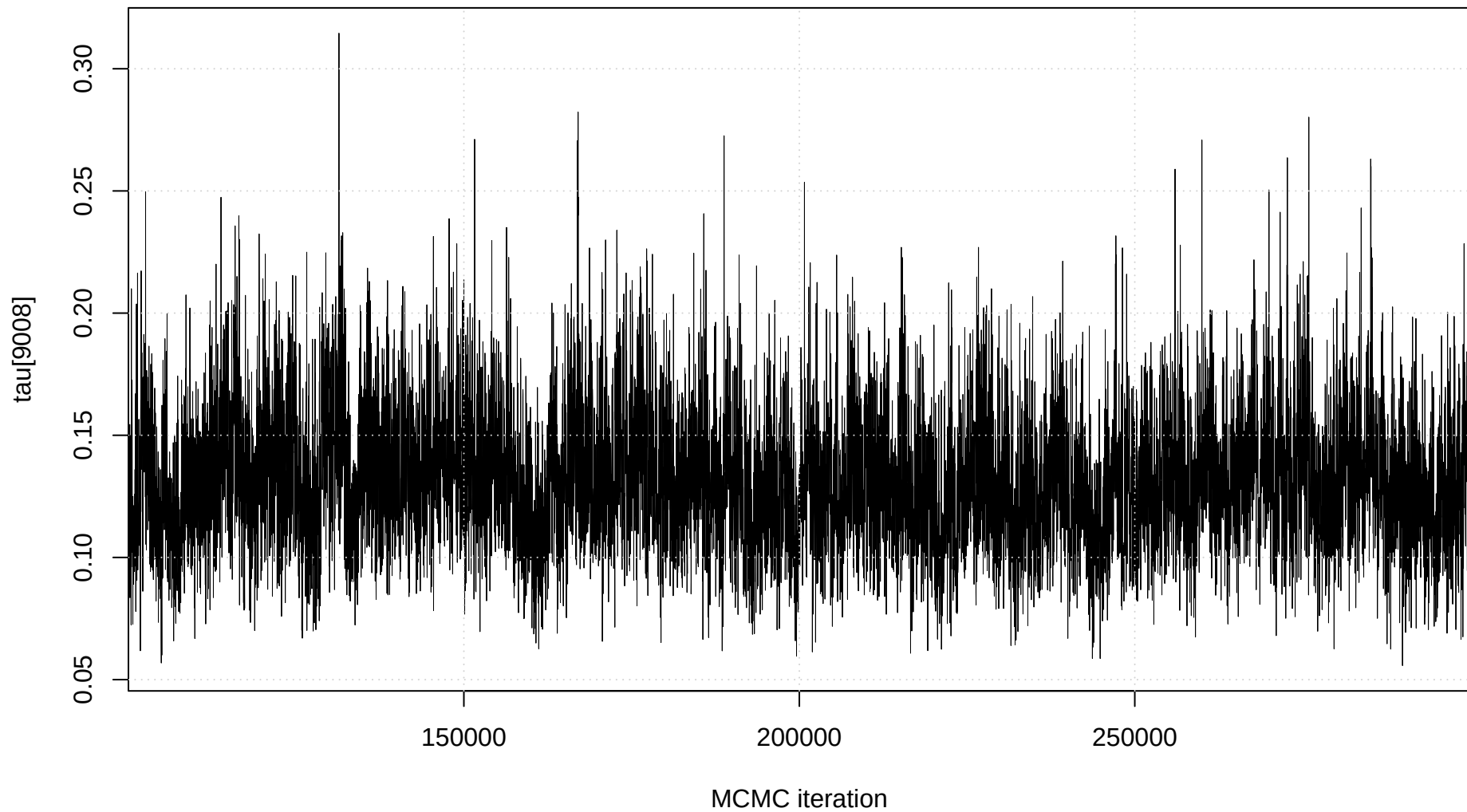
Trace plot: tau[9008]
