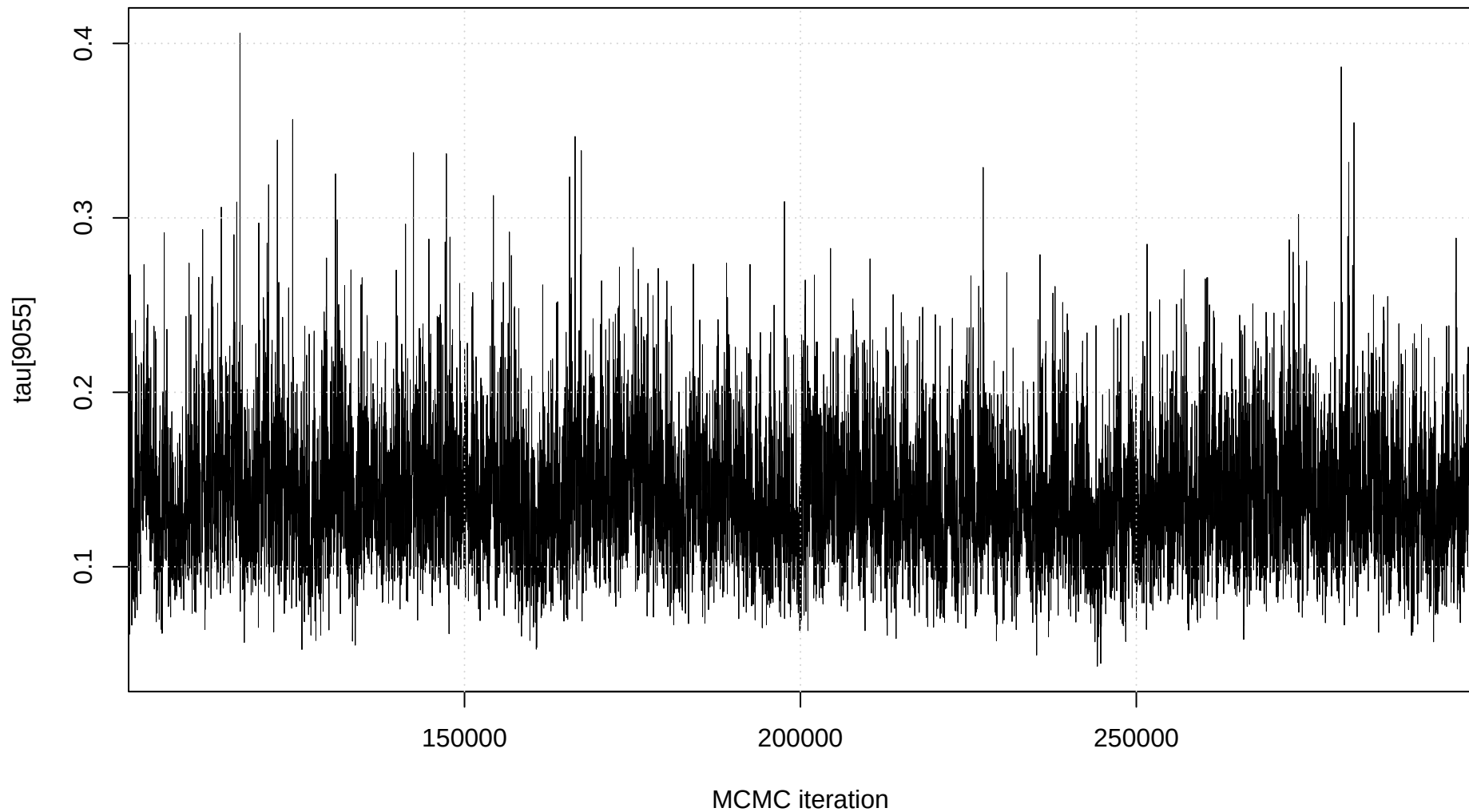
Trace plot: tau[9055]
