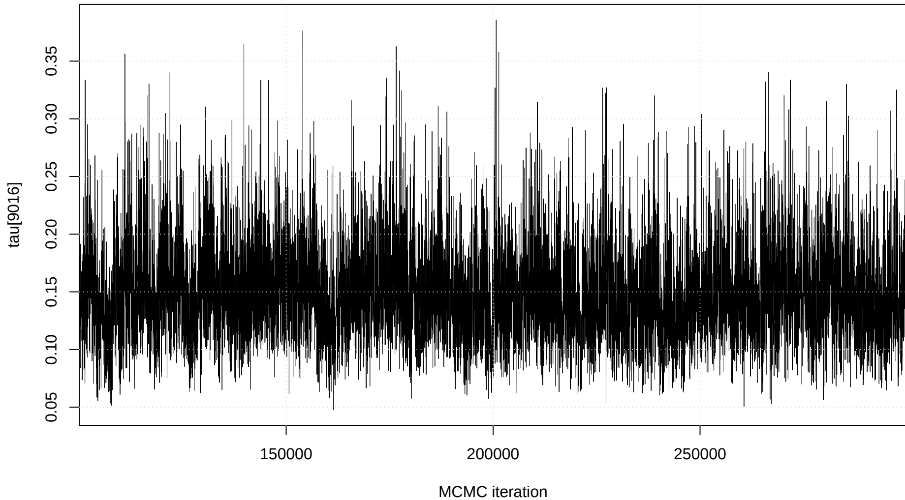
Trace plot: tau[9016]
