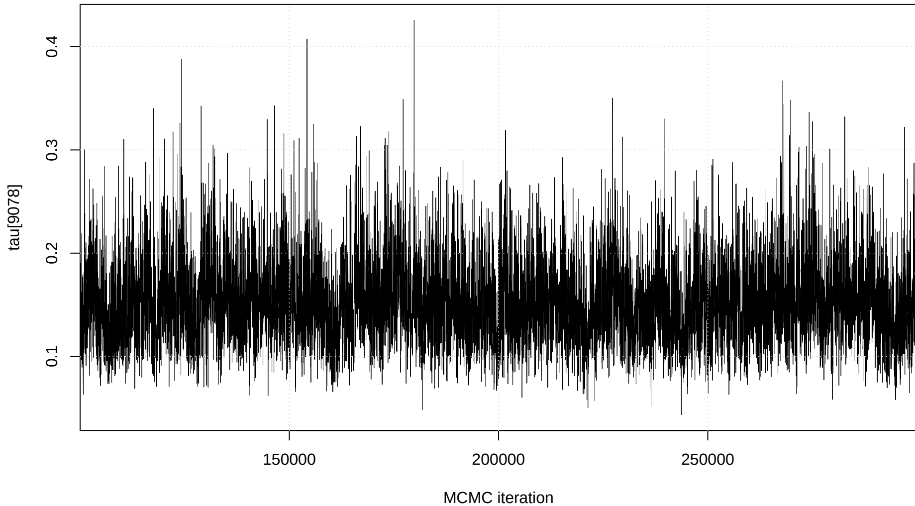
Trace plot: tau[9078]
