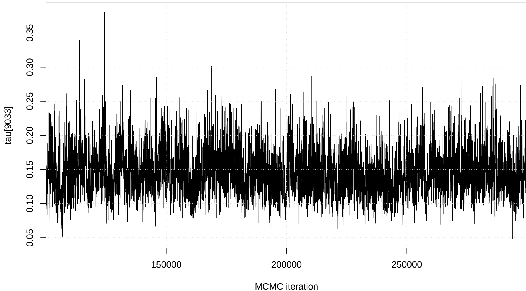
Trace plot: tau[9033]
