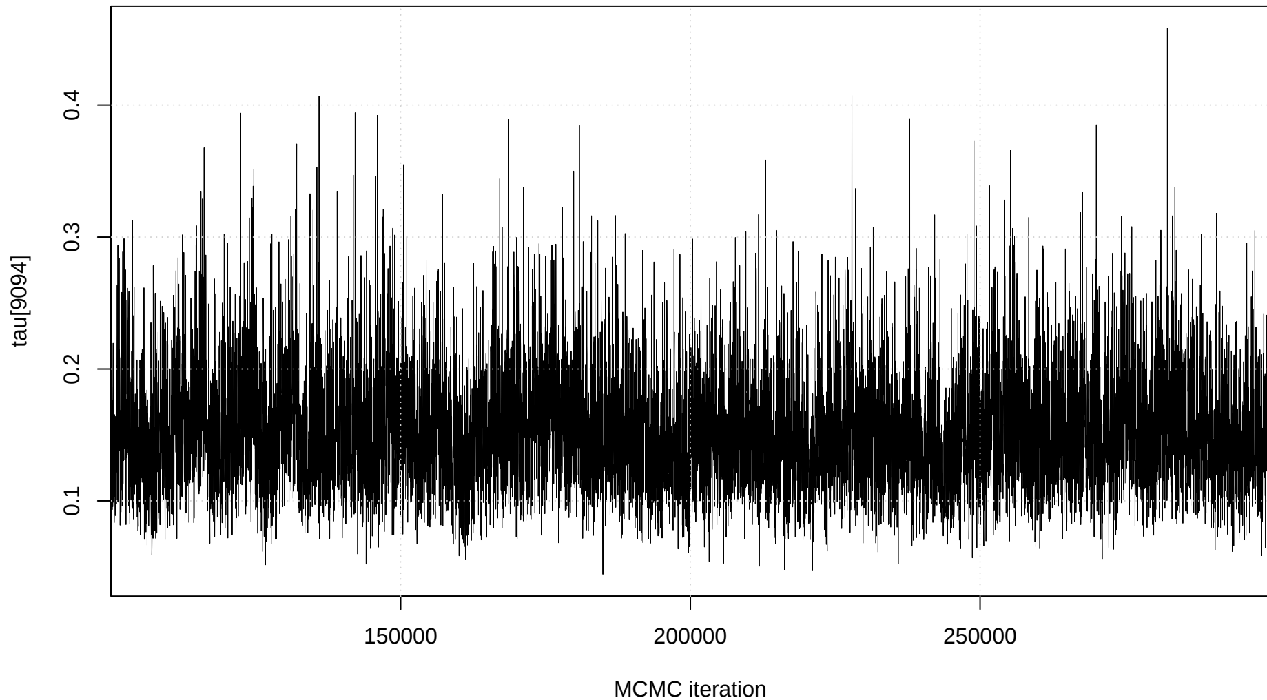
Trace plot: tau[9094]
