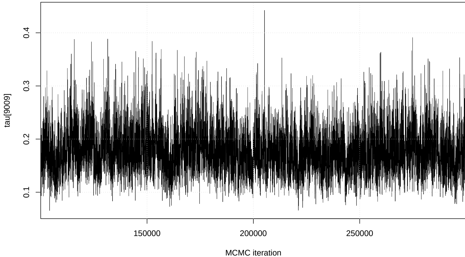
Trace plot: tau[9009]
