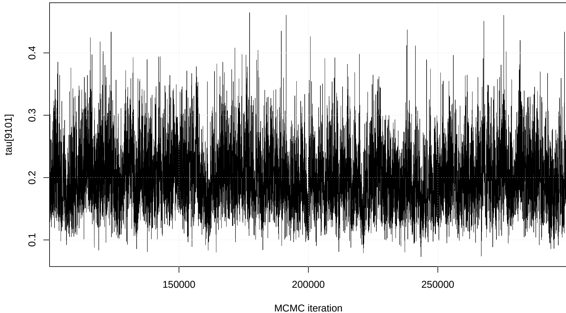
Trace plot: tau[9101]
