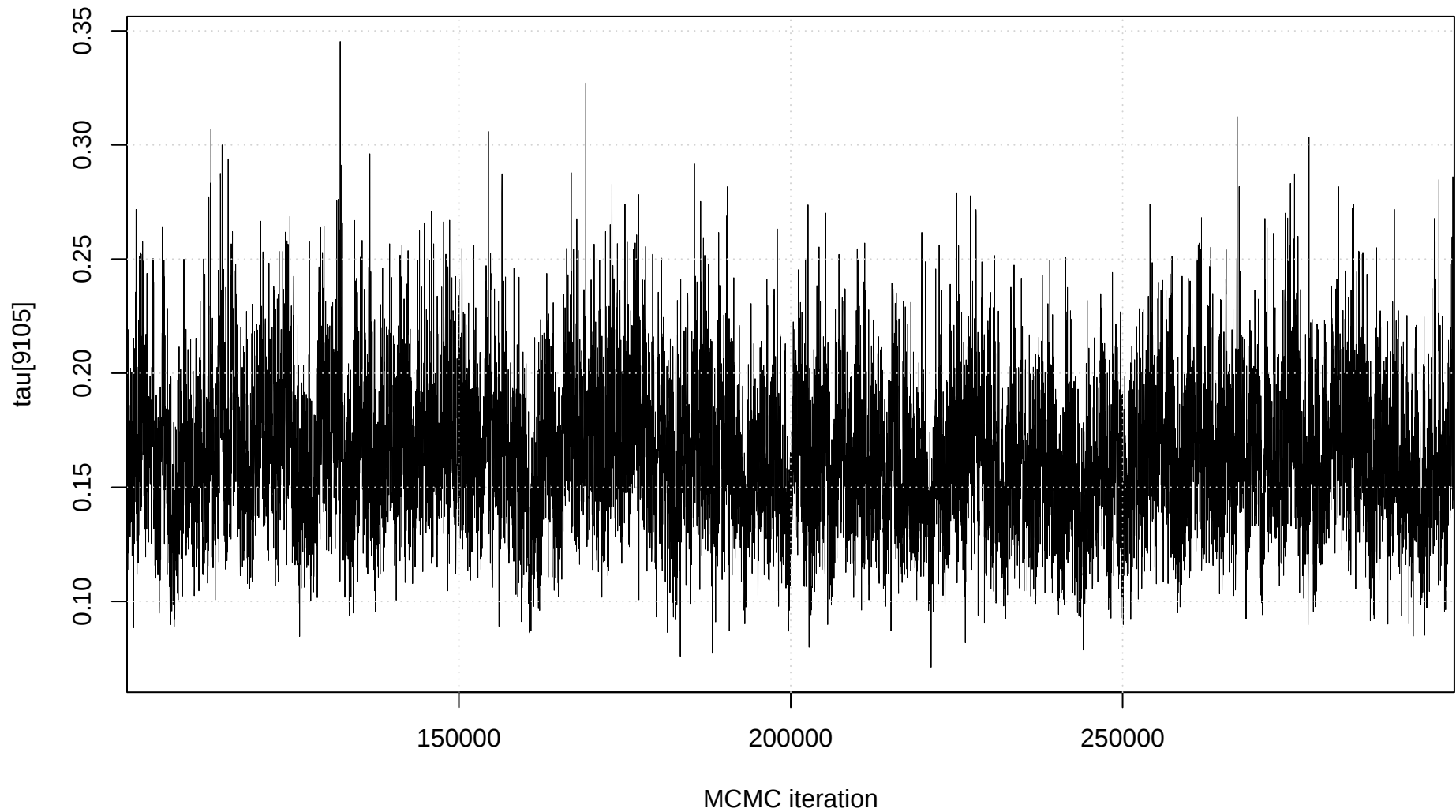
Trace plot: tau[9105]
