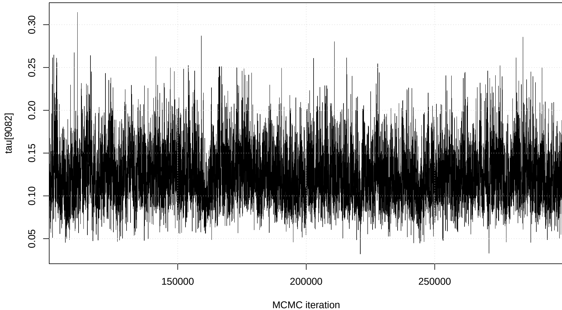
Trace plot: tau[9082]
