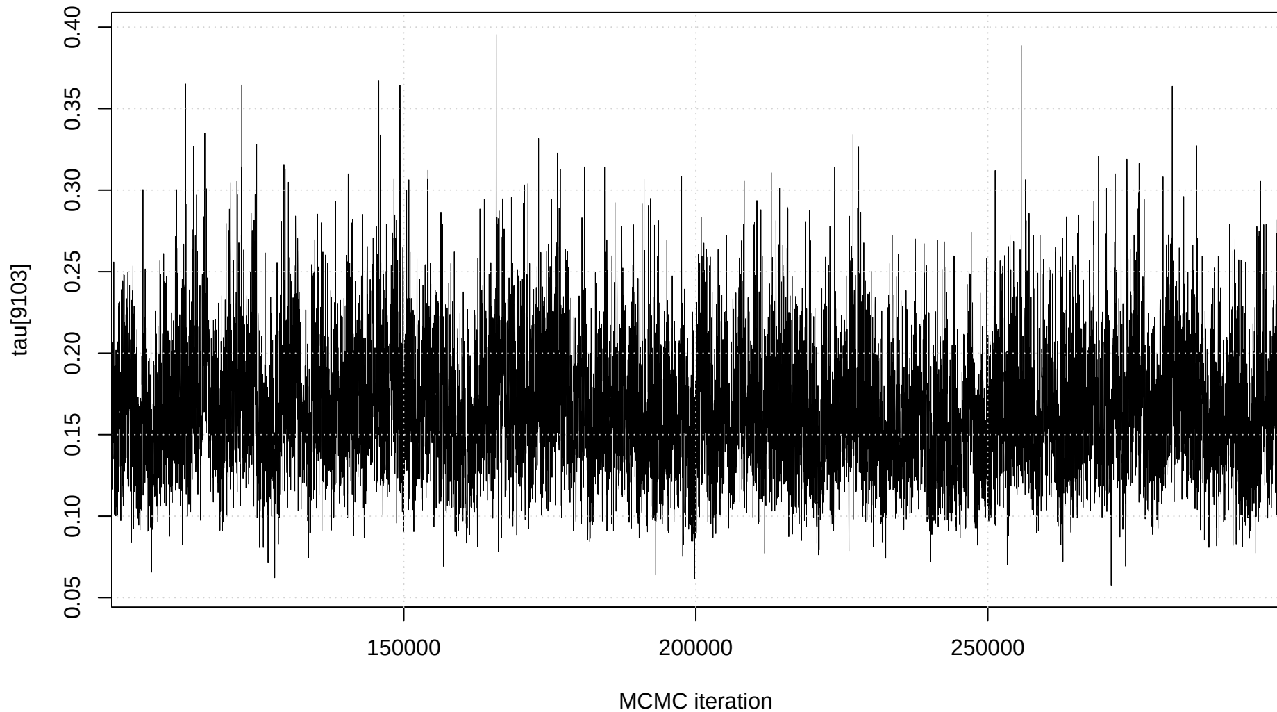
Trace plot: tau[9103]
