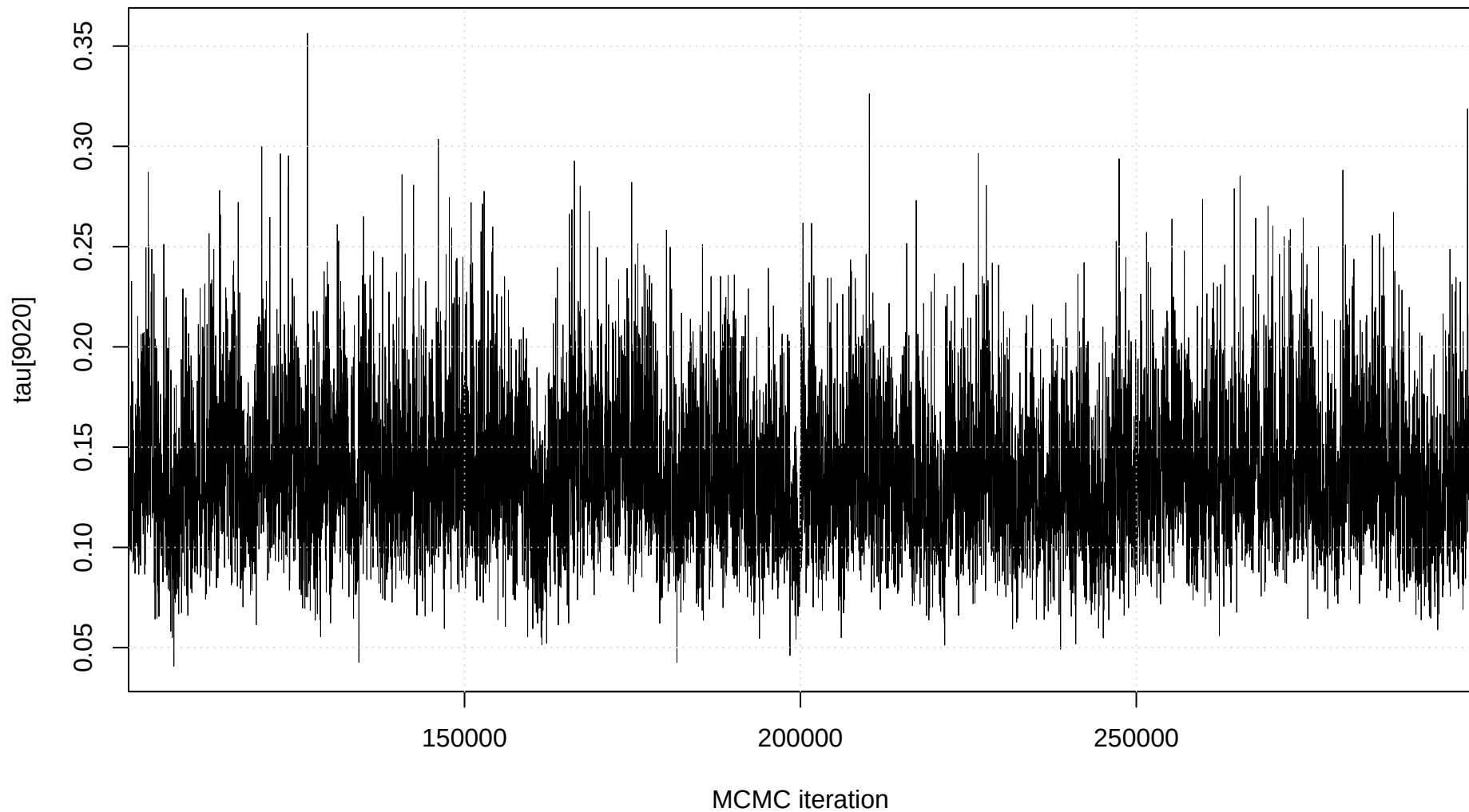
Trace plot: tau[9020]
