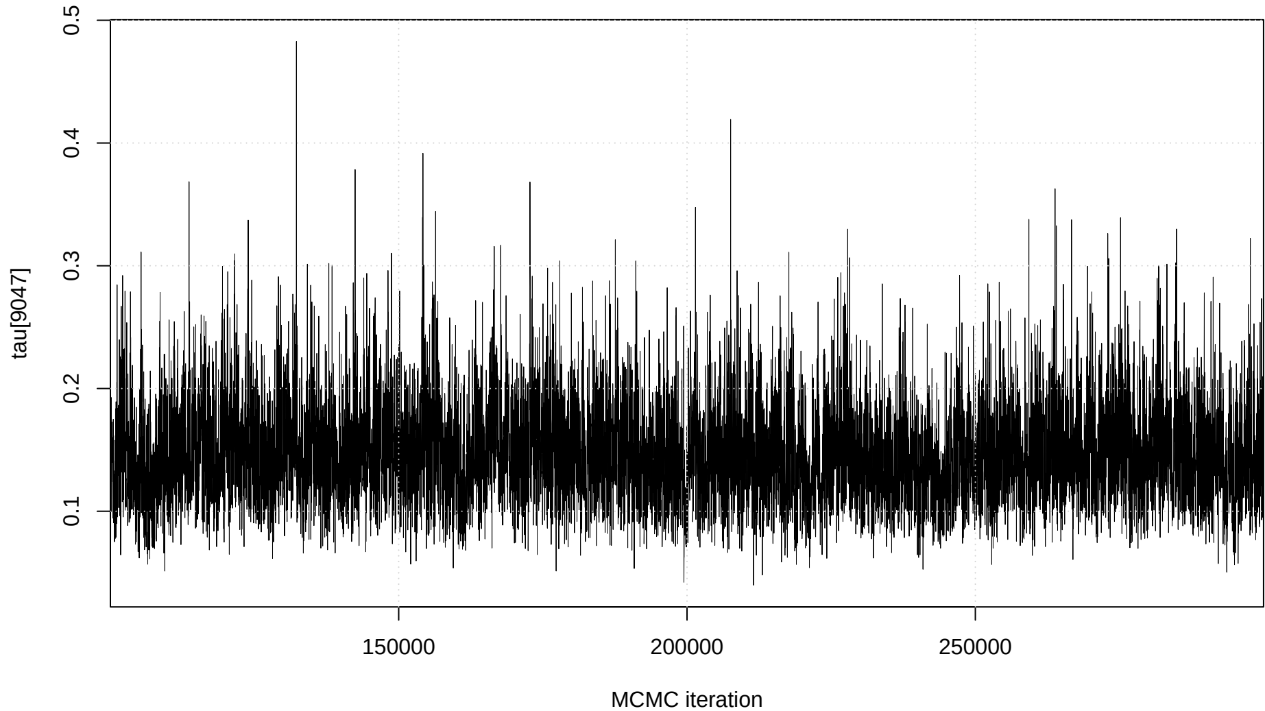
Trace plot: tau[9047]
