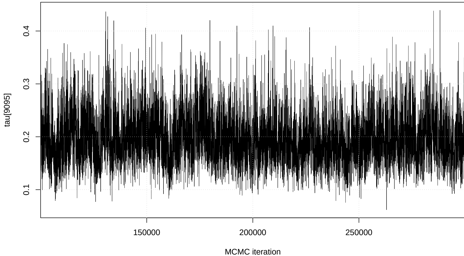
Trace plot: tau[9095]
