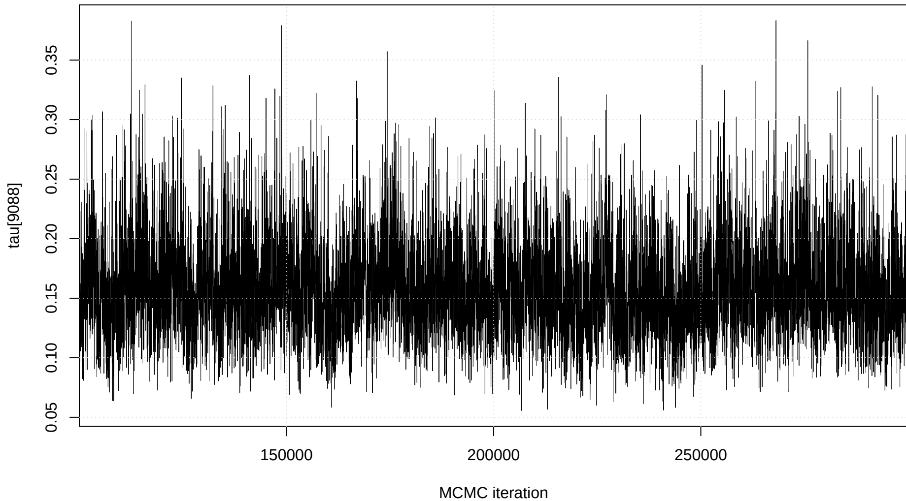
Trace plot: tau[9088]
