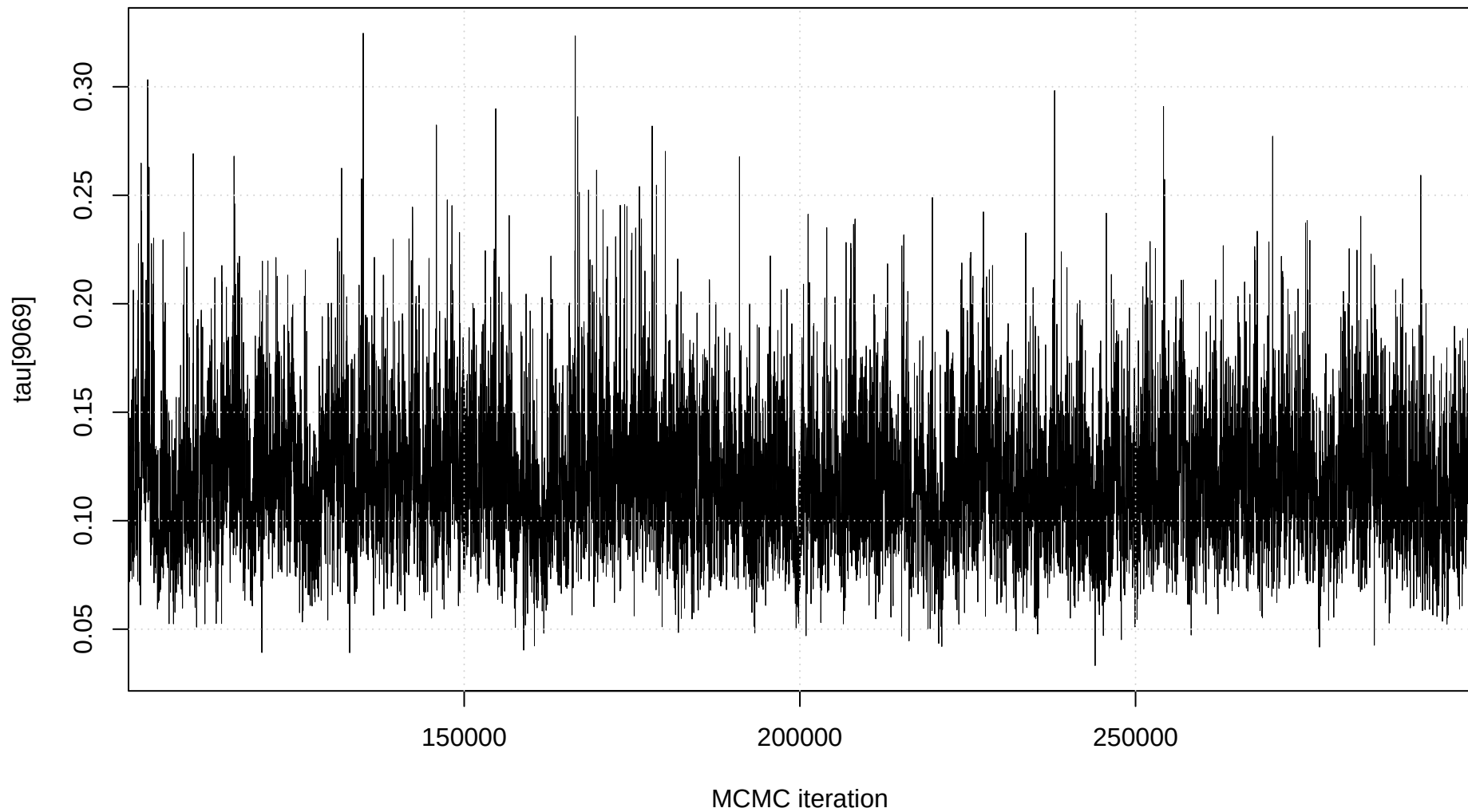
Trace plot: tau[9069]
