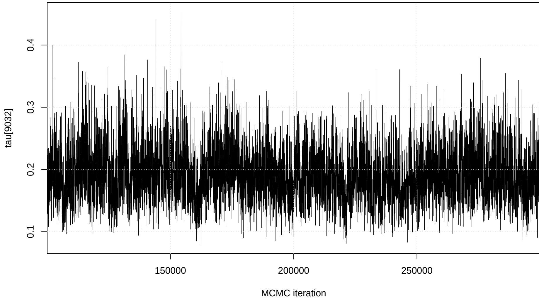
Trace plot: tau[9032]
