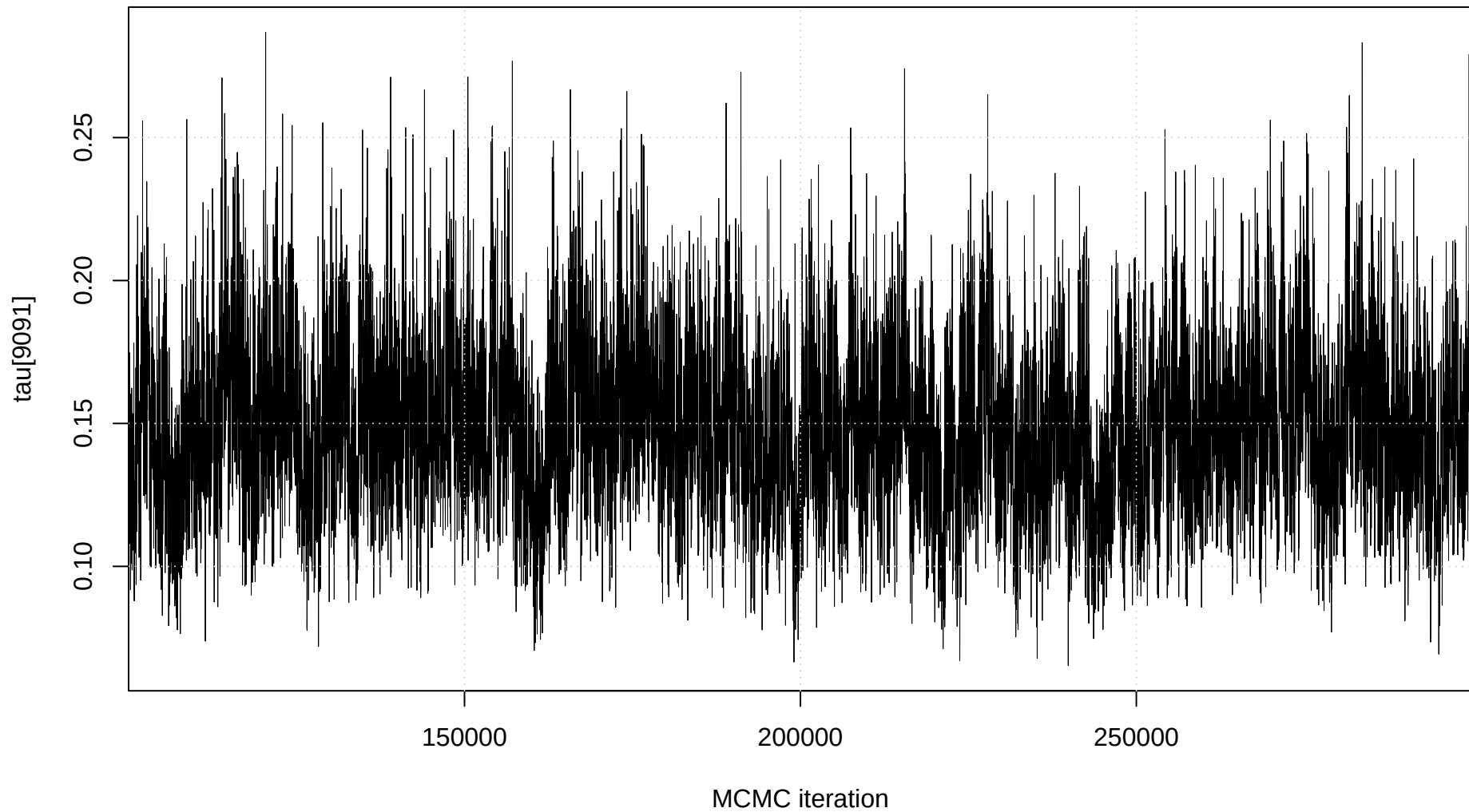
Trace plot: tau[9091]
