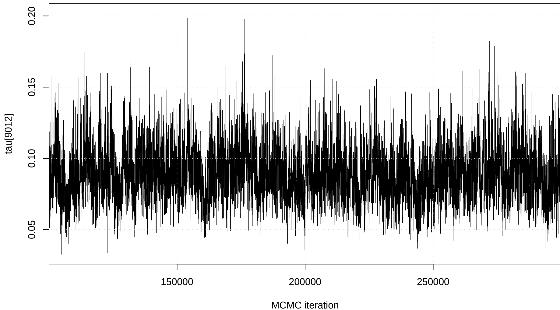
Trace plot: tau[9012]
