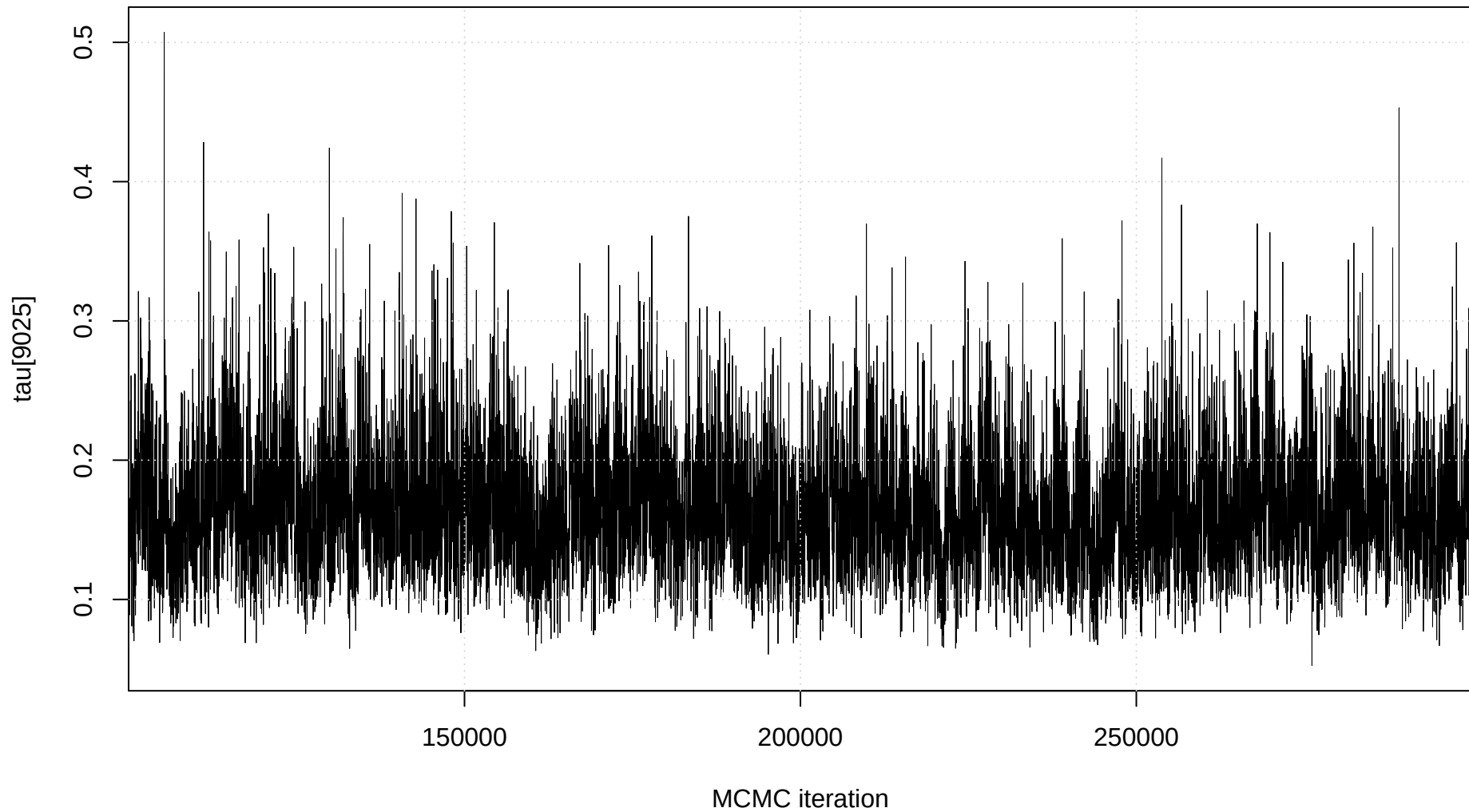
Trace plot: tau[9025]
