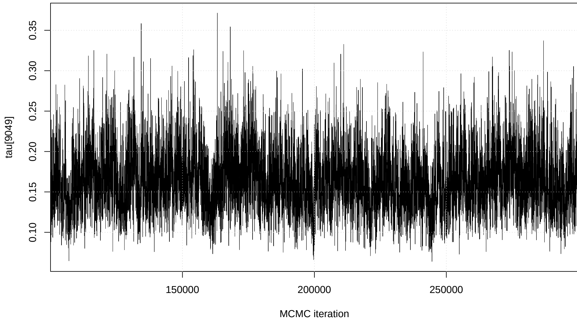
Trace plot: tau[9049]
