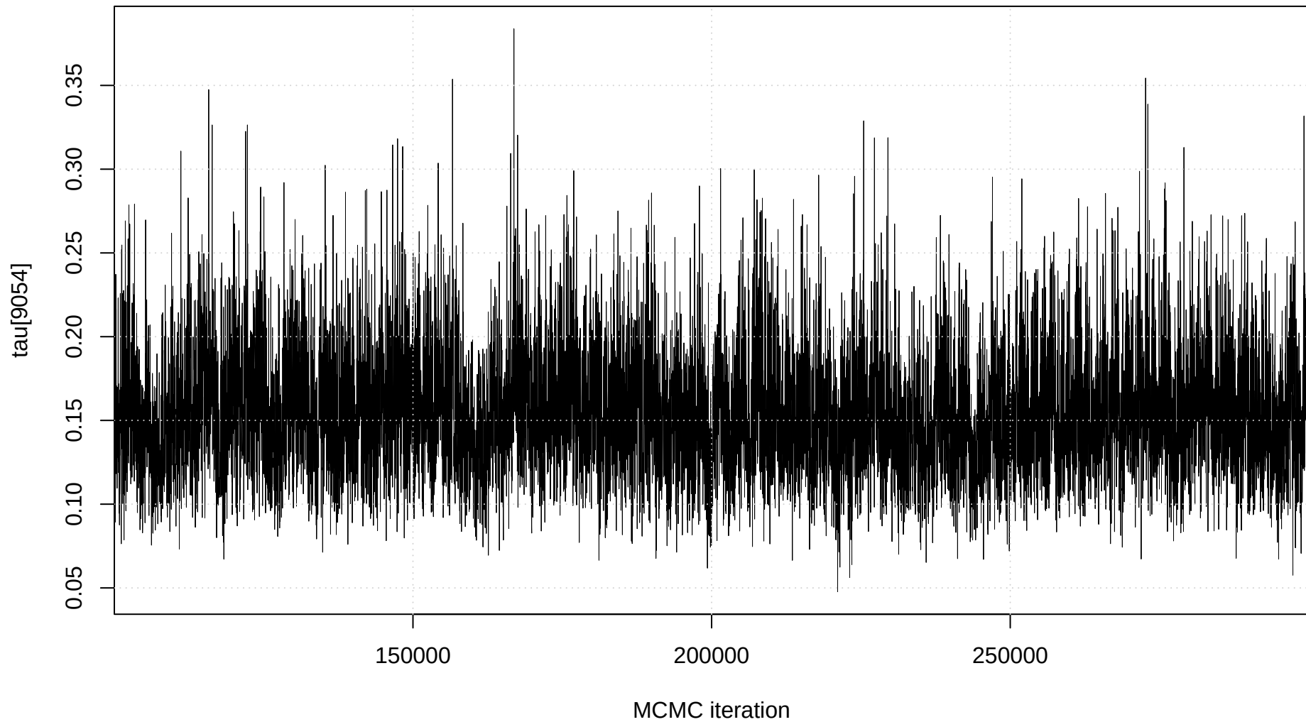
Trace plot: tau[9054]
