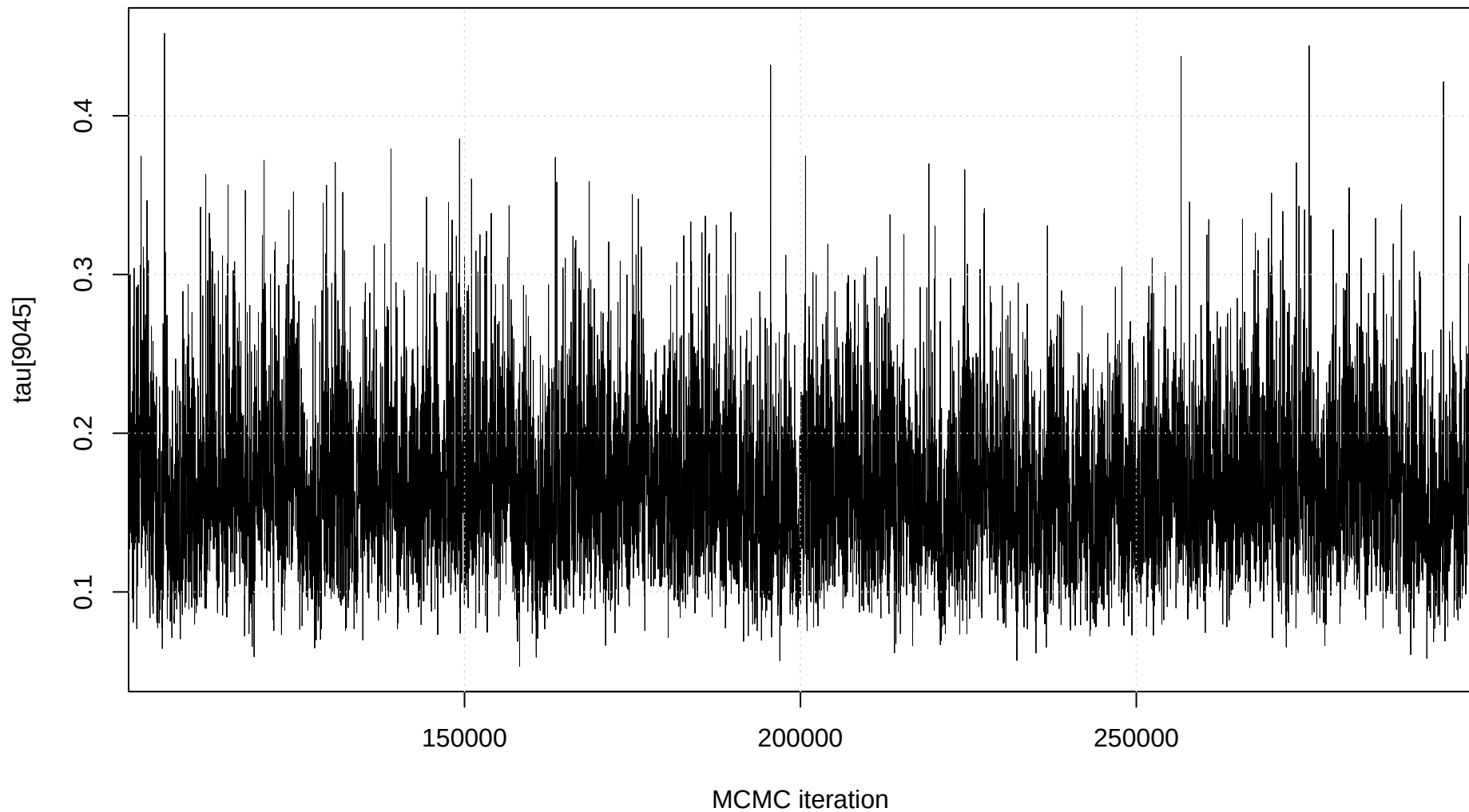
Trace plot: tau[9045]
