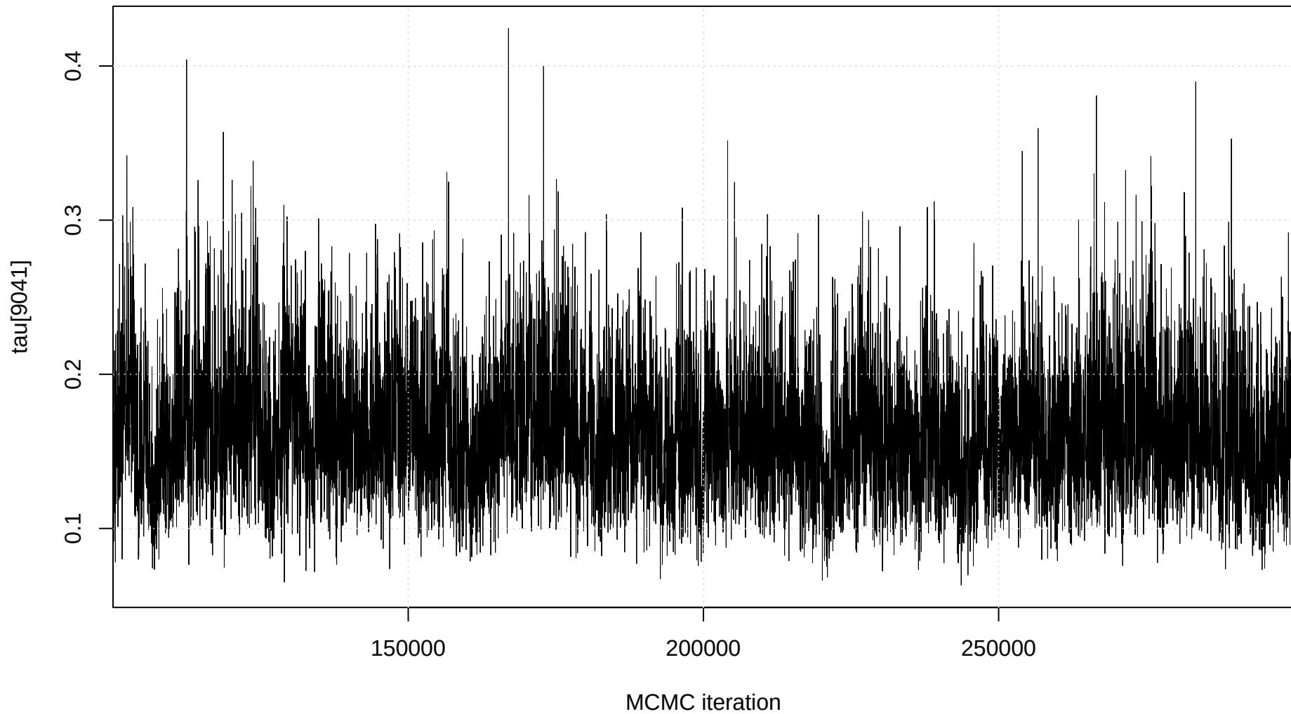
Trace plot: tau[9041]
