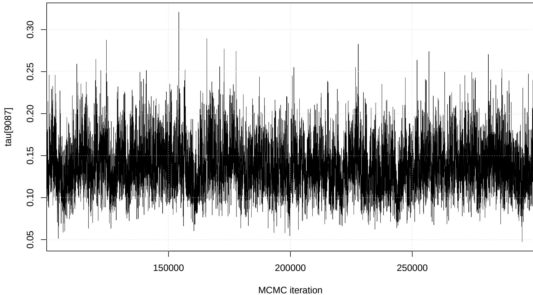
Trace plot: tau[9087]
