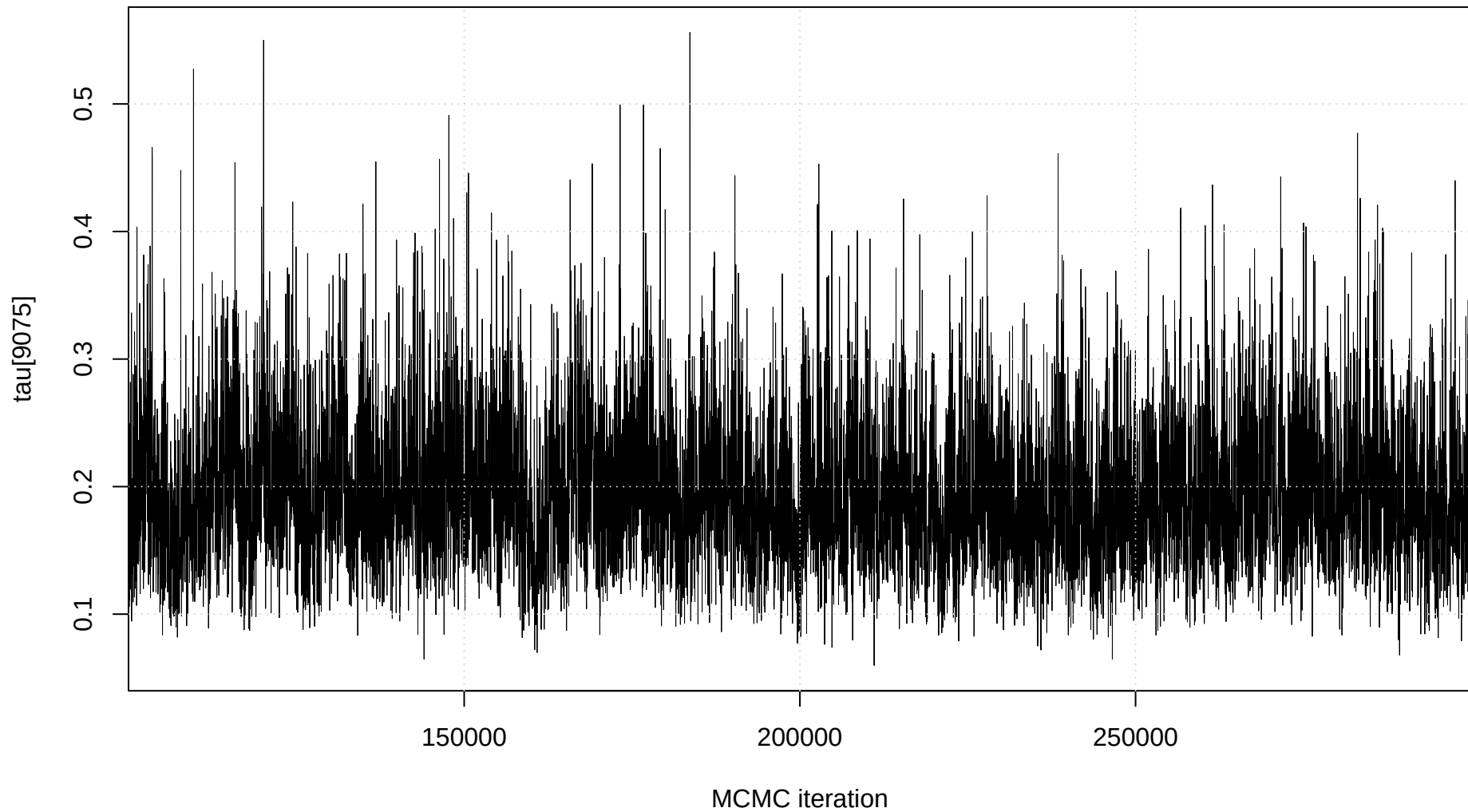
Trace plot: tau[9075]
