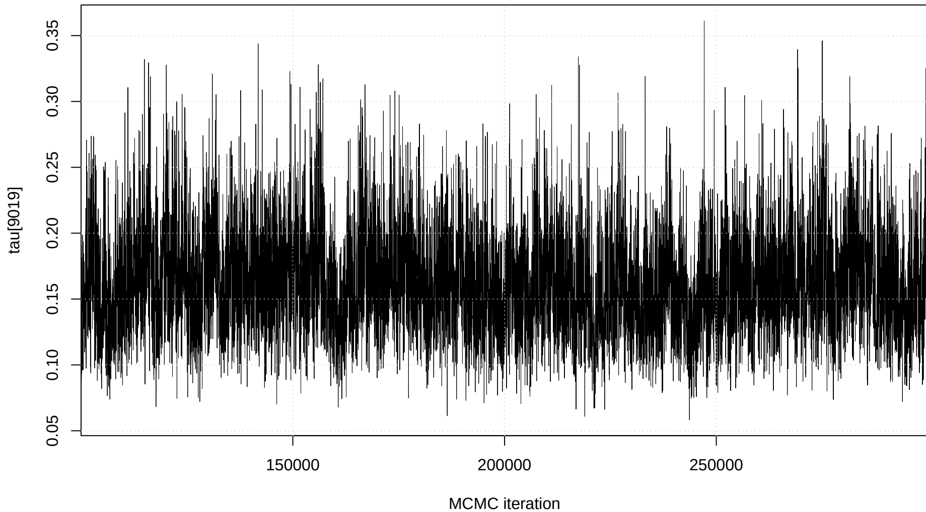
Trace plot: tau[9019]
