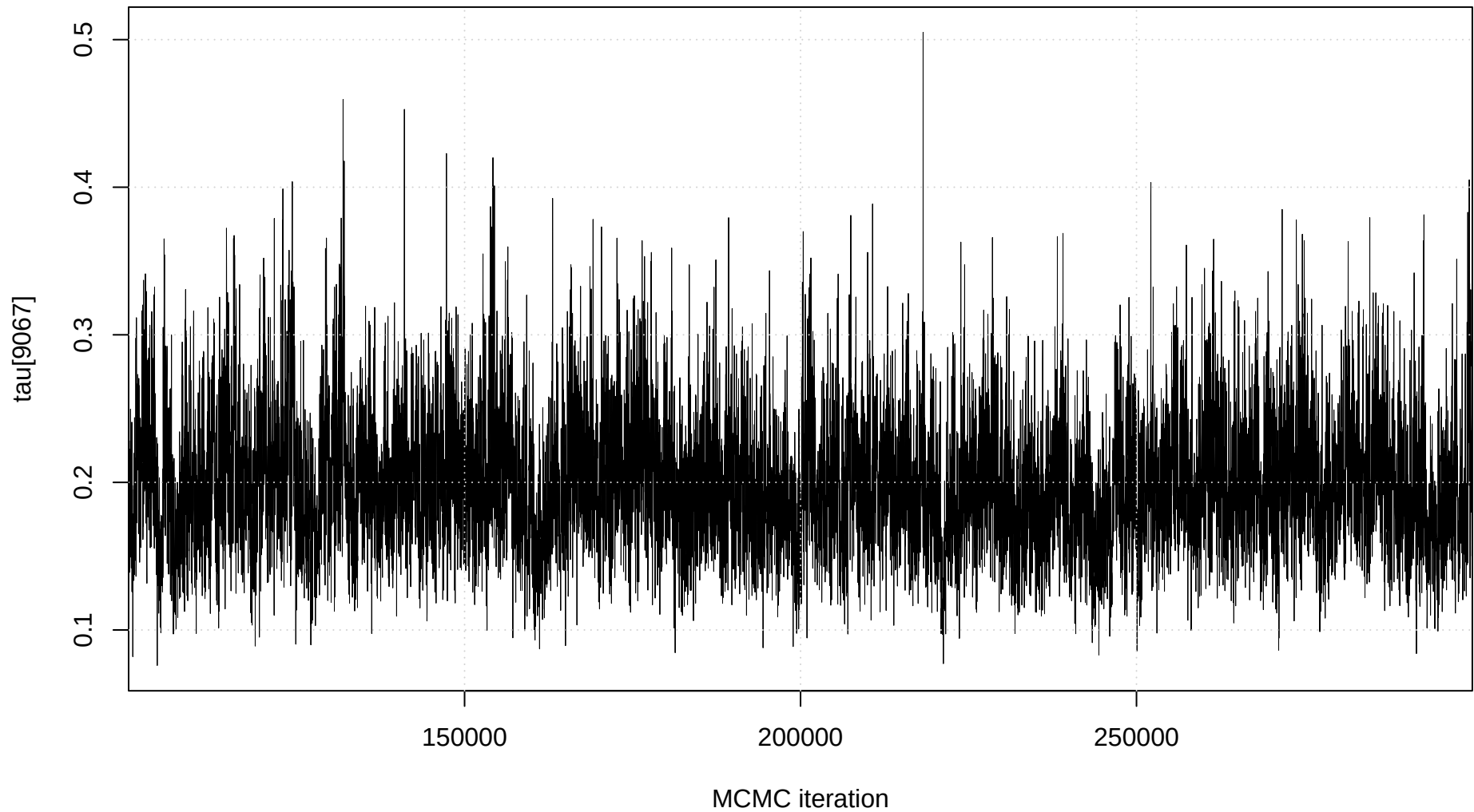
Trace plot: tau[9067]
