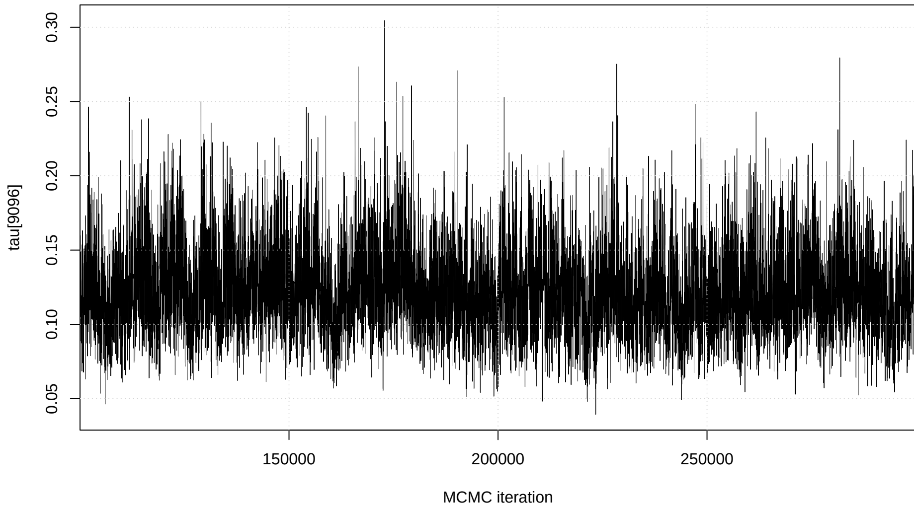
Trace plot: tau[9096]
