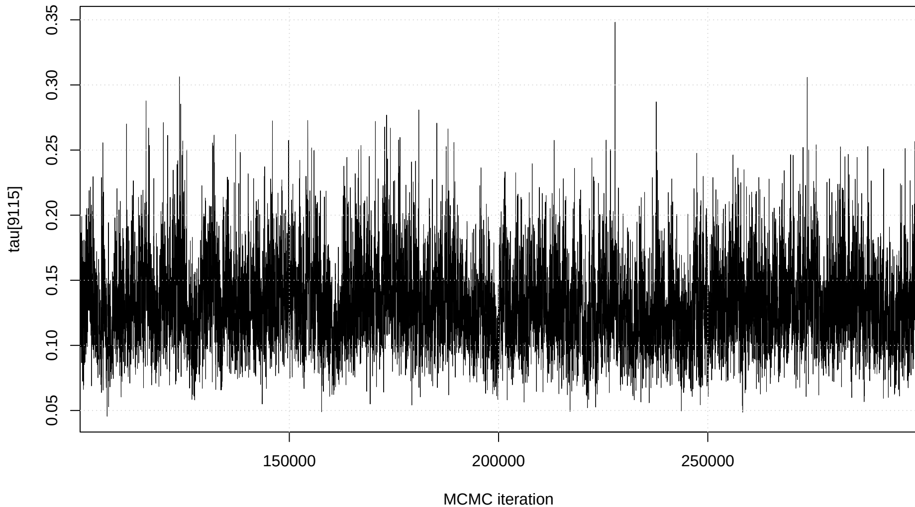
Trace plot: tau[9115]
