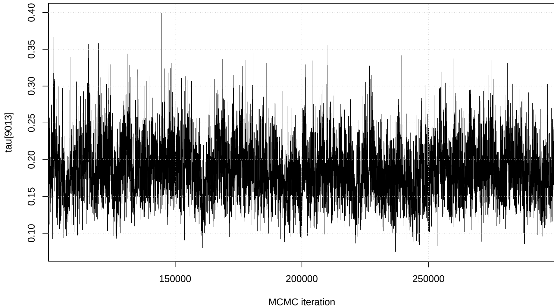
Trace plot: tau[9013]
