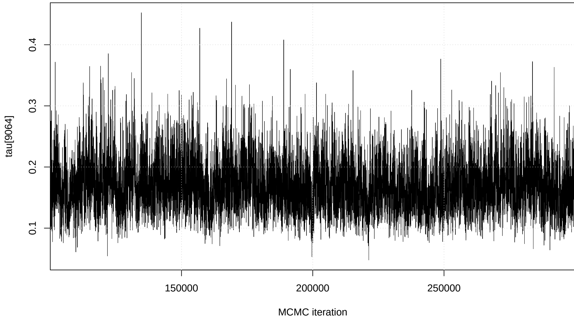
Trace plot: tau[9064]
