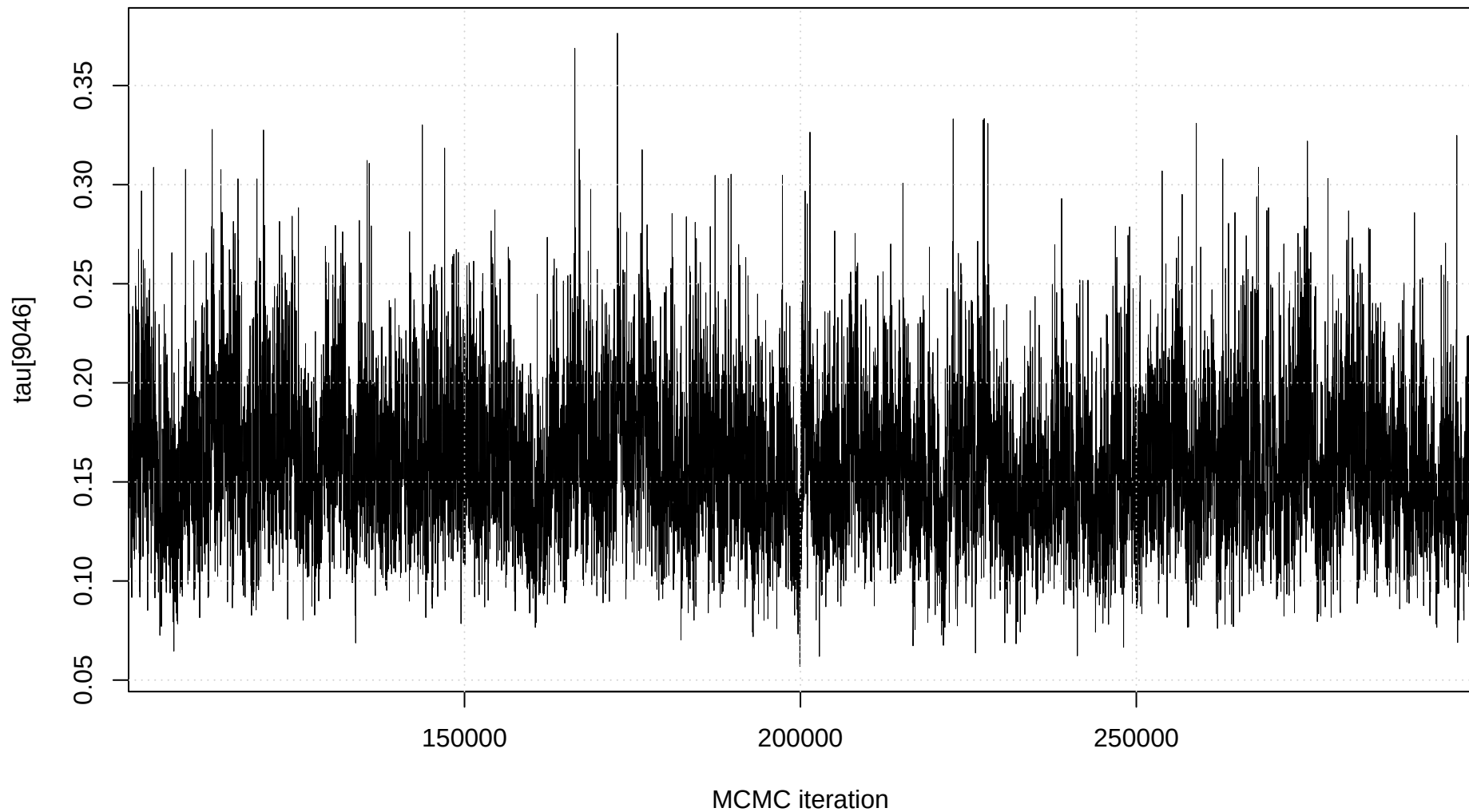
Trace plot: tau[9046]
