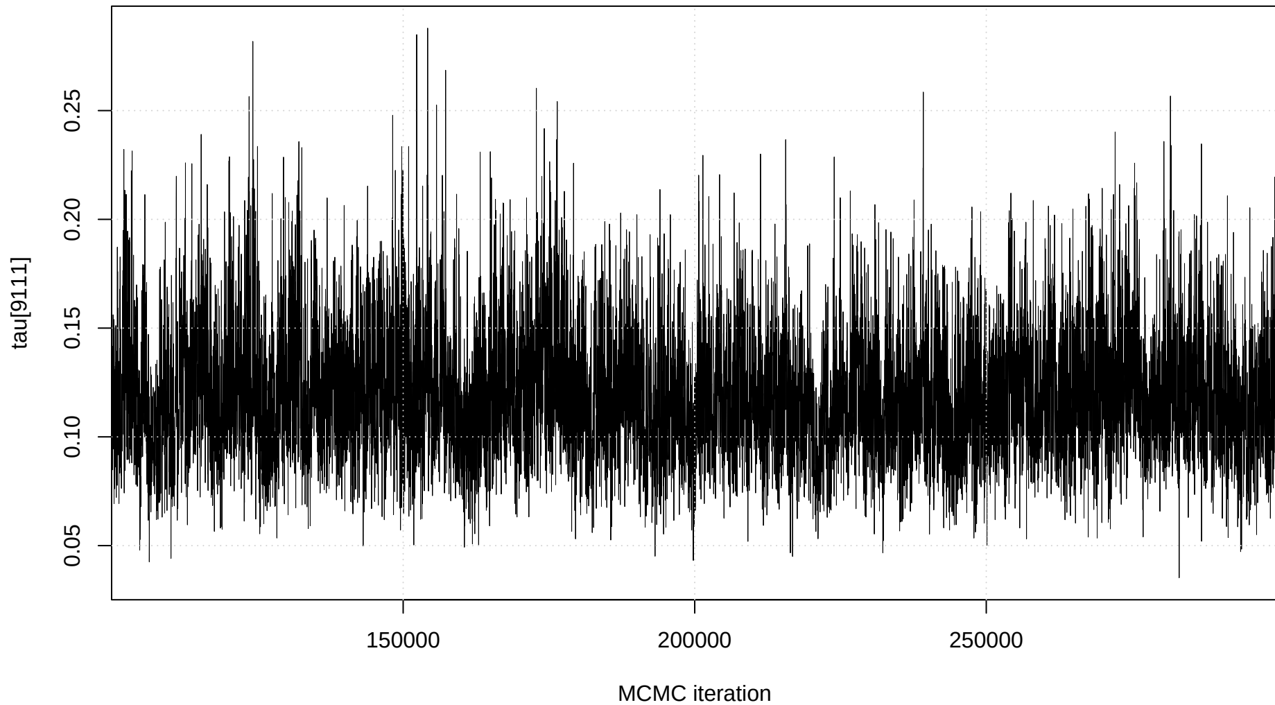
Trace plot: tau[9111]
