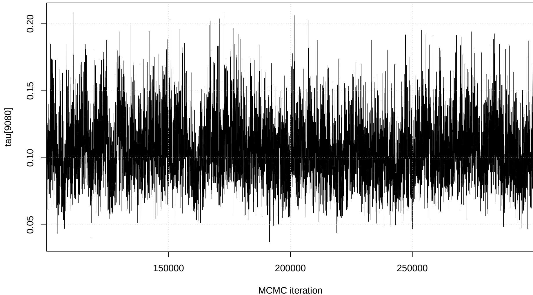
Trace plot: tau[9080]
