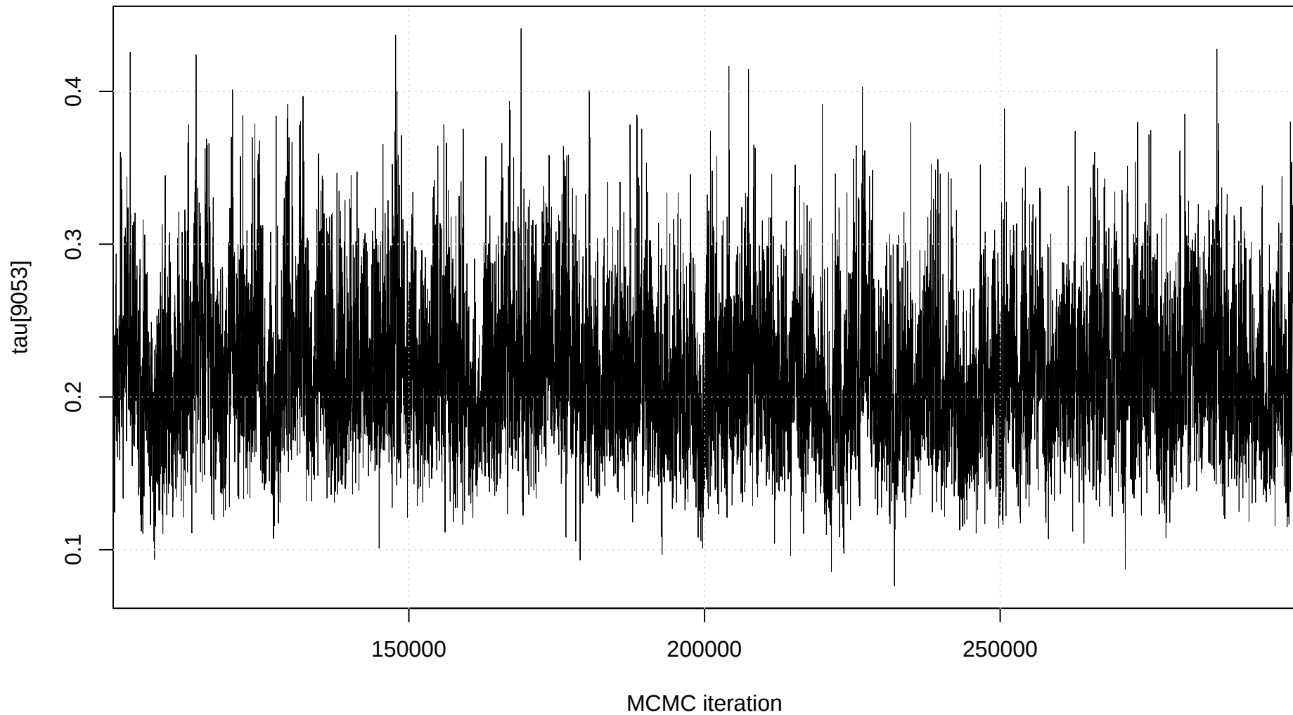
Trace plot: tau[9053]
