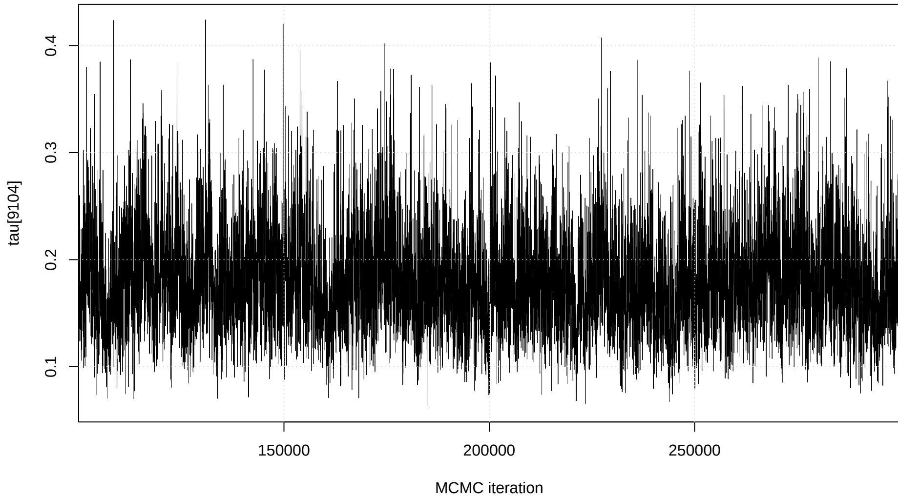
Trace plot: tau[9104]
