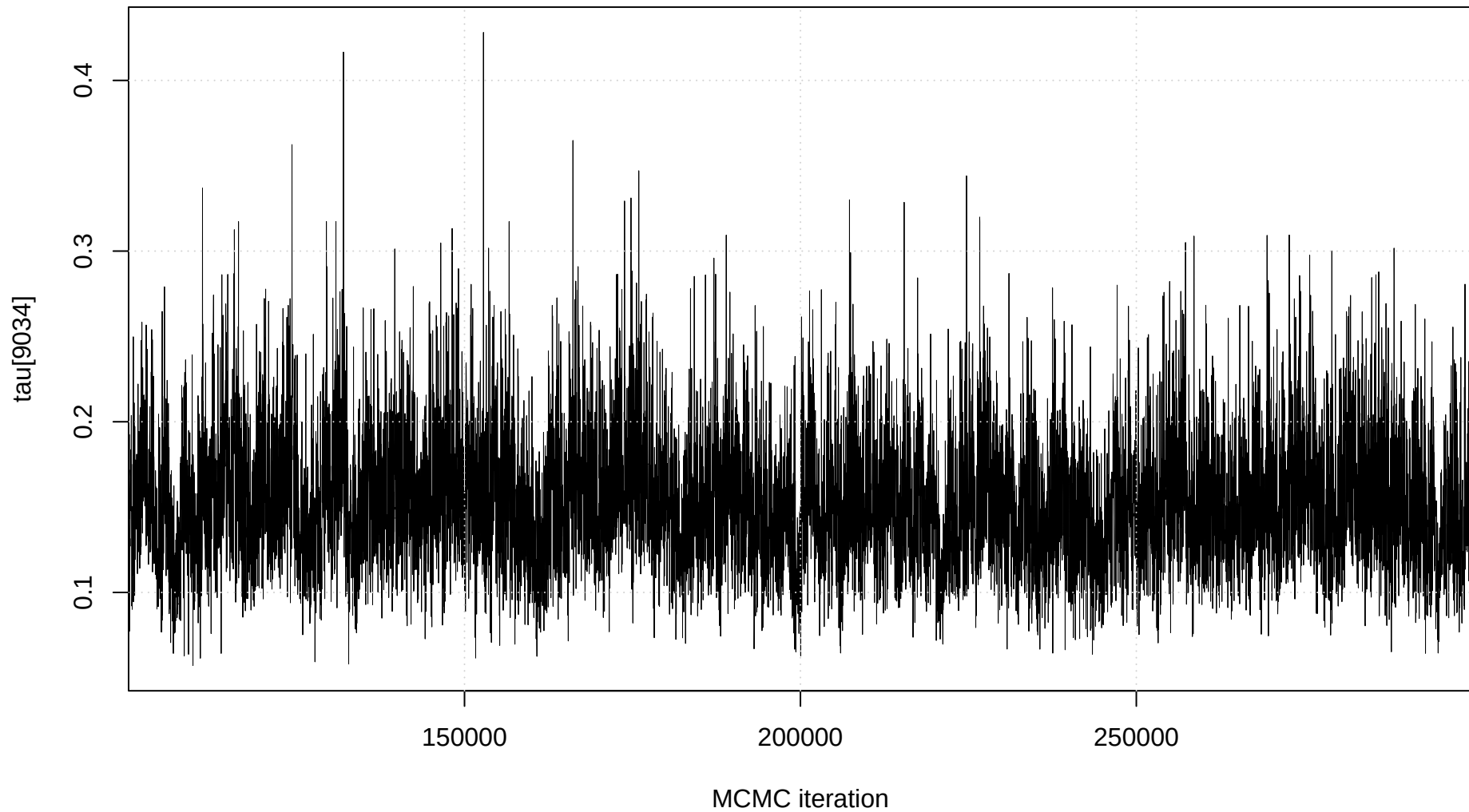
Trace plot: tau[9034]
