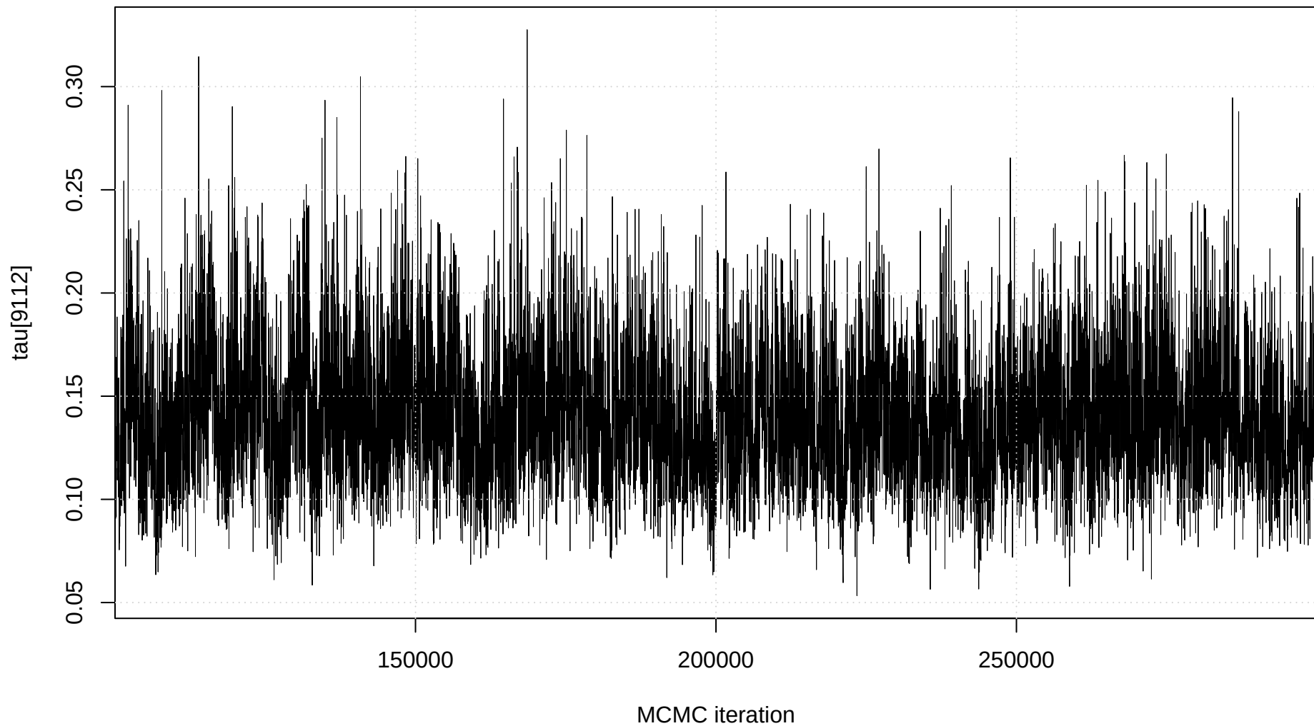
Trace plot: tau[9112]
