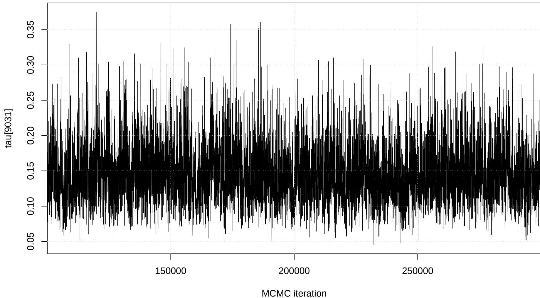
Trace plot: tau[9031]
