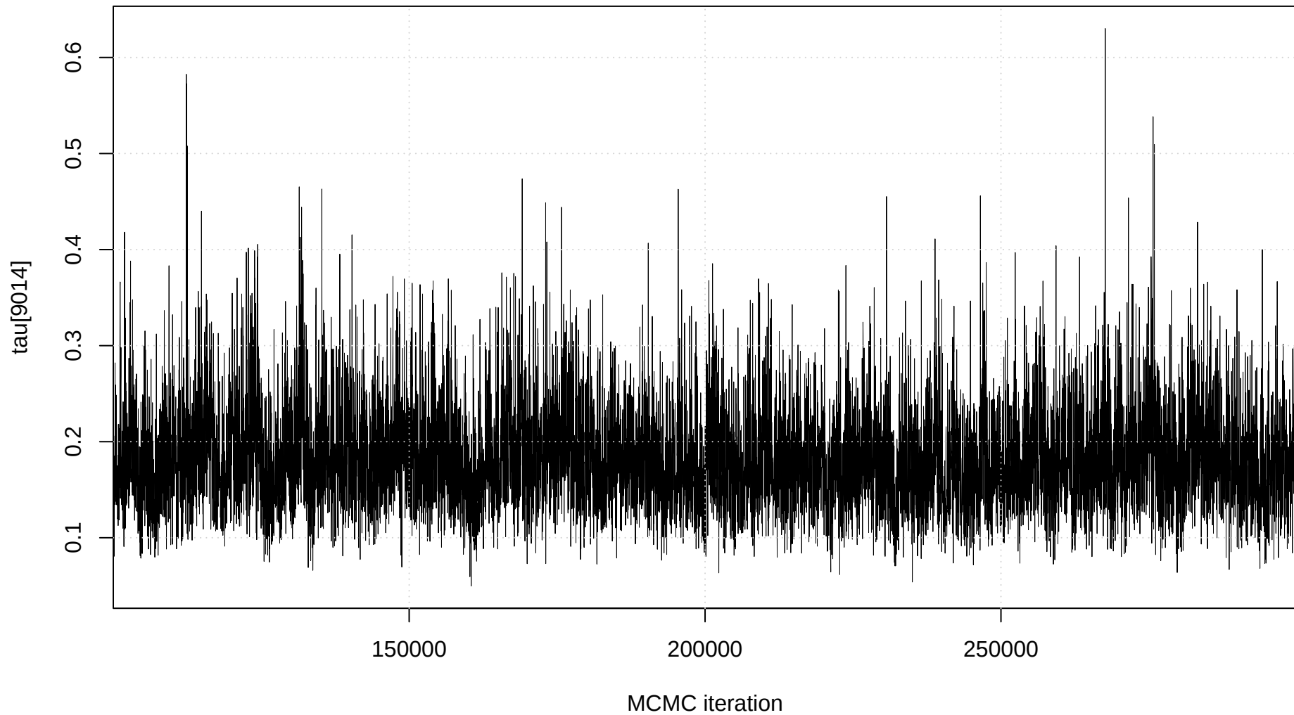
Trace plot: tau[9014]
