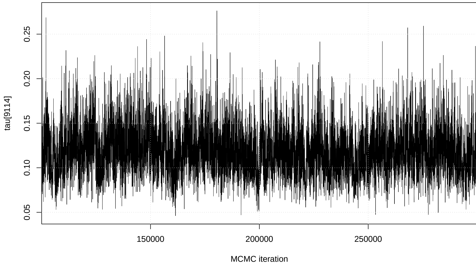
Trace plot: tau[9114]
