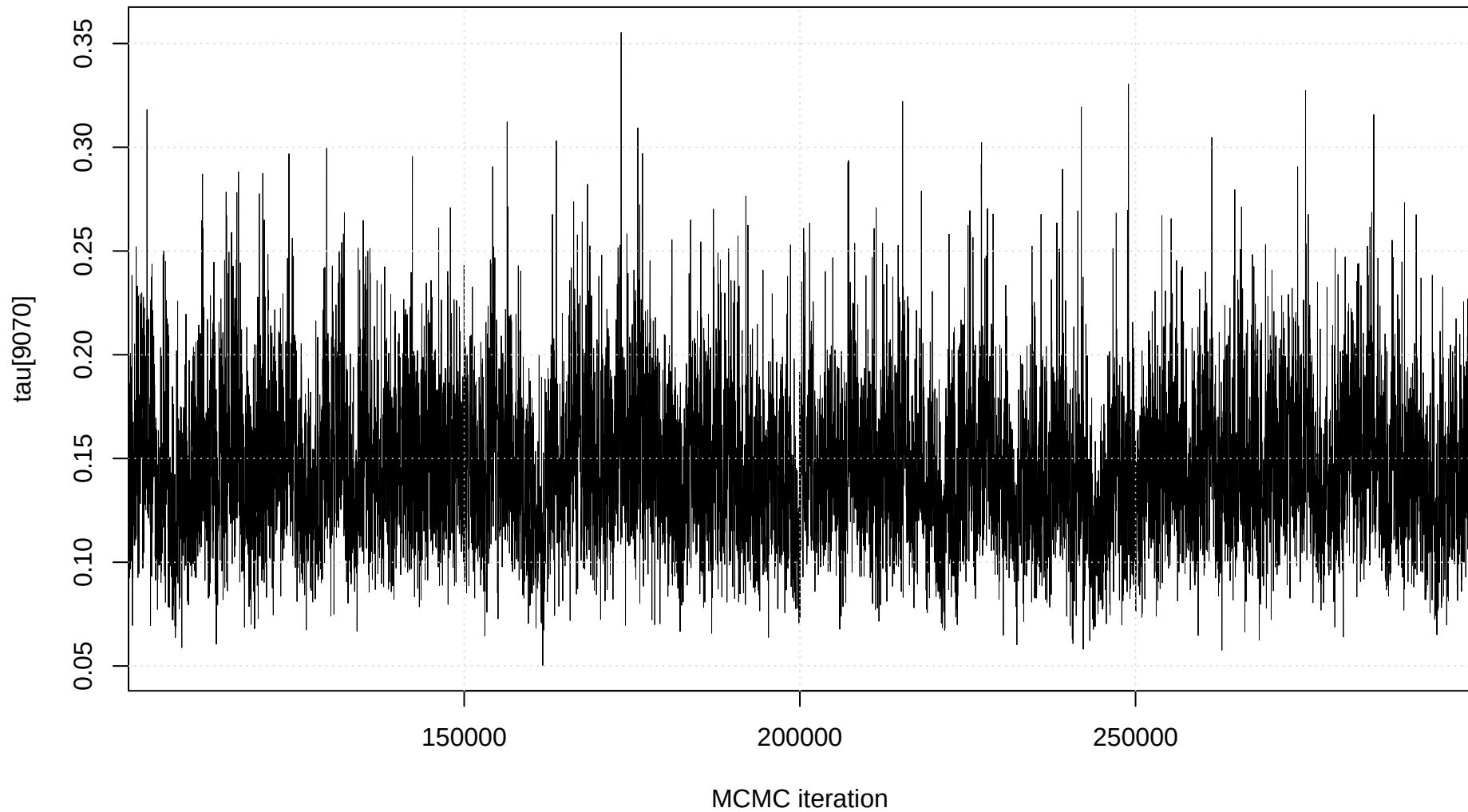
Trace plot: tau[9070]
