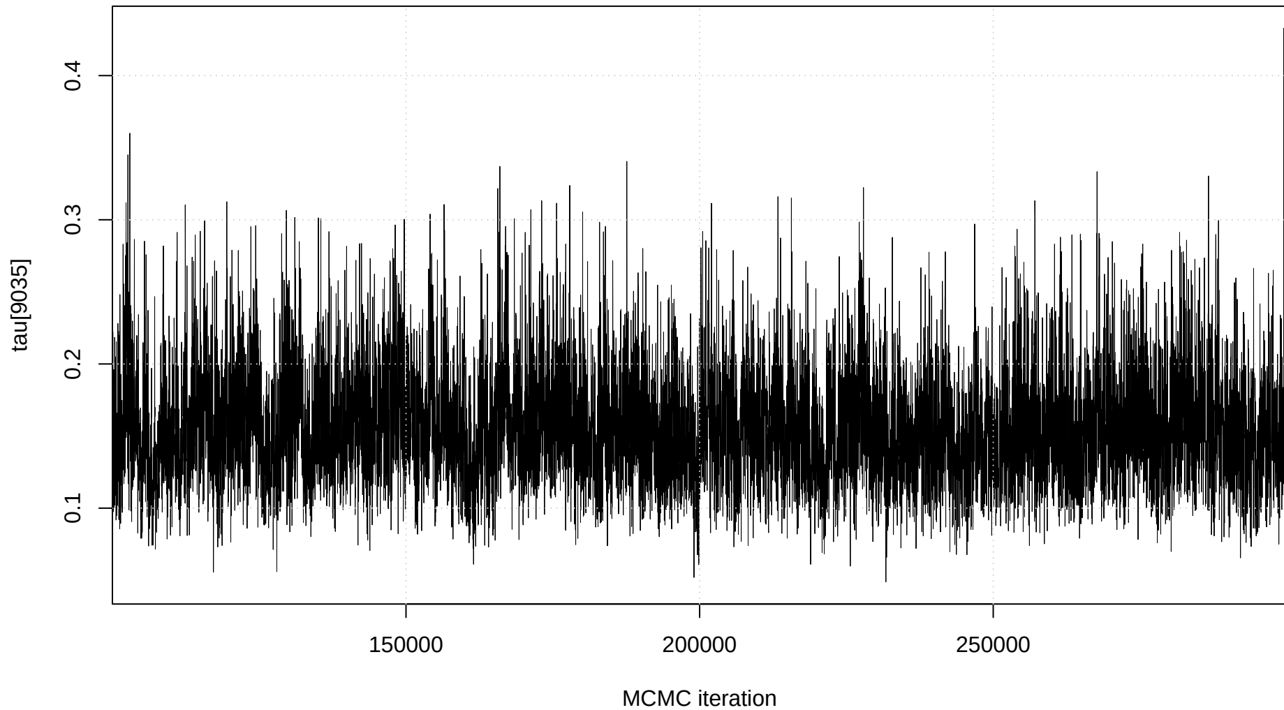
Trace plot: tau[9035]
