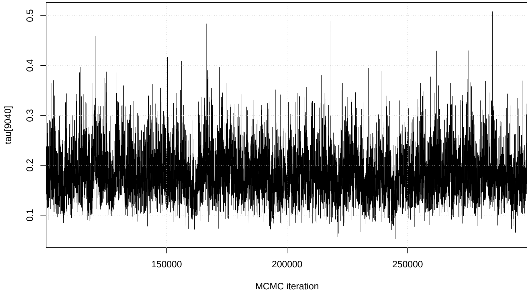
Trace plot: tau[9040]
