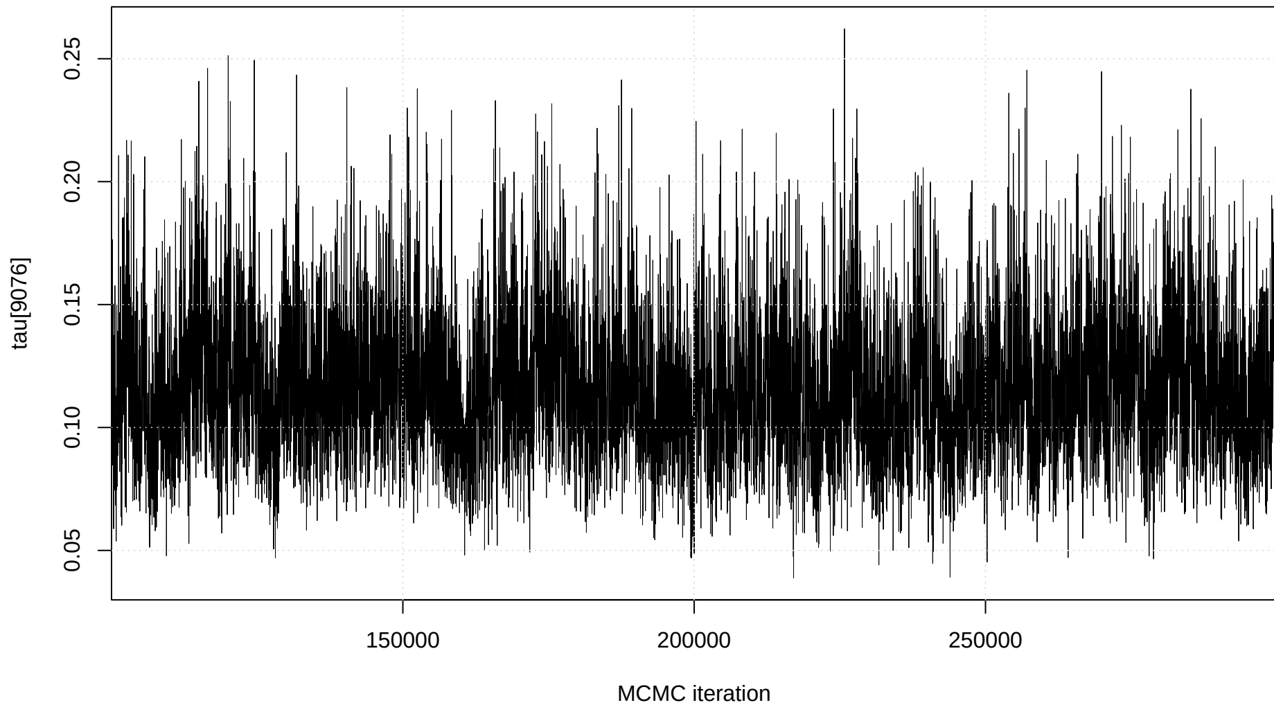
Trace plot: tau[9076]
