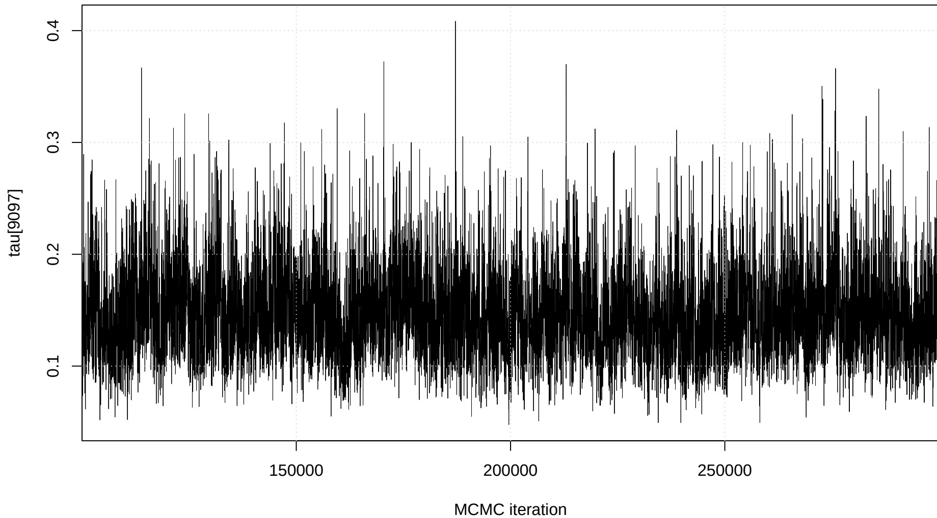
Trace plot: tau[9097]
