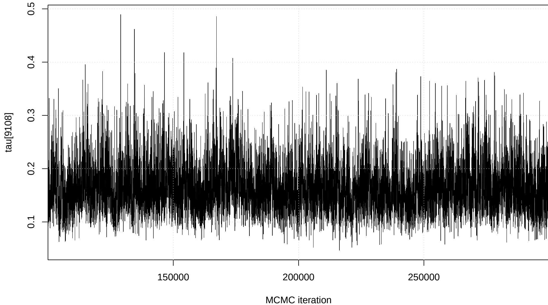
Trace plot: tau[9108]
