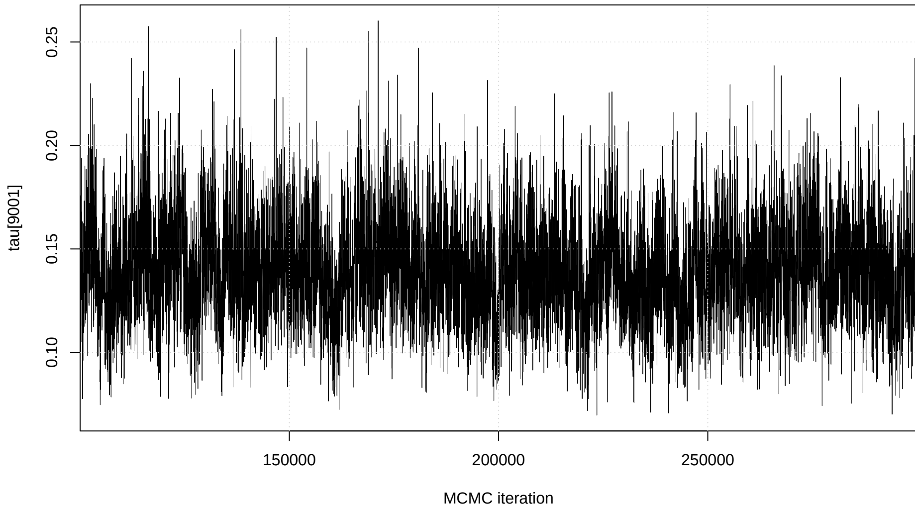
Trace plot: tau[9001]
