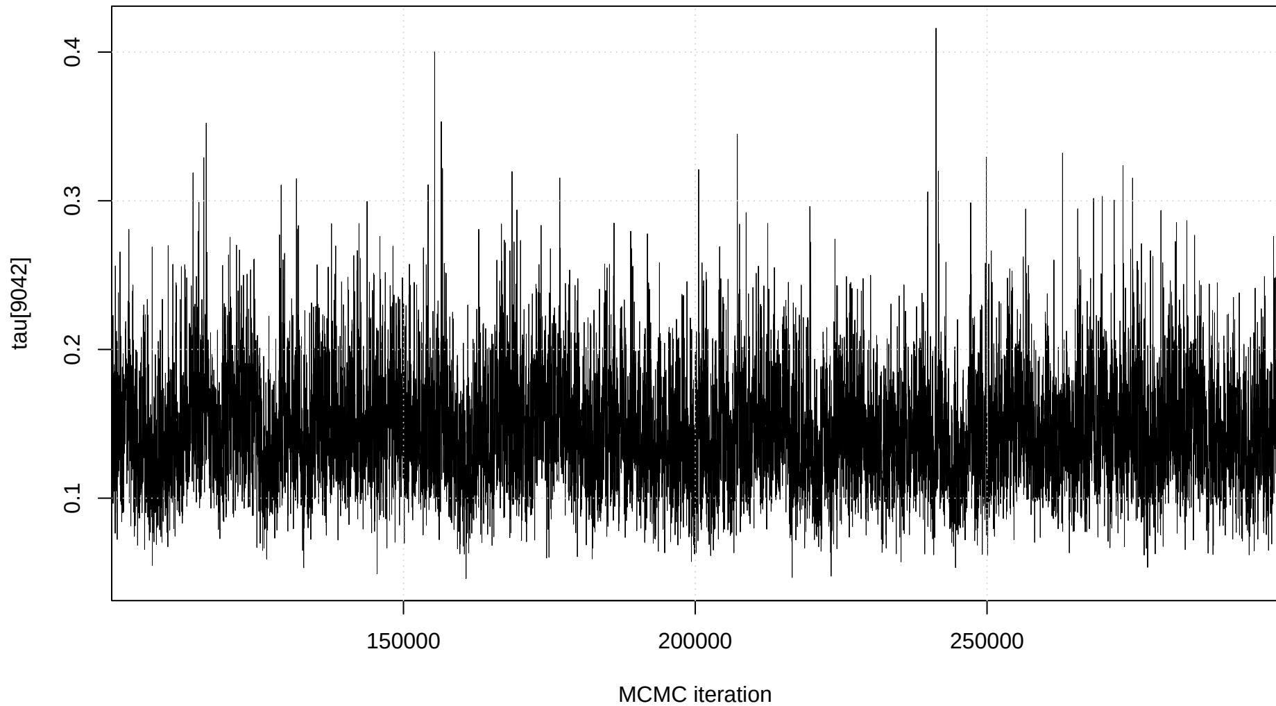
Trace plot: tau[9042]
