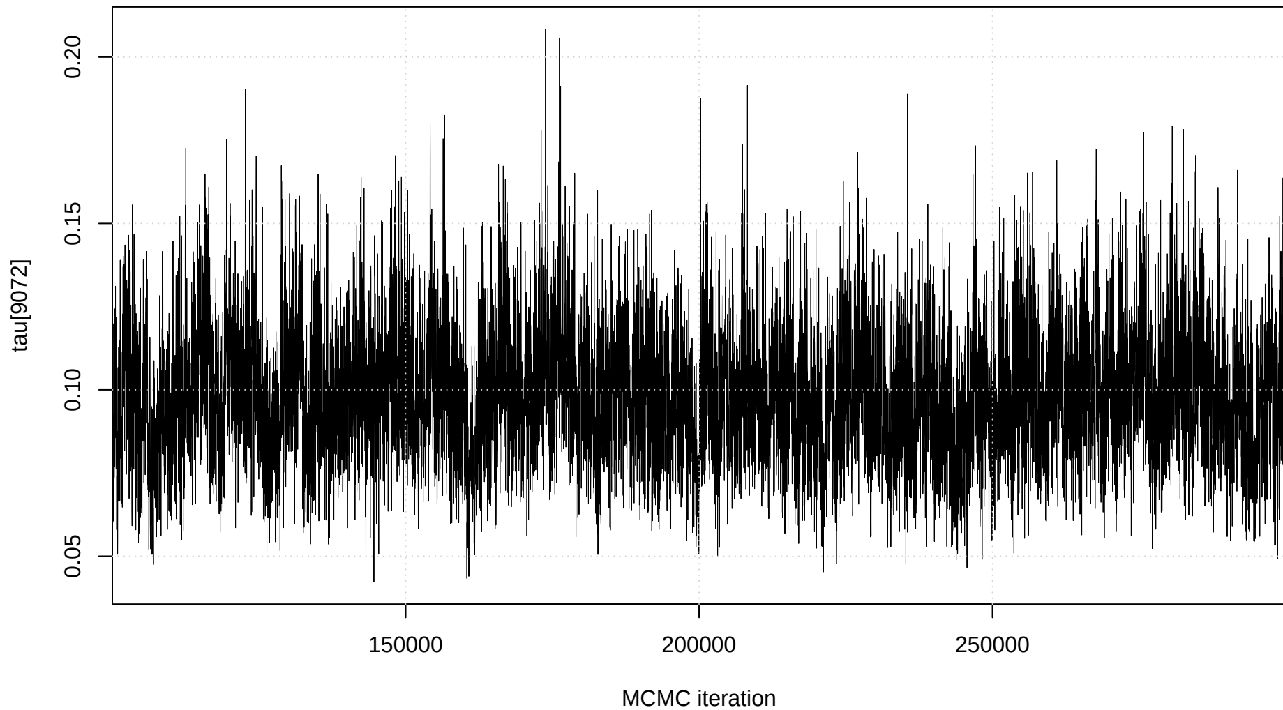
Trace plot: tau[9072]
