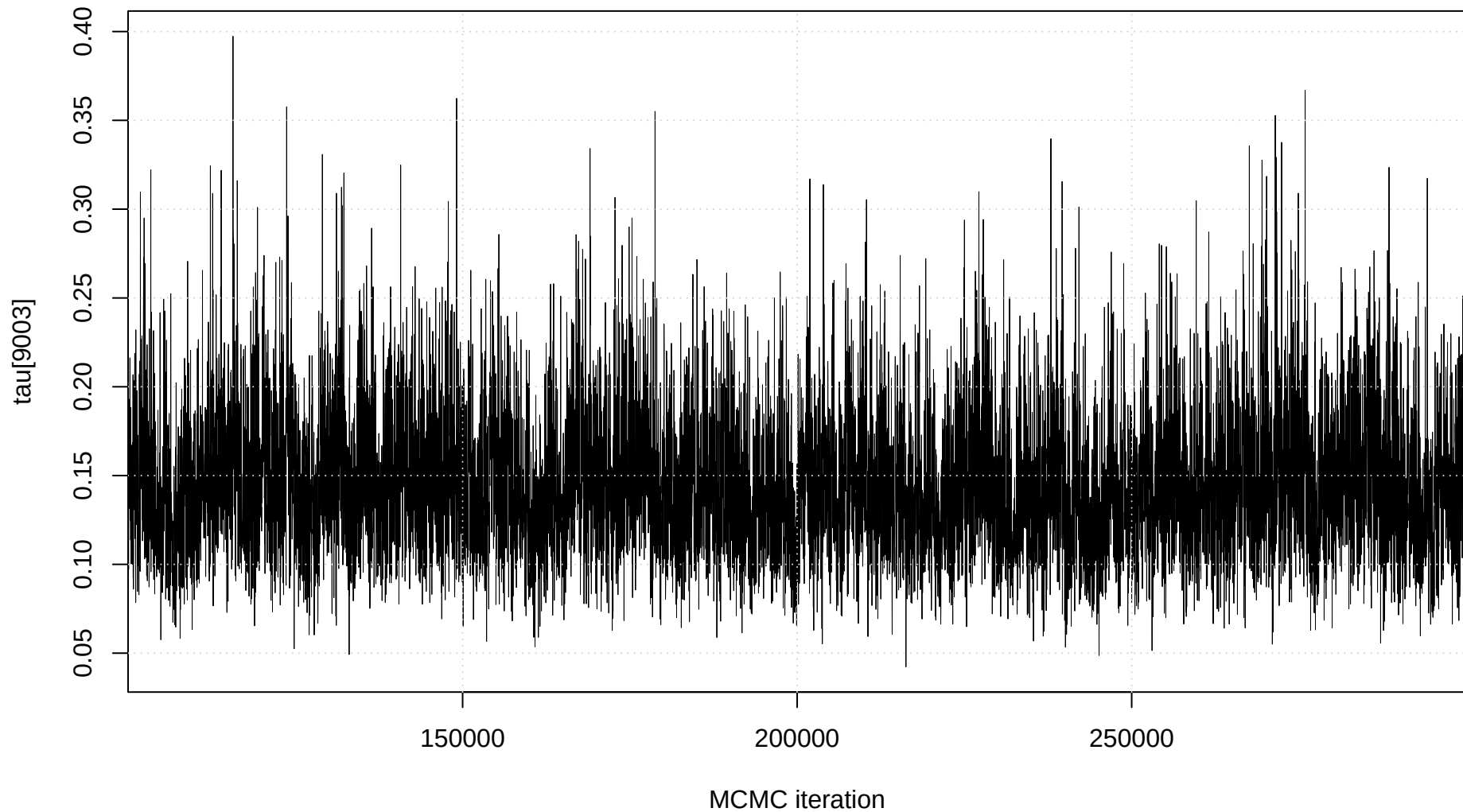
Trace plot: tau[9003]
