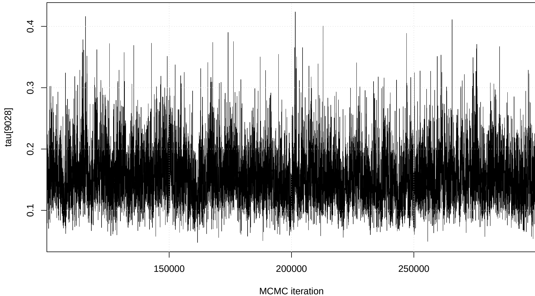
Trace plot: tau[9028]
