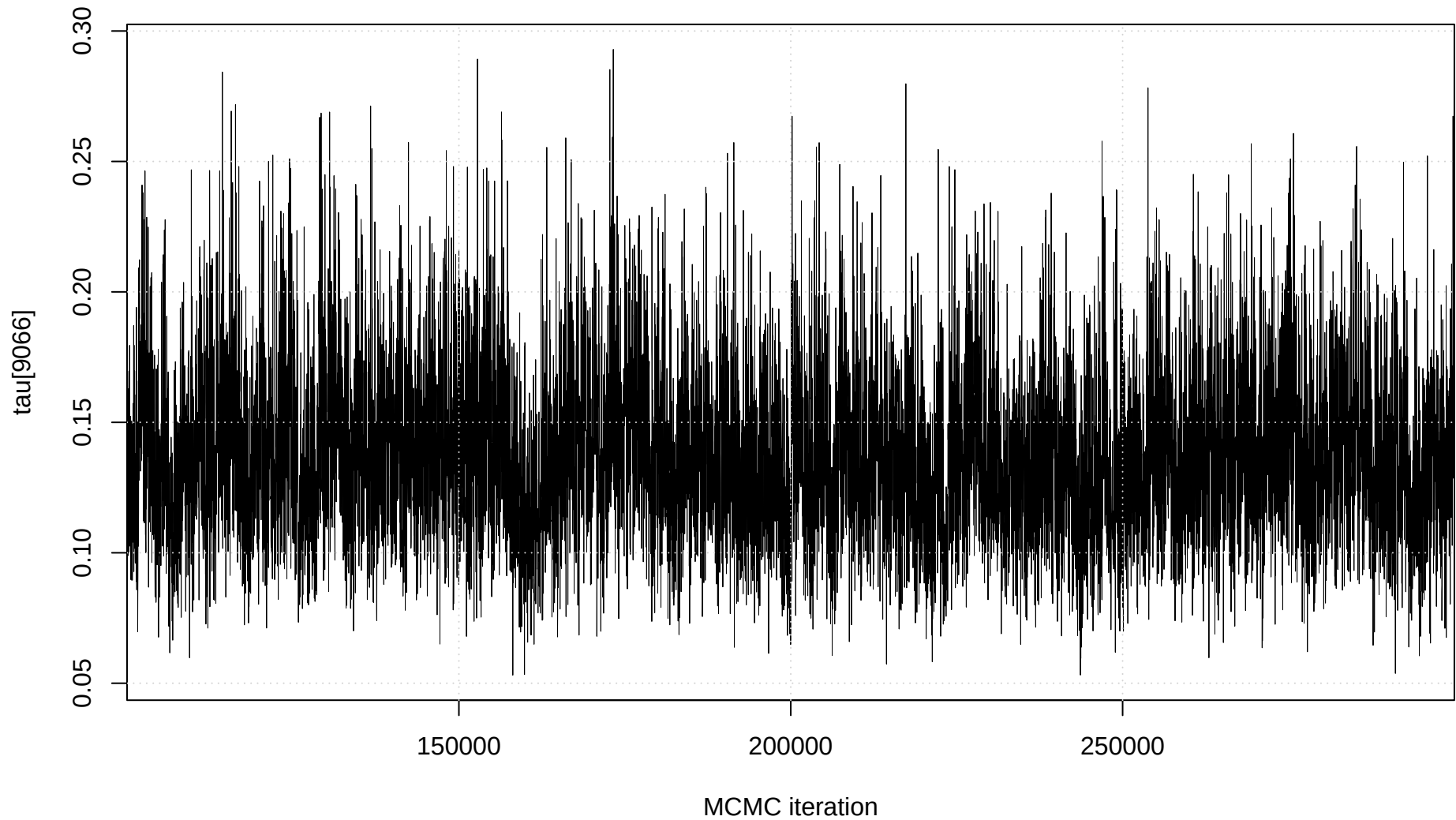
Trace plot: tau[9066]
