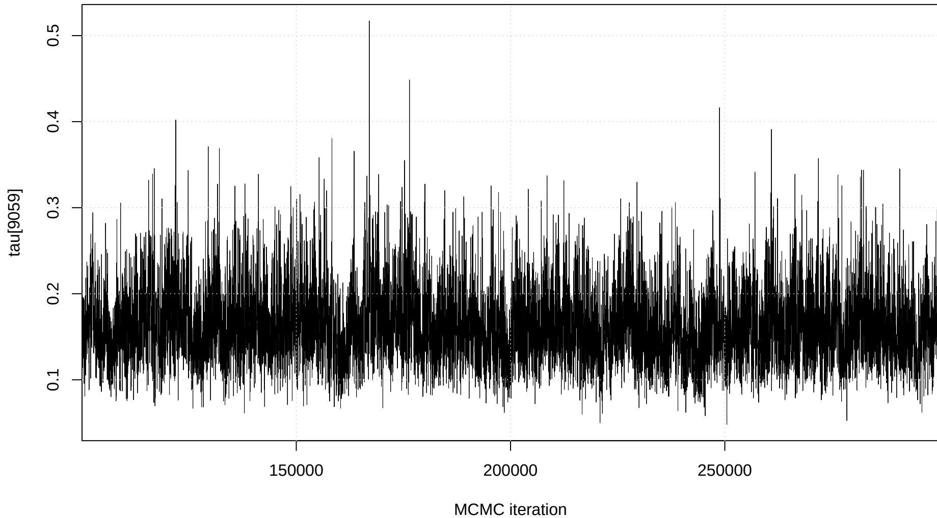
Trace plot: tau[9059]
