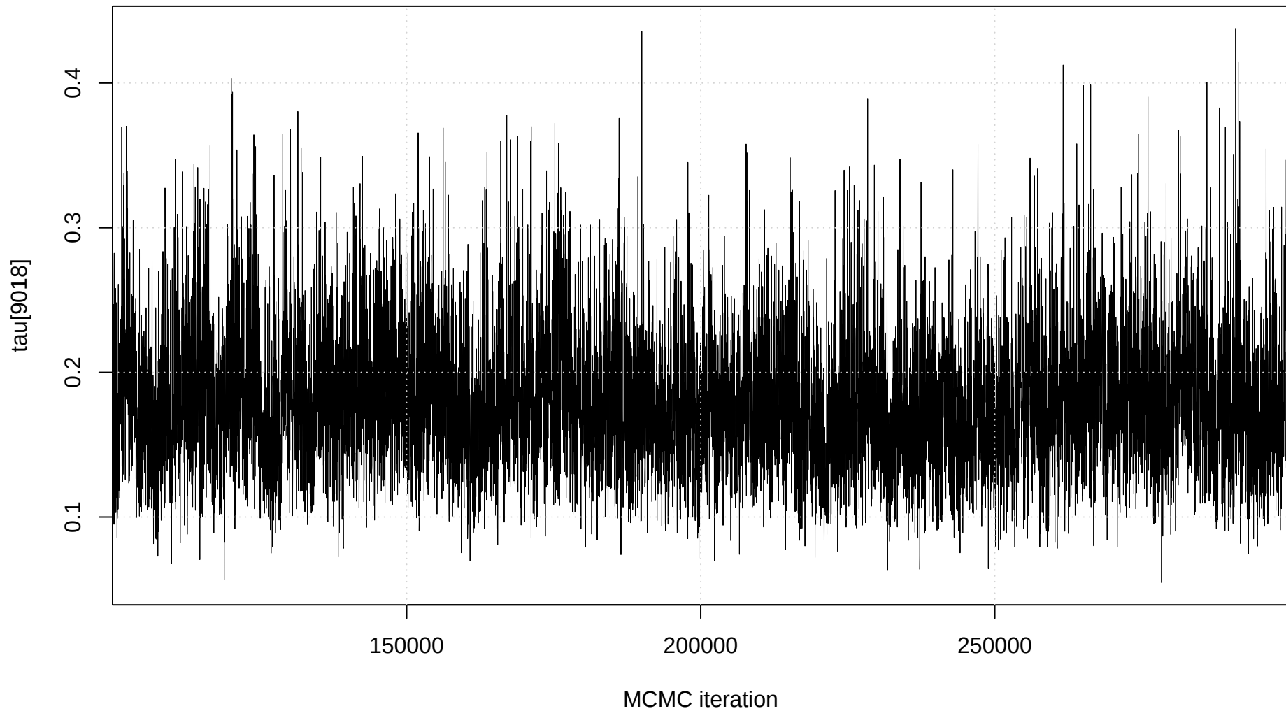
Trace plot: tau[9018]
