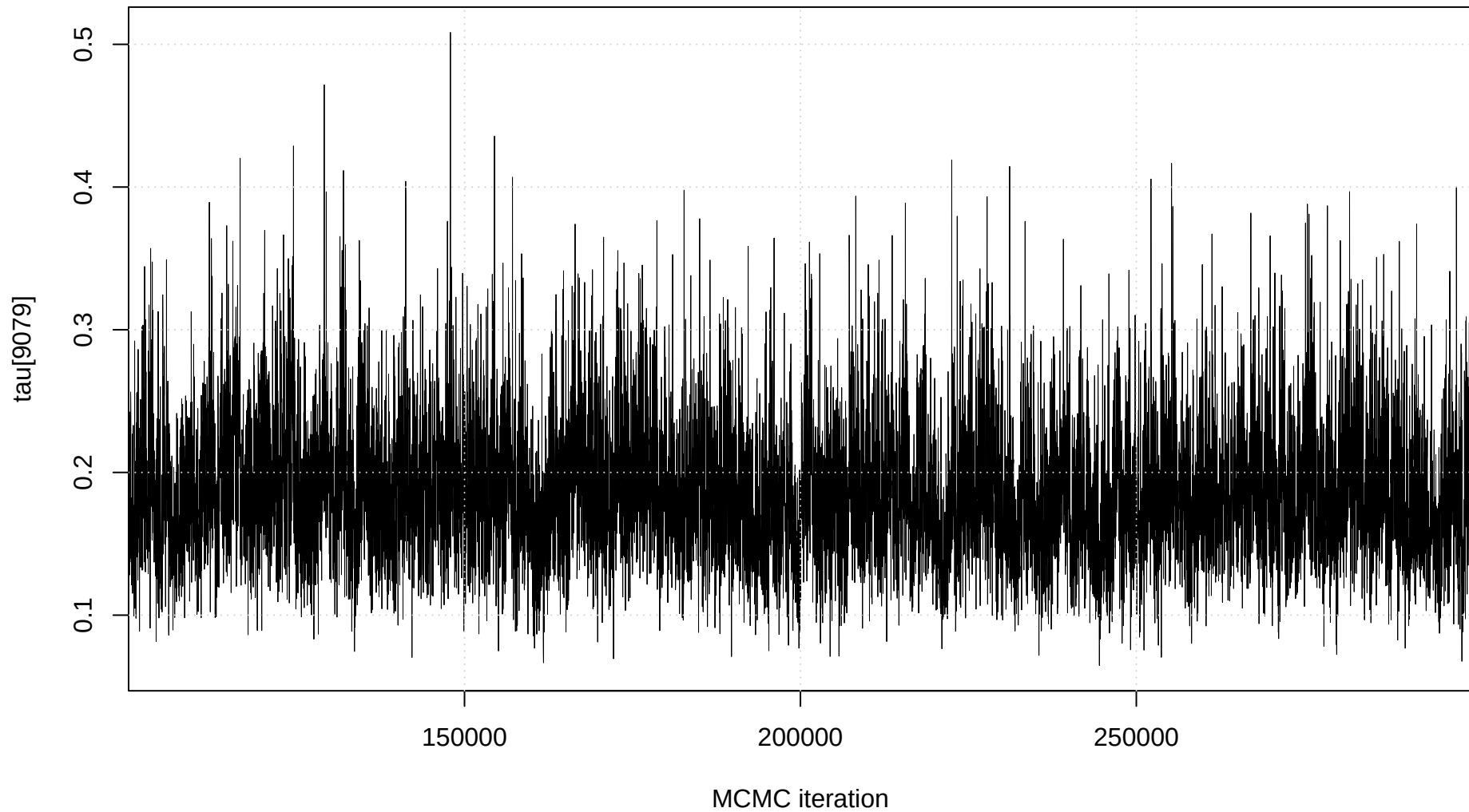
Trace plot: tau[9079]
