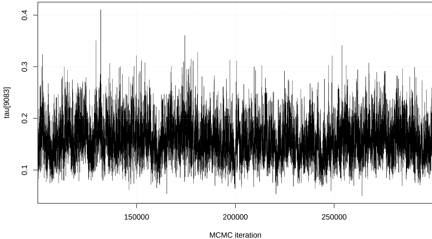
Trace plot: tau[9083]
