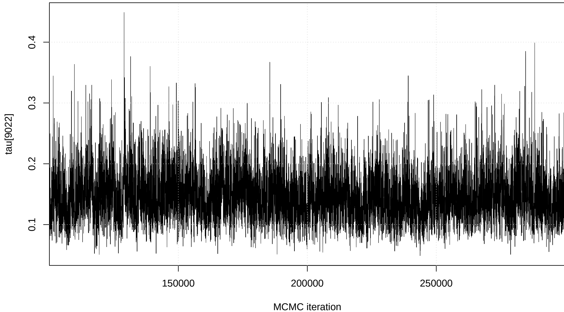
Trace plot: tau[9022]
