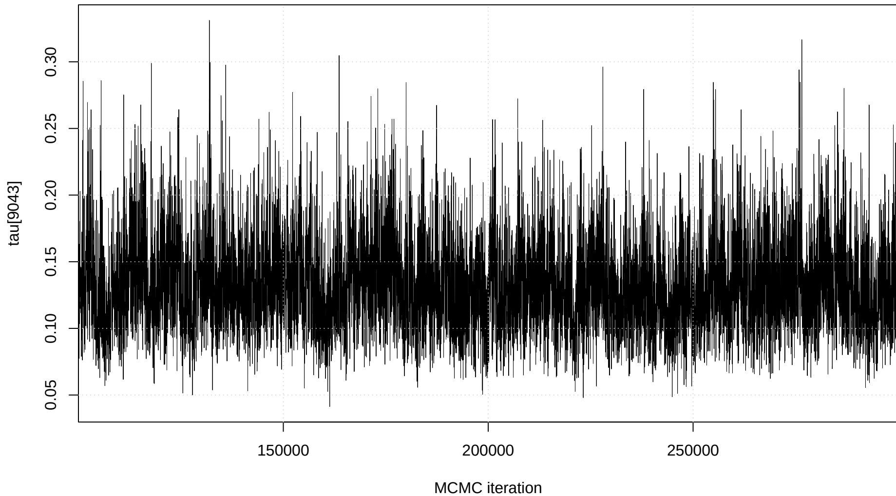
Trace plot: tau[9043]
