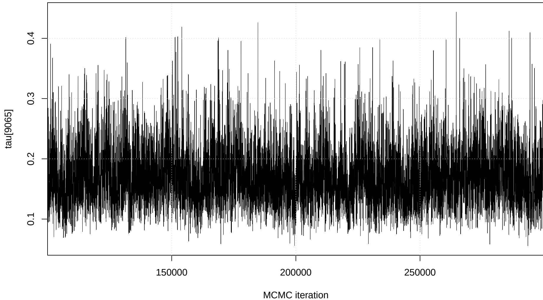
Trace plot: tau[9065]
