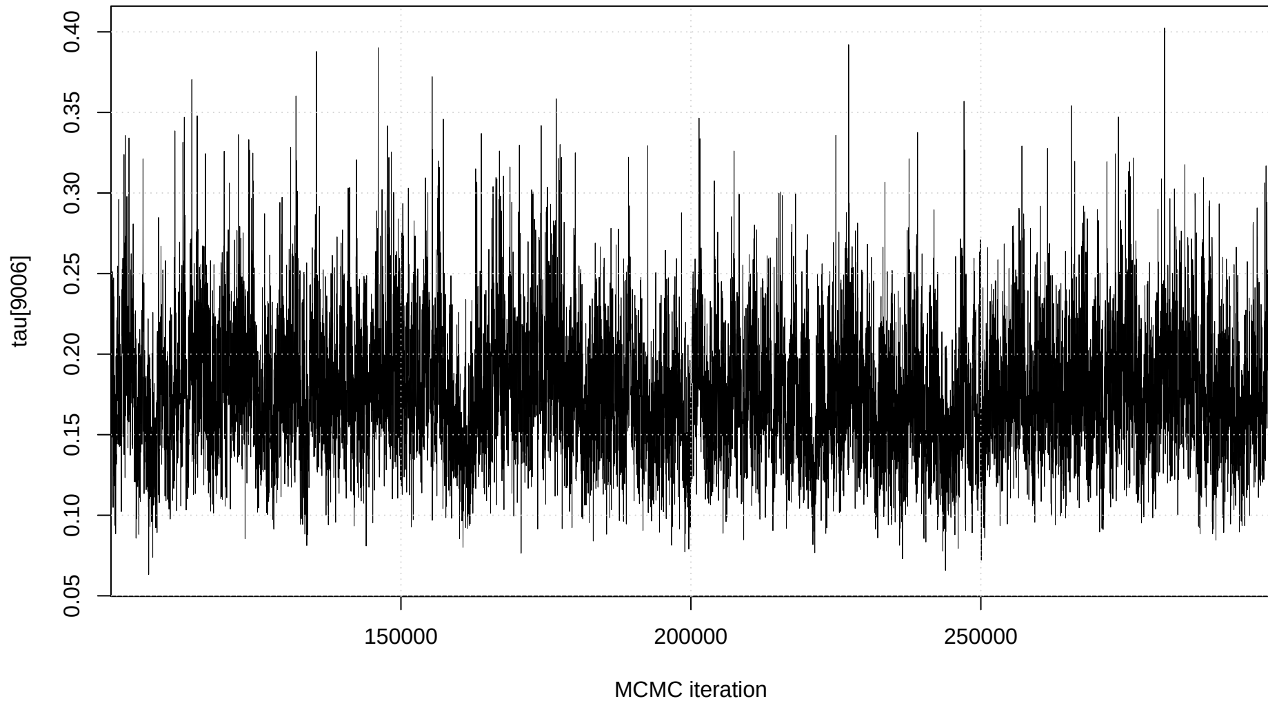
Trace plot: tau[9006]
