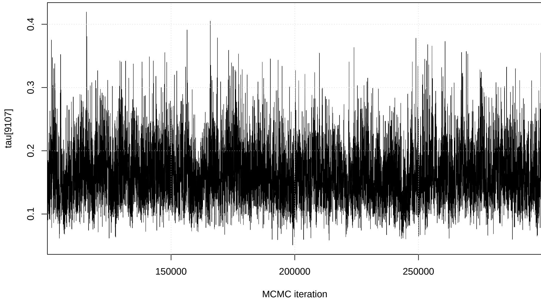
Trace plot: tau[9107]
