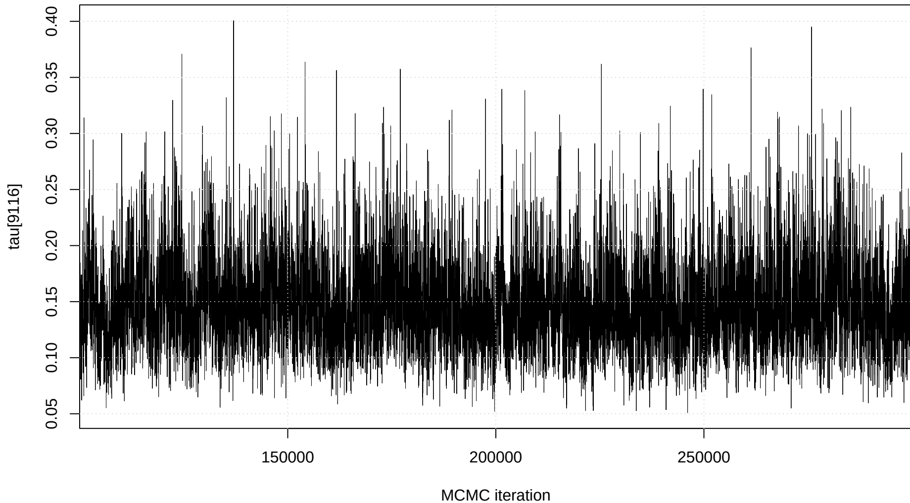
Trace plot: tau[9116]
