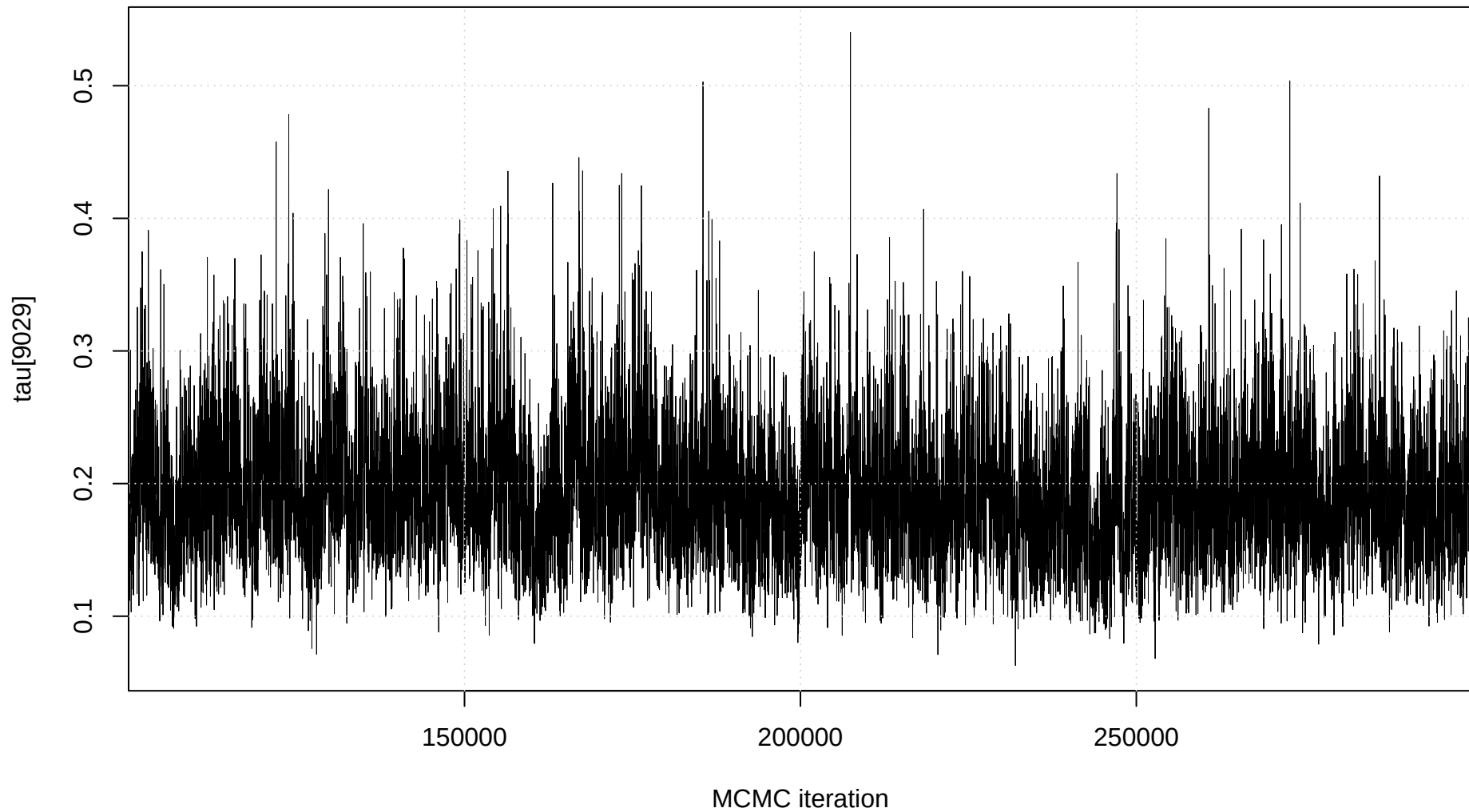
Trace plot: tau[9029]
