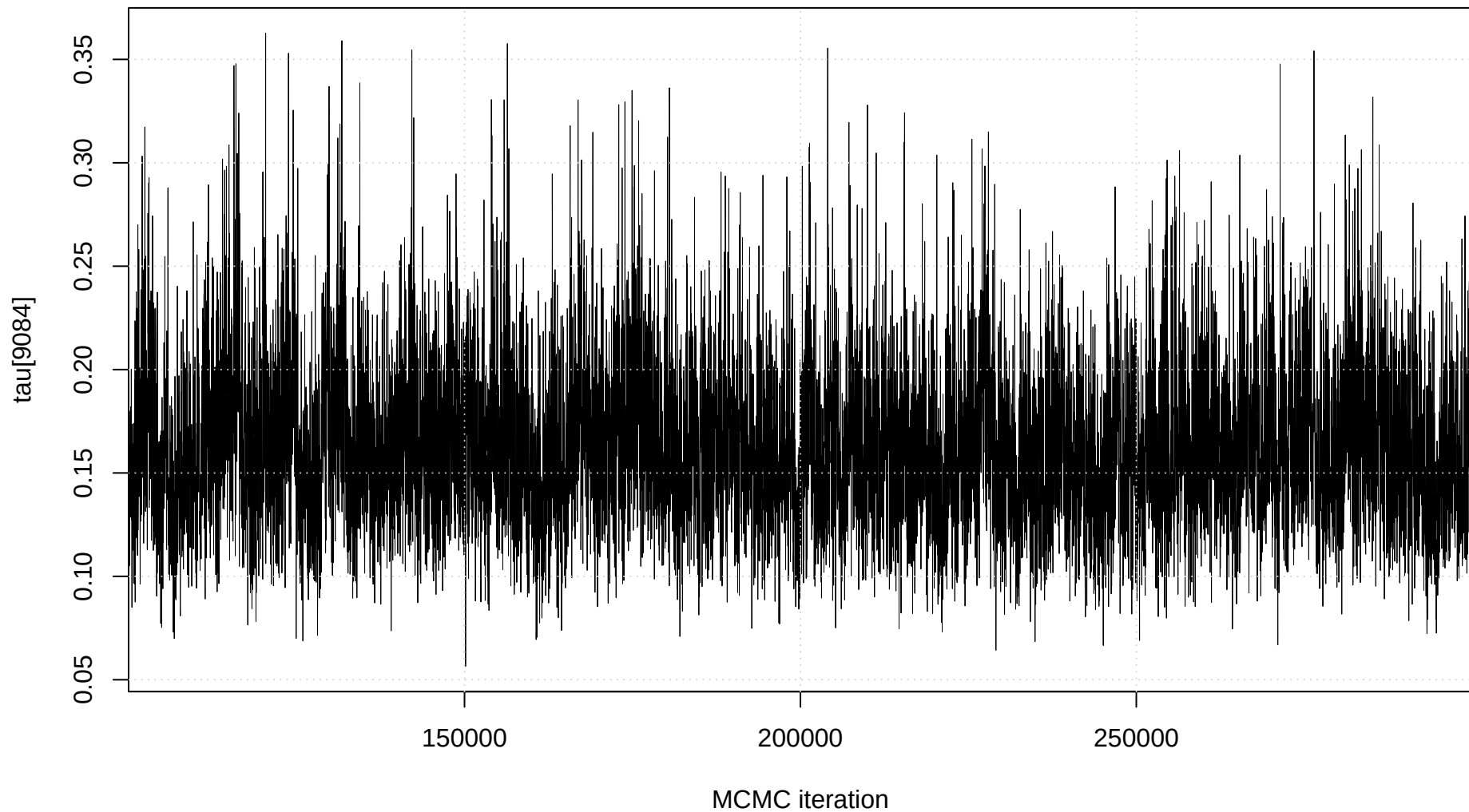
Trace plot: tau[9084]
