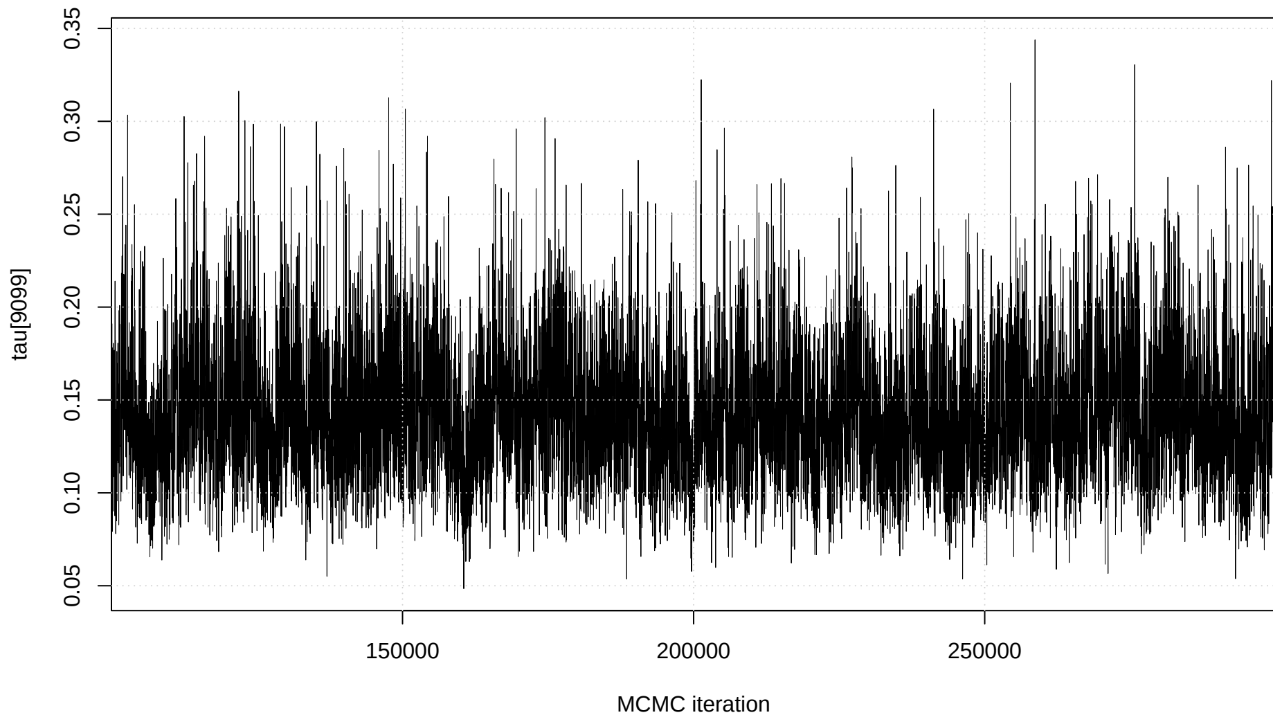
Trace plot: tau[9099]
