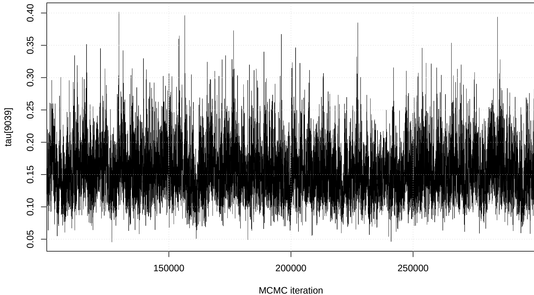
Trace plot: tau[9039]
