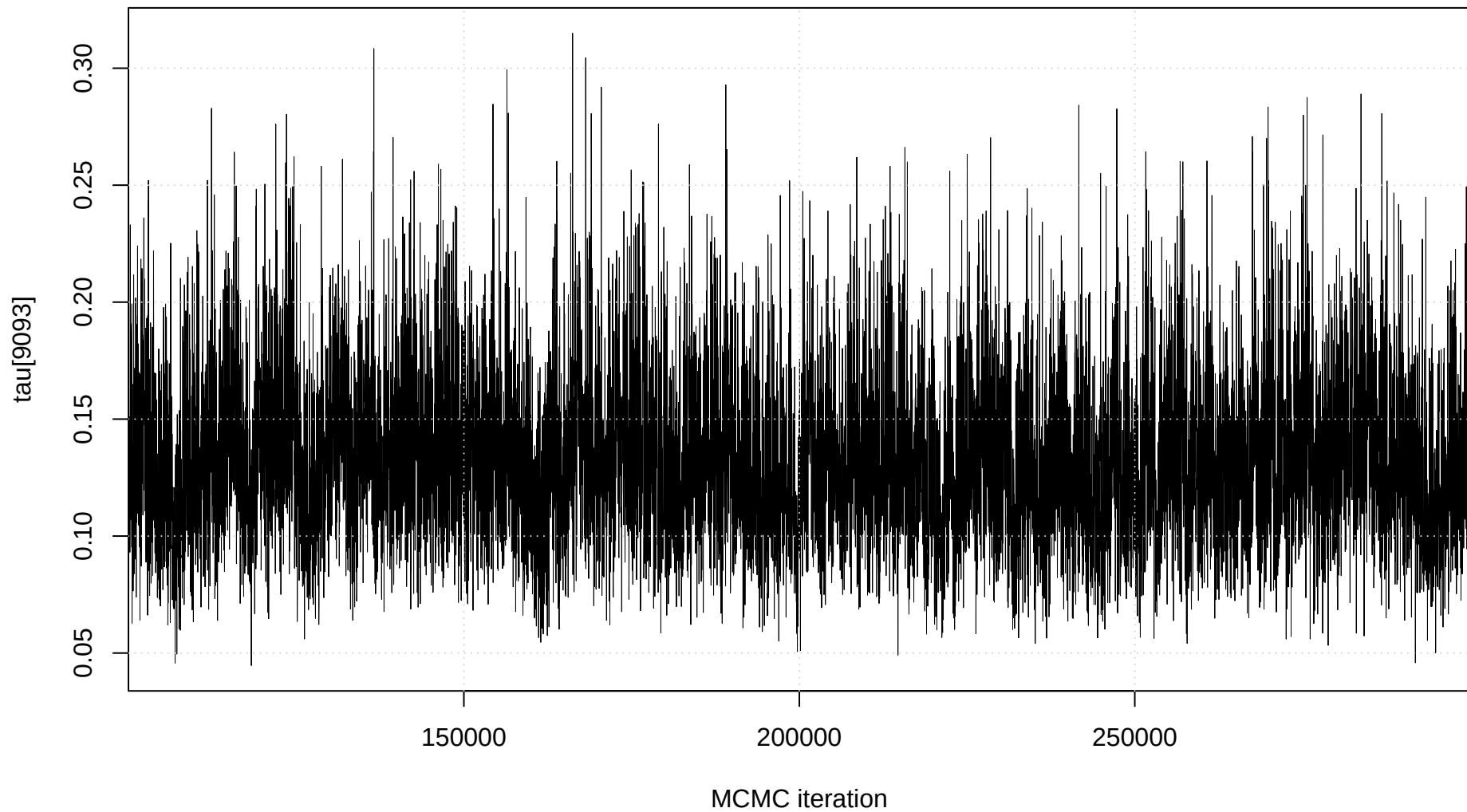
Trace plot: tau[9093]
