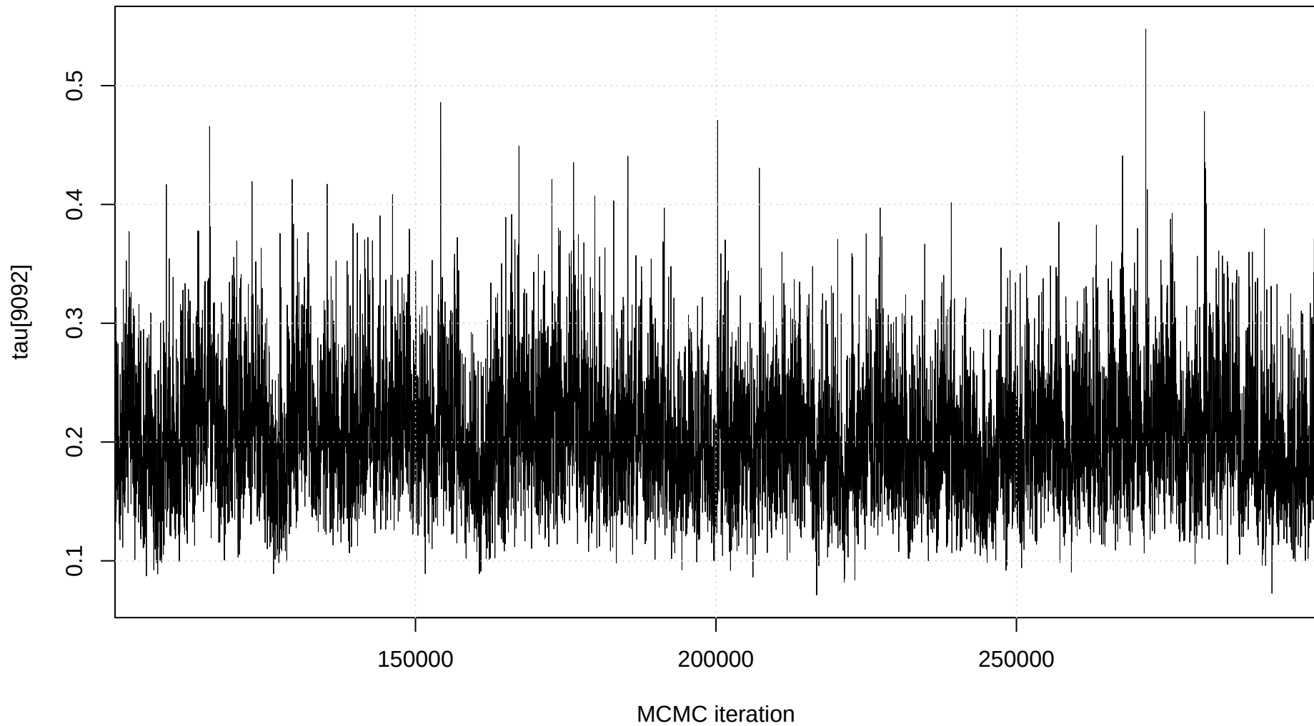
Trace plot: tau[9092]
