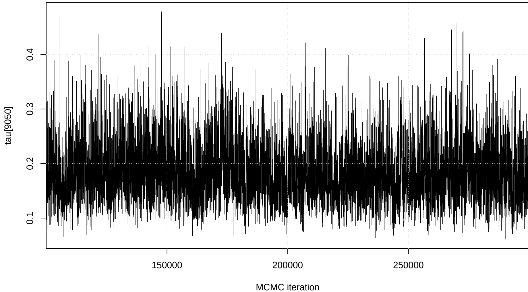
Trace plot: tau[9050]
