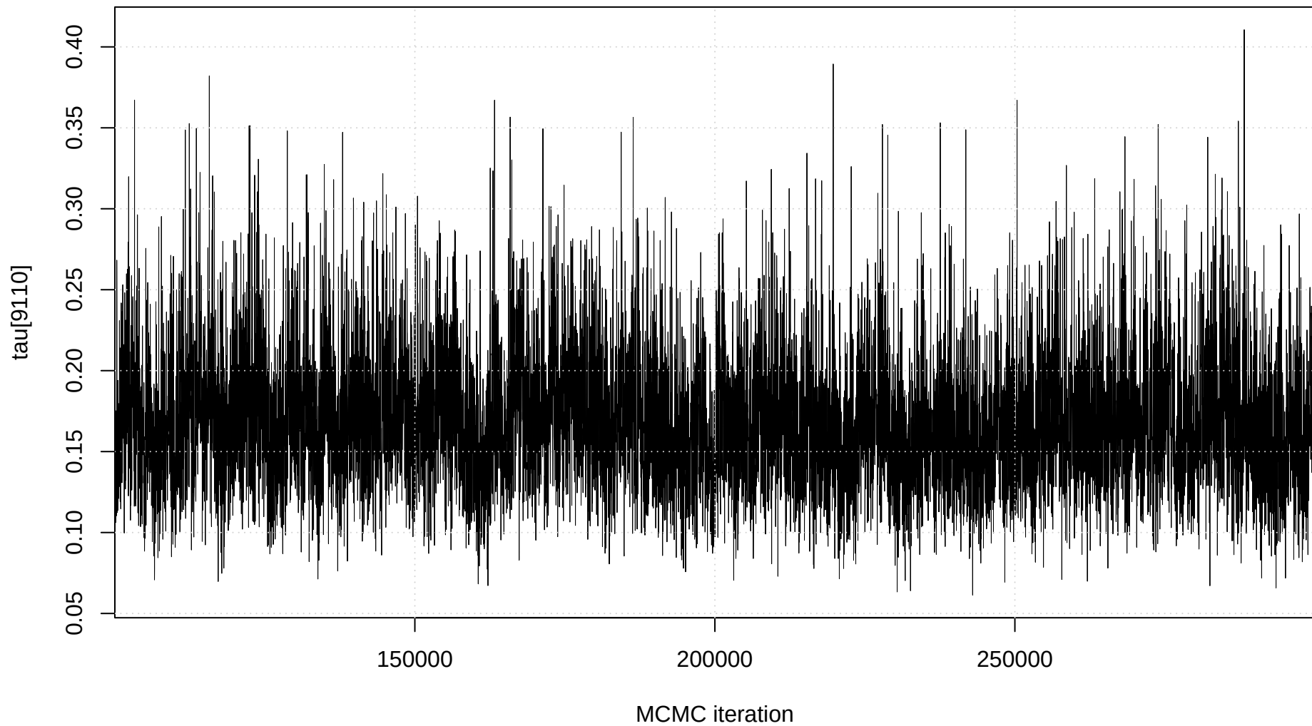
Trace plot: tau[9110]
