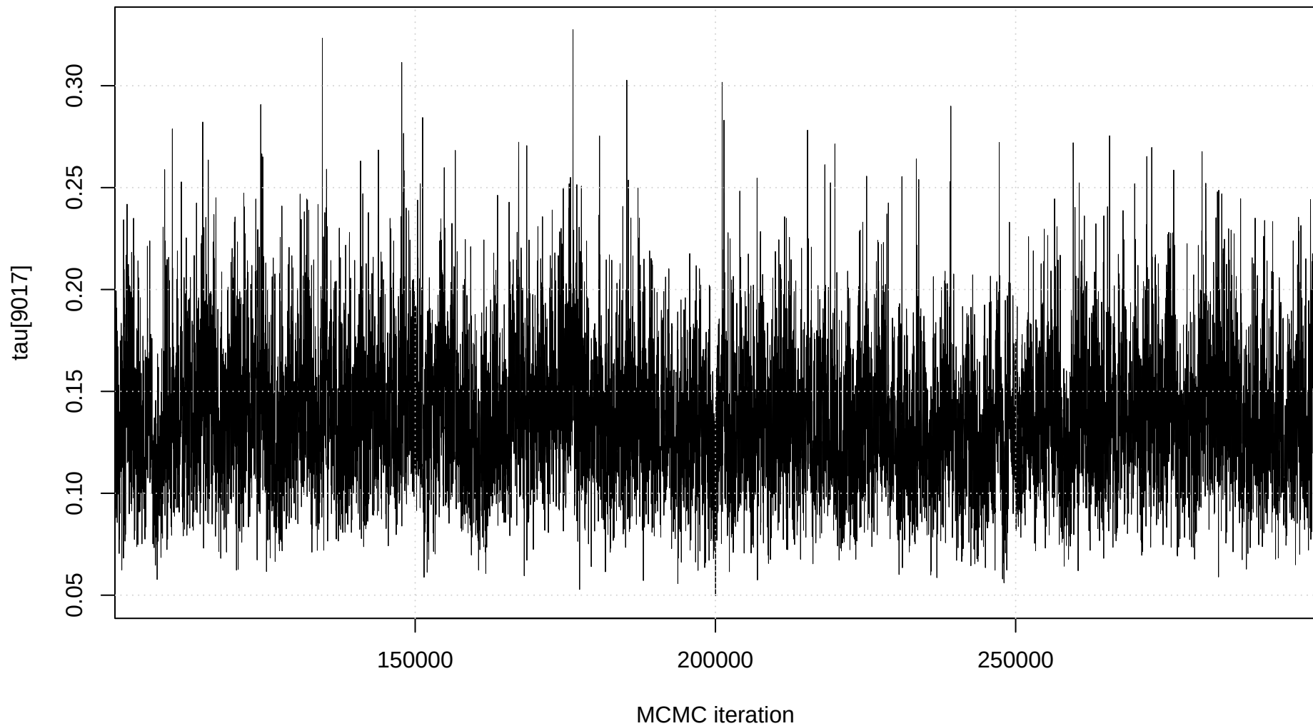
Trace plot: tau[9017]
