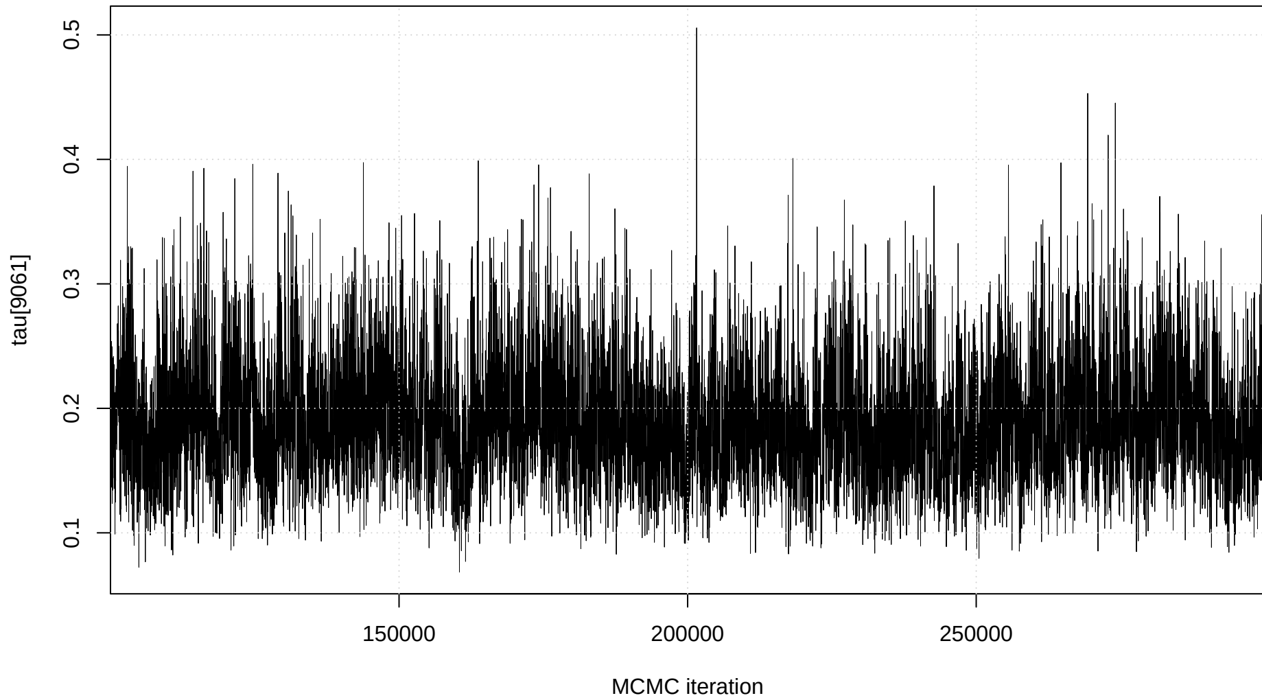
Trace plot: tau[9061]
