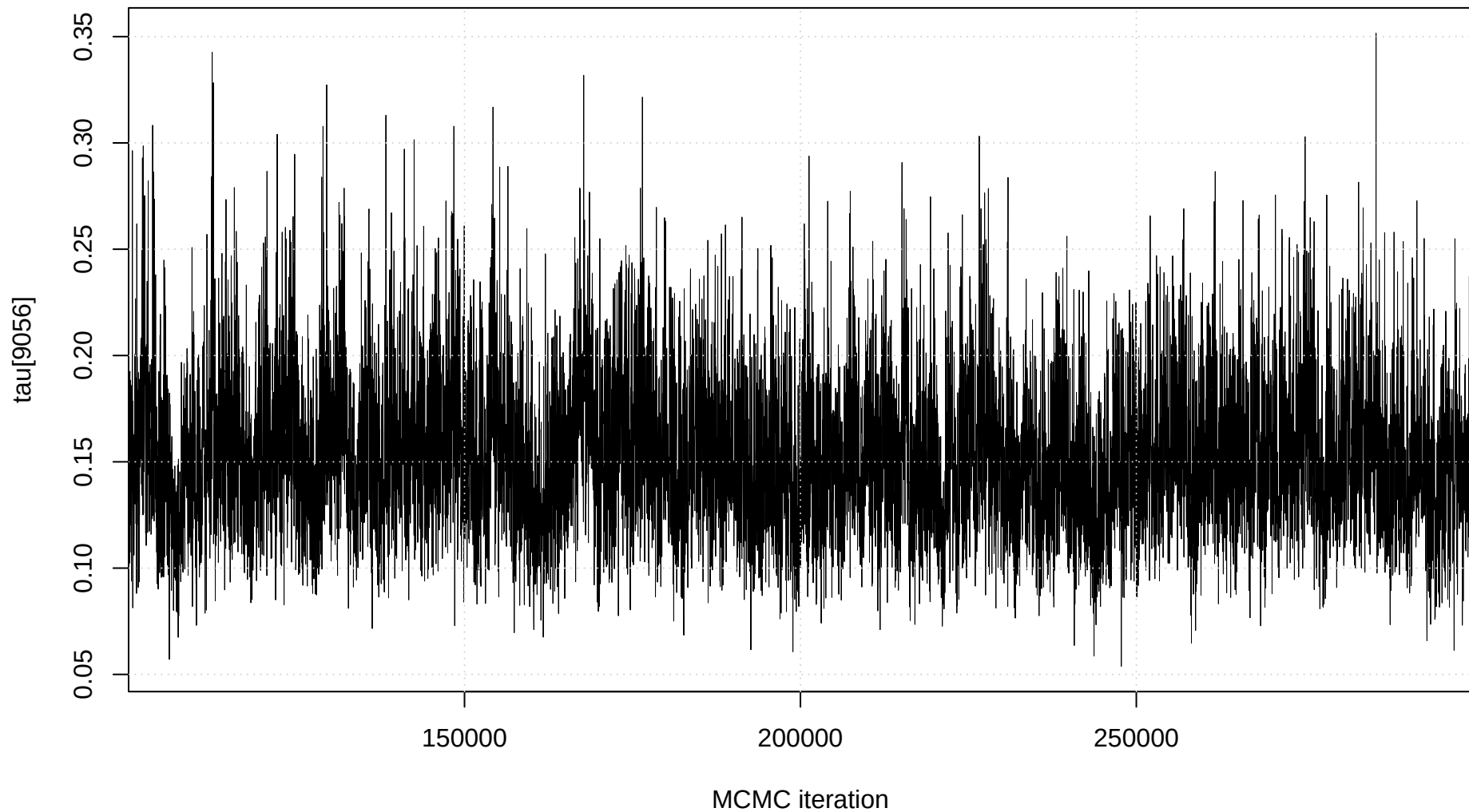
Trace plot: tau[9056]
