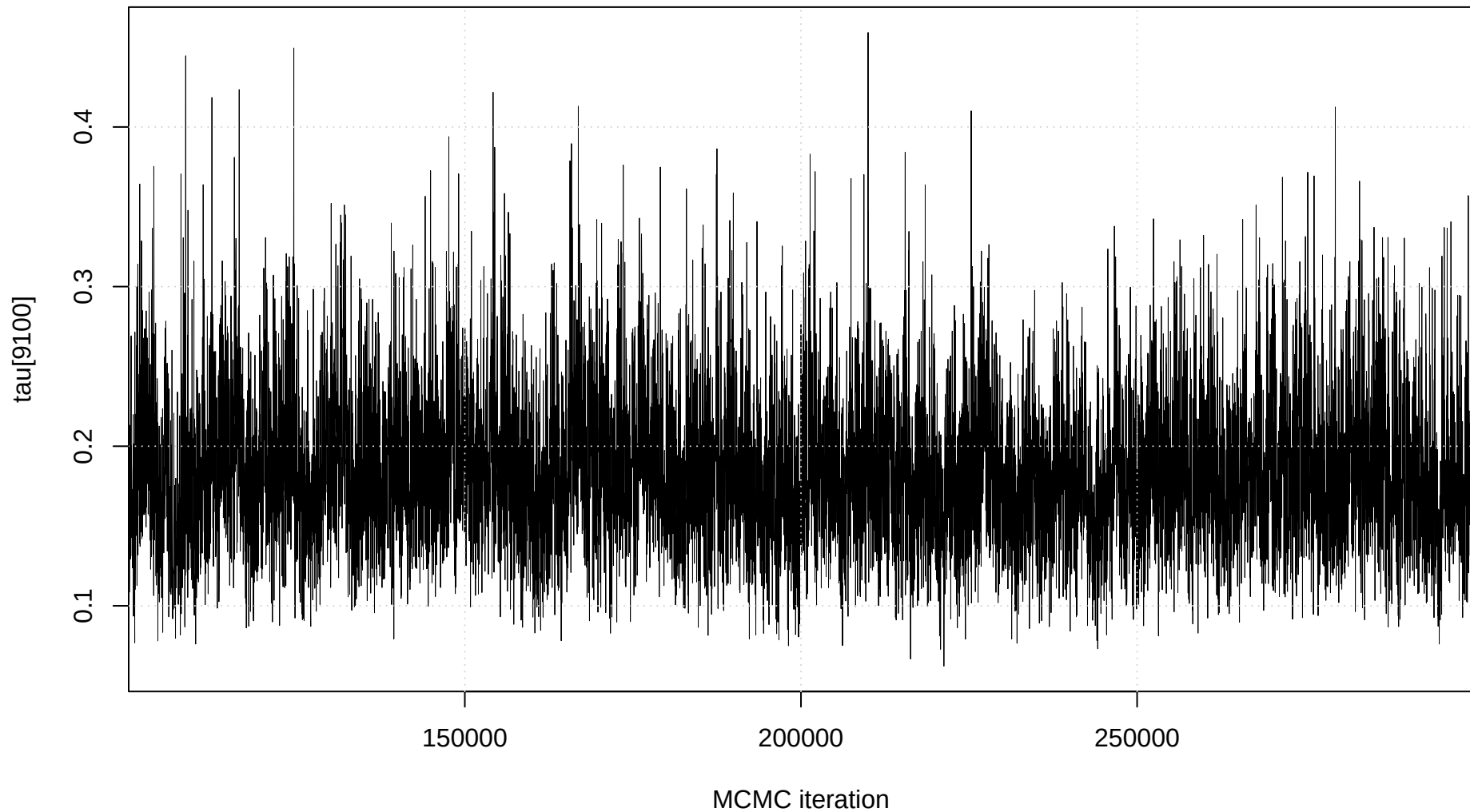
Trace plot: tau[9100]
