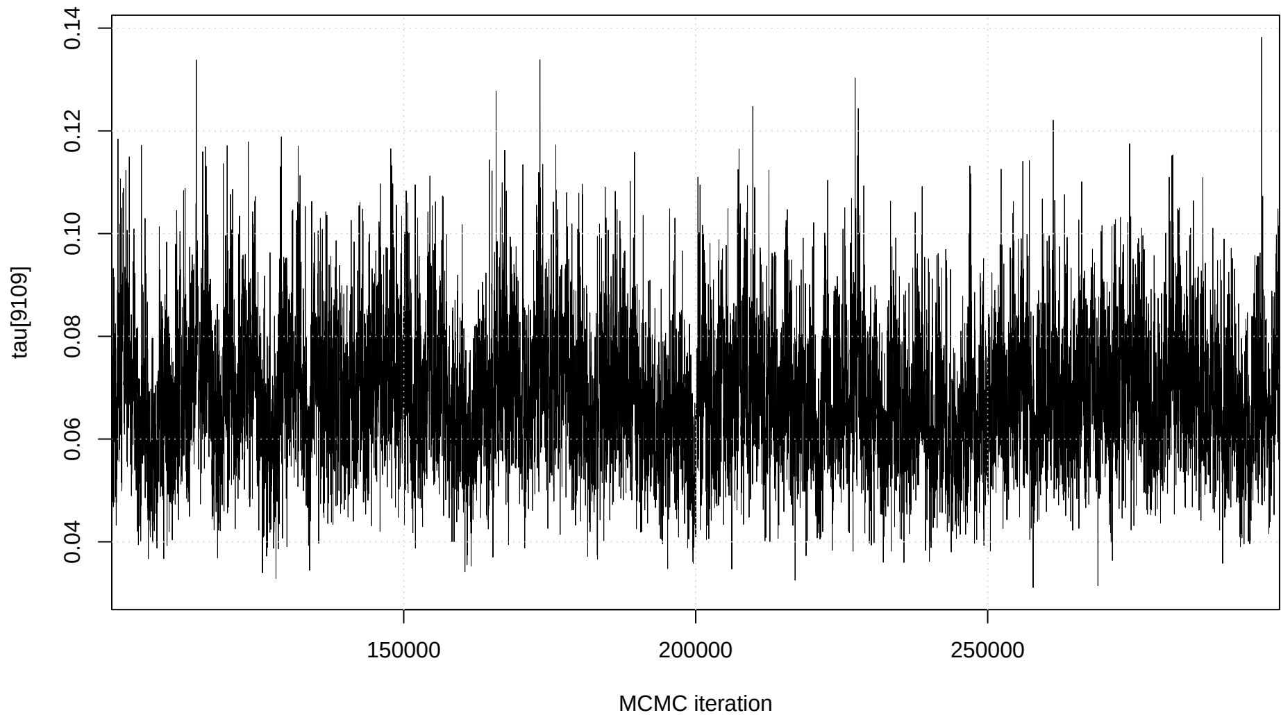
Trace plot: tau[9109]
