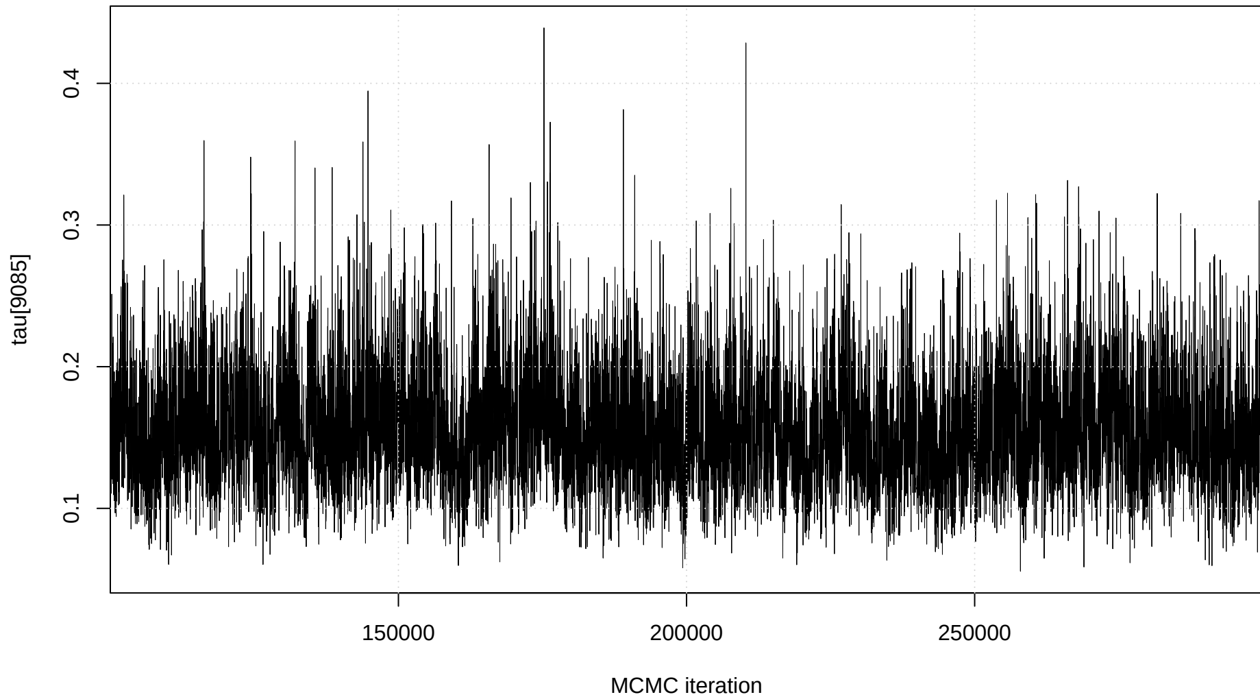
Trace plot: tau[9085]
