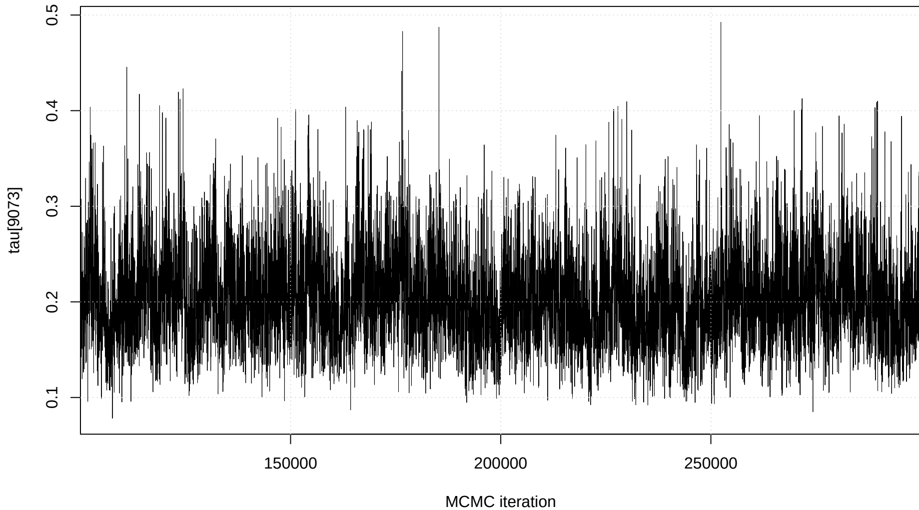
Trace plot: tau[9073]
