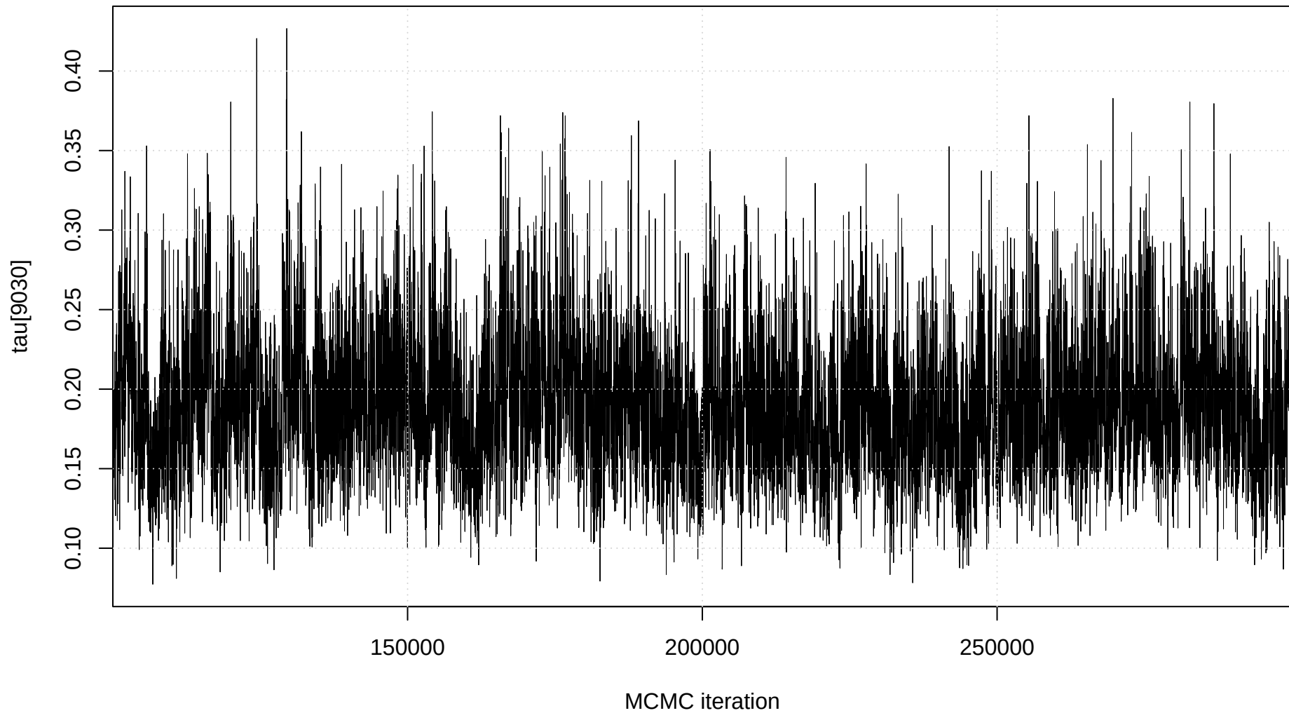
Trace plot: tau[9030]
