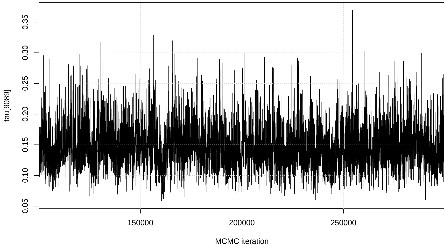
Trace plot: tau[9089]
