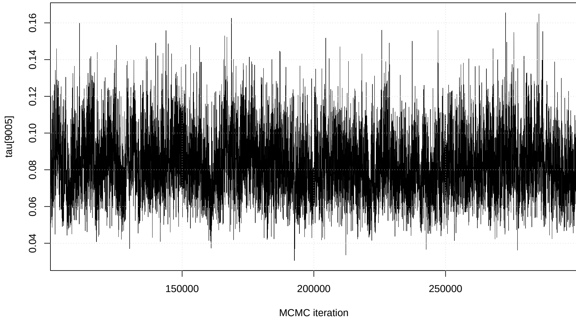
Trace plot: tau[9005]
