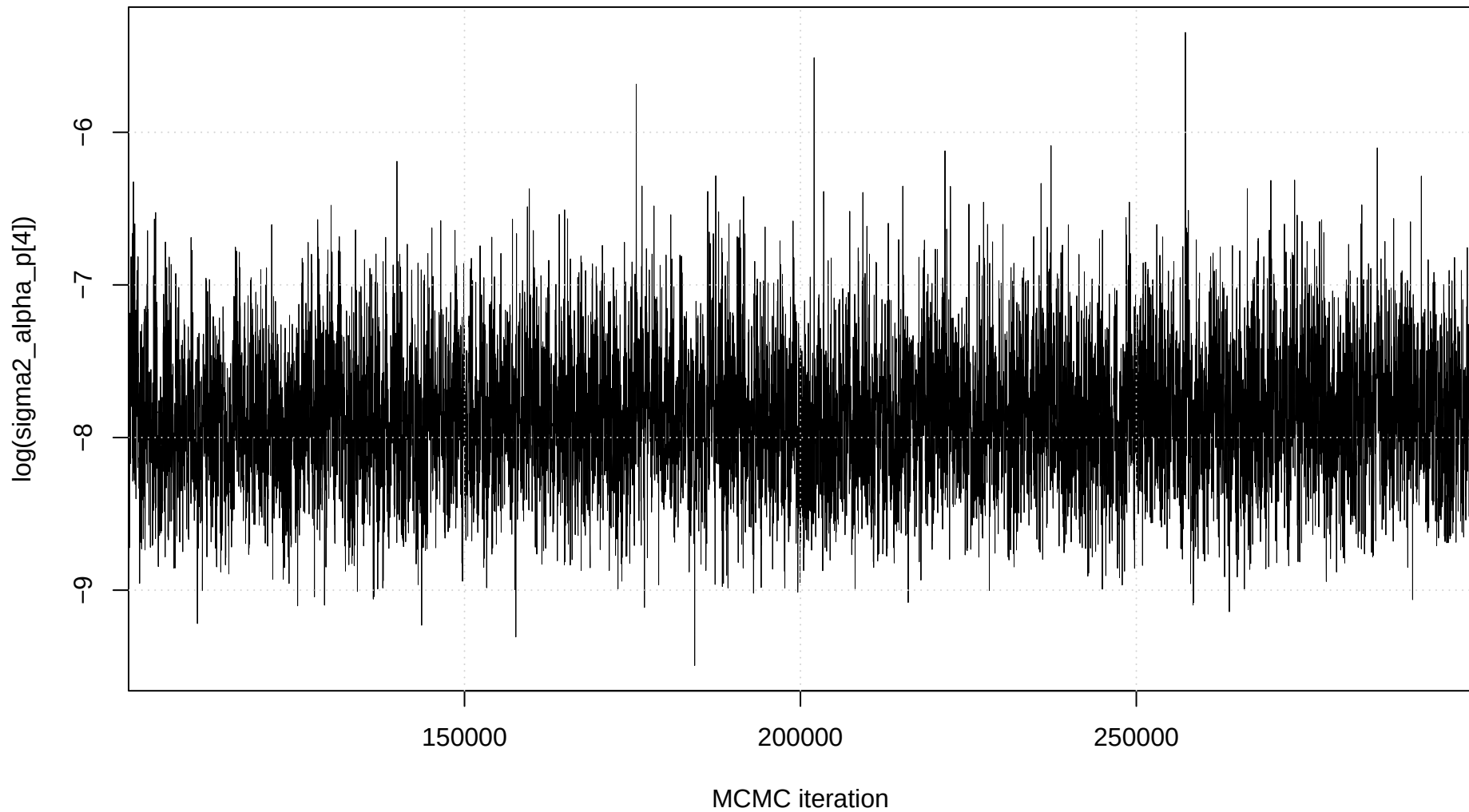
Trace plot: \log(\text{sigma2\_alpha\_p}[4])
