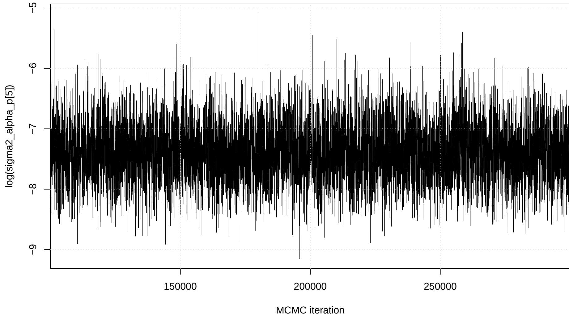
Trace plot: \log(\text{sigma2\_alpha\_p}[5])
