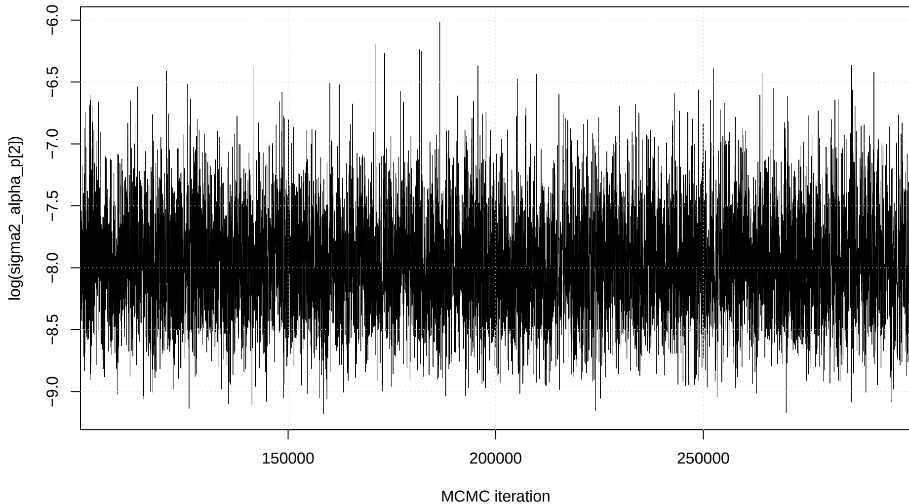
Trace plot: \log(\text{sigma2\_alpha\_p}[2])
