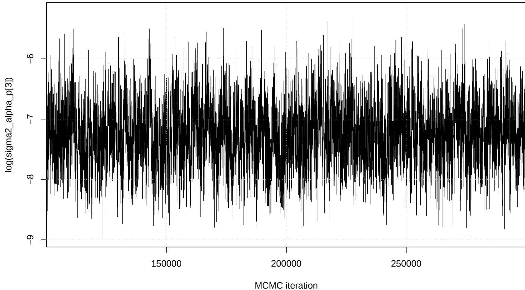
Trace plot: \log(\text{sigma2\_alpha\_p}[3])
