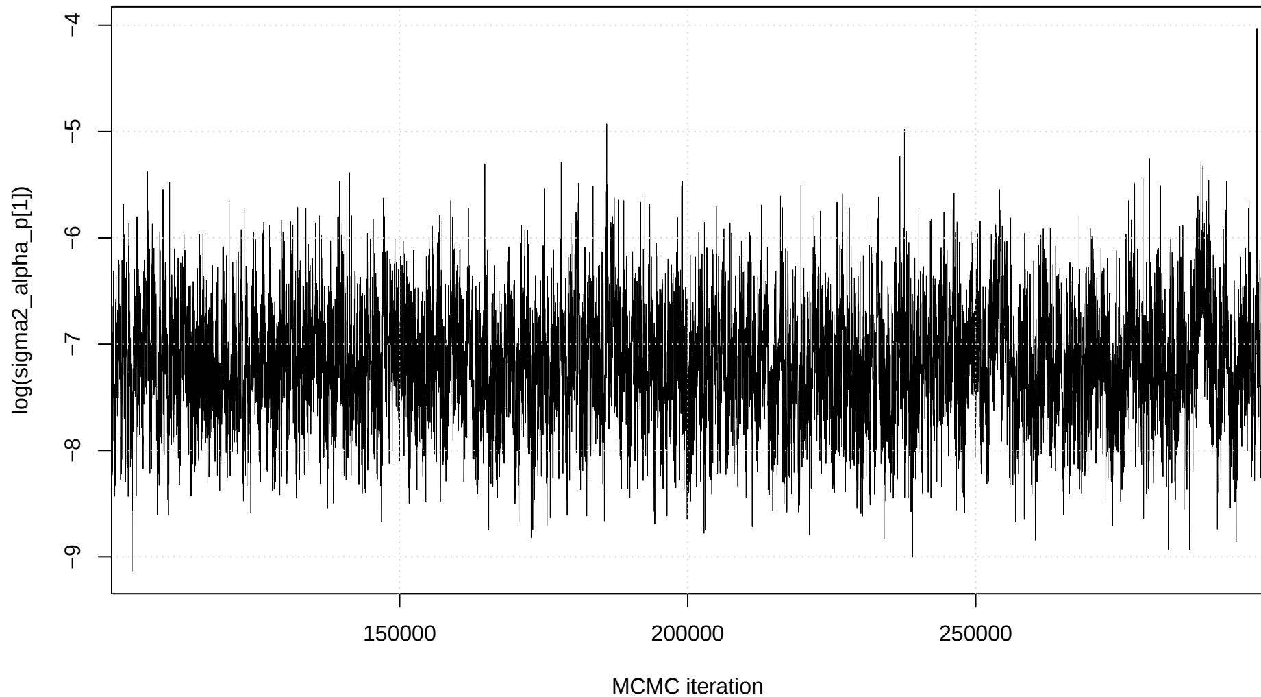
Trace plot: \log(\text{sigma2\_alpha\_p}[1])
