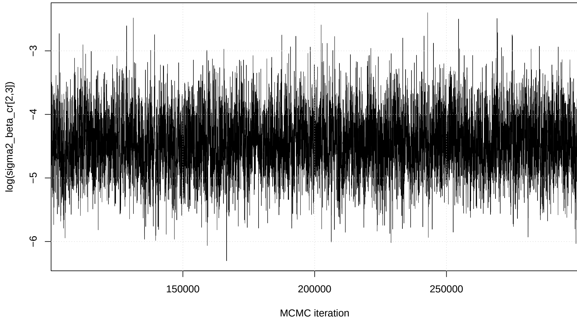
Trace plot: \log(\text{sigma2\_beta\_cr}[2,3])
