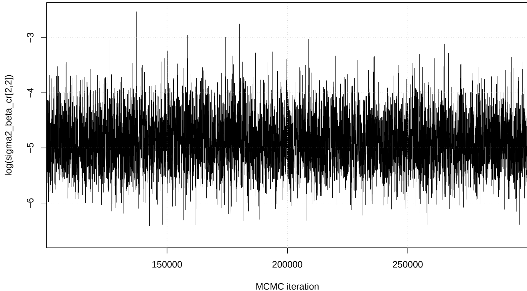
Trace plot: \log(\text{sigma2\_beta\_cr}[2,2])
