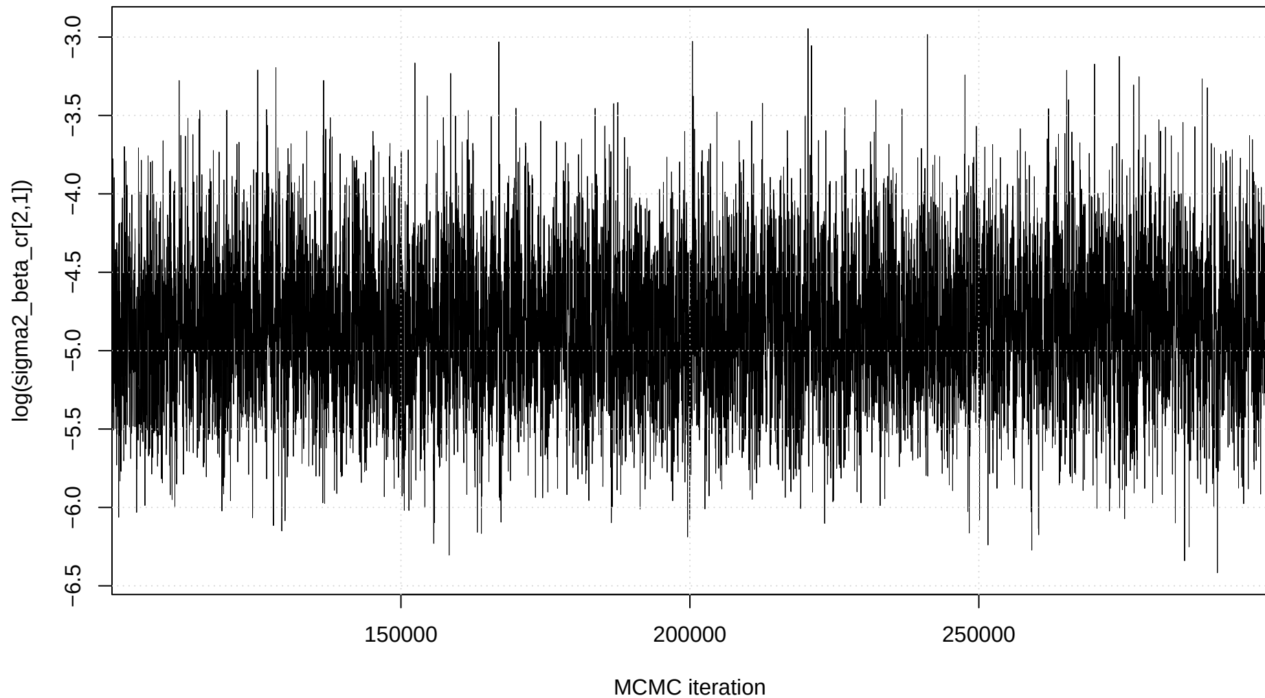
Trace plot: \log(\text{sigma2\_beta\_cr}[2,1])
