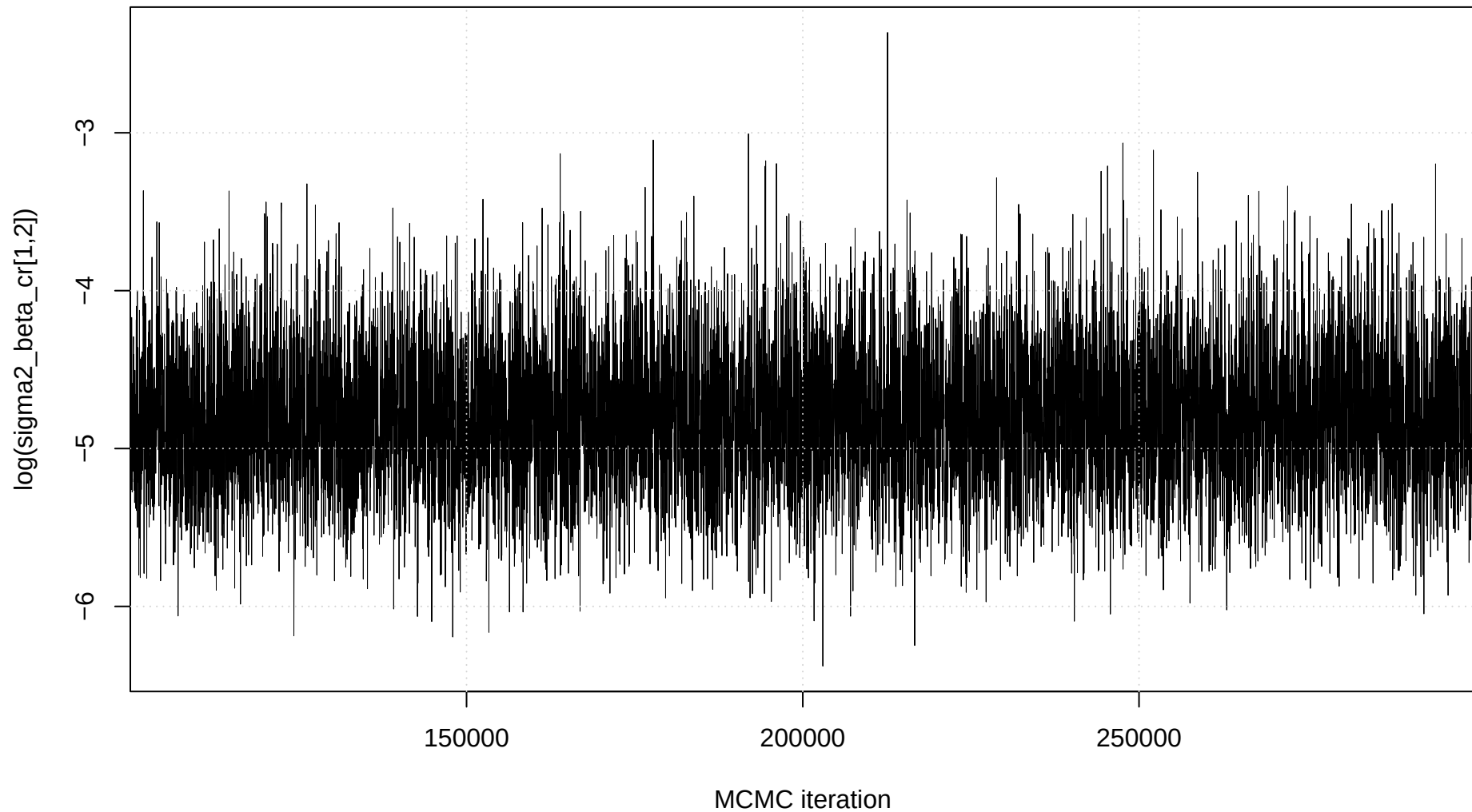
Trace plot: \log(\text{sigma2\_beta\_cr}[1,2])
