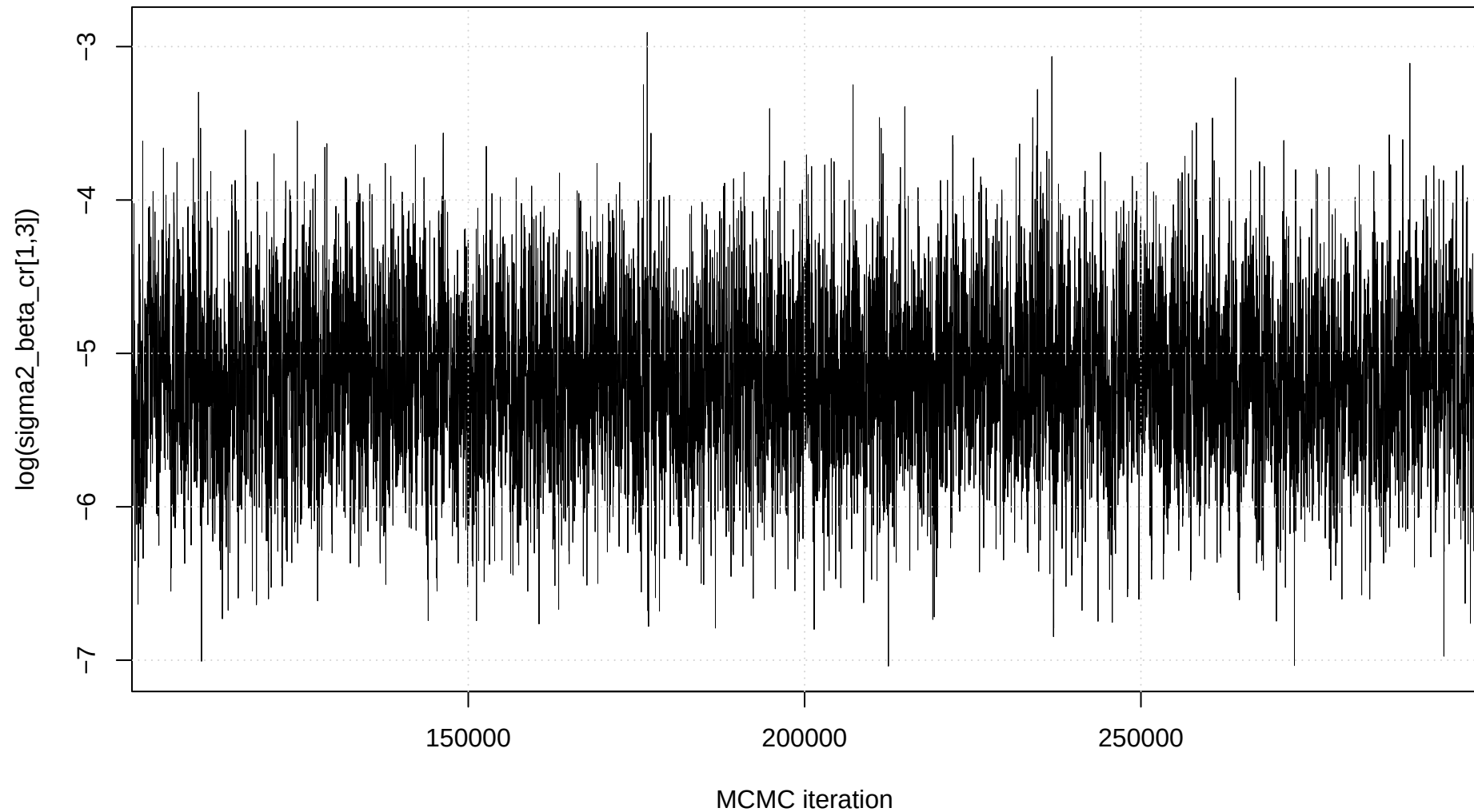
Trace plot: \log(\text{sigma2\_beta\_cr}[1,3])
