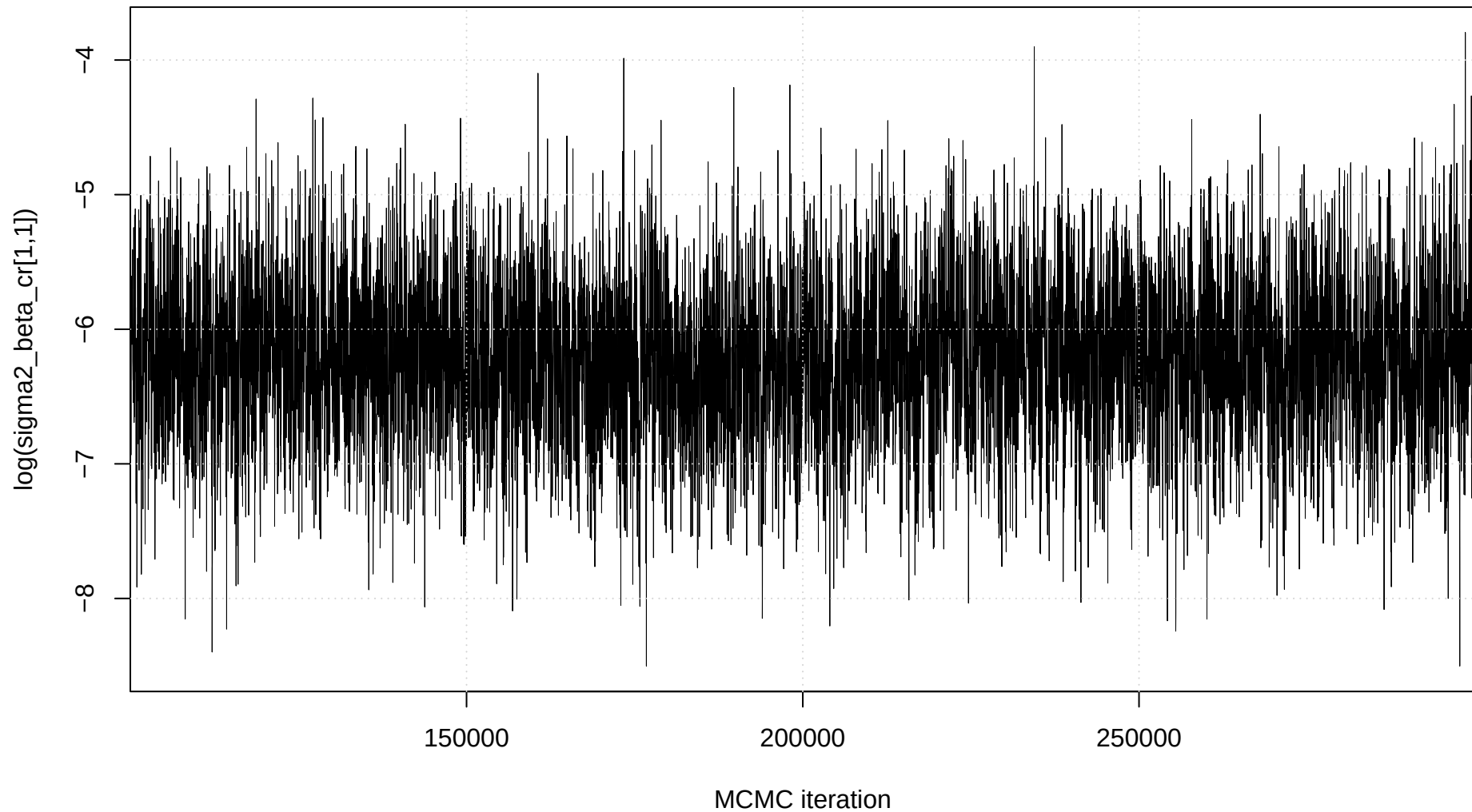
Trace plot: \log(\text{sigma2\_beta\_cr}[1,1])
