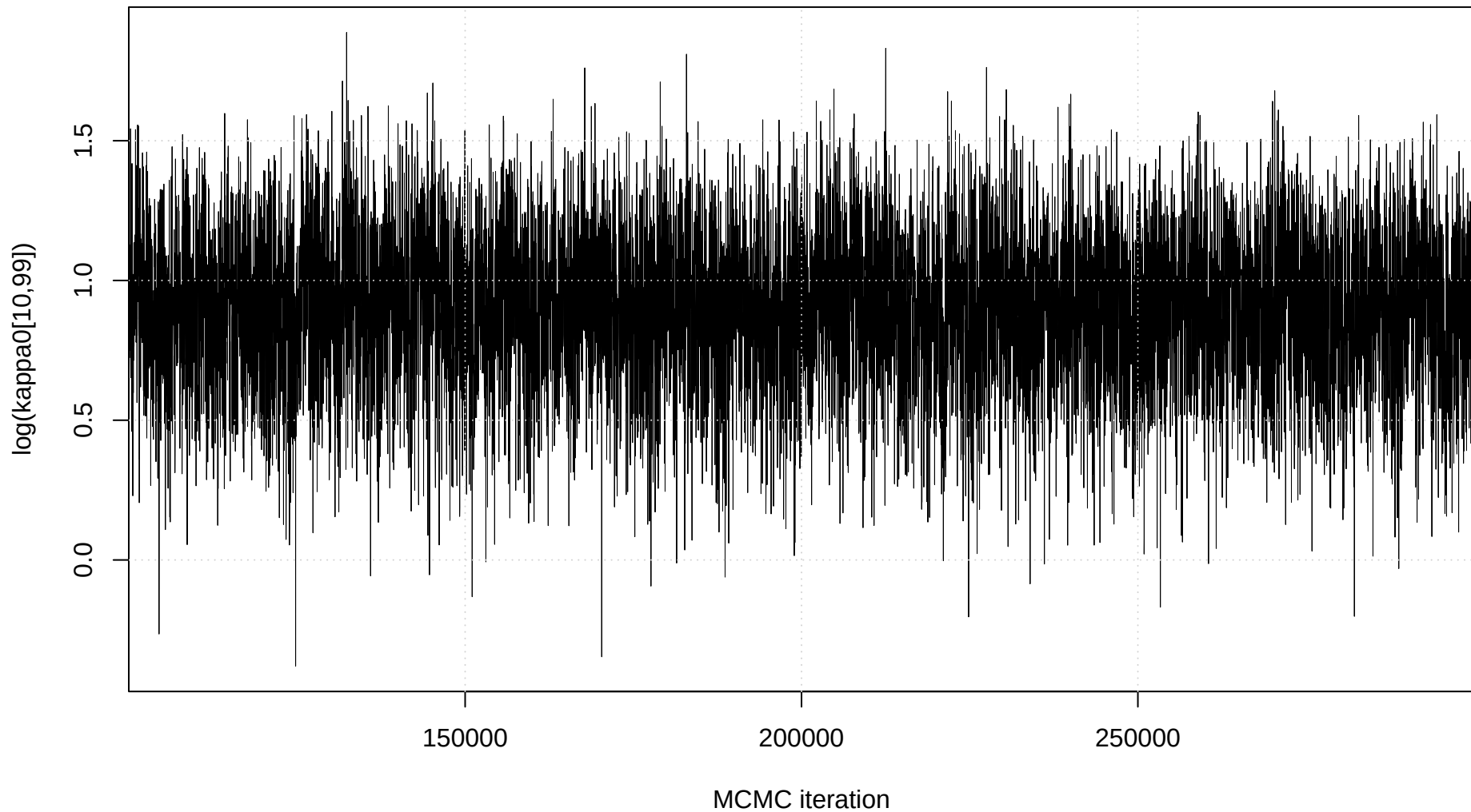
Trace plot: \log(\kappa_0[10,99])
