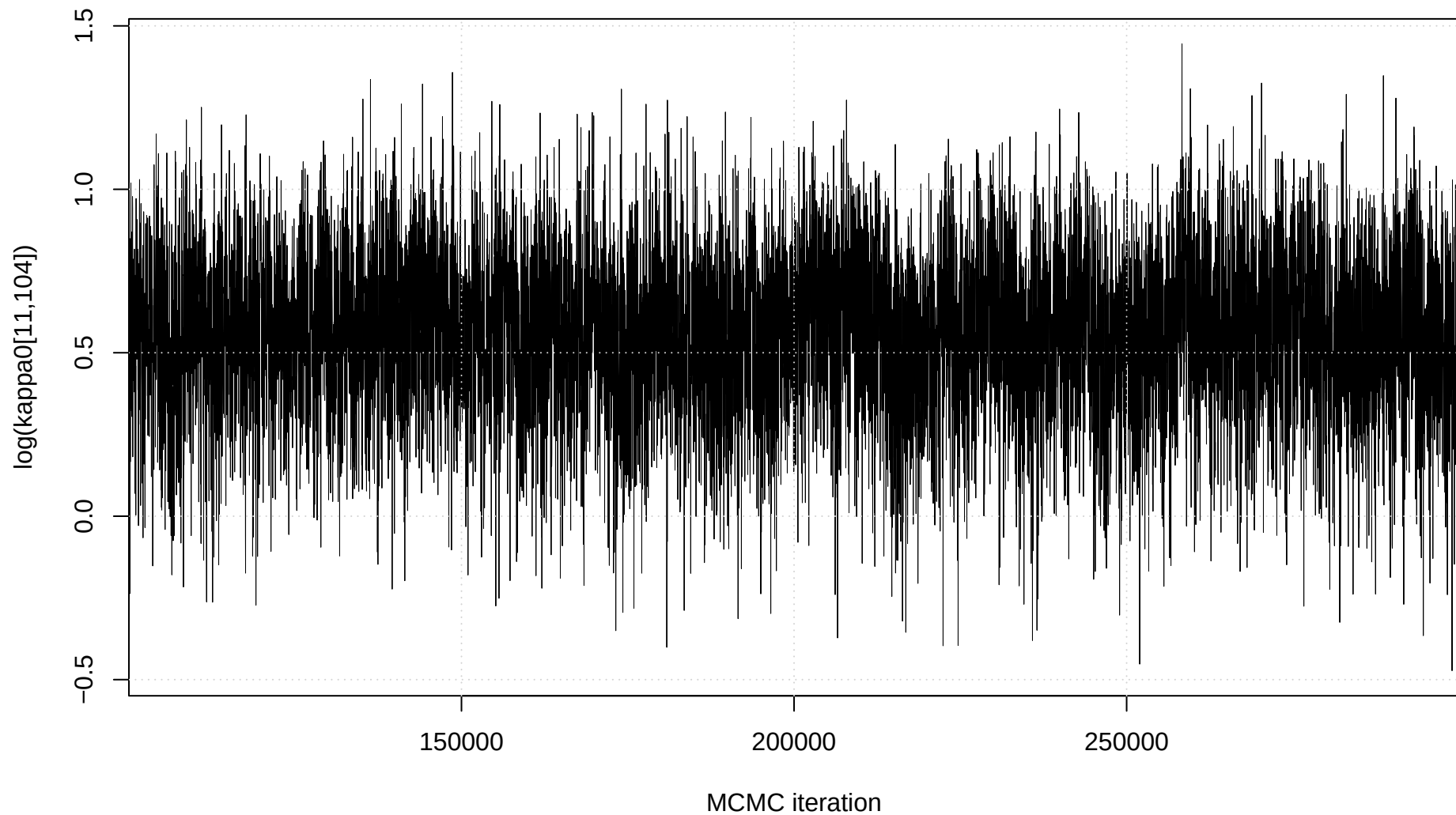
Trace plot: \log(\kappa_0[11,104])
