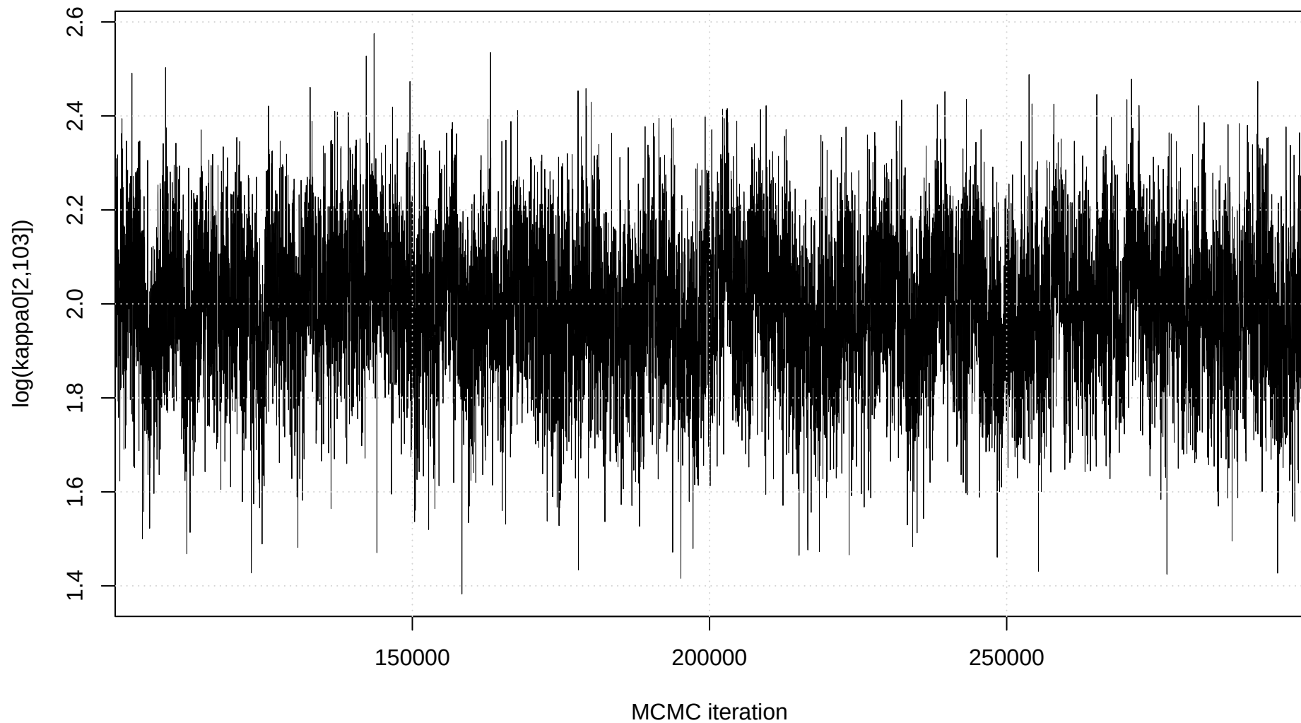
Trace plot: \log(\kappa_0[2,103])
