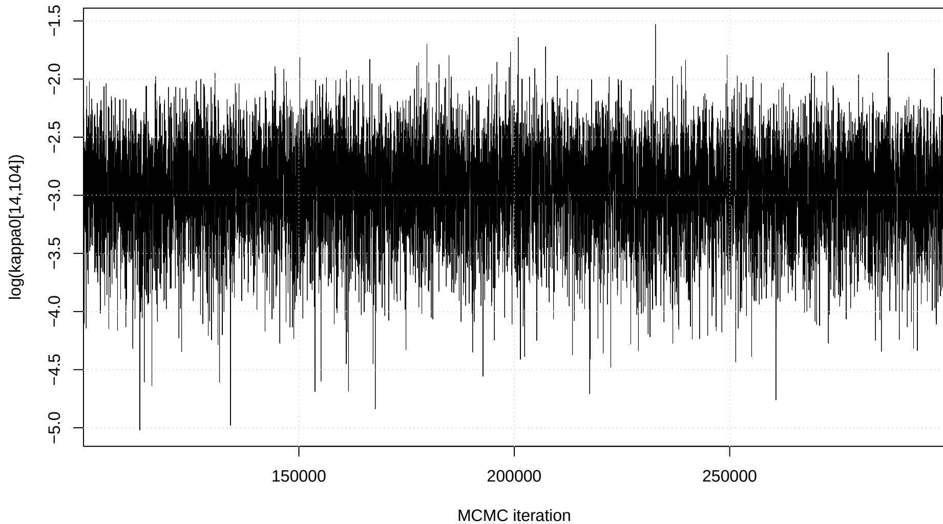
Trace plot: \log(\kappa_0[14,104])
