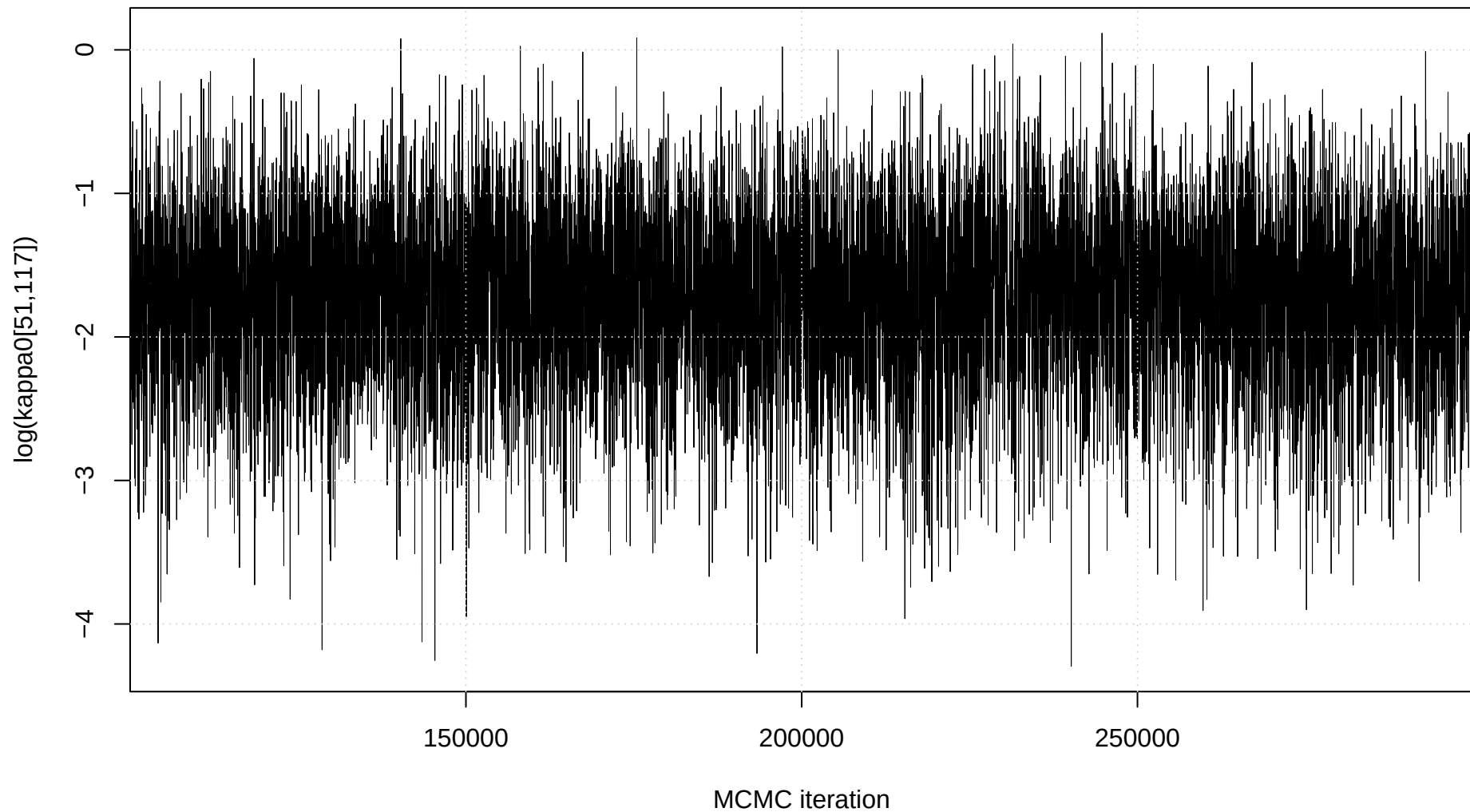
Trace plot: \log(\kappa_0[51,117])
