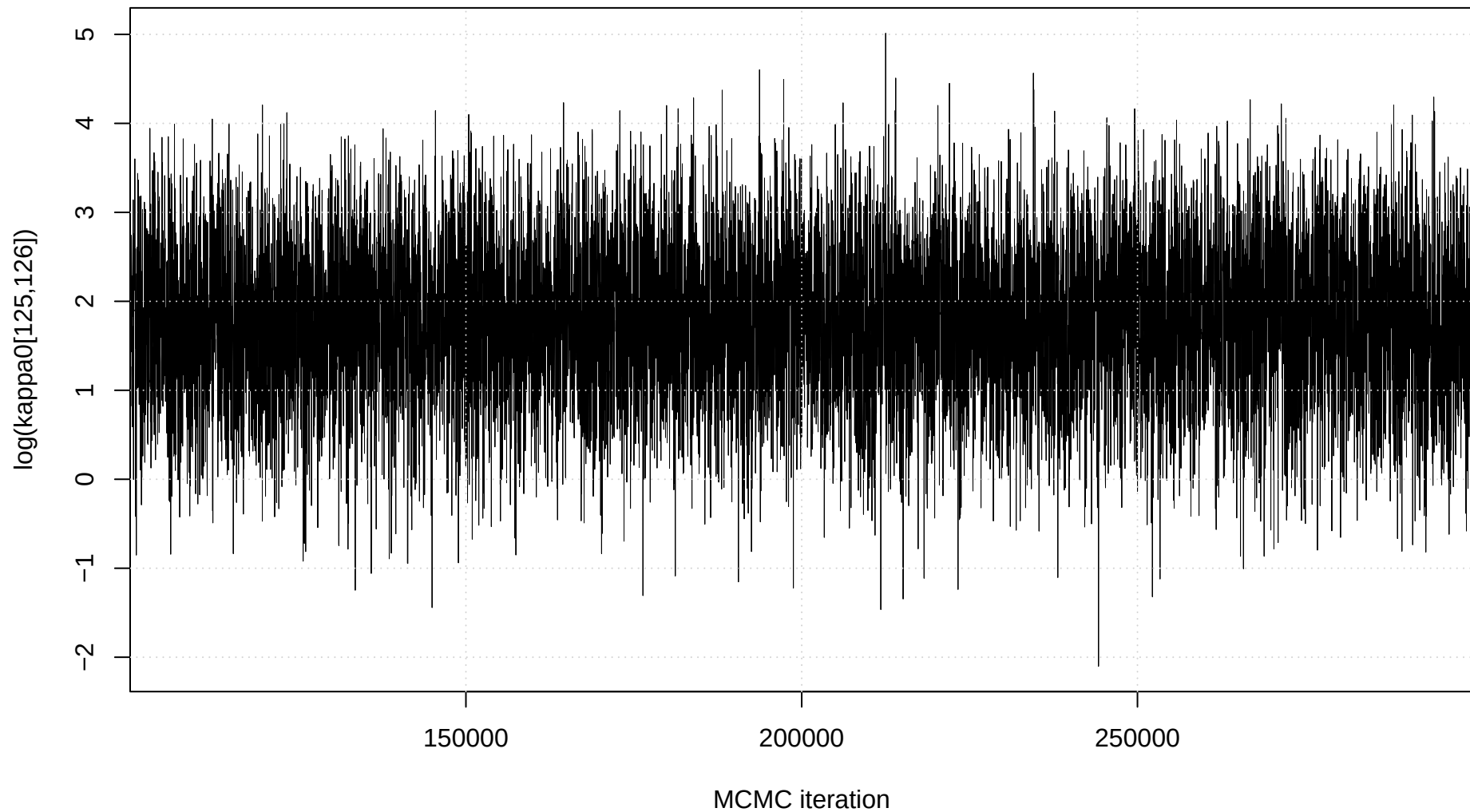
Trace plot: \log(\text{kappa0}[125,126])
