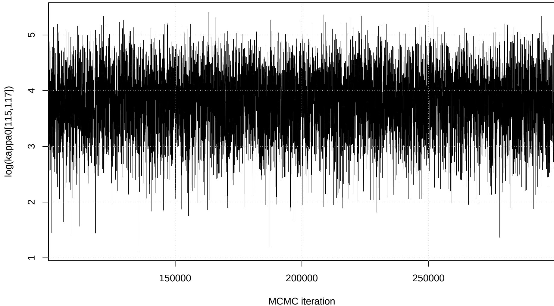
Trace plot: \log(\kappa_0[115,117])
