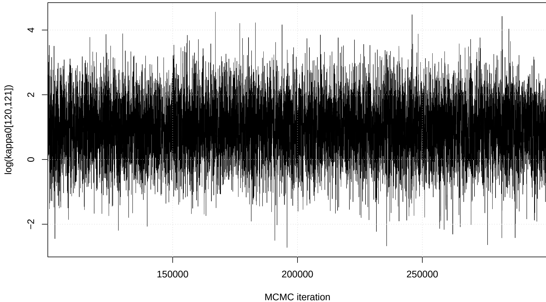
Trace plot: \log(\kappa_0[120,121])
