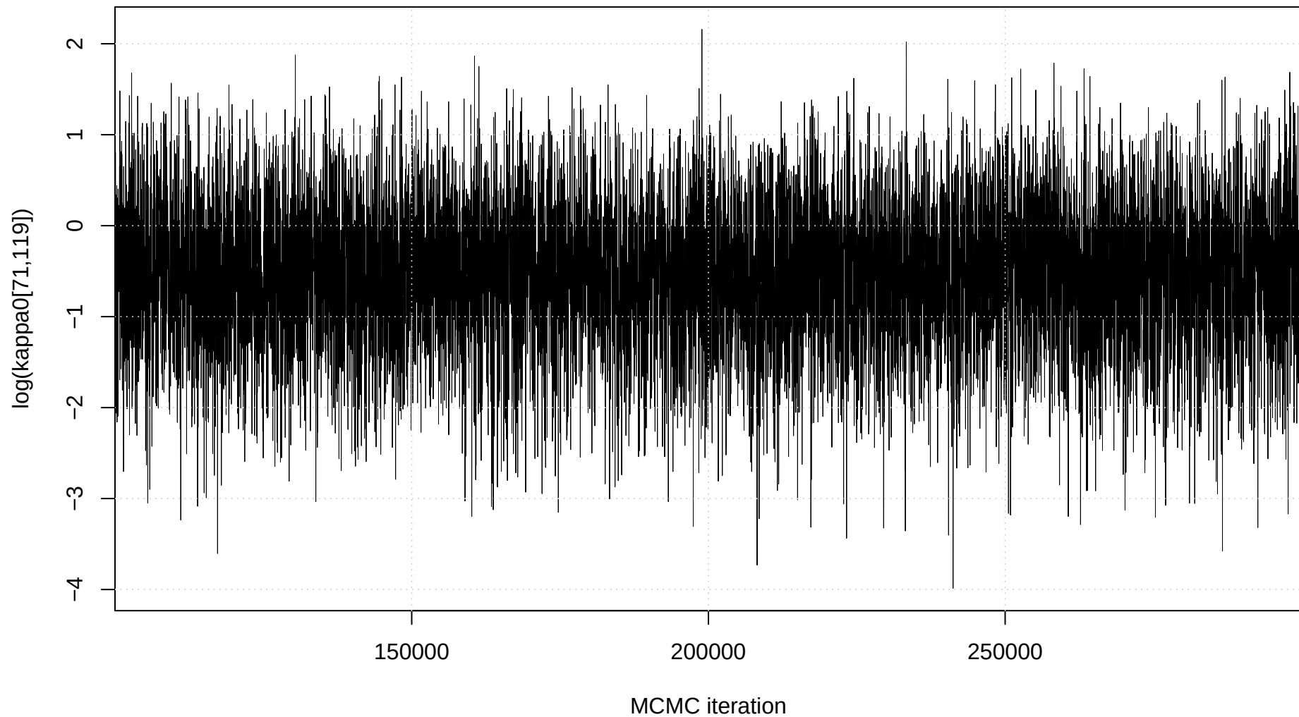
Trace plot: \log(\kappa_0[71,119])
