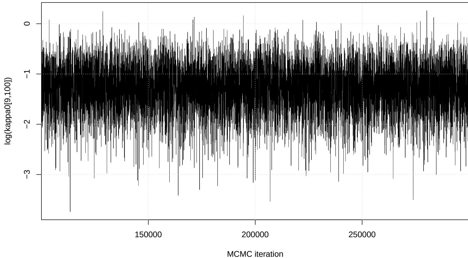
Trace plot: \log(\kappa_0[9,100])
