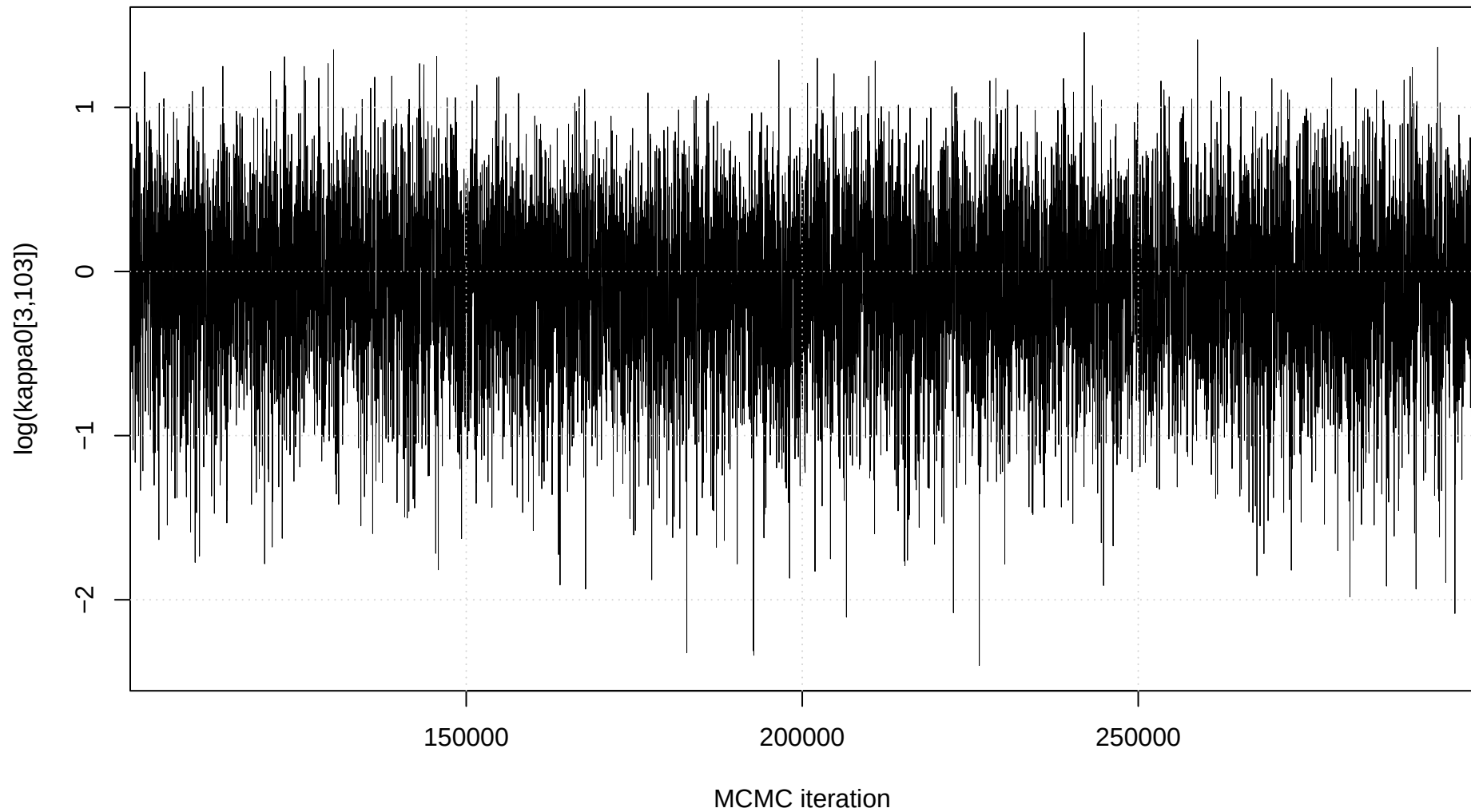
Trace plot: \log(\kappa_0[3,103])
