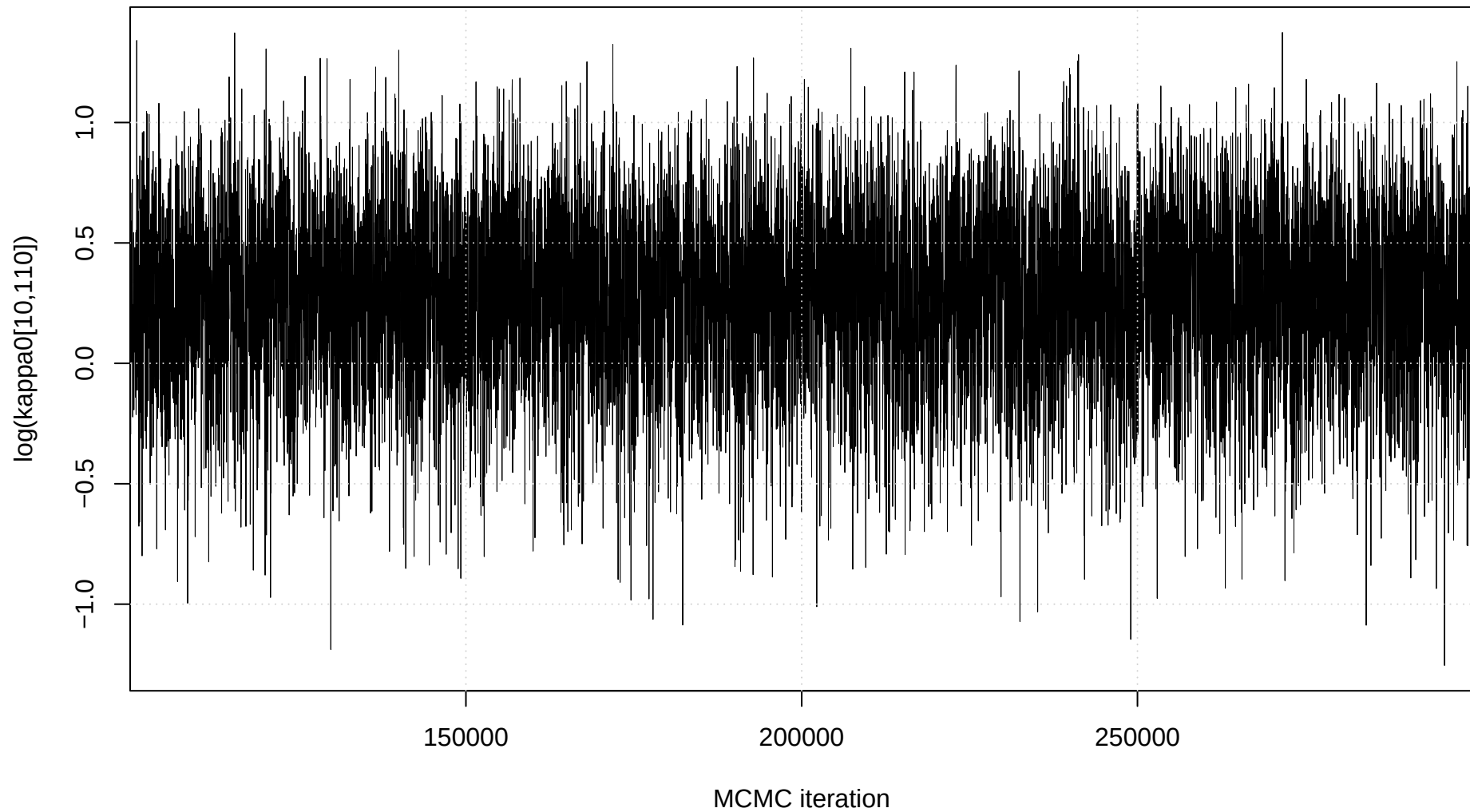
Trace plot: \log(\kappa_0[10,110])
