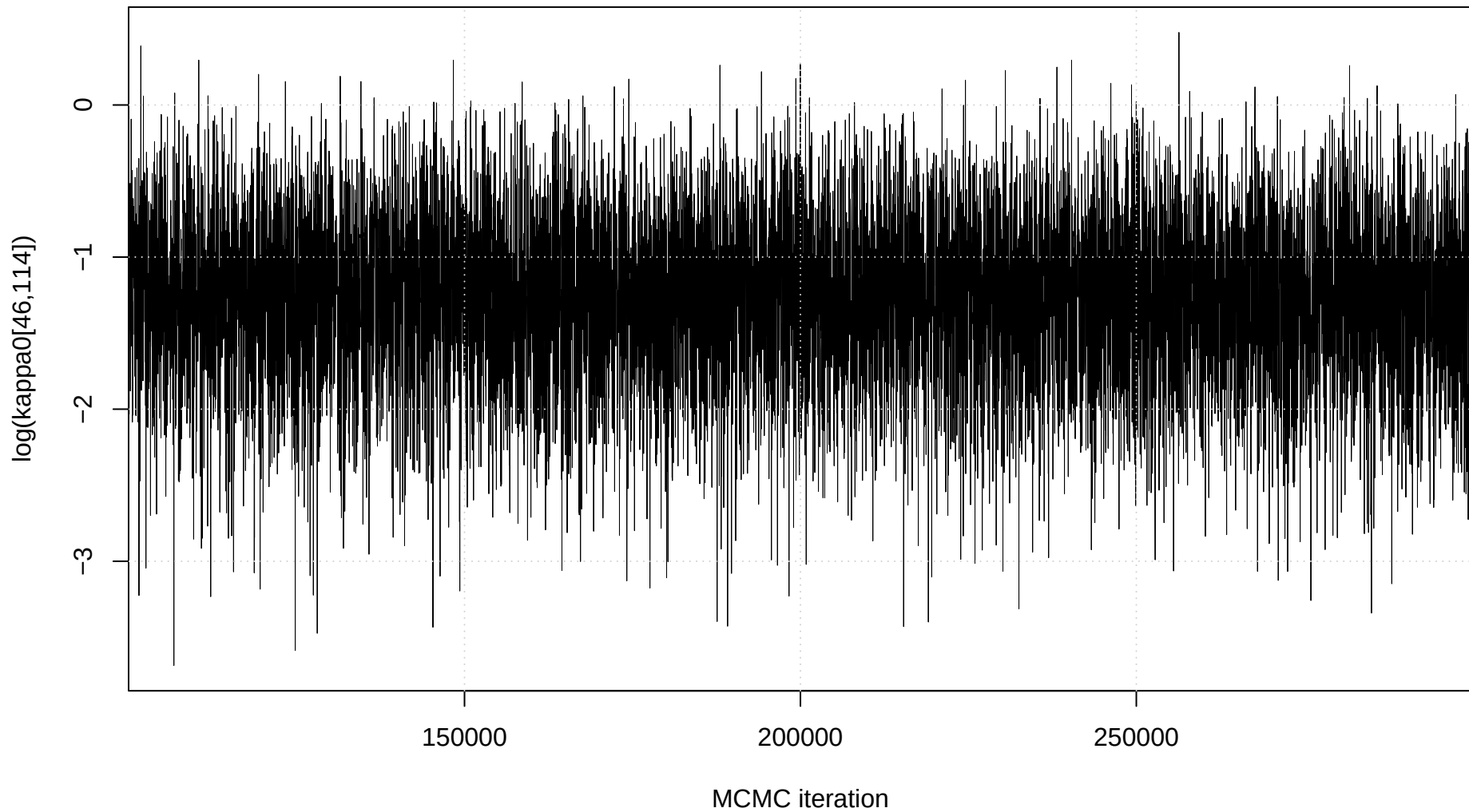
Trace plot: \log(\kappa_0[46,114])
