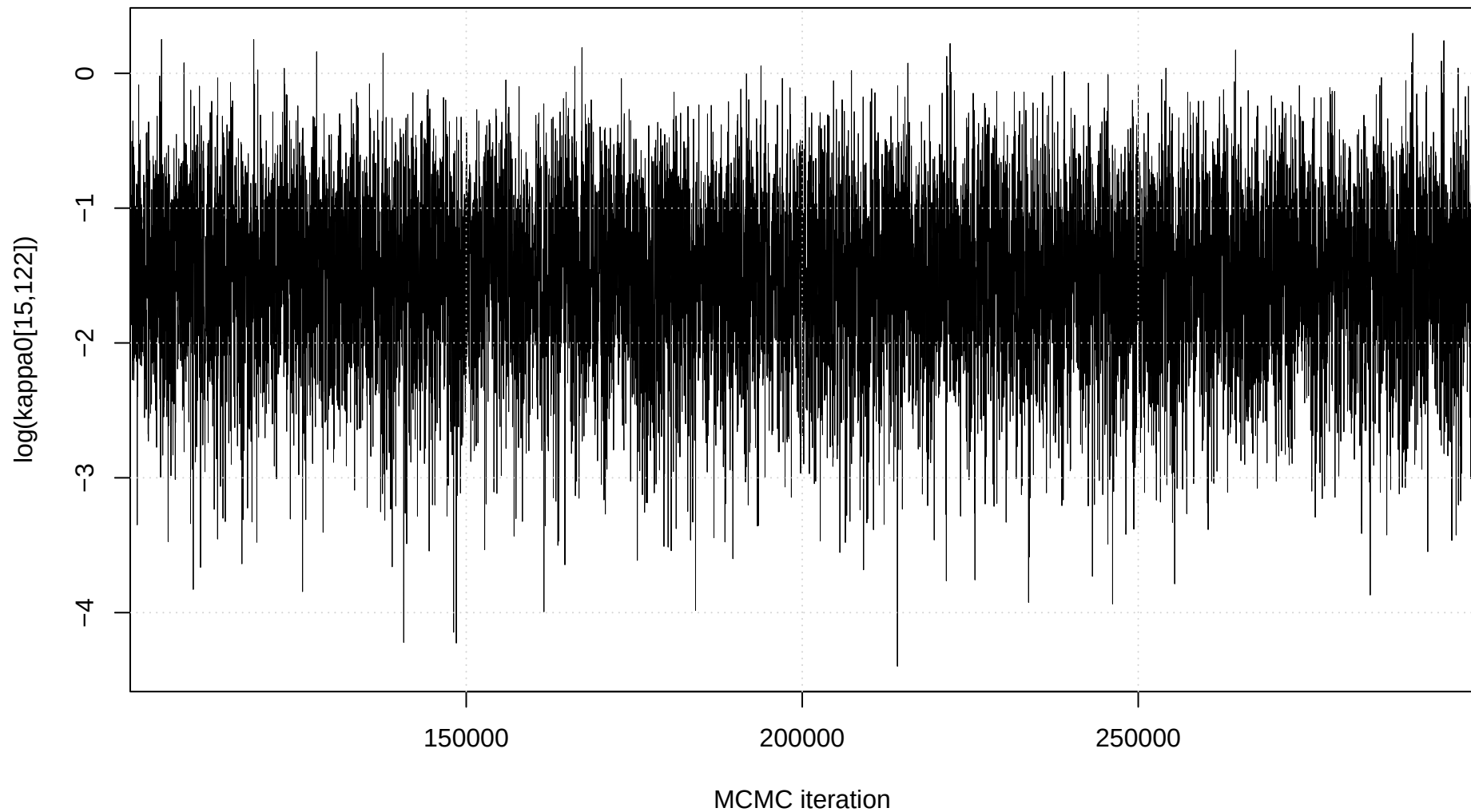
Trace plot: \log(\kappa_0[15,122])
