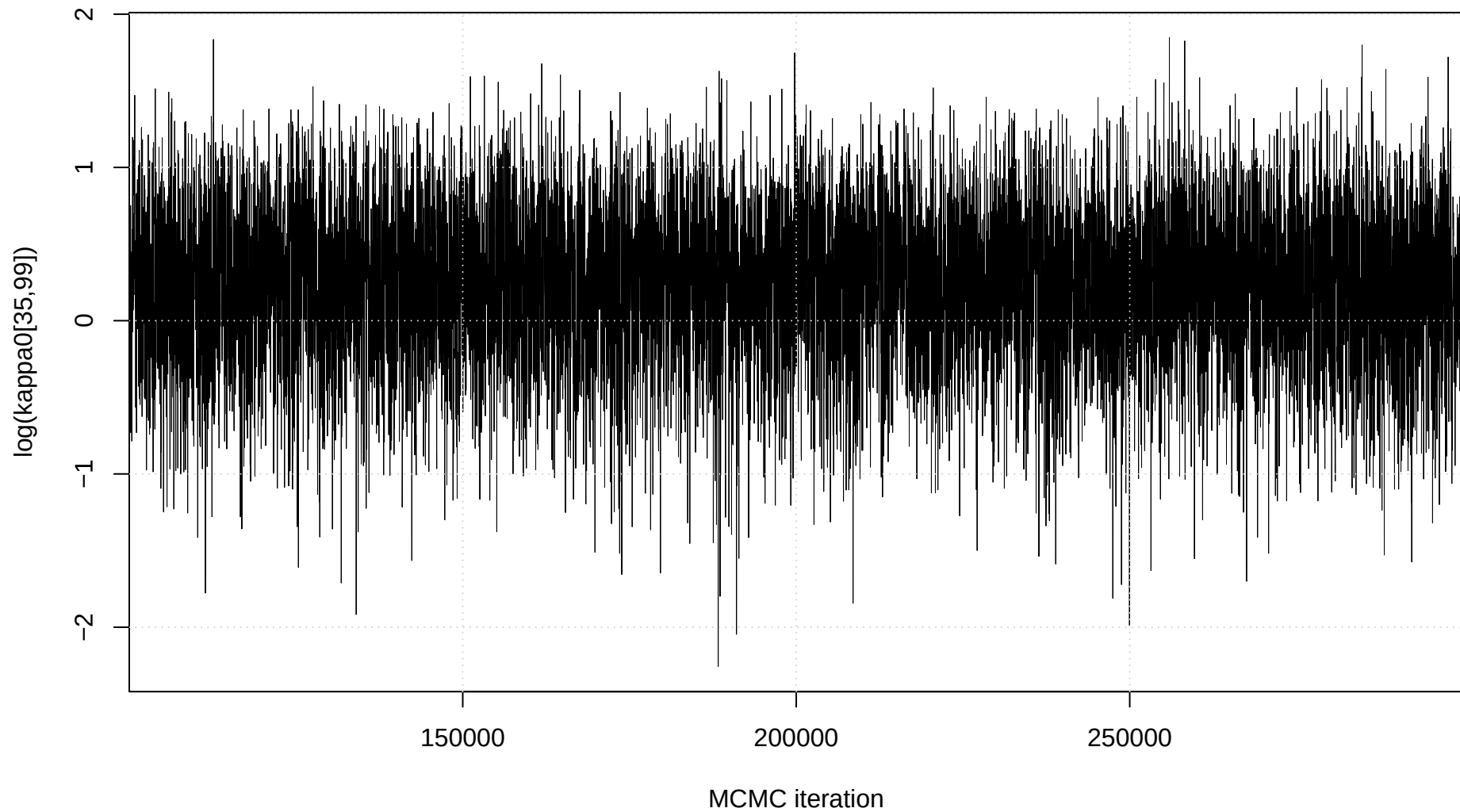
Trace plot: \log(\kappa_0[35,99])
