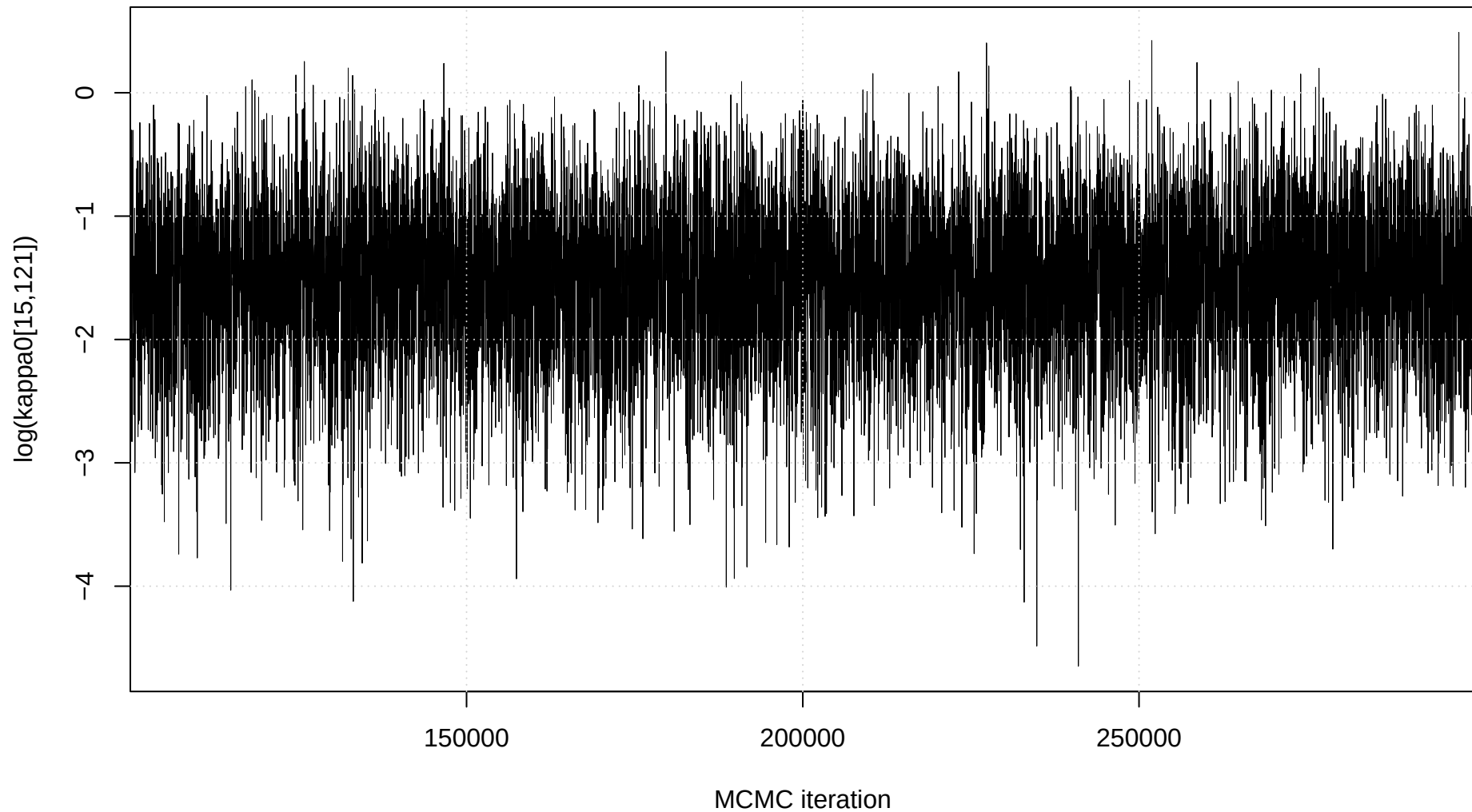
Trace plot: \log(\text{kappa0}[15,121])
