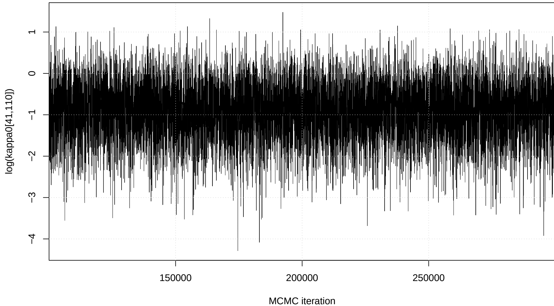
Trace plot: \log(\kappa_0[41,110])
