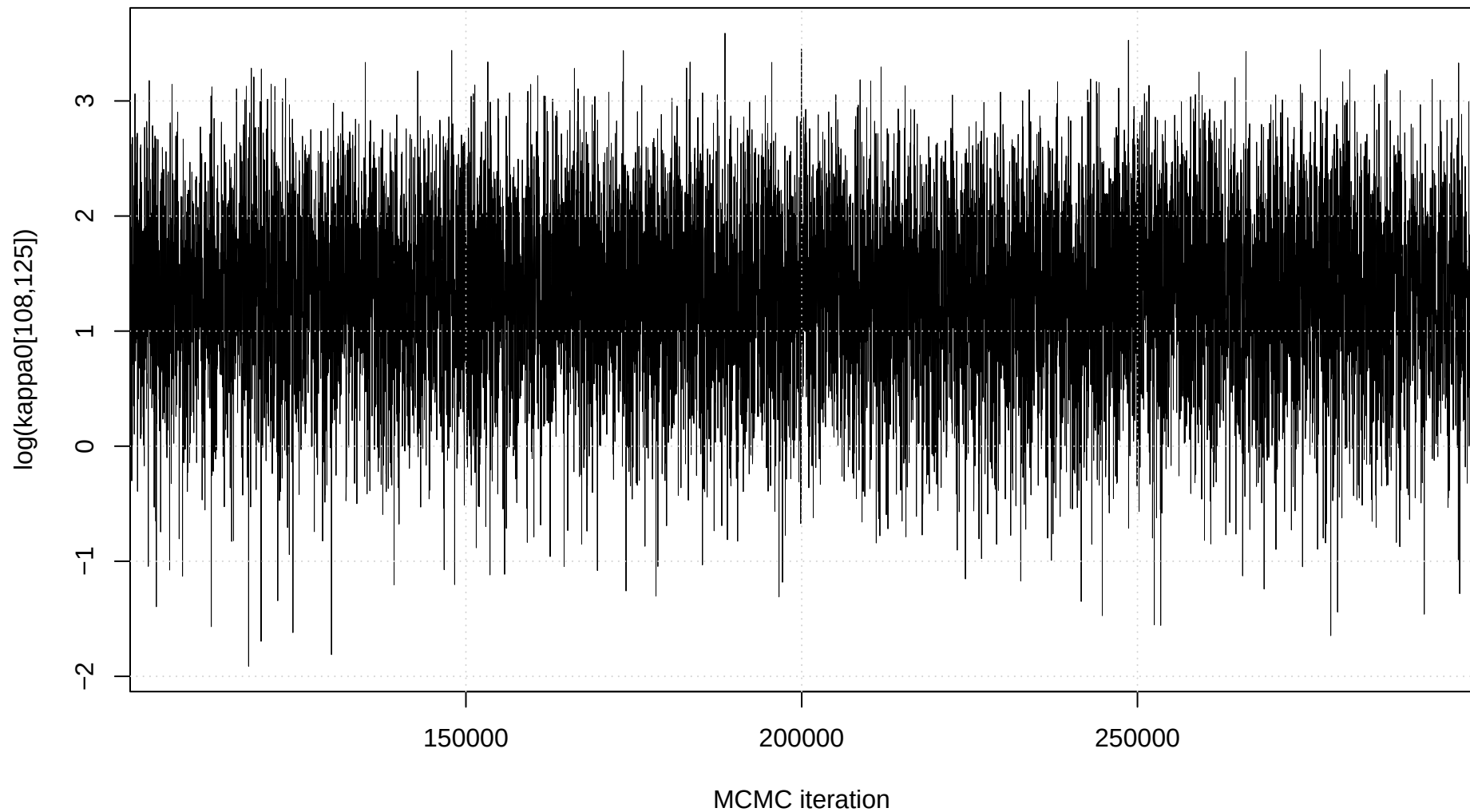
Trace plot: \log(\kappa_0[108,125])
