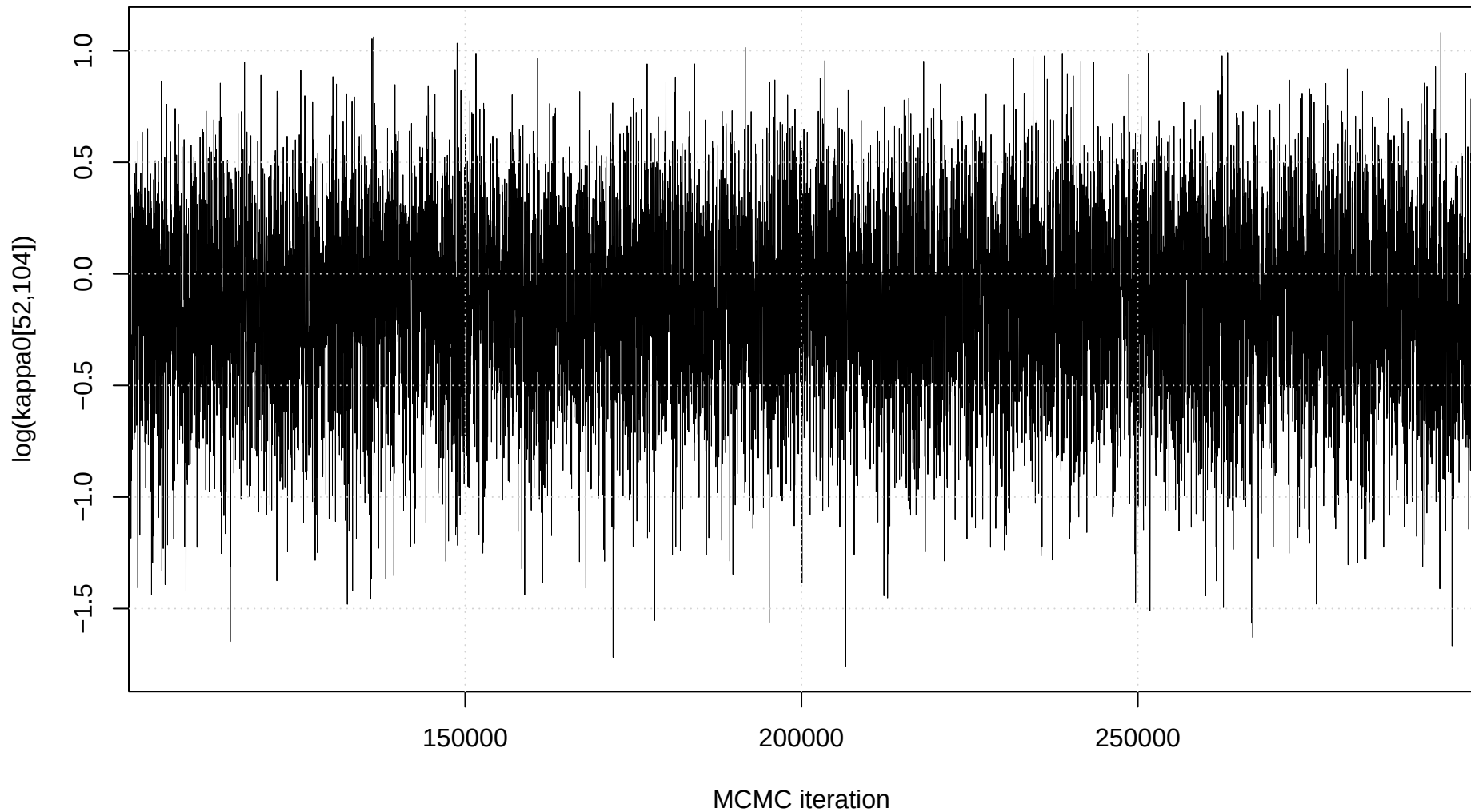
Trace plot: \log(\kappa_0[52,104])
