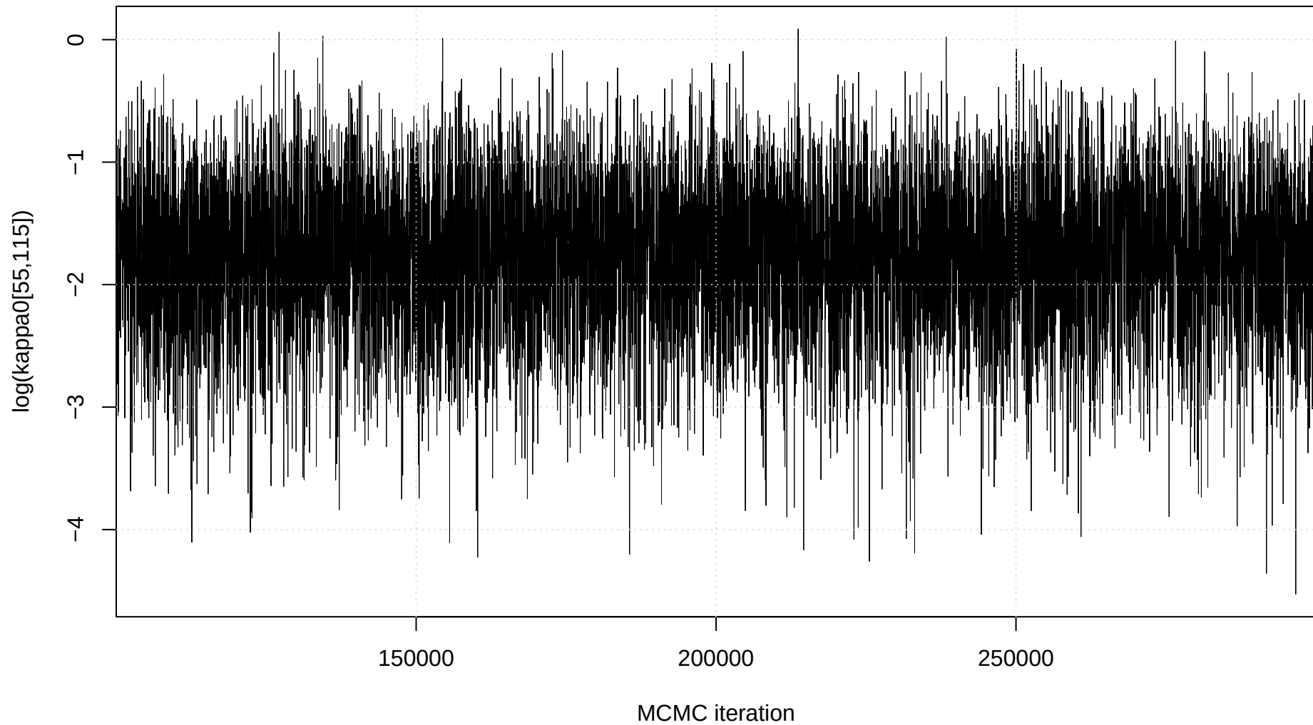
Trace plot: \log(\kappa_0[55,115])
