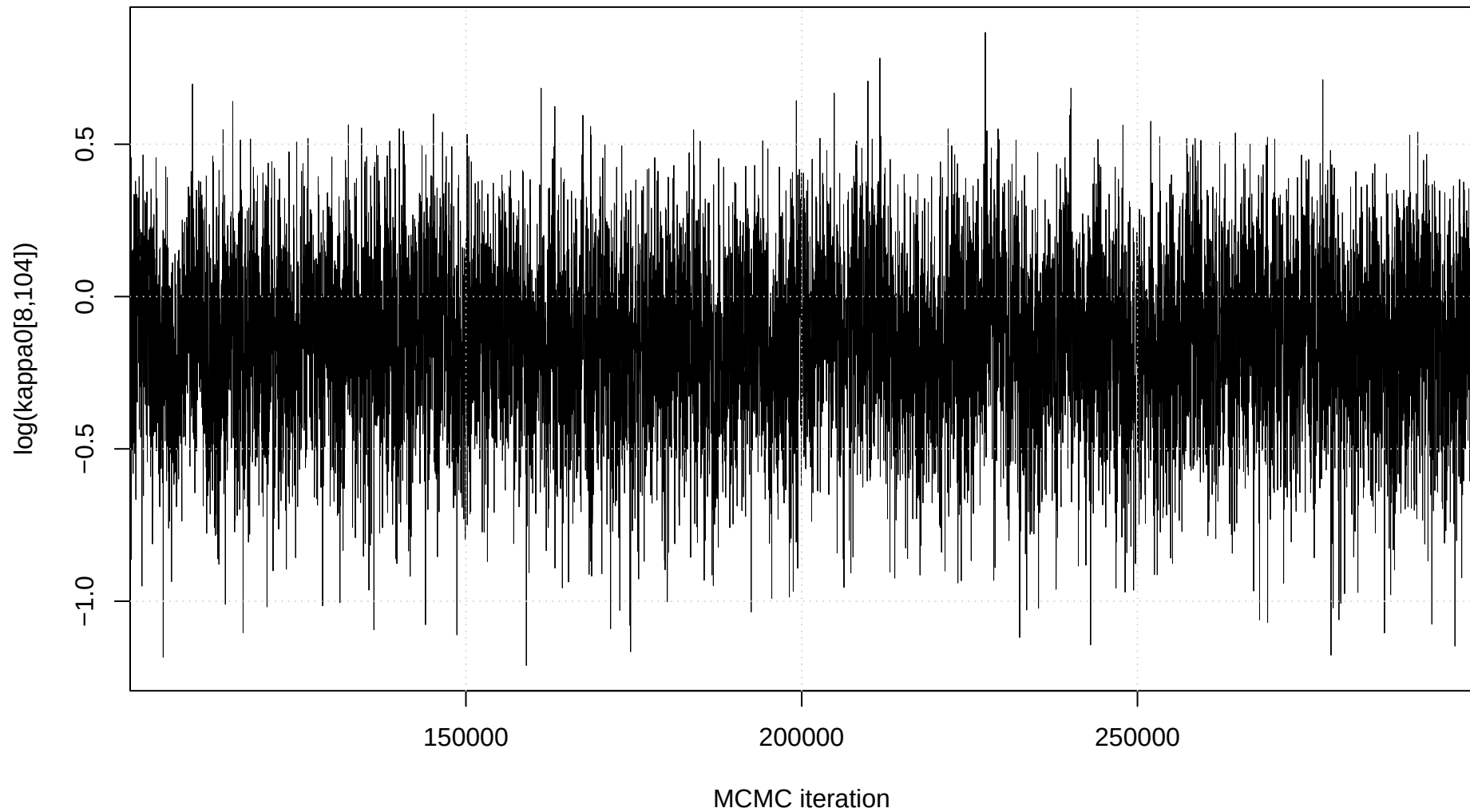
Trace plot: \log(\kappa_0[8,104])
