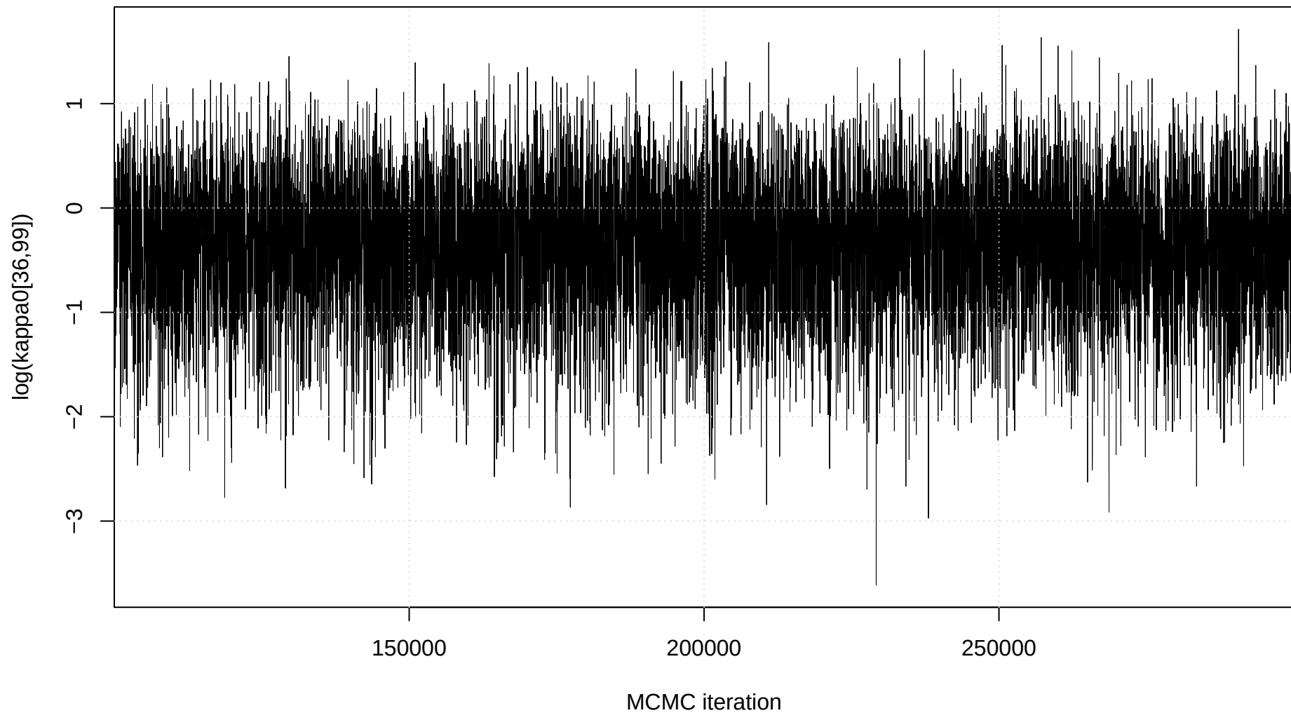
Trace plot: \log(\kappa_0[36,99])
