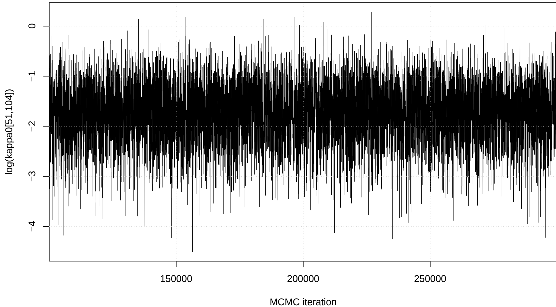
Trace plot: \log(\text{kappa0}[51,104])
