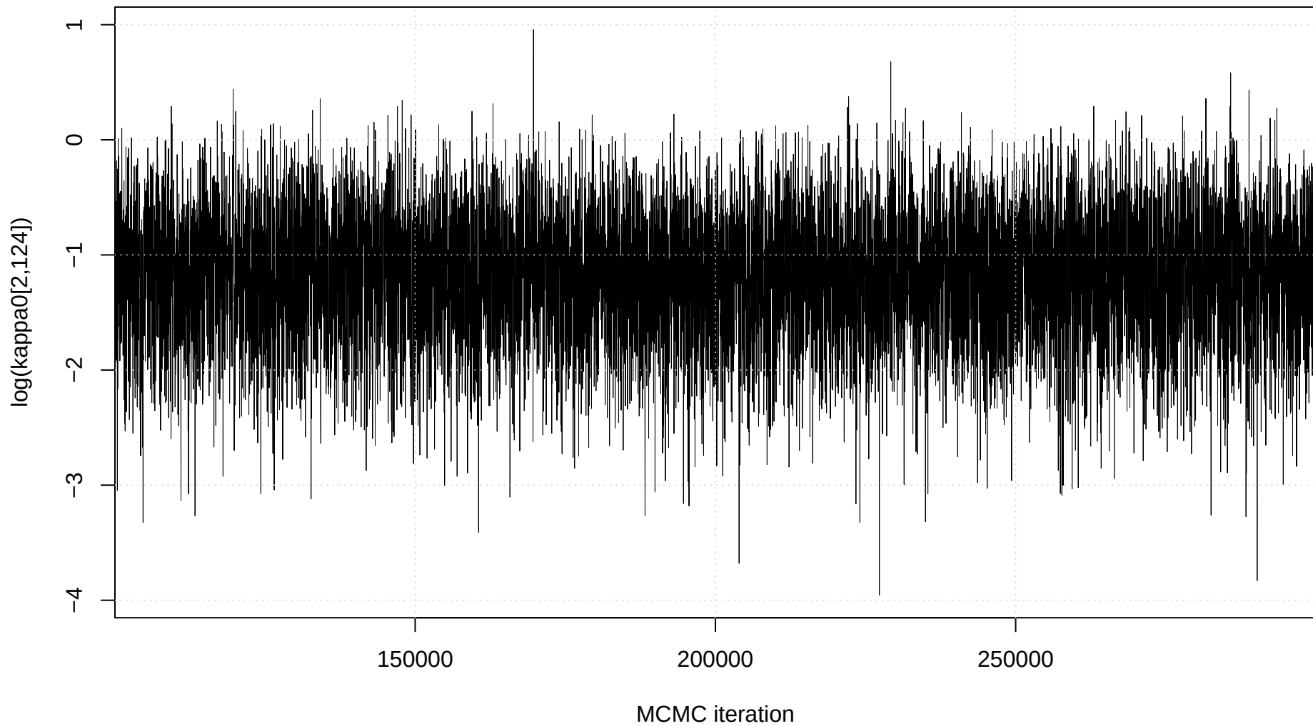
Trace plot: \log(\kappa_0[2,124])
