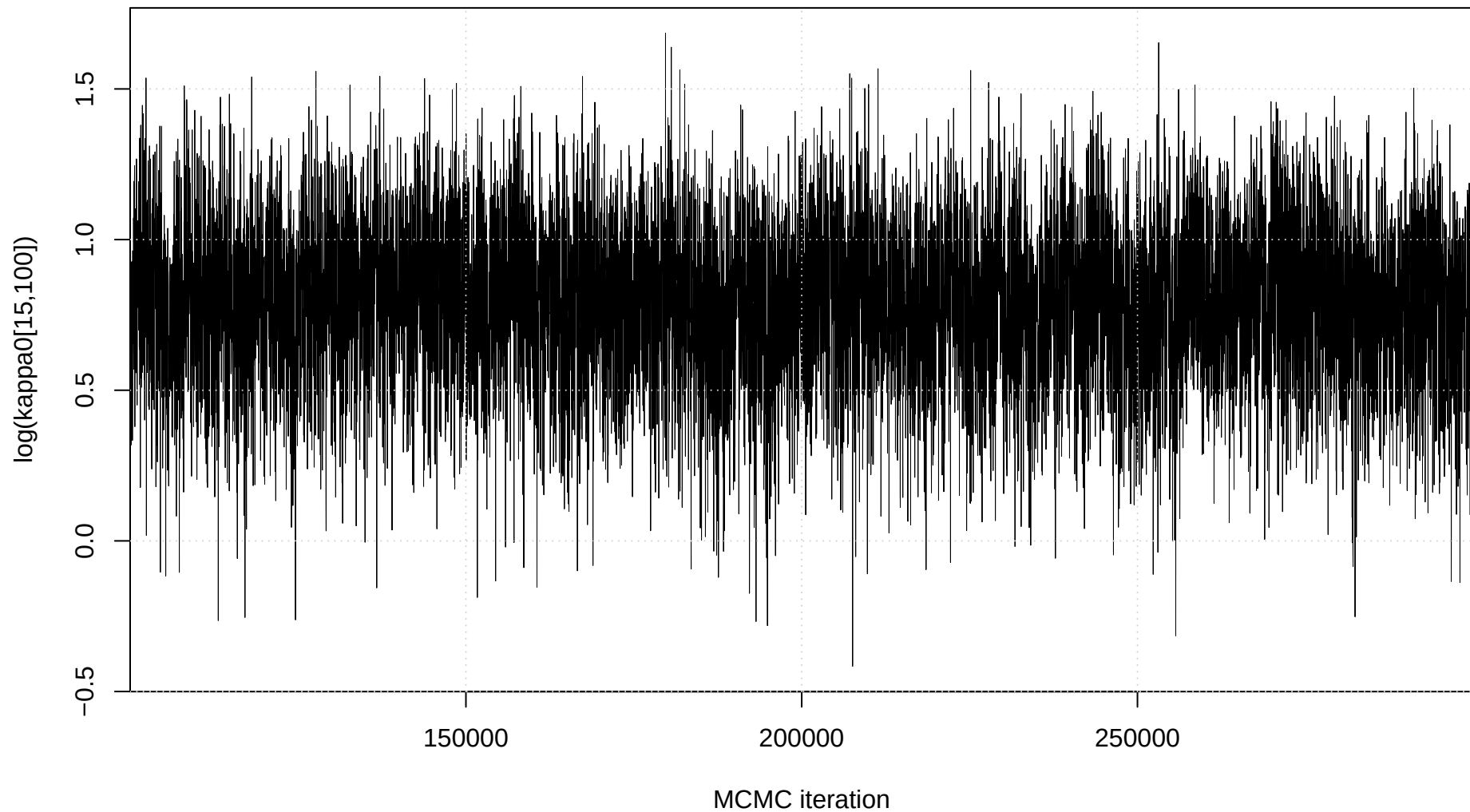
Trace plot: \log(\kappa_0[15,100])
