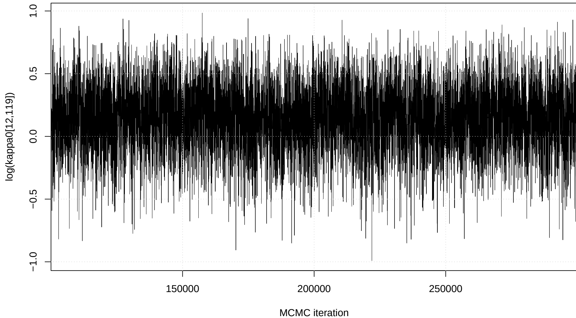
Trace plot: \log(\kappa_0[12,119])
