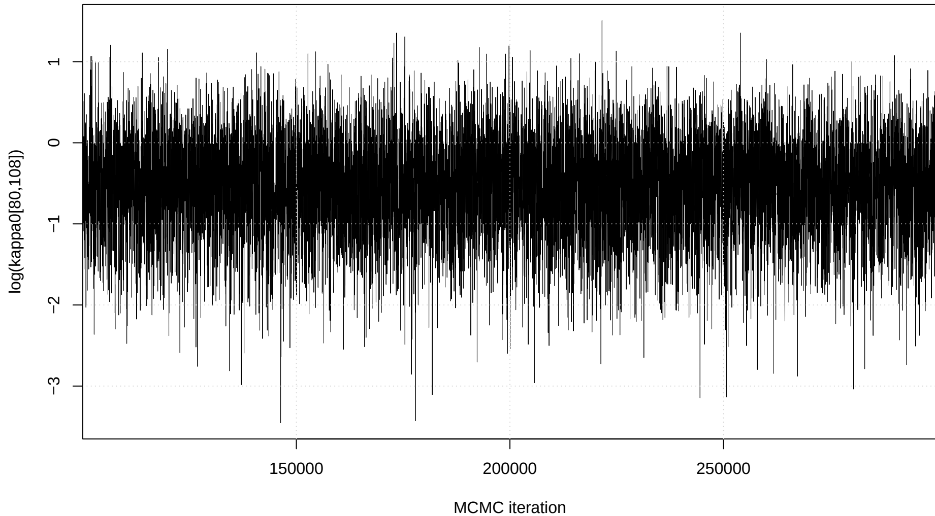
Trace plot: \log(\kappa_0[80,108])
