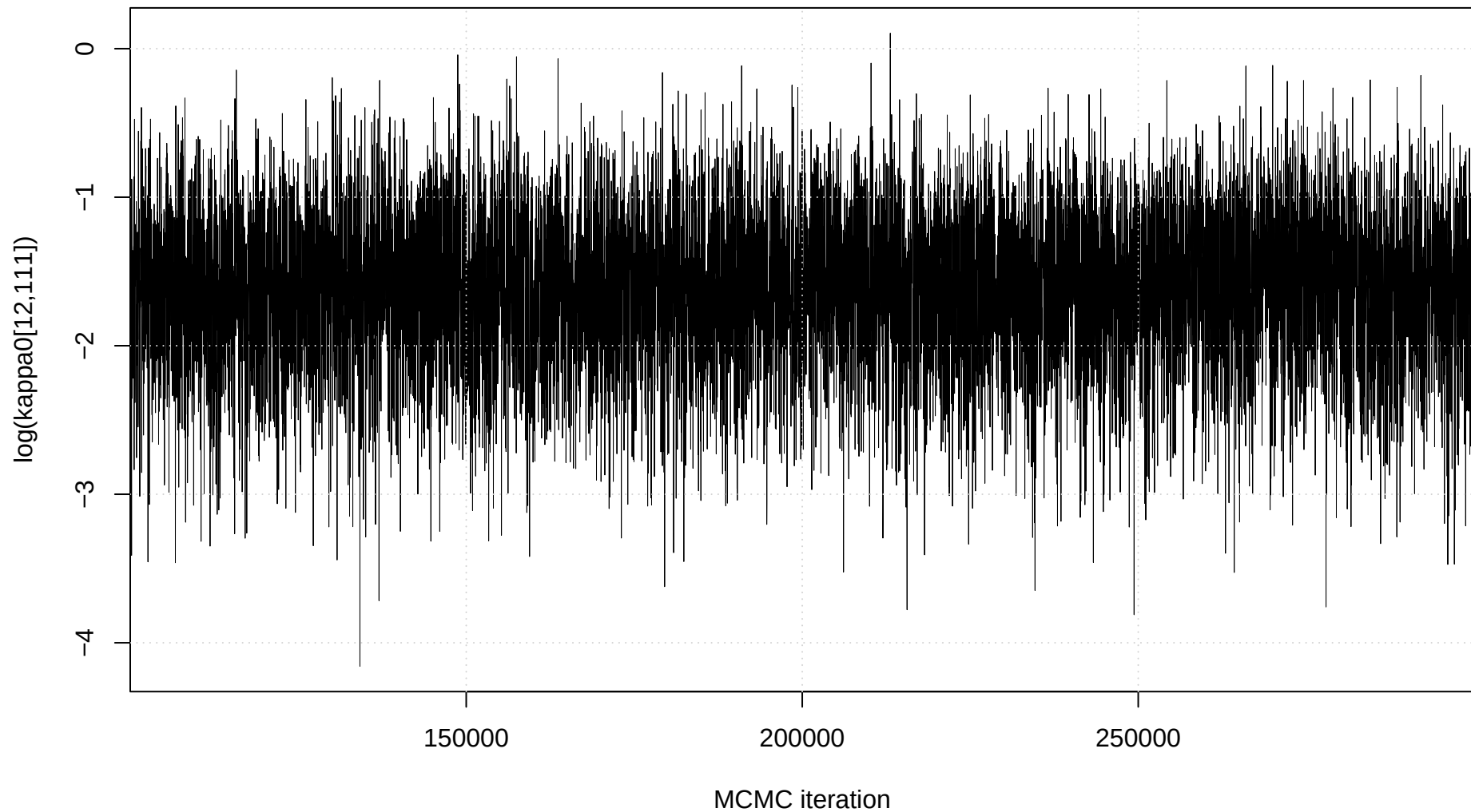
Trace plot: \log(\kappa_0[12,111])
