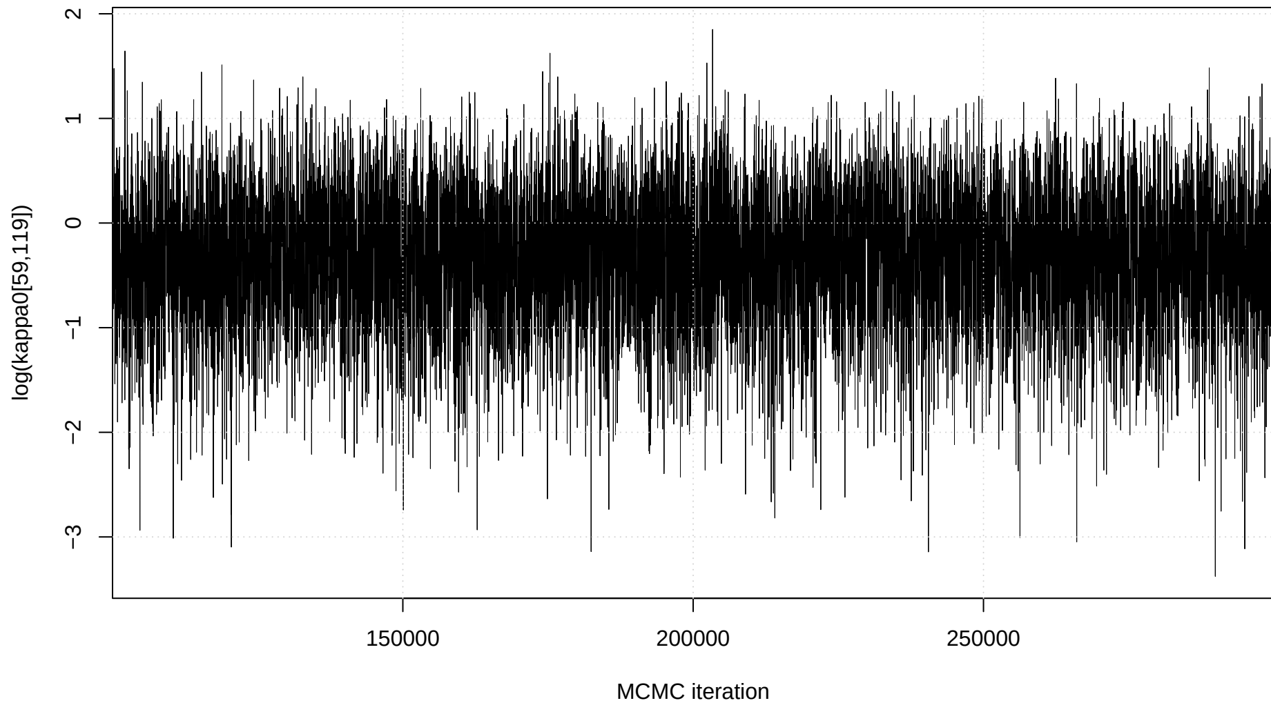
Trace plot: \log(\kappa_0[59,119])
