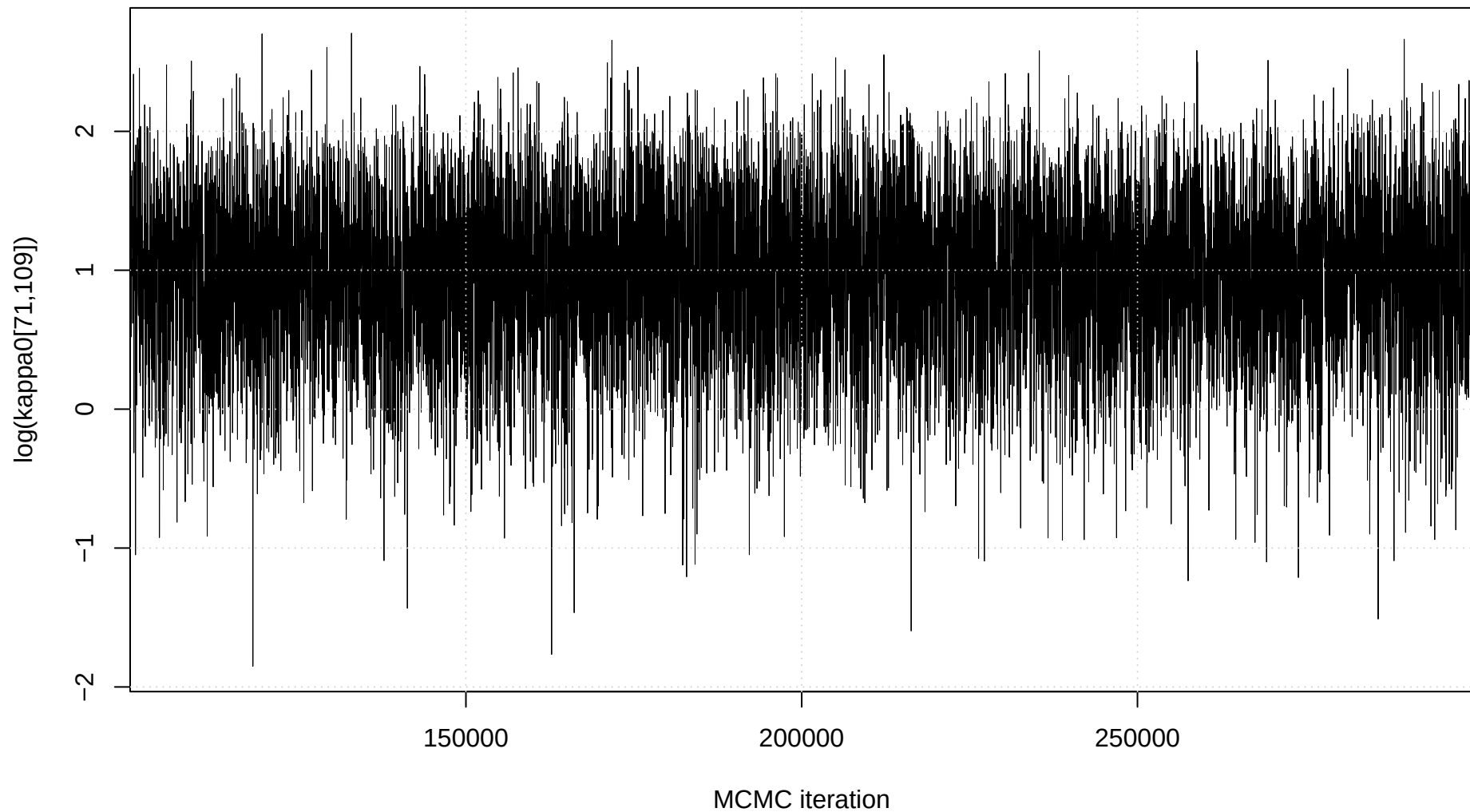
Trace plot: \log(\kappa_0[71,109])
