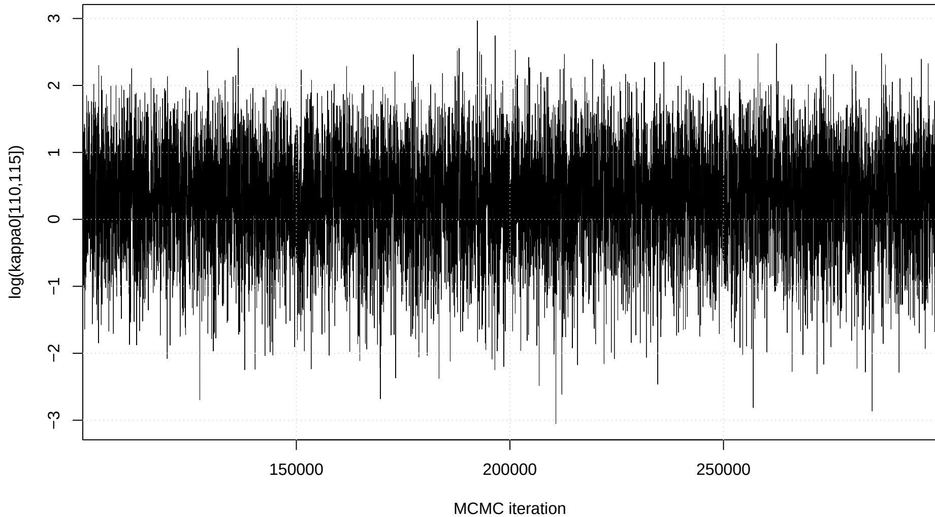
Trace plot: \log(\kappa_0[110,115])
