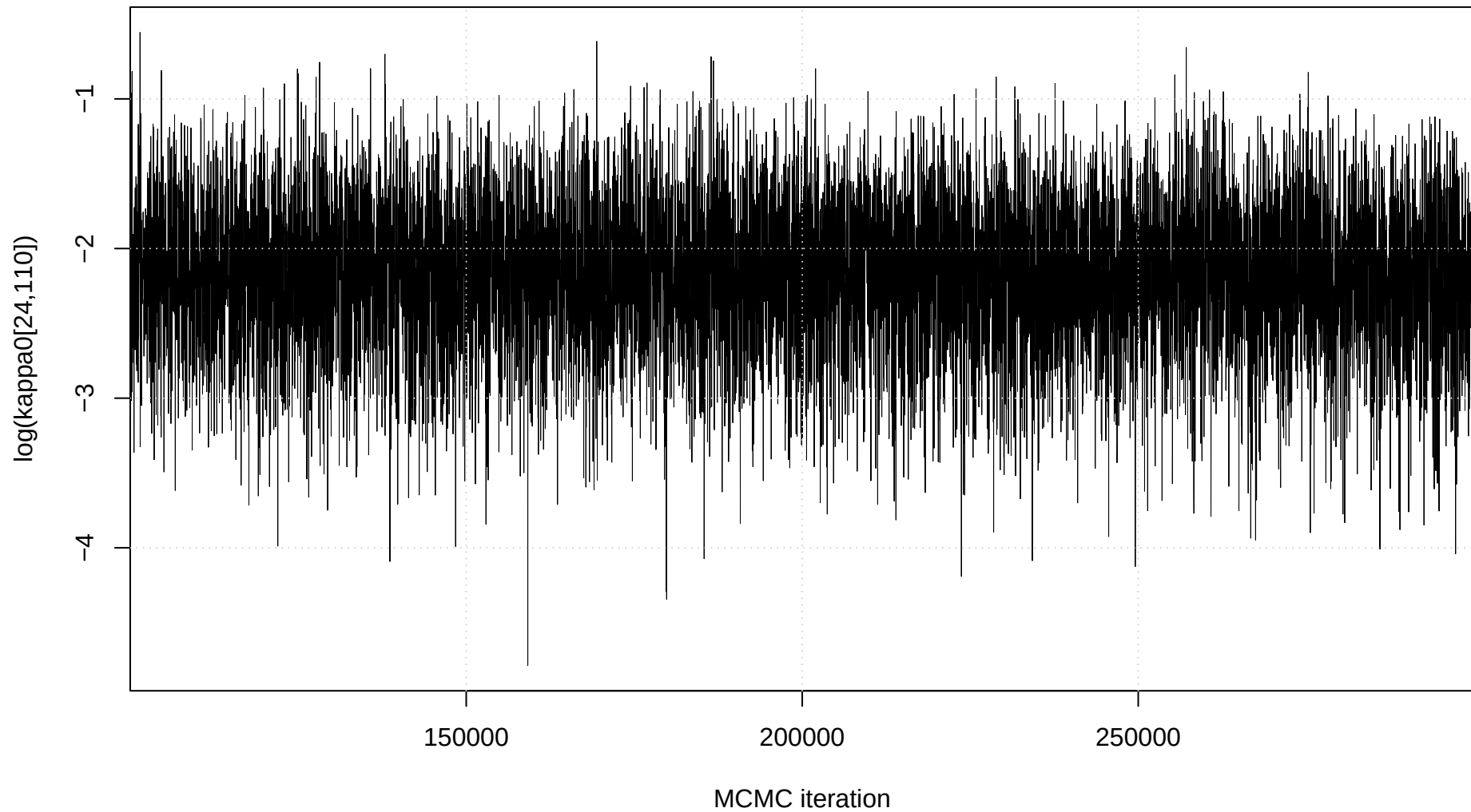
Trace plot: \log(\kappa_0[24,110])
