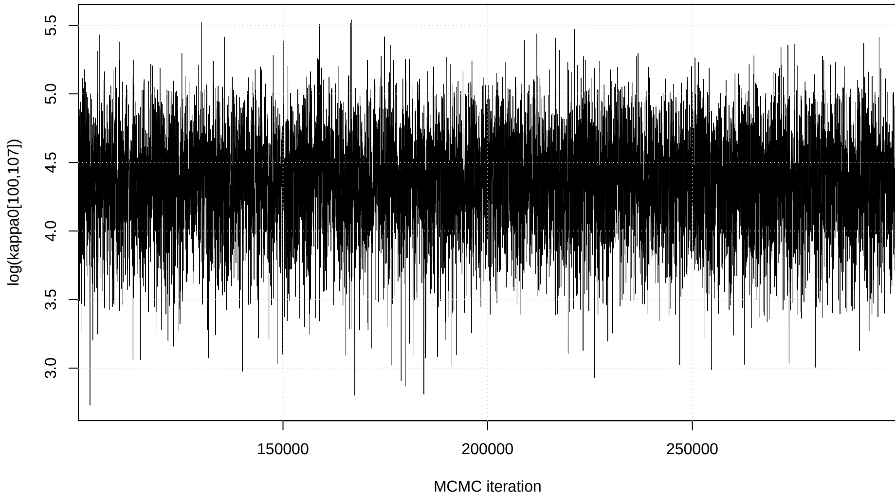
Trace plot: \log(\text{kappa0}[100,107])
