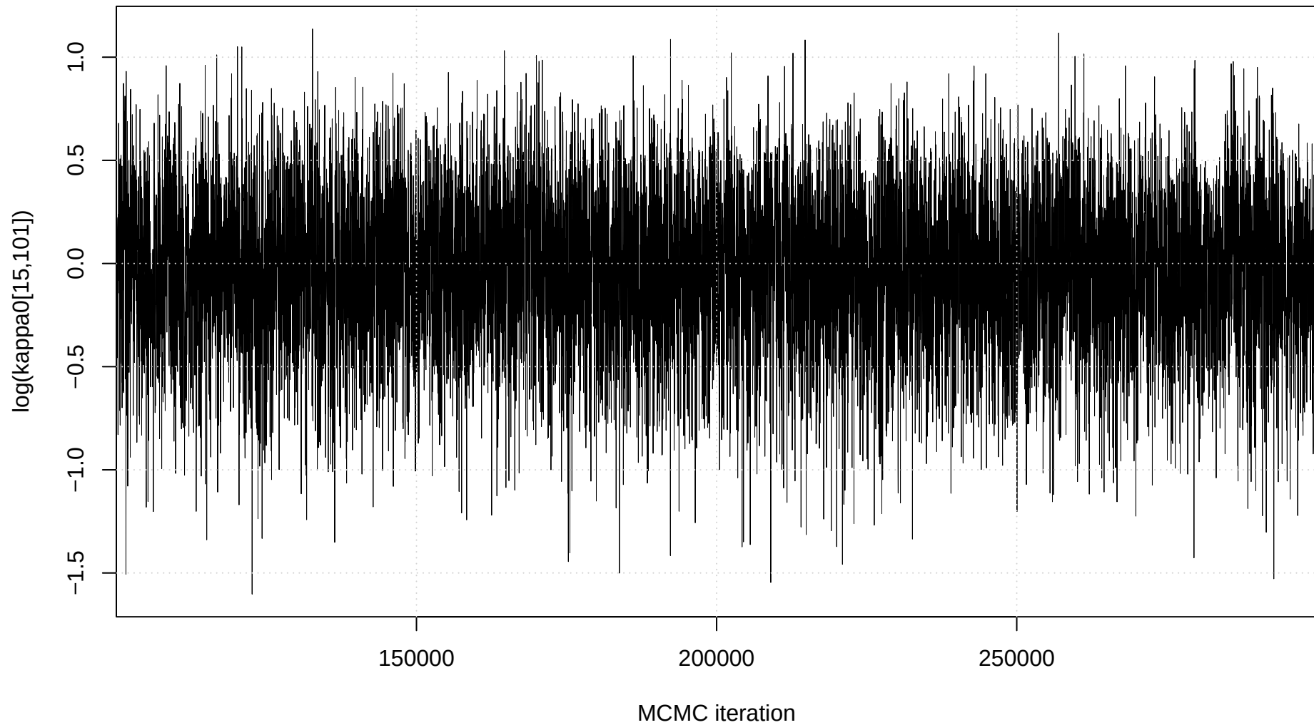
Trace plot: \log(\text{kappa0}[15,101])
