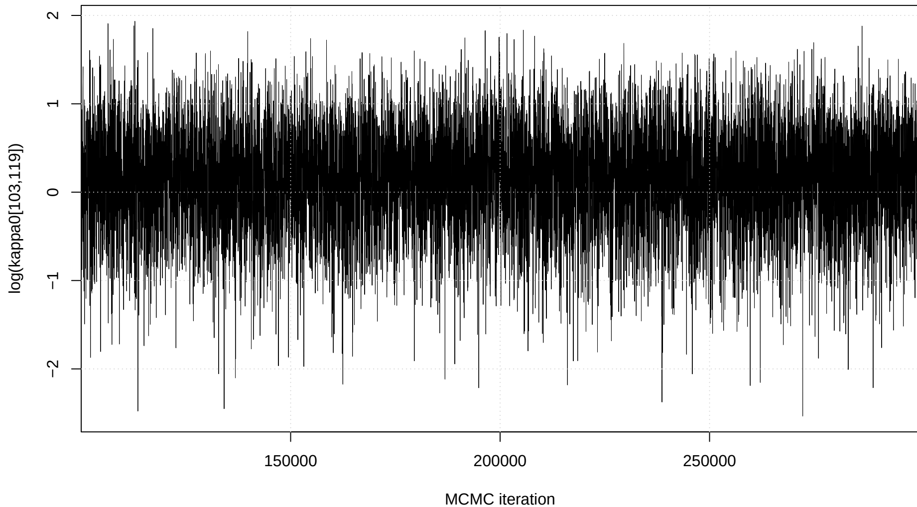
Trace plot: \log(\kappa_0[103,119])
