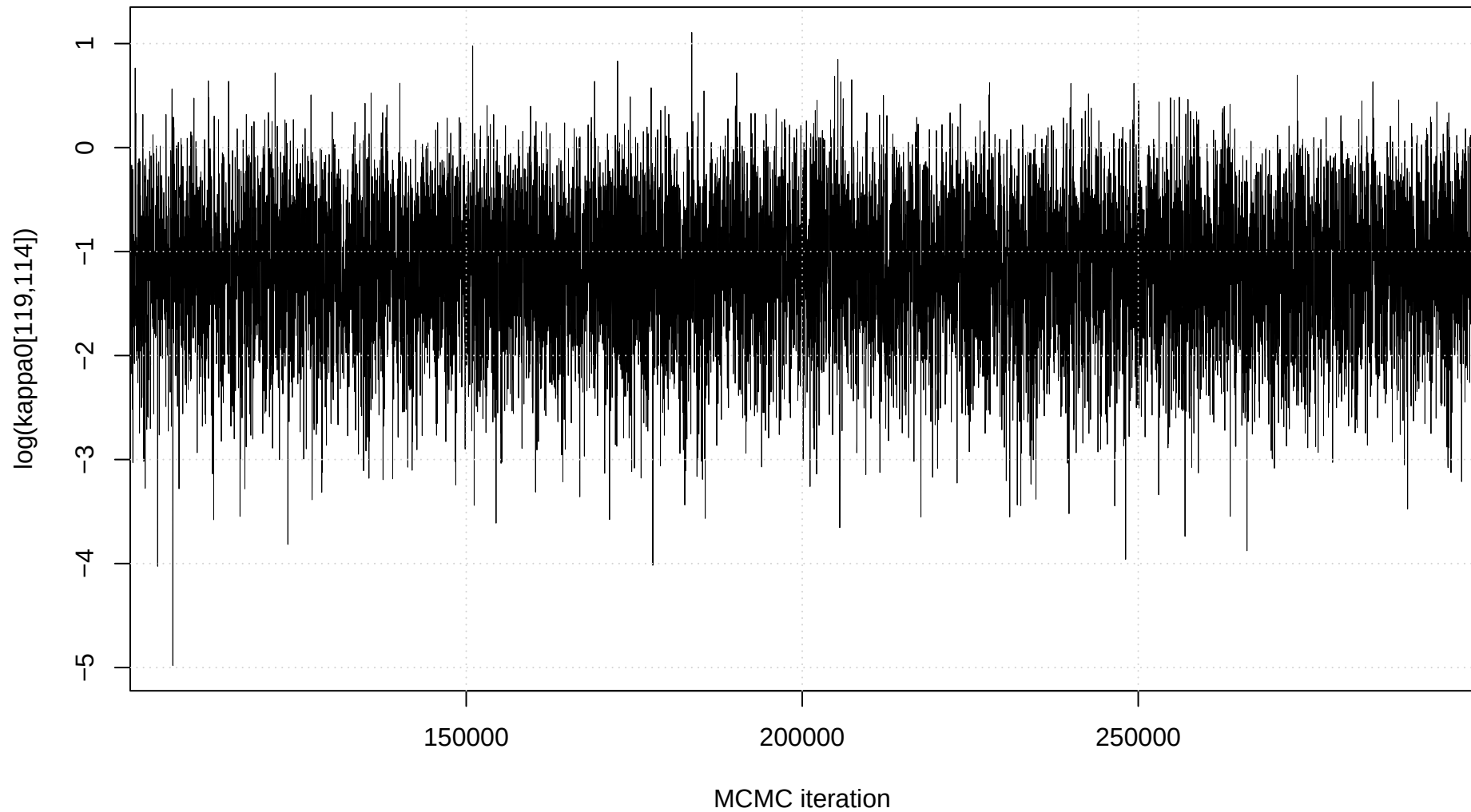
Trace plot: \log(\kappa_0[119,114])
