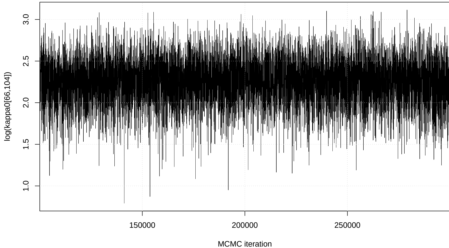
Trace plot: \log(\kappa_0[66,104])
