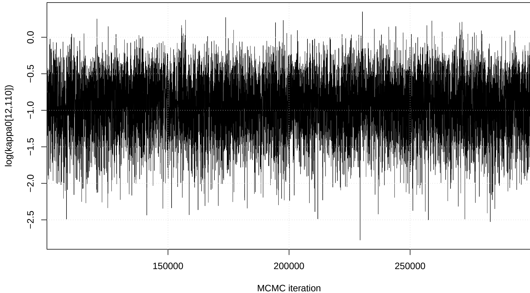
Trace plot: \log(\kappa_0[12,110])
