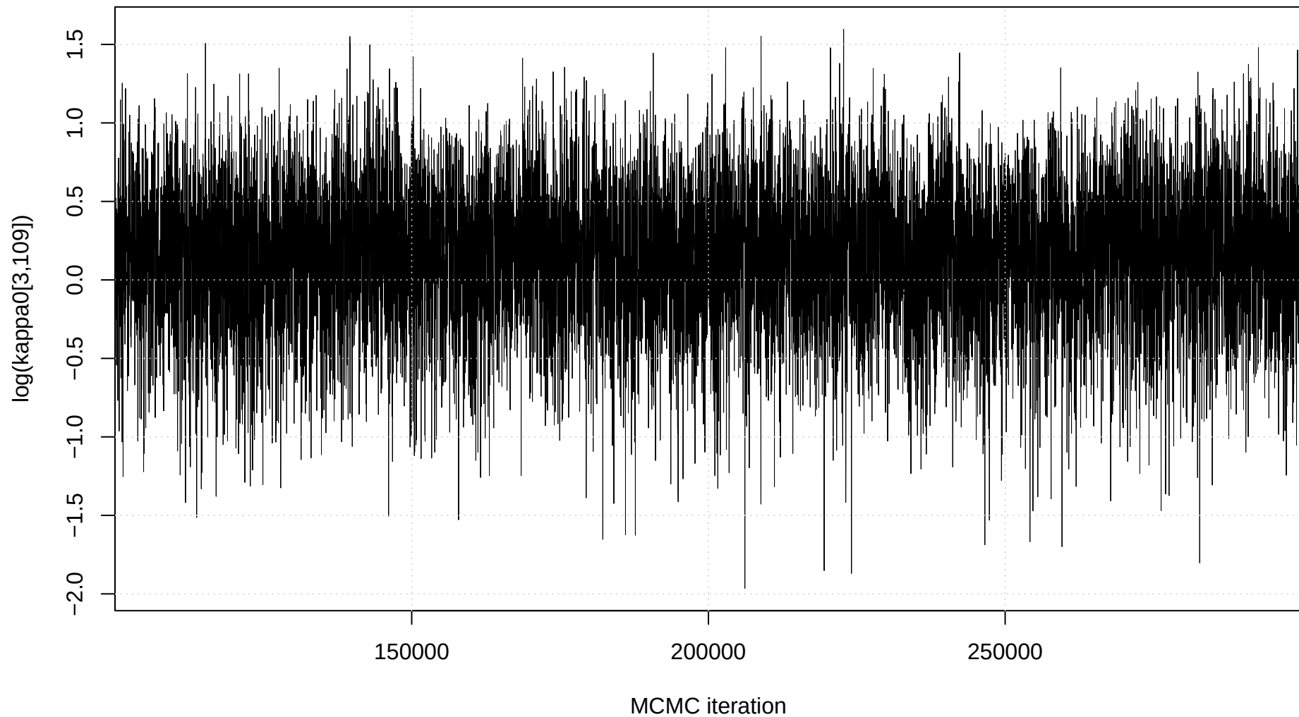
Trace plot: \log(\kappa_0[3,109])
