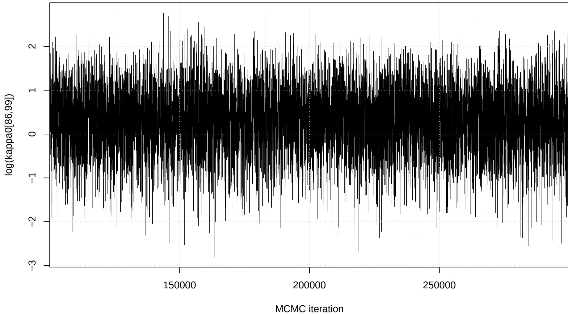
Trace plot: \log(\kappa_{0[86,99]})
