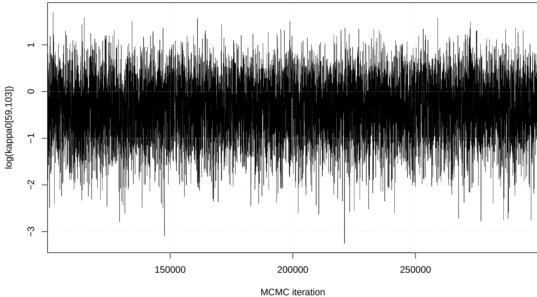
Trace plot: \log(\text{kappa0}[59,103])
