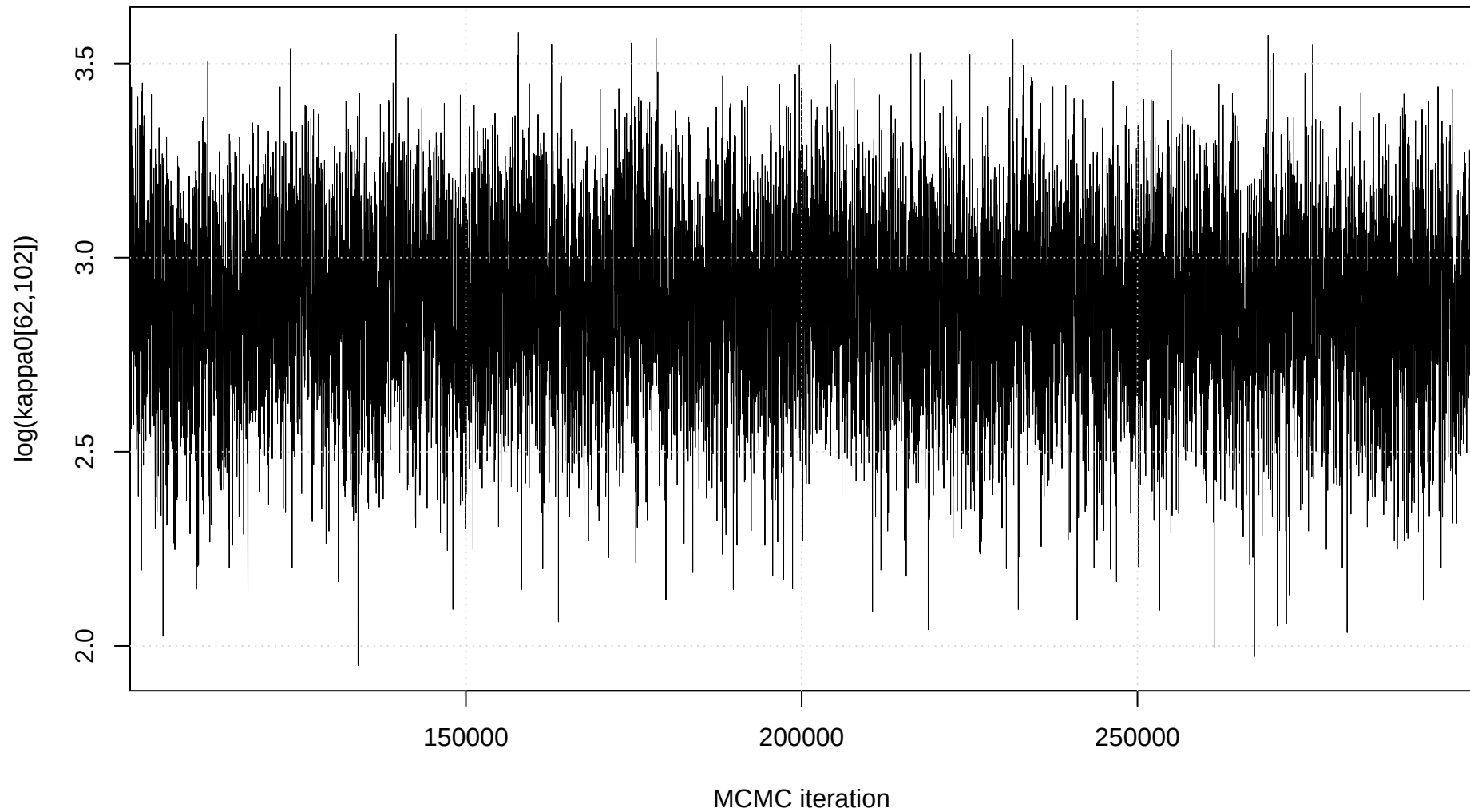
Trace plot: \log(\kappa_0[62,102])
