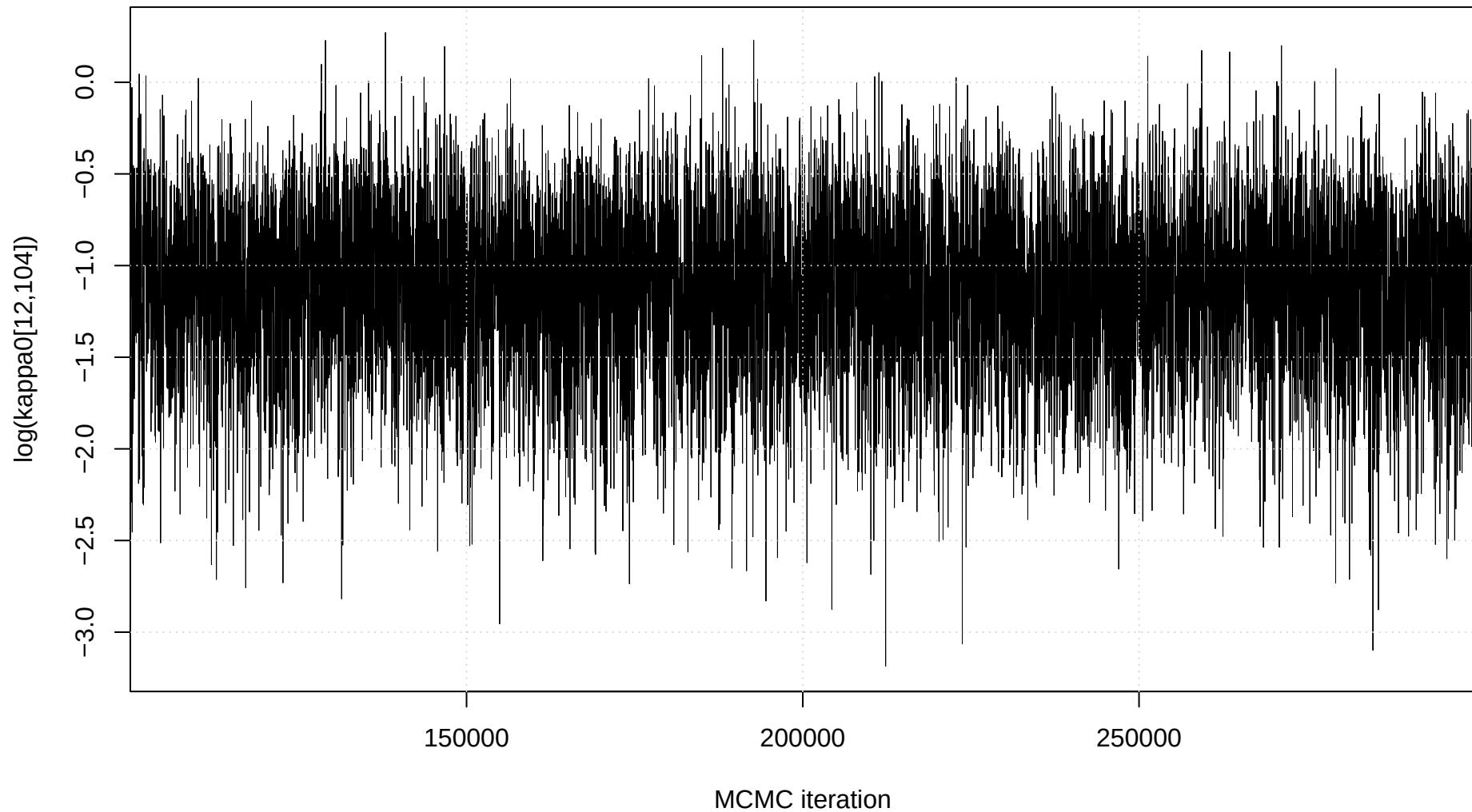
Trace plot: \log(\kappa_0[12,104])
