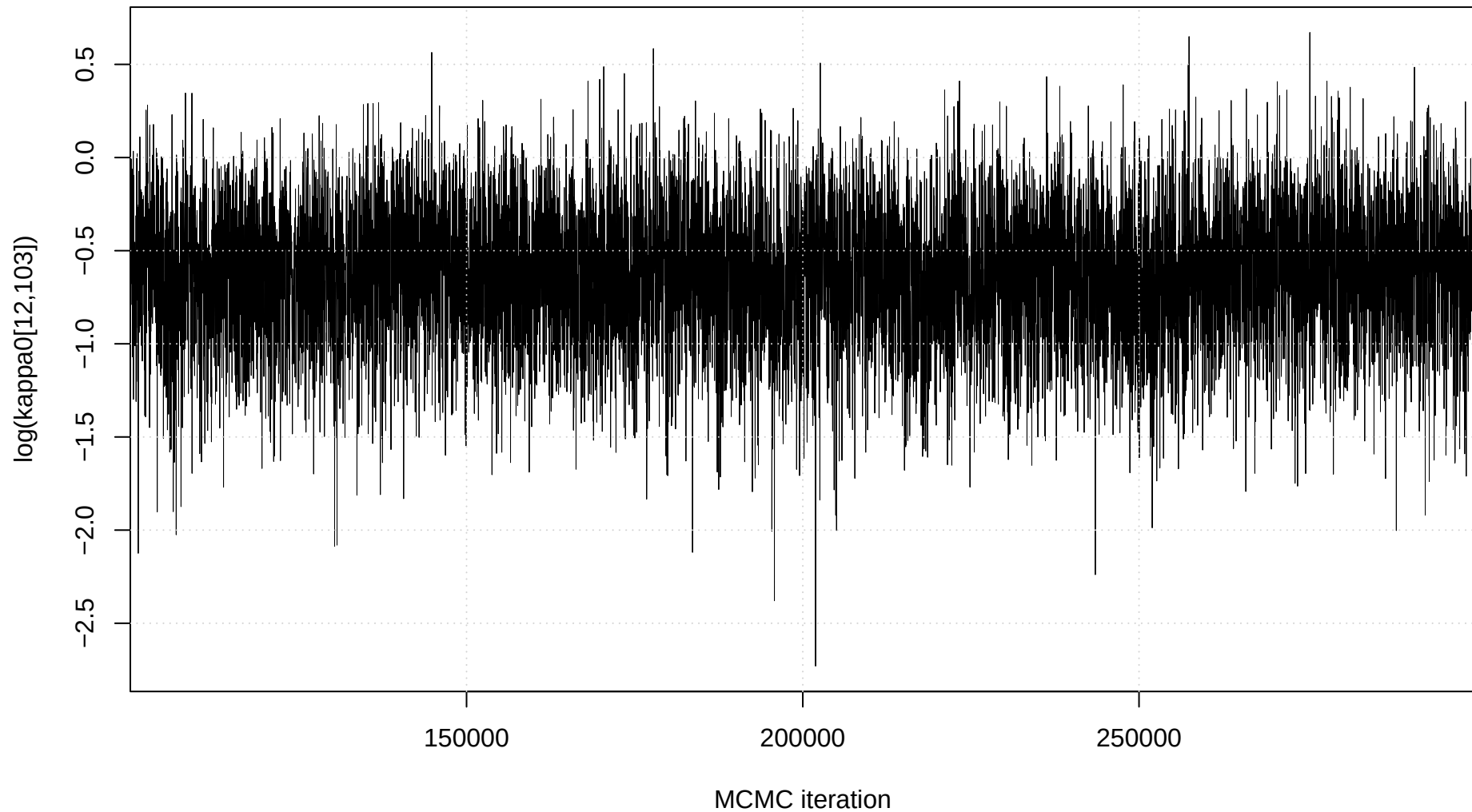
Trace plot: \log(\kappa_0[12,103])
