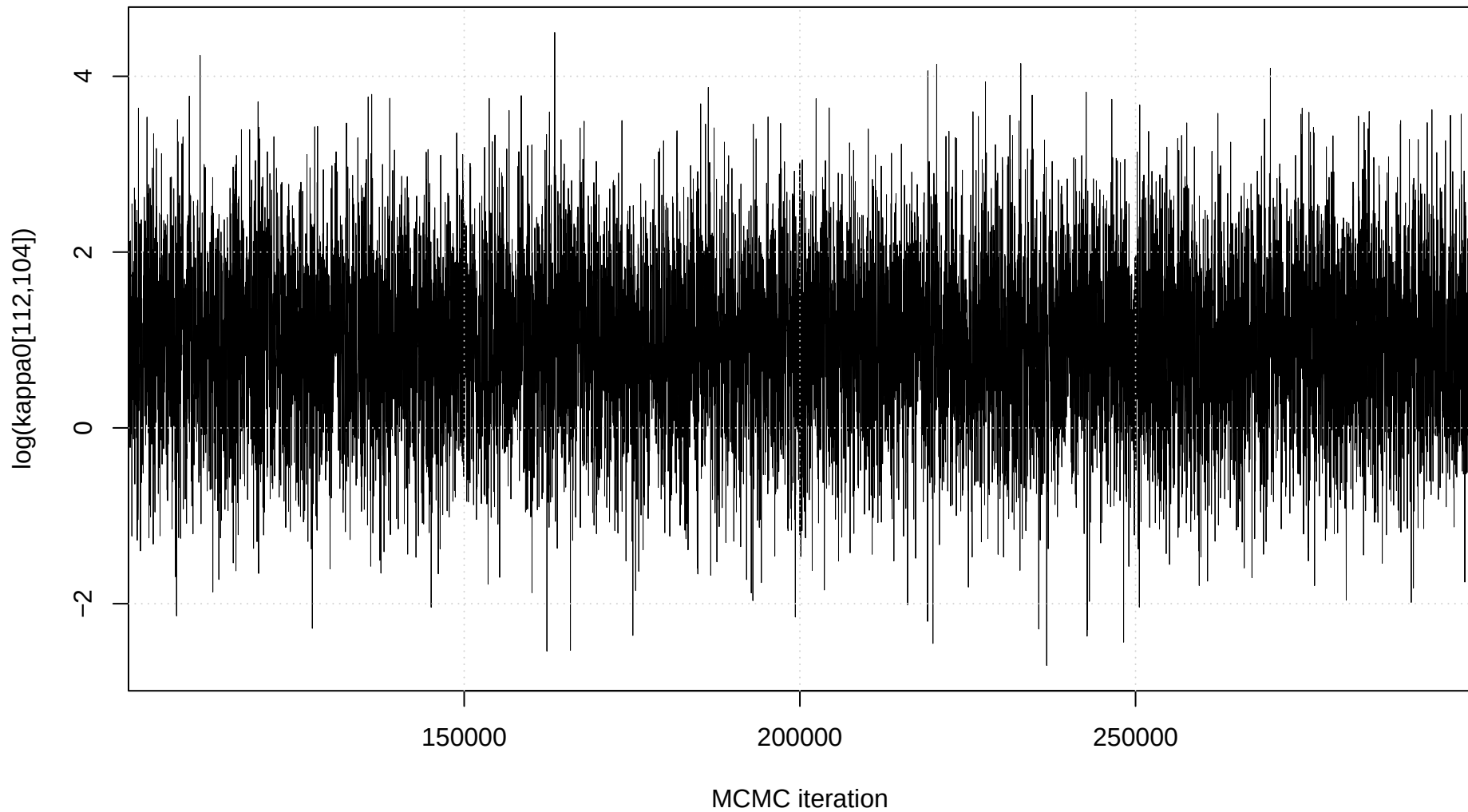
Trace plot: \log(\kappa_0[112,104])
