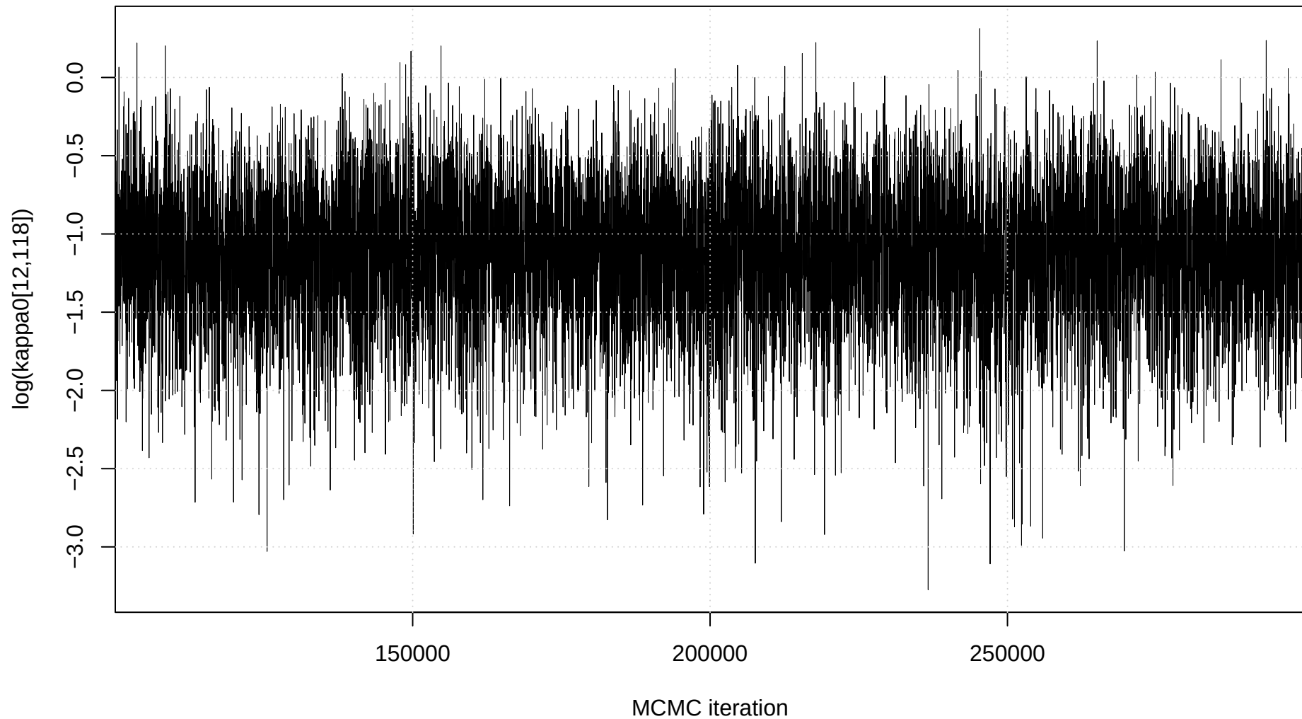
Trace plot: \log(\kappa_0[12,118])
