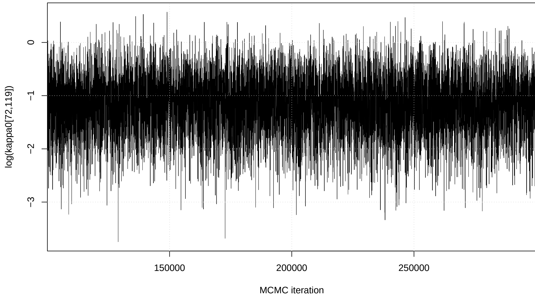
Trace plot: \log(\kappa_0[72,119])
