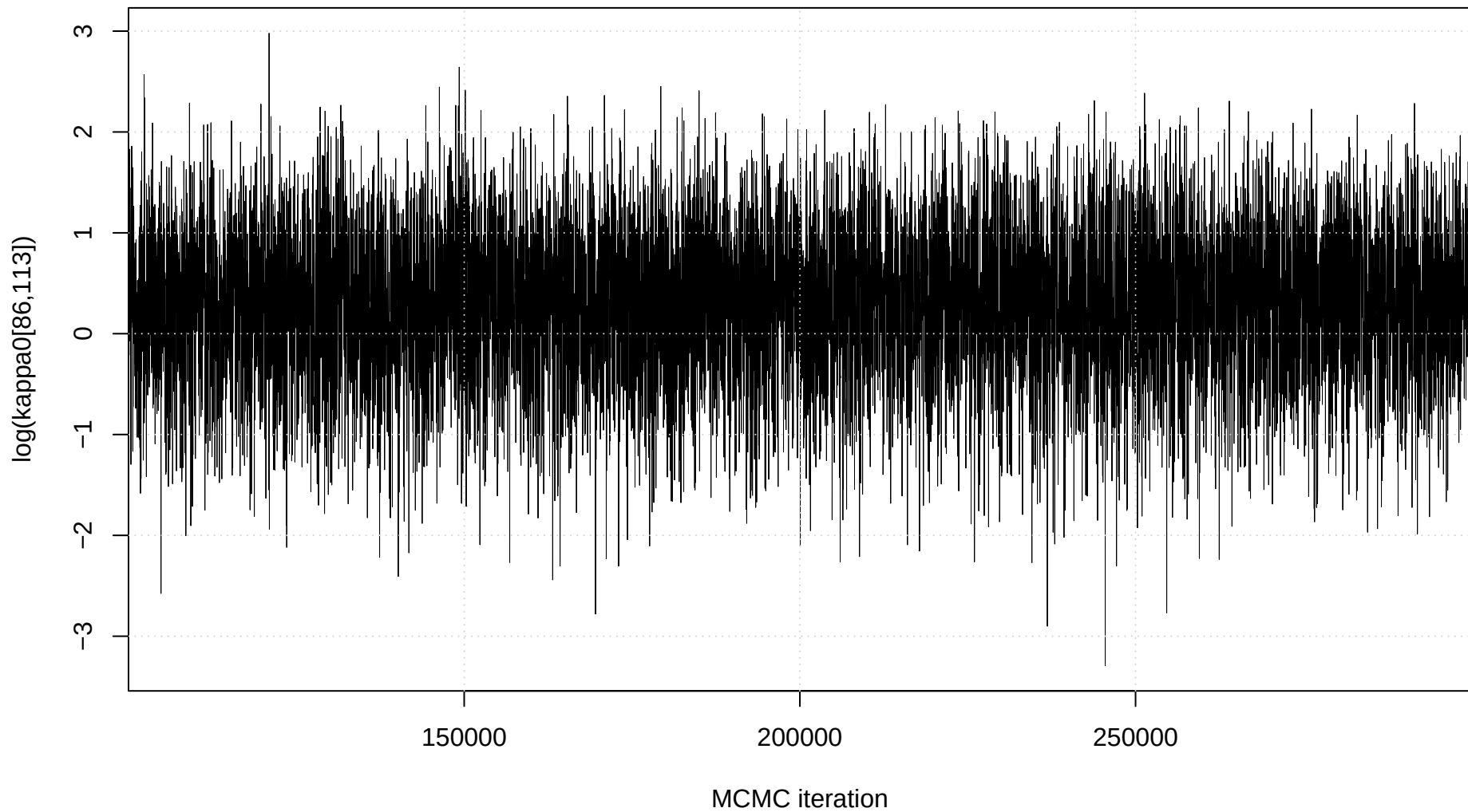
Trace plot: \log(\kappa_0[86,113])
