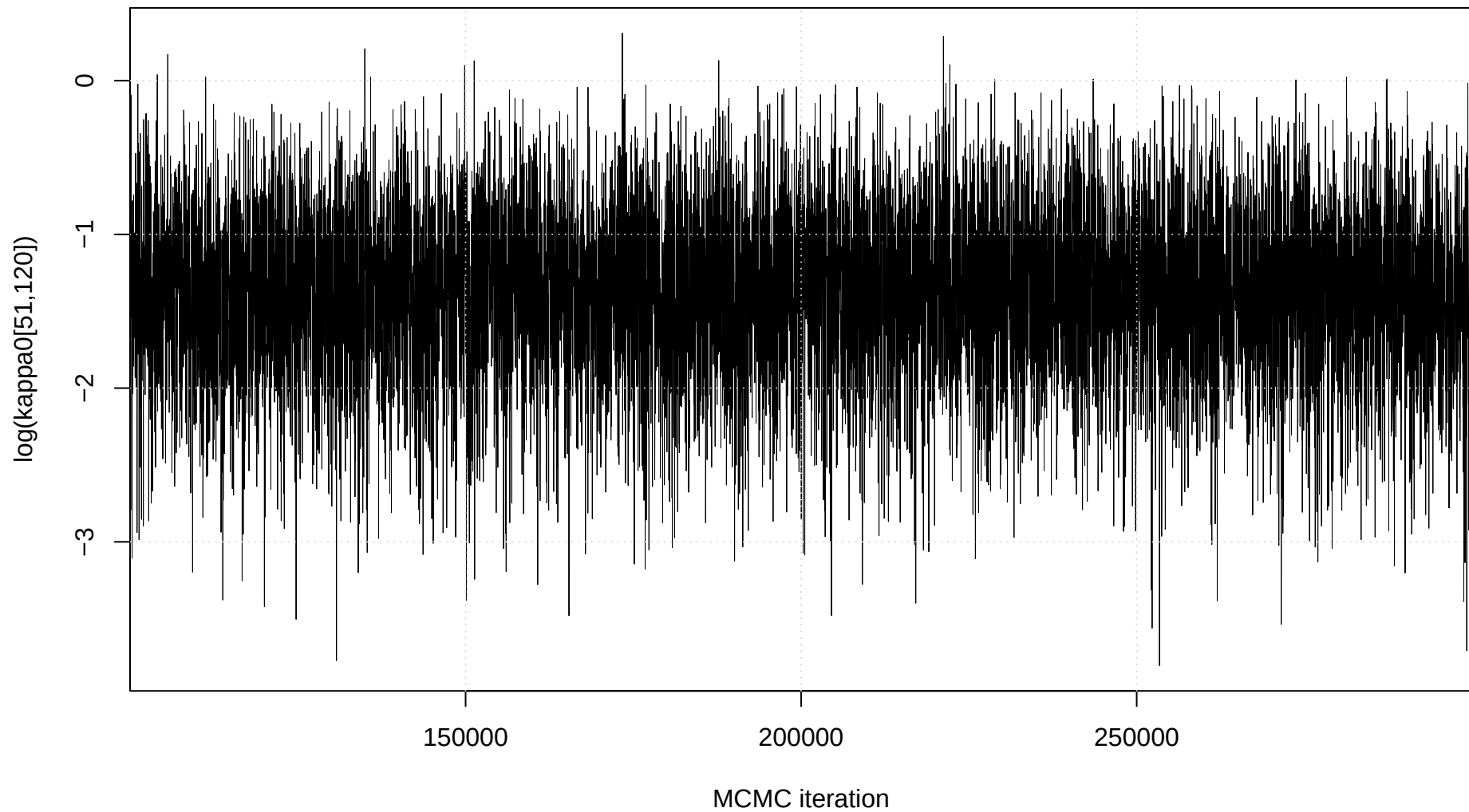
Trace plot: \log(\kappa_0[51,120])
