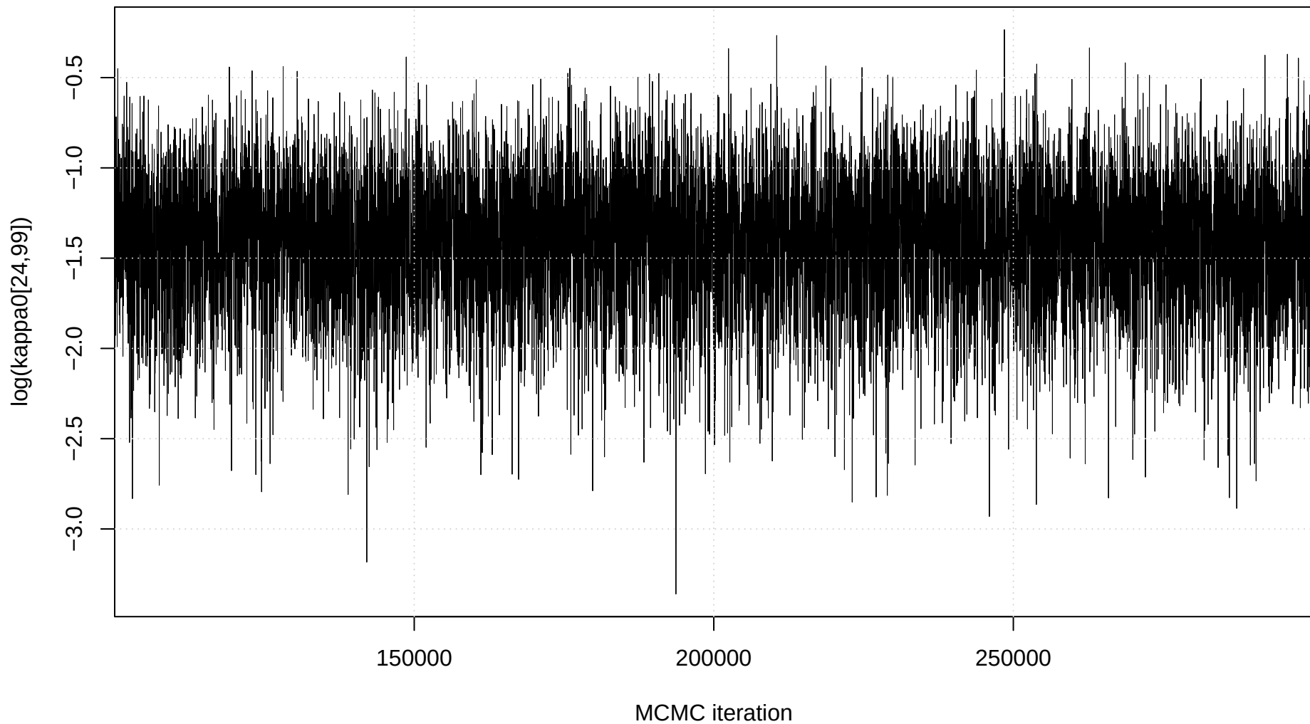
Trace plot: \log(\kappa_0[24,99])
