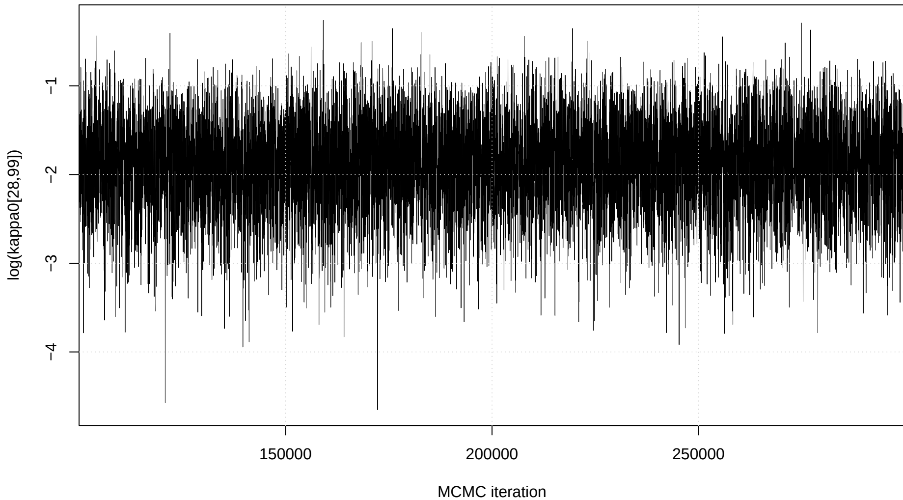
Trace plot: \log(\kappa_0[28,99])
