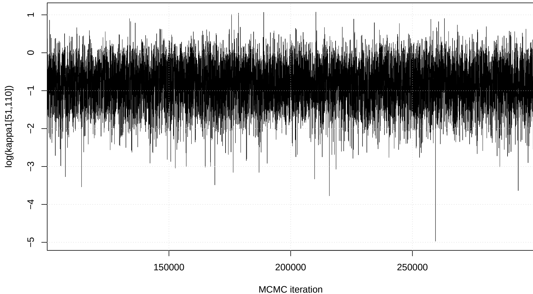
Trace plot: \log(\kappa_1[51,110])
