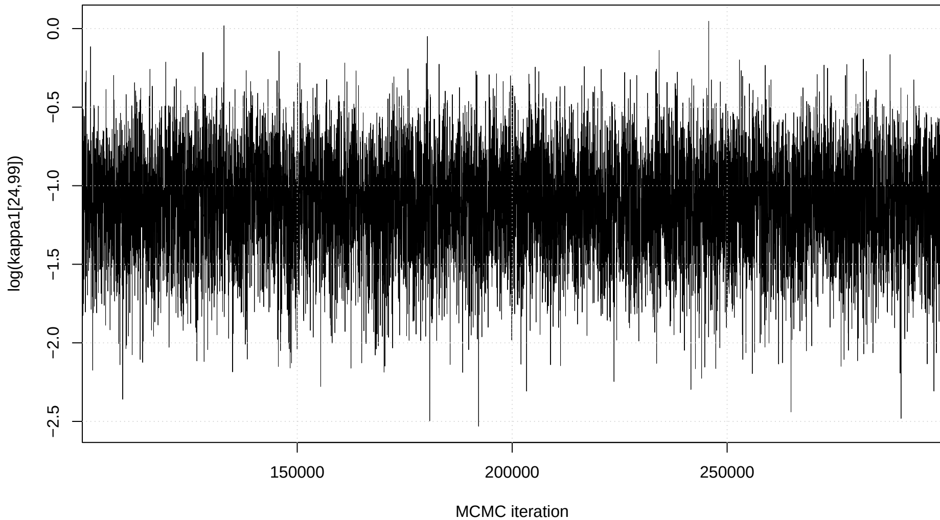
Trace plot: \log(\kappa_1[24,99])
