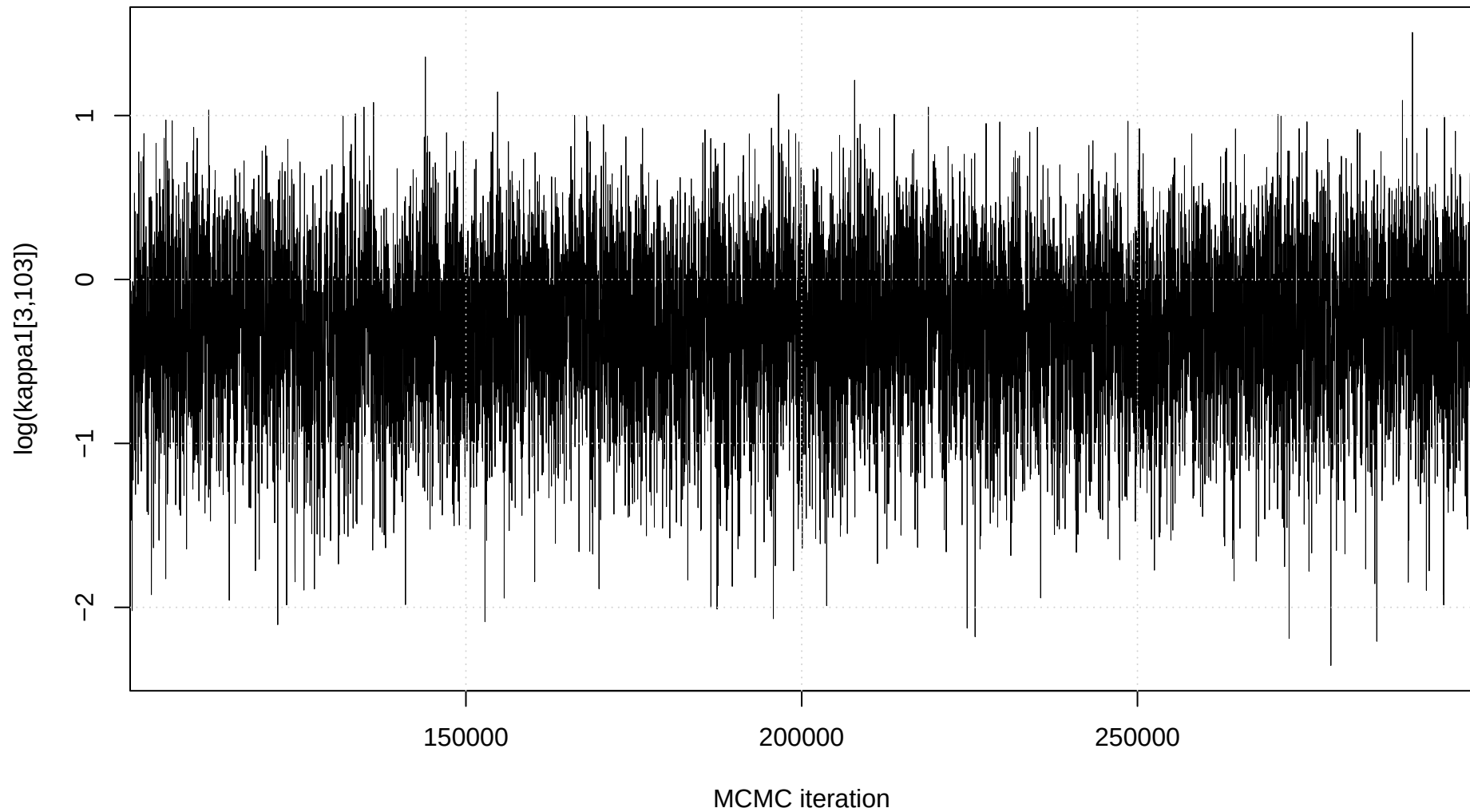
Trace plot: \log(\kappa_1[3,103])
