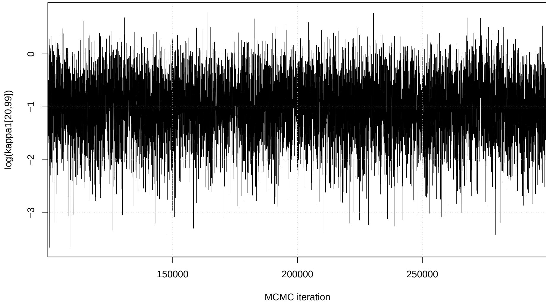
Trace plot: \log(\kappa_1[20,99])
