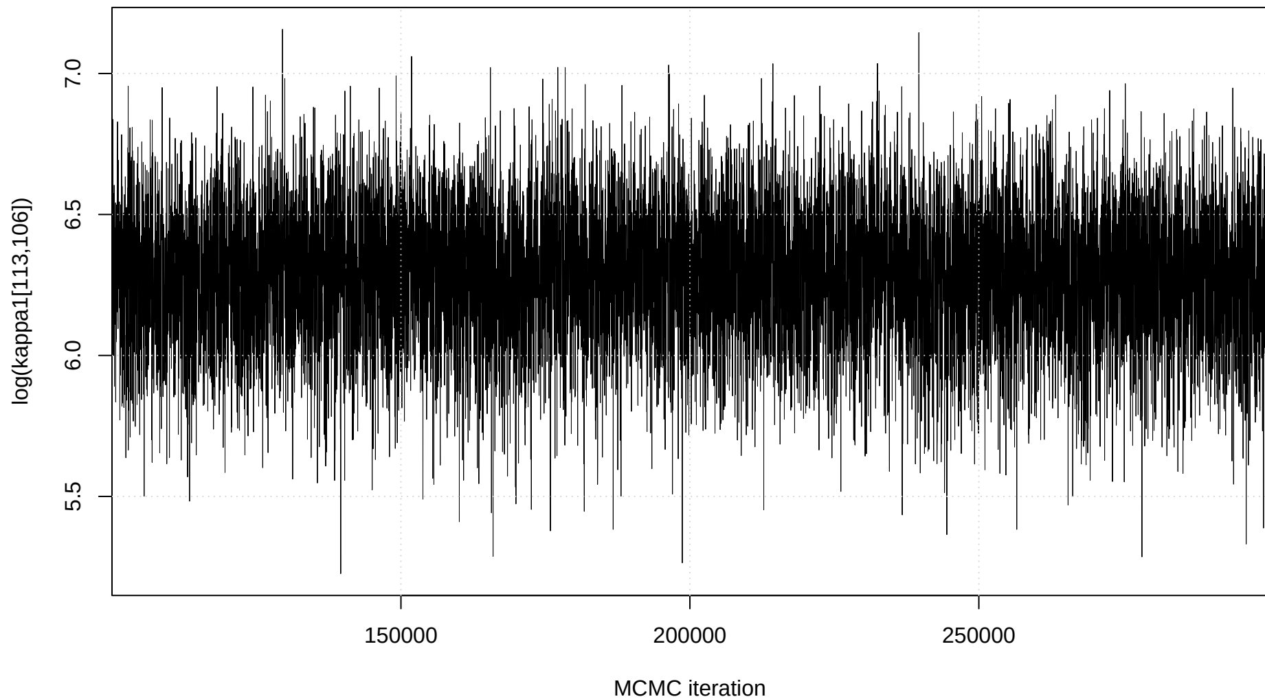
Trace plot: \log(\text{kappa1}[113,106])
