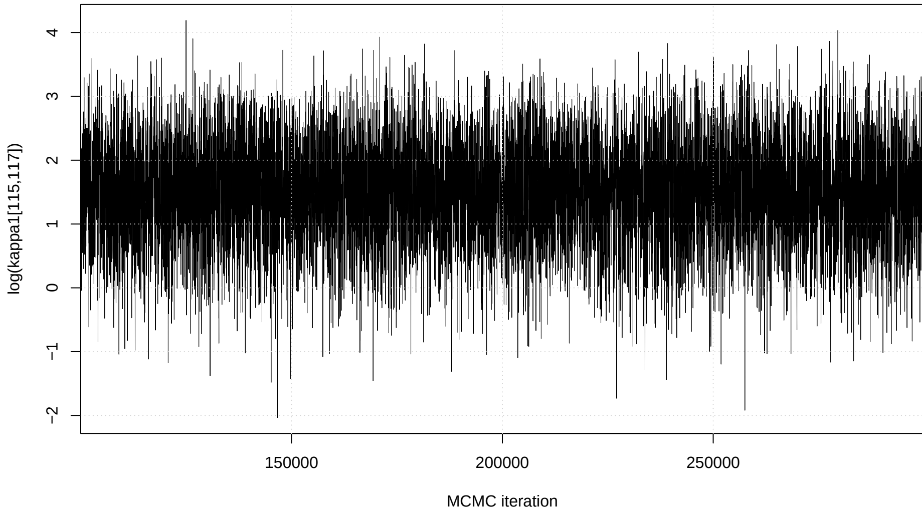
Trace plot: \log(\kappa_1[115,117])
