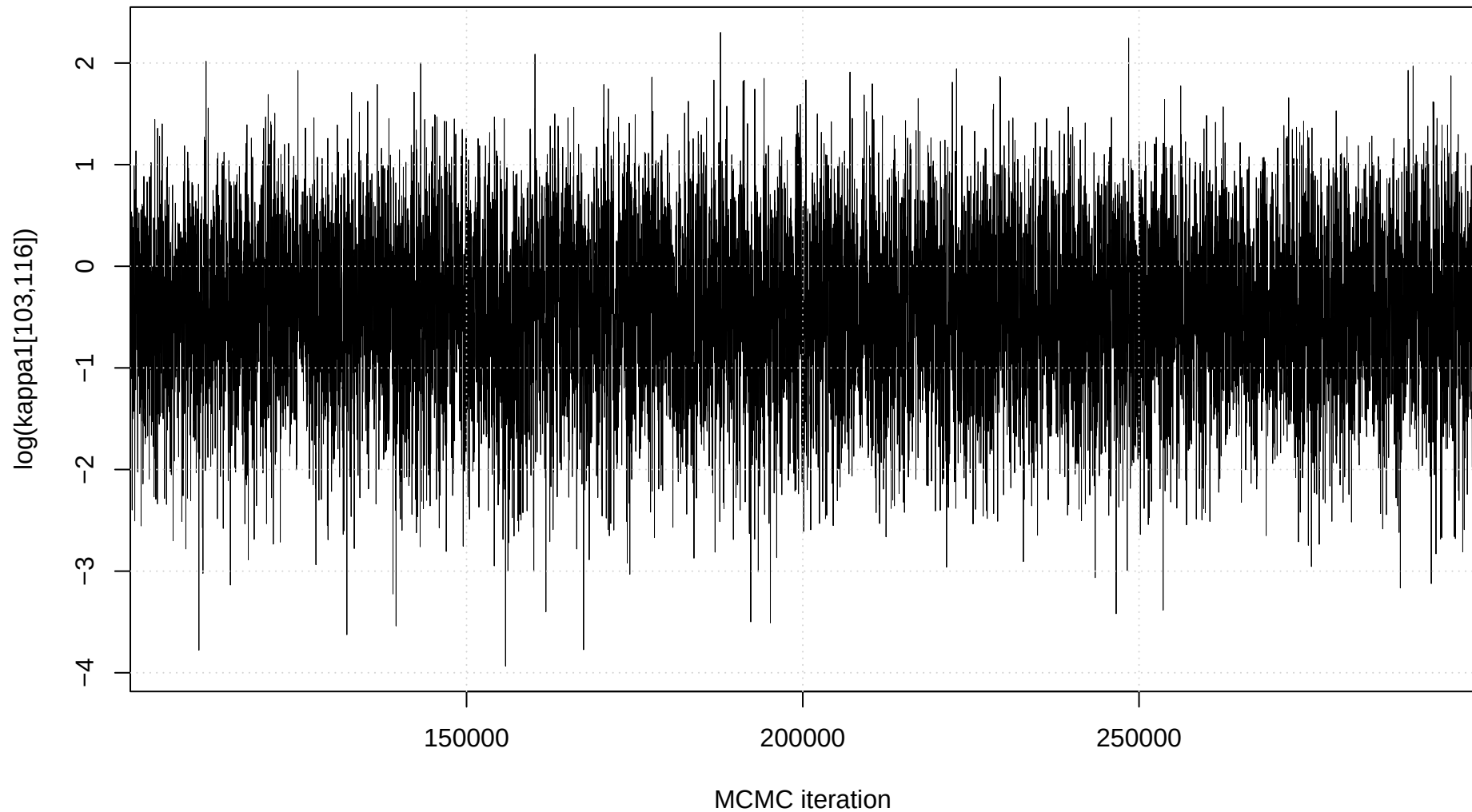
Trace plot: \log(\text{kappa1}[103,116])
