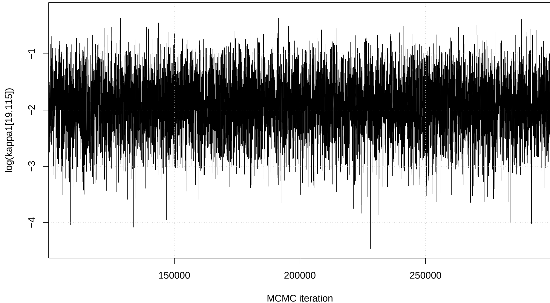
Trace plot: \log(\kappa_1[19,115])
