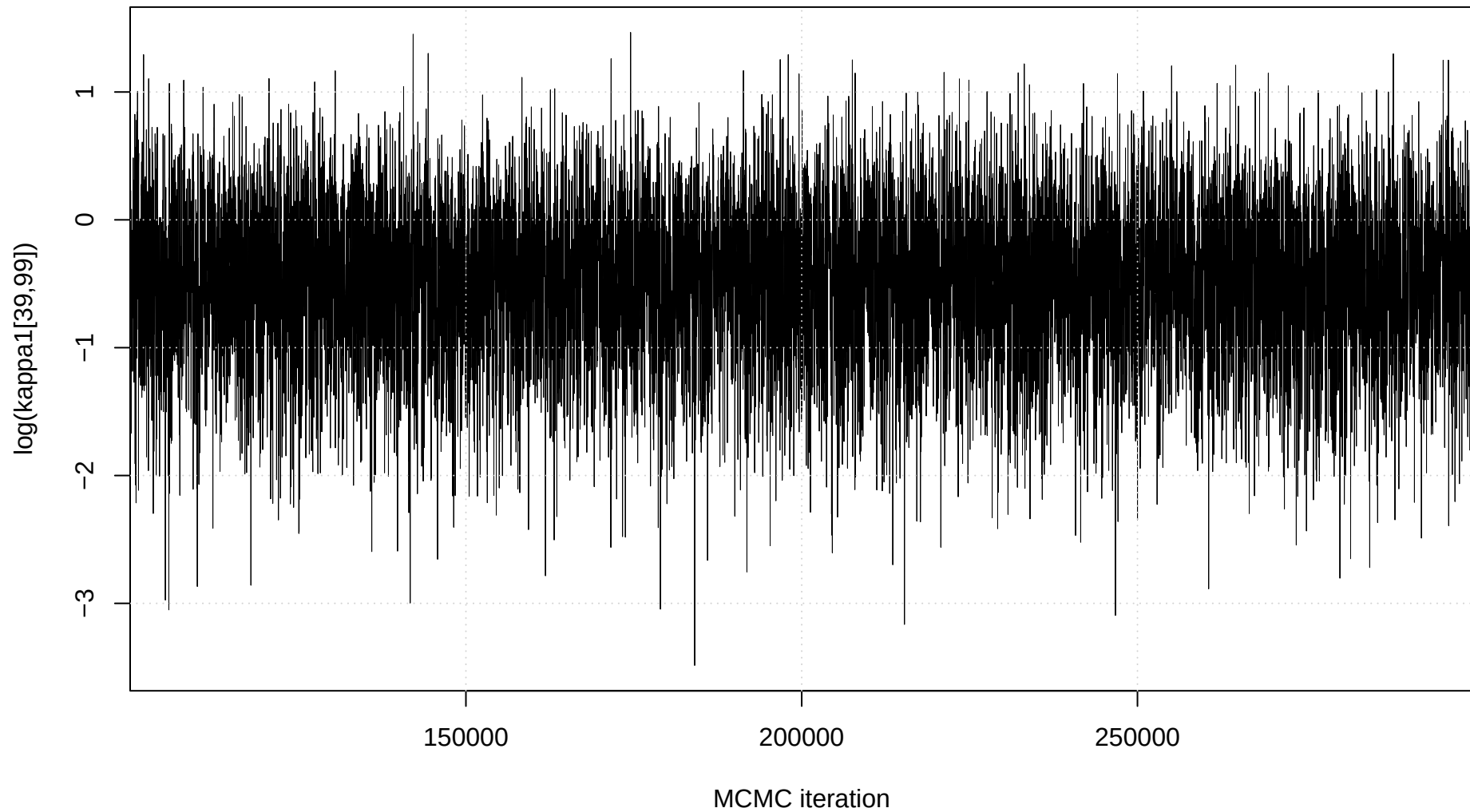
Trace plot: \log(\kappa_1[39,99])
