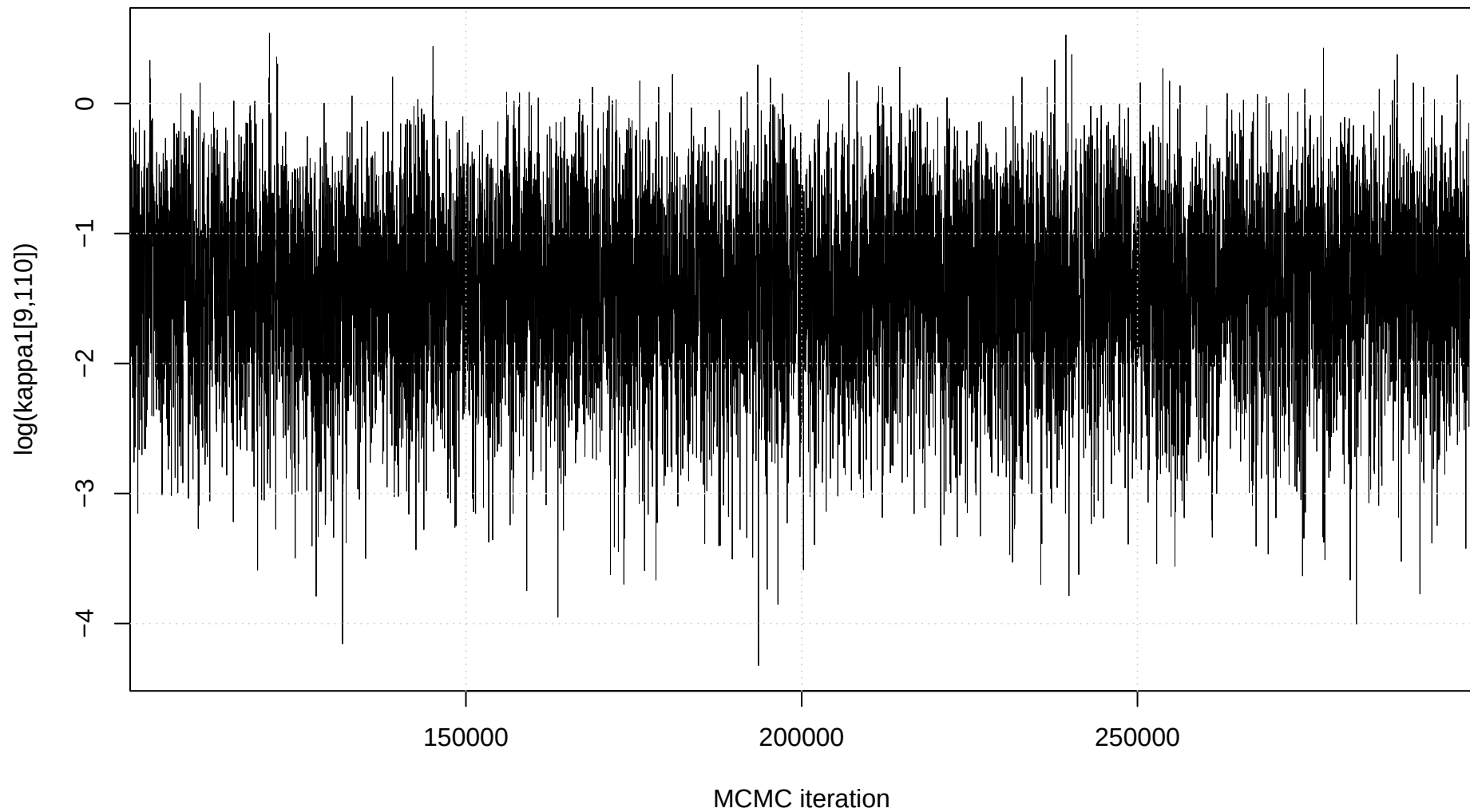
Trace plot: \log(\kappa_1[9,110])
