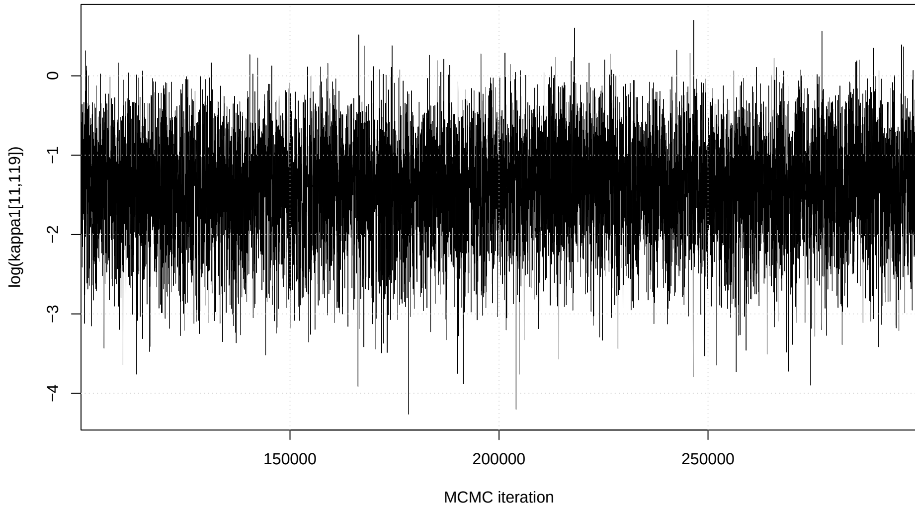
Trace plot: \log(\kappa_1[11,119])
