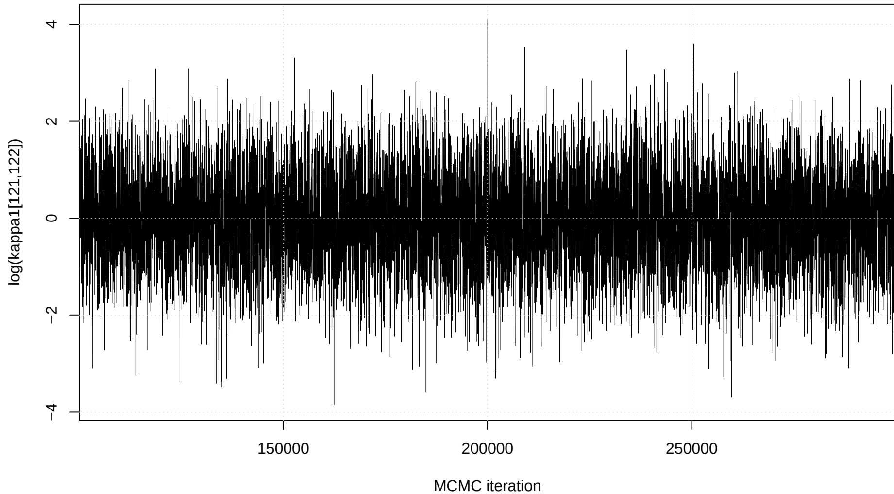
Trace plot: \log(\text{kappa1}[121,122])
