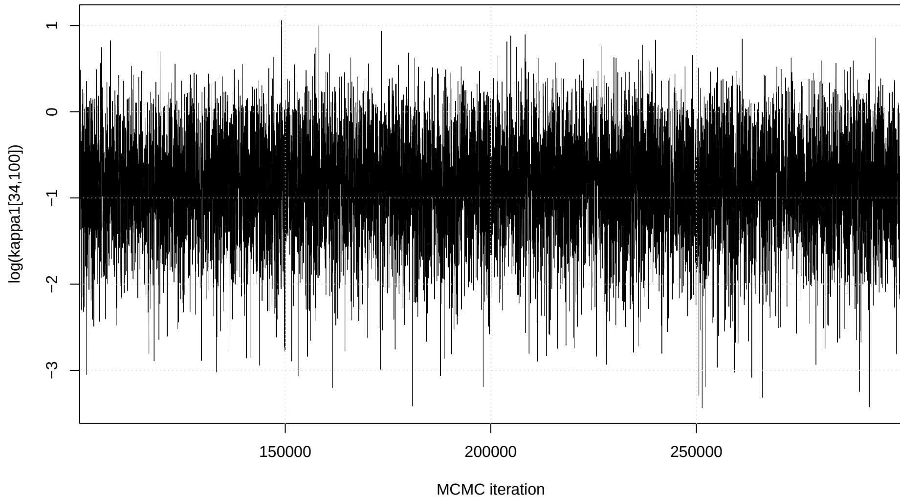
Trace plot: \log(\kappa_1[34,100])
