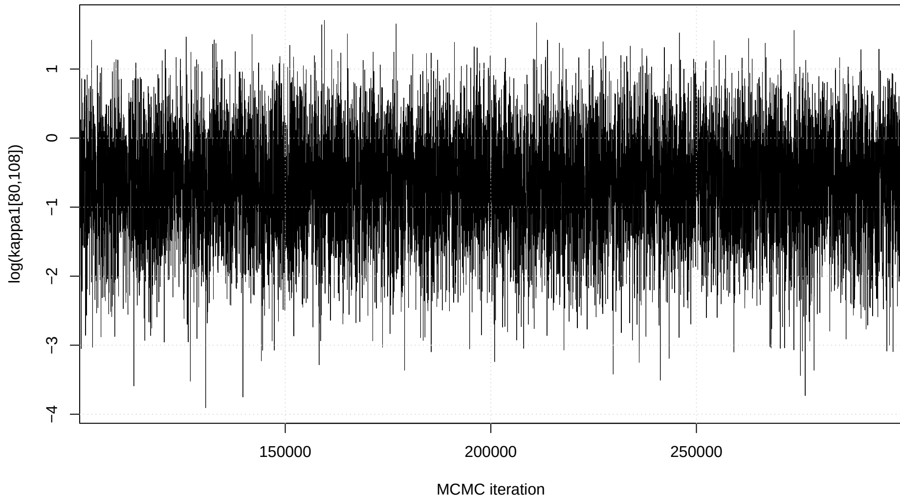
Trace plot: \log(\kappa_1[80,108])
