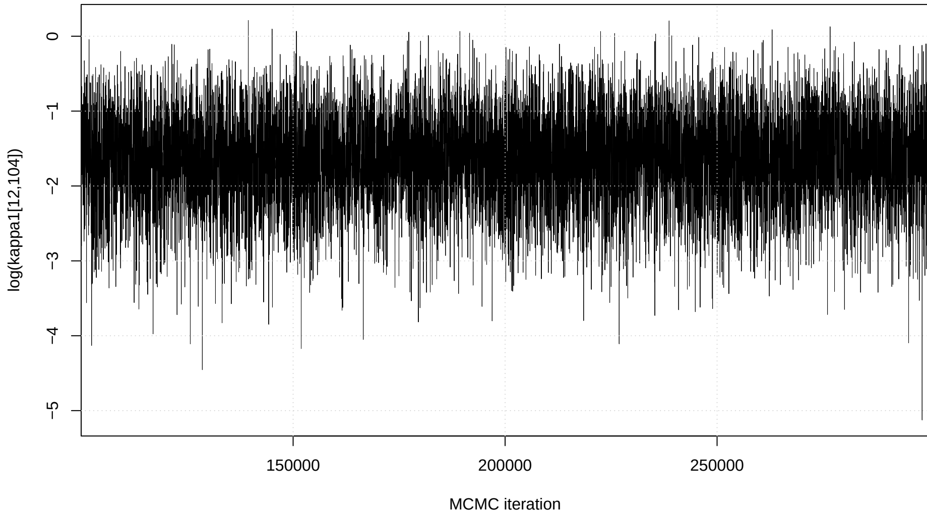
Trace plot: \log(\kappa_1[12,104])
