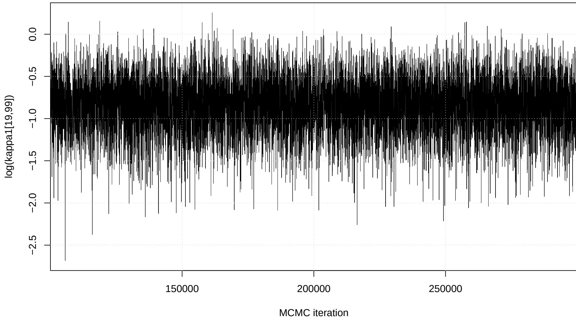
Trace plot: \log(\kappa_1[19,99])
