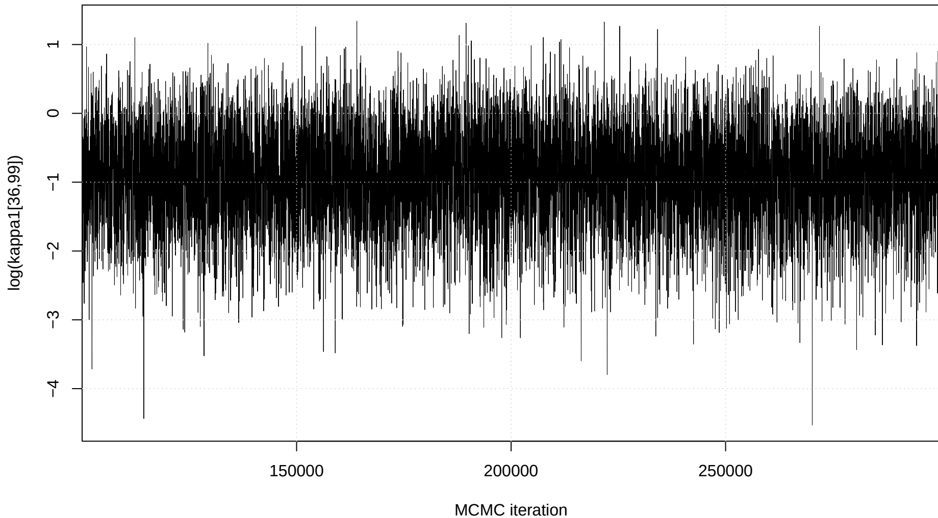
Trace plot: \log(\kappa_1[36,99])
