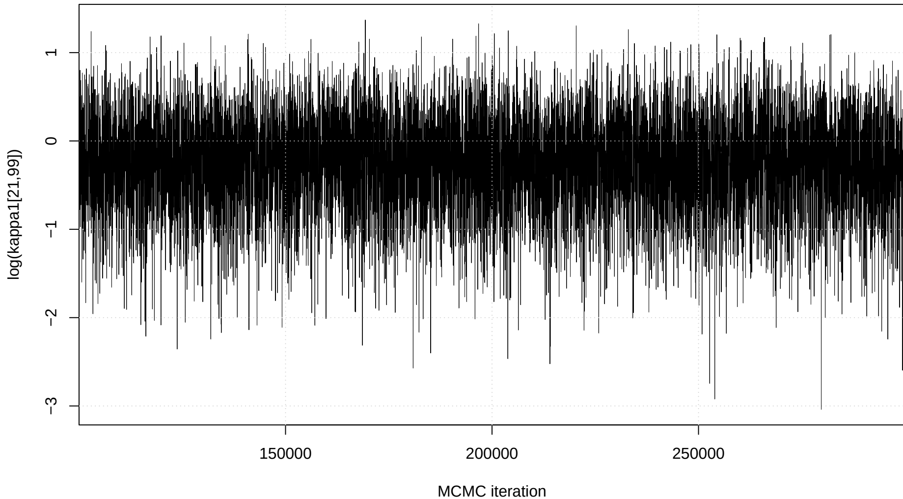
Trace plot: \log(\kappa_{1[21,99]})
