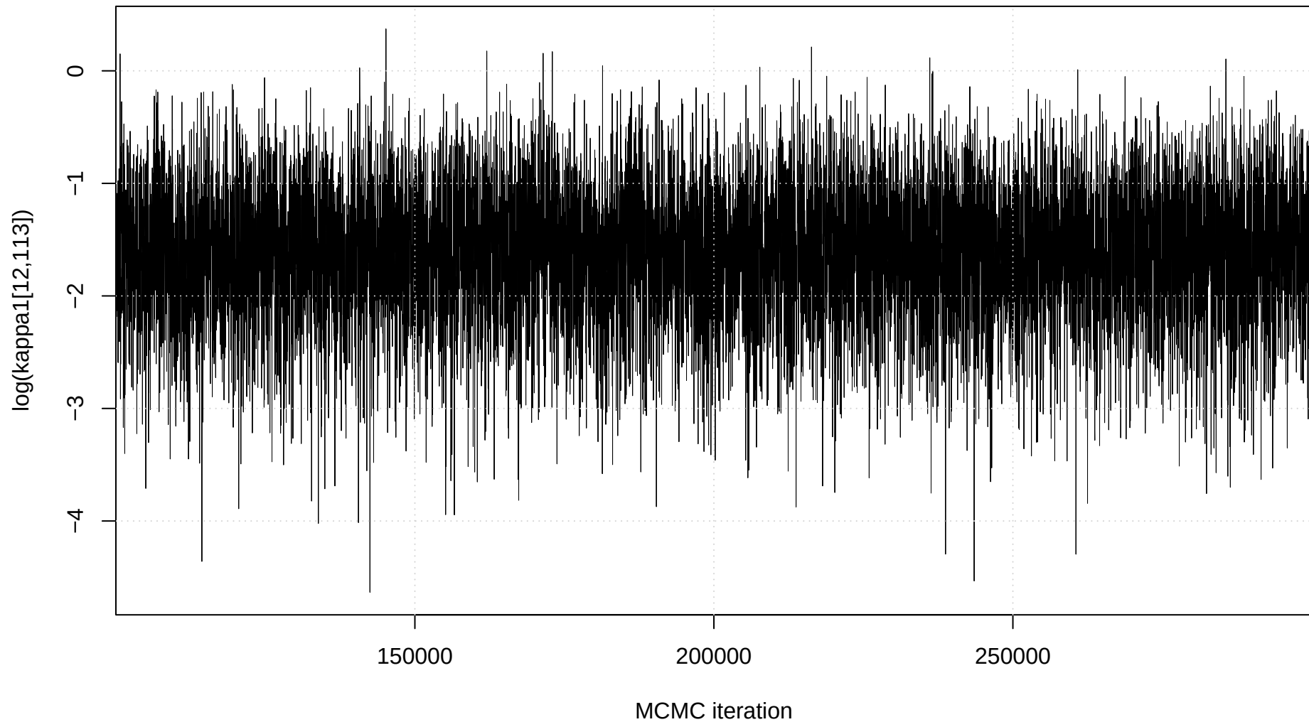
Trace plot: \log(\kappa_1[12,113])
