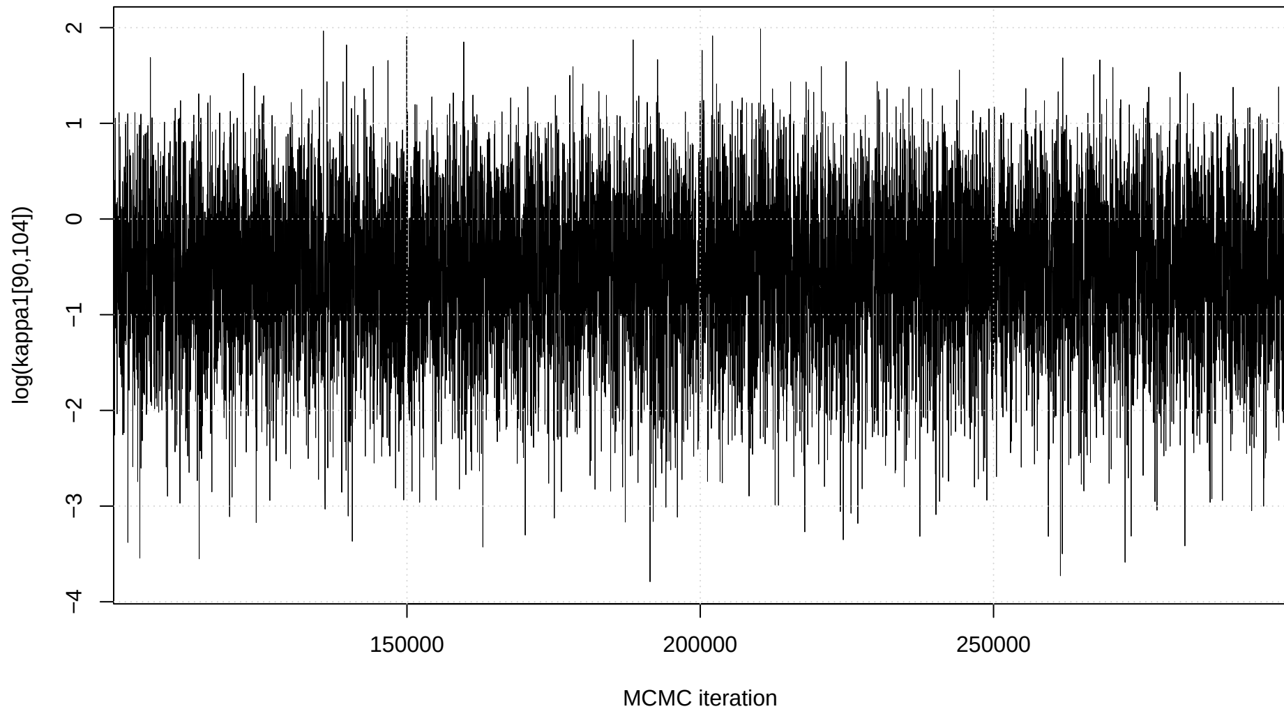
Trace plot: \log(\kappa_1[90,104])
