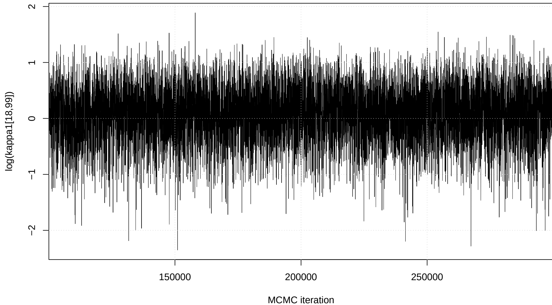
Trace plot: \log(\kappa_1[18,99])
