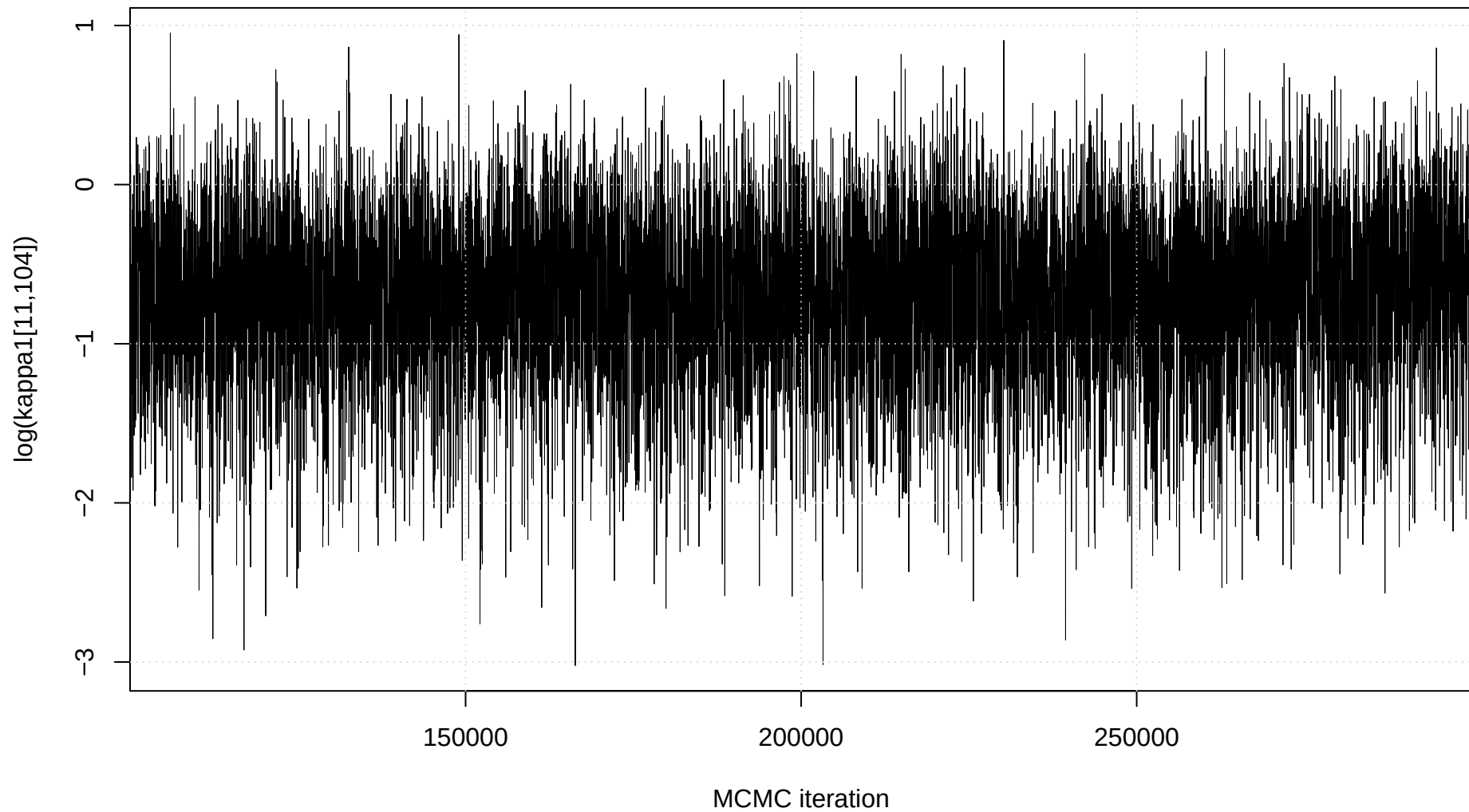
Trace plot: \log(\kappa_1[11,104])
