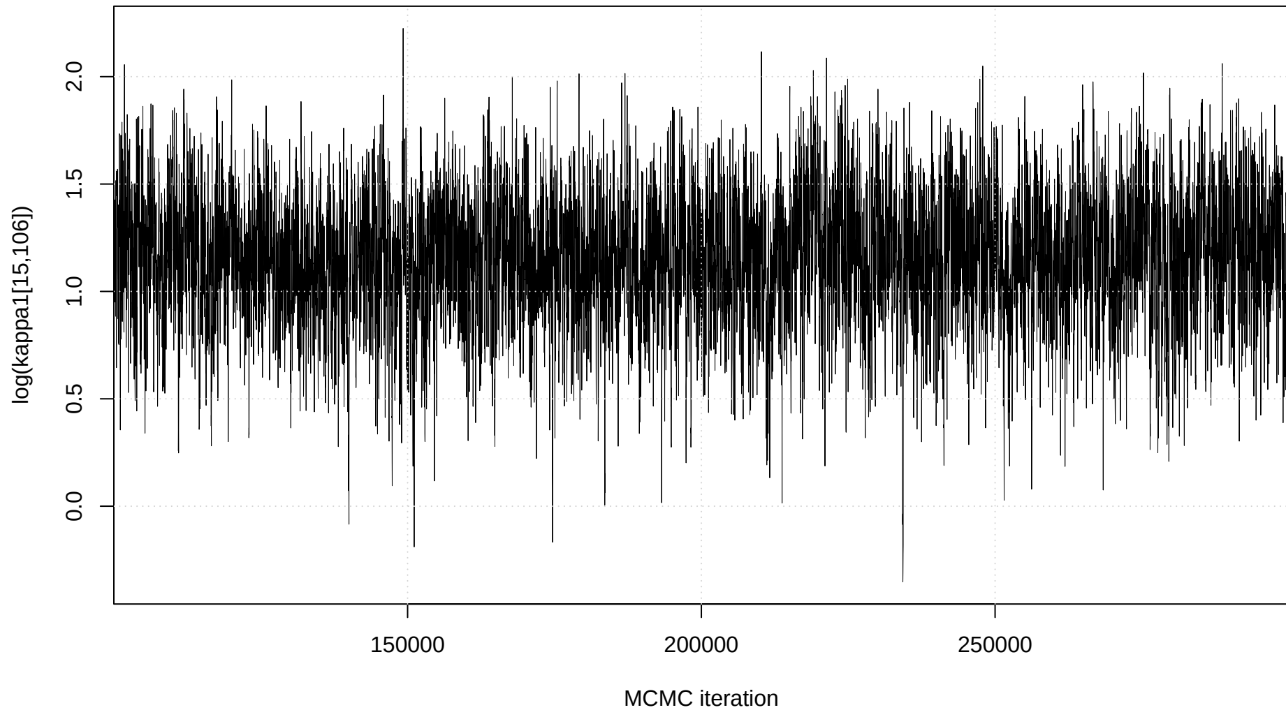
Trace plot: \log(\kappa_1[15,106])
