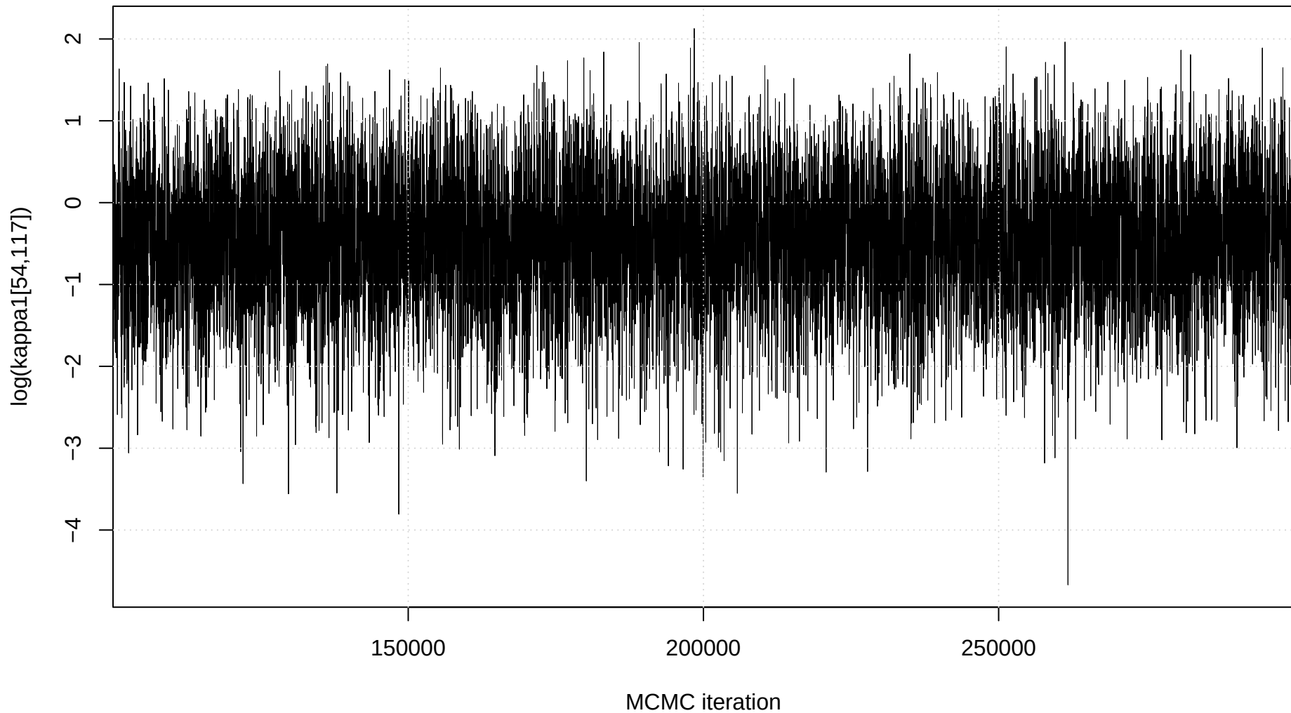
Trace plot: \log(\kappa_1[54,117])
