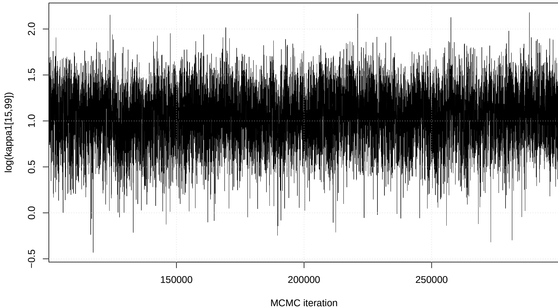
Trace plot: \log(\kappa_1[15,99])
