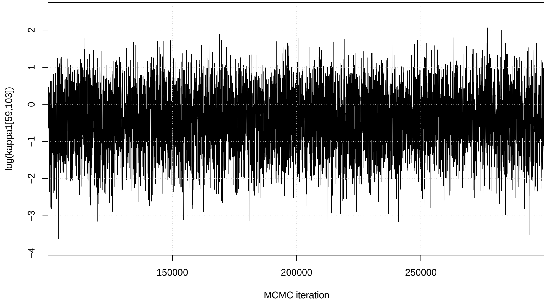
Trace plot: \log(\kappa_1[59,103])
