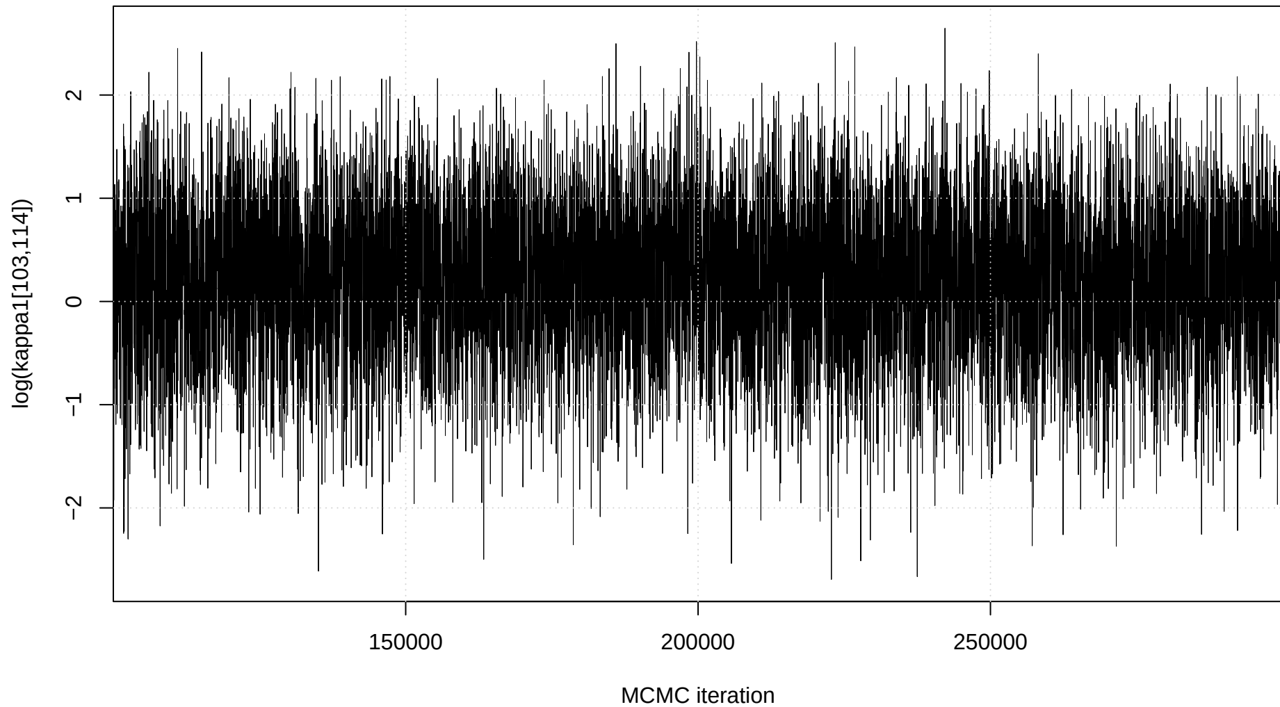
Trace plot: \log(\kappa_1[103,114])
