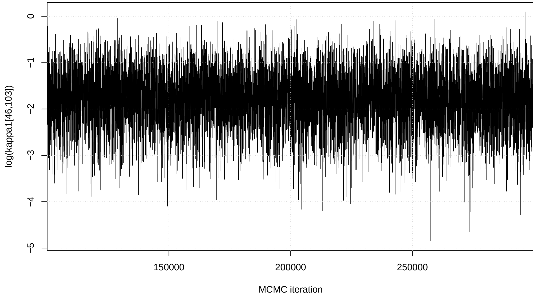
Trace plot: \log(\kappa_1[46,103])
