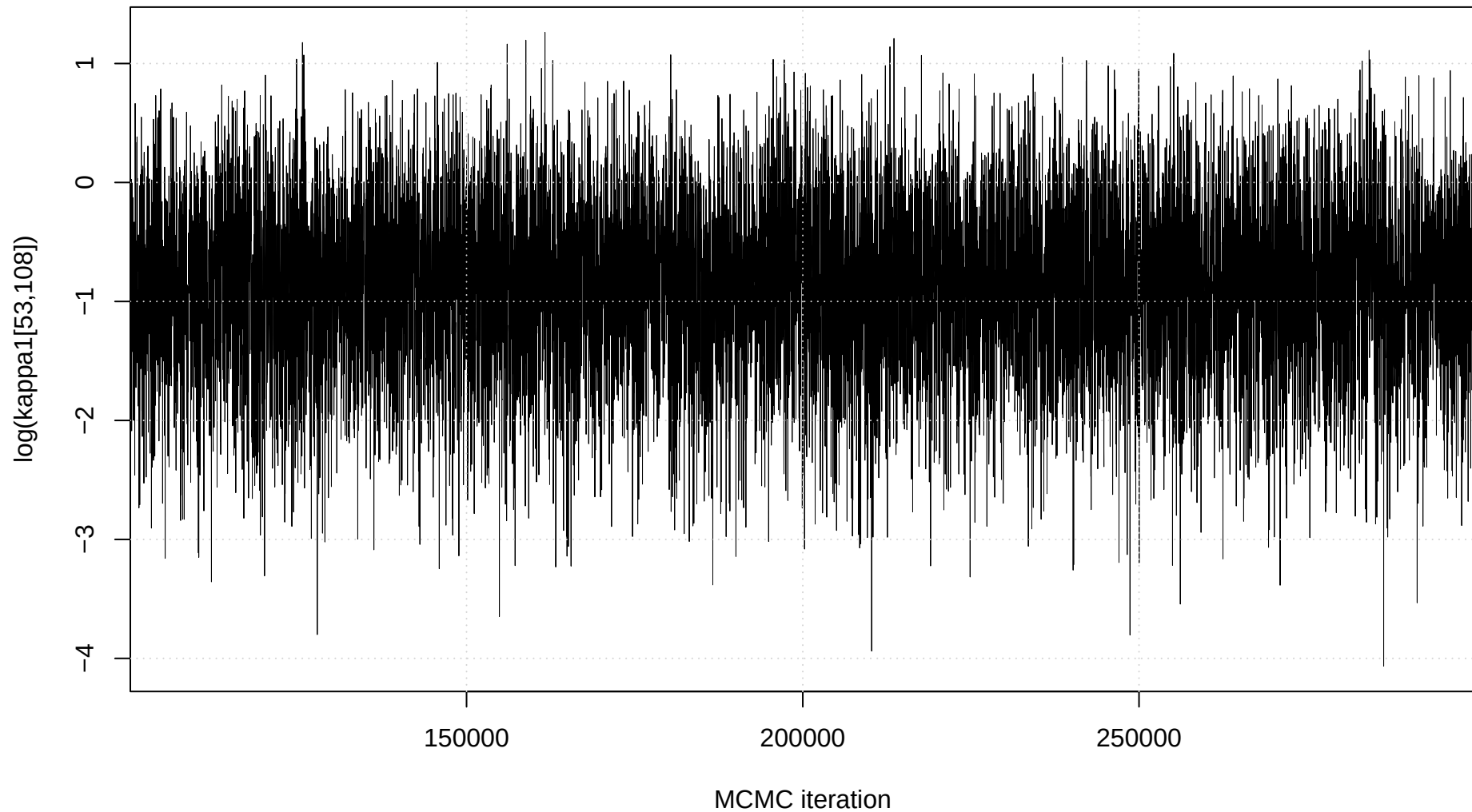
Trace plot: \log(\kappa_1[53,108])
