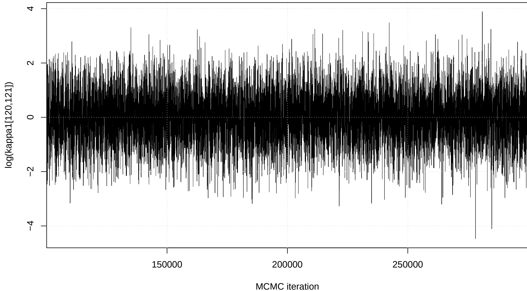
Trace plot: \log(\kappa_1[120,121])
