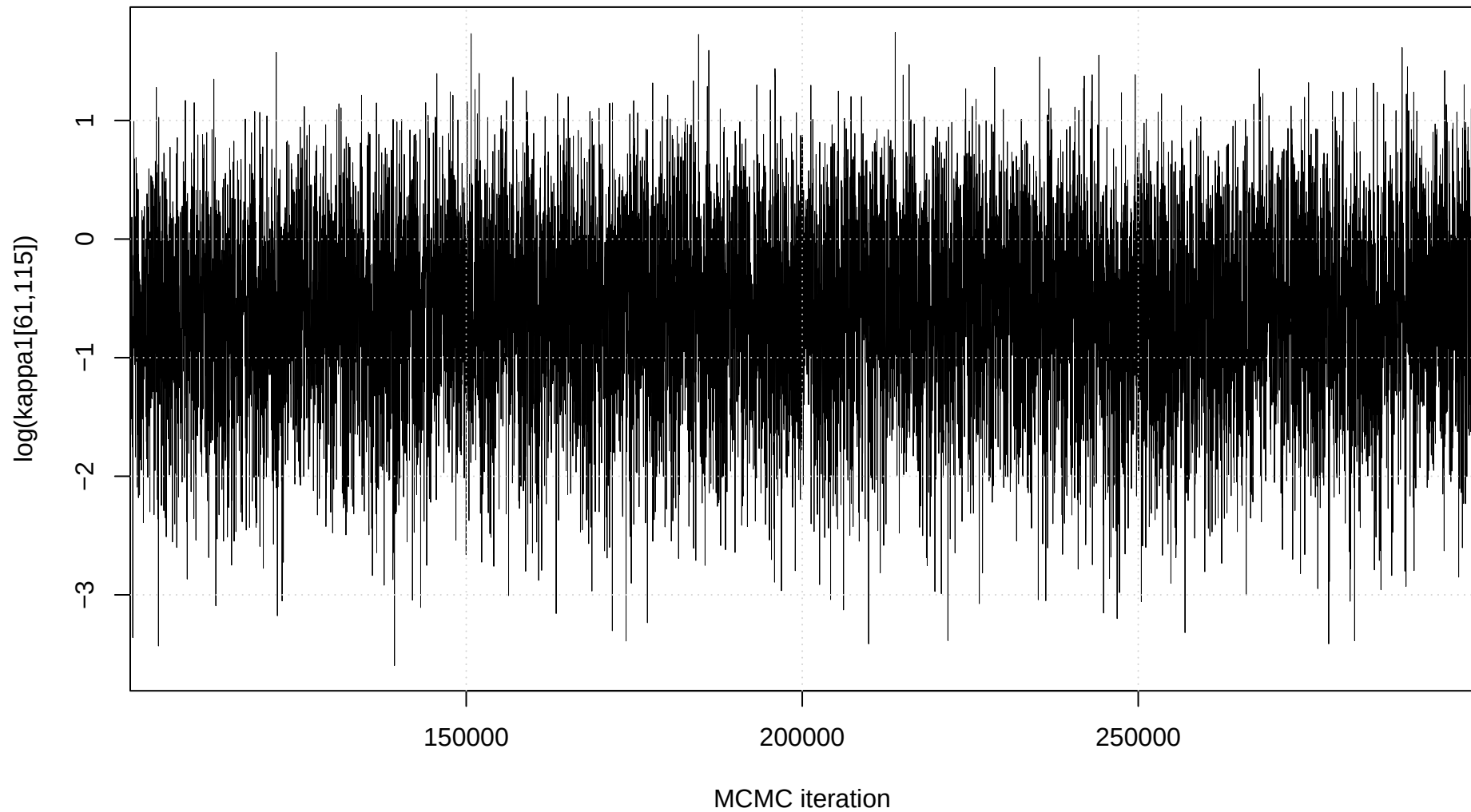
Trace plot: \log(\kappa_1[61,115])
