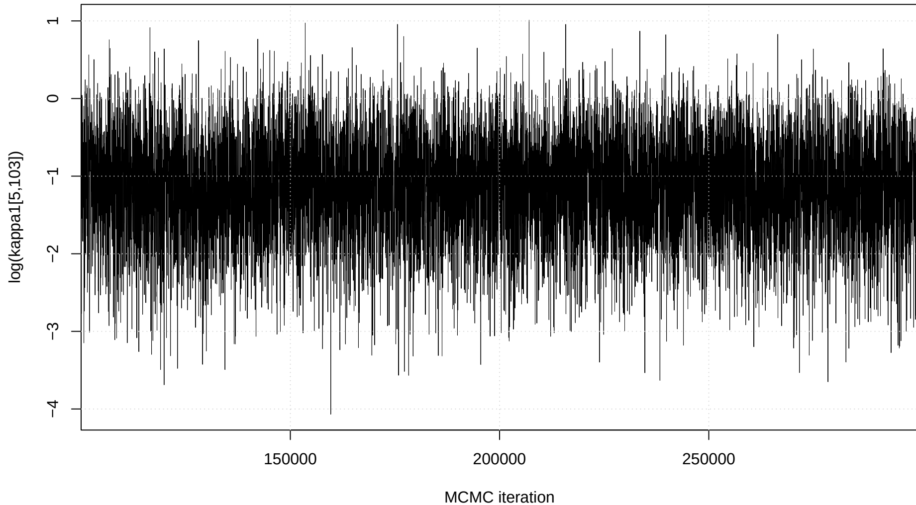
Trace plot: \log(\kappa_1[5,103])
