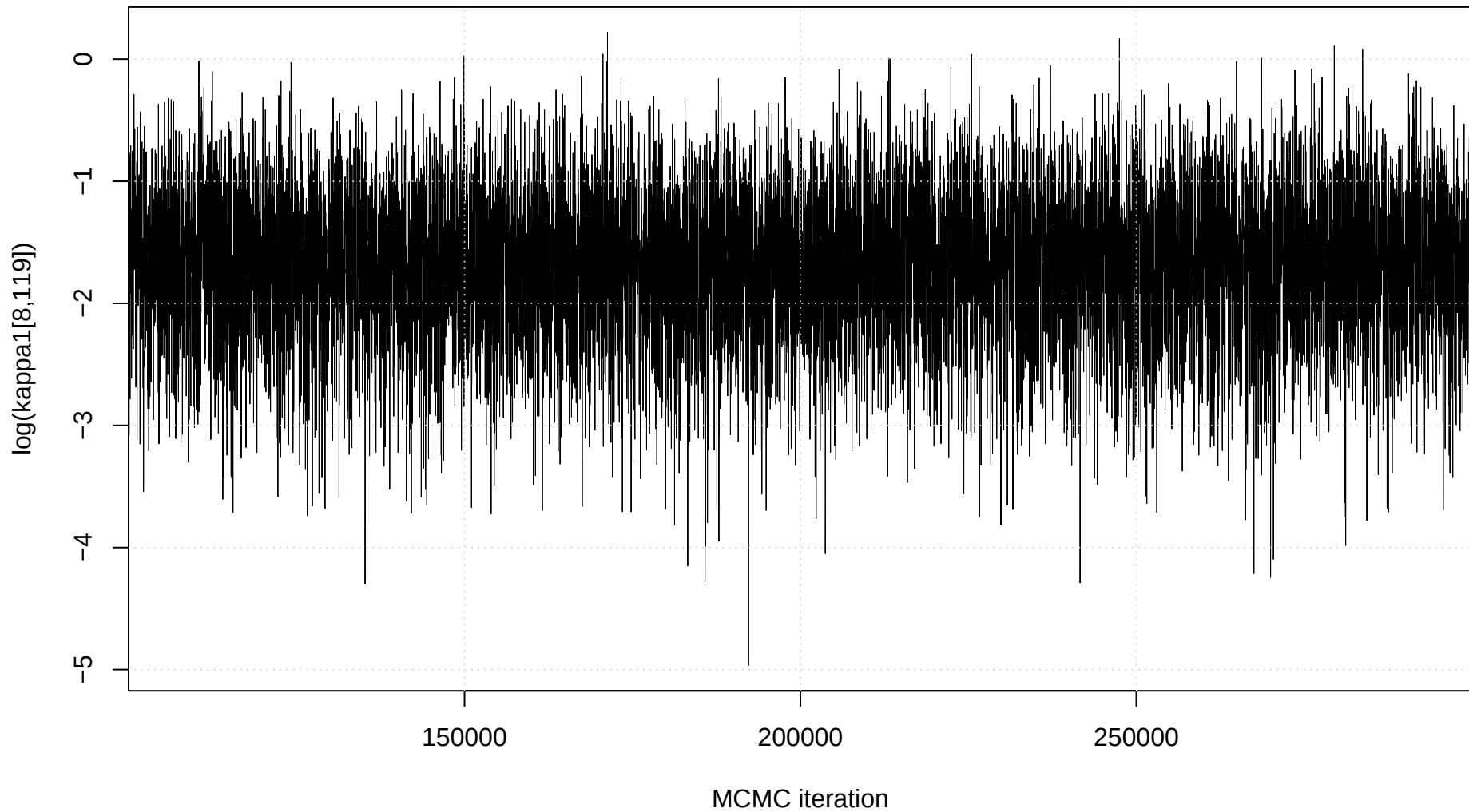
Trace plot: \log(\kappa_1[8,119])
