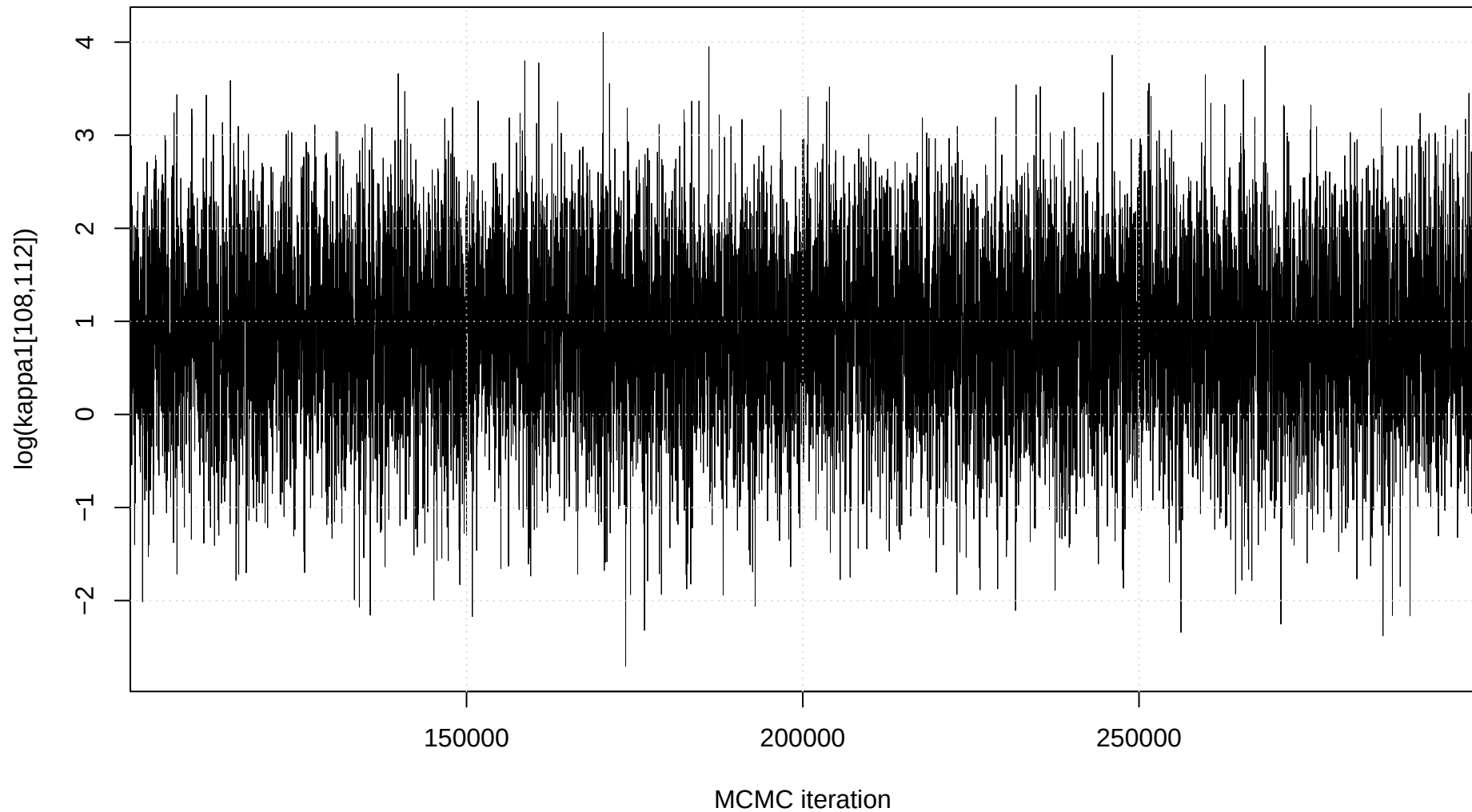
Trace plot: \log(\text{kappa1}[108,112])
