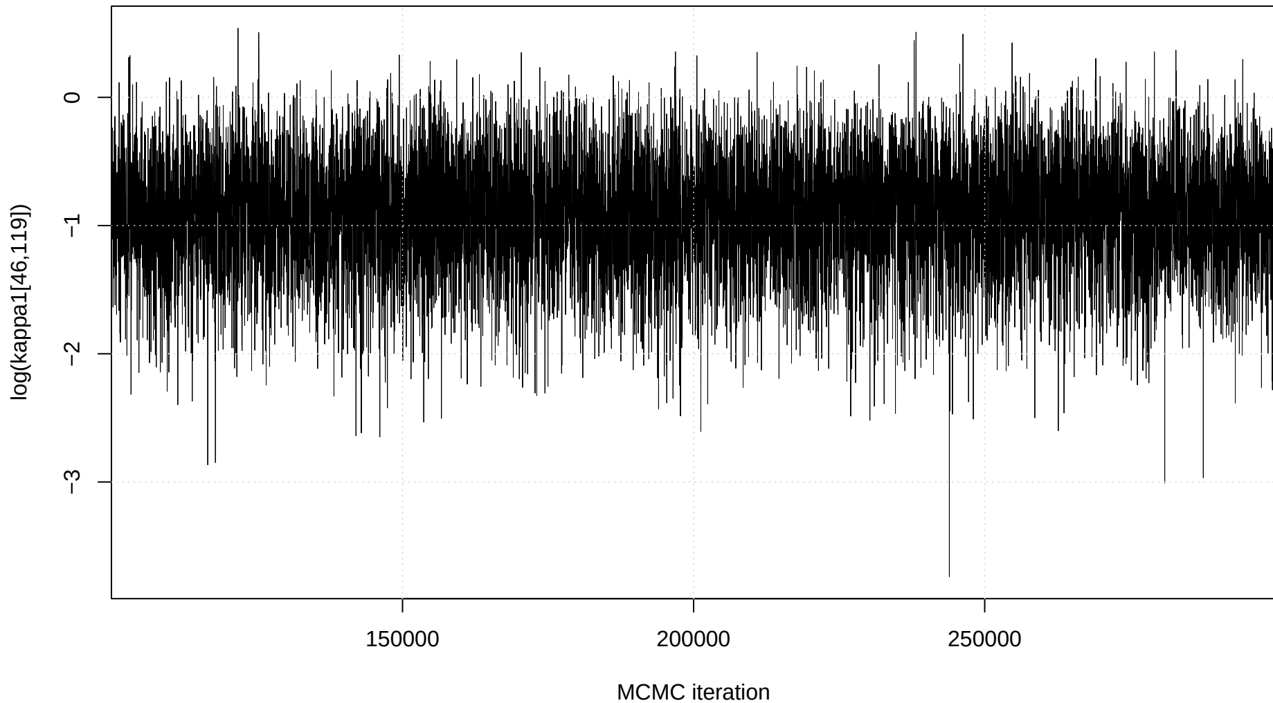
Trace plot: \log(\text{kappa1}[46,119])
