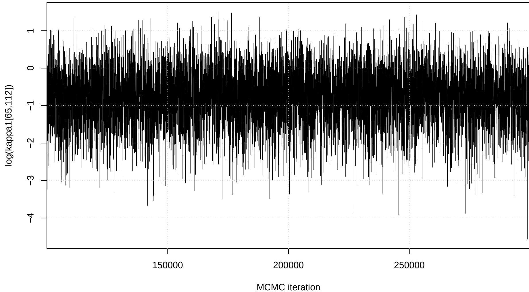
Trace plot: \log(\kappa_1[65,112])
