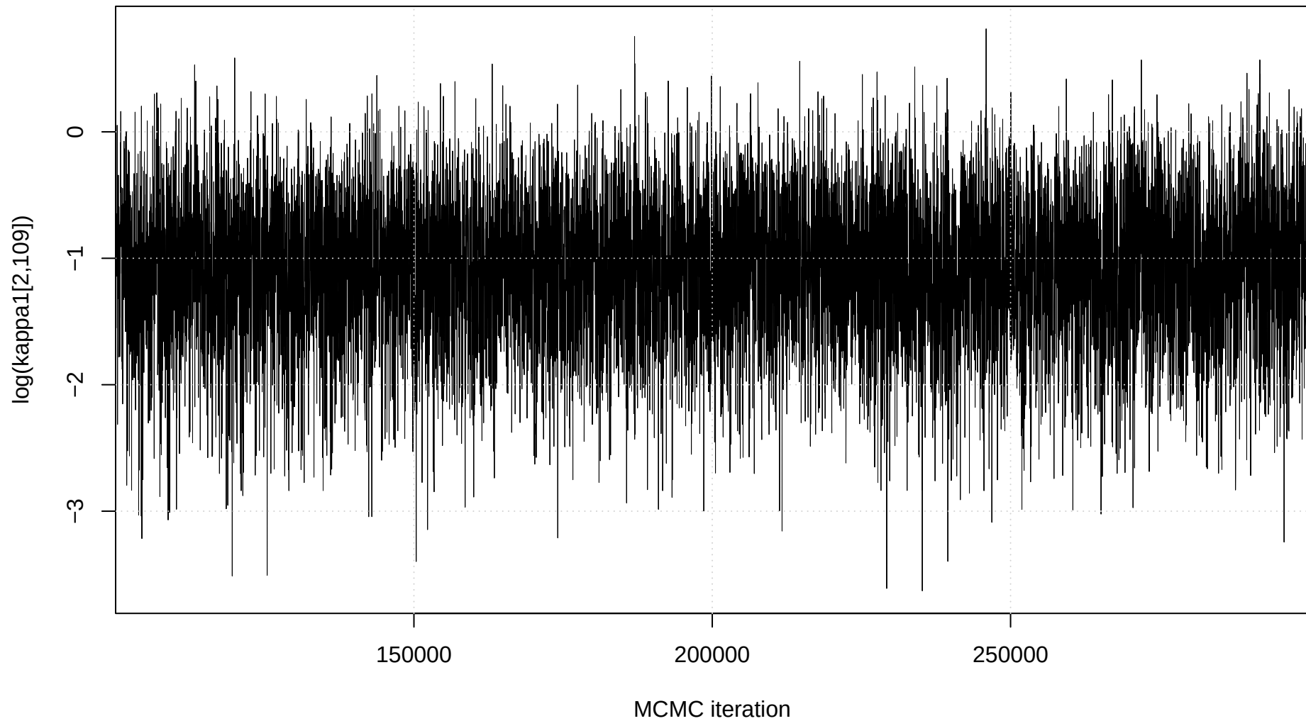
Trace plot: \log(\kappa_1[2,109])
