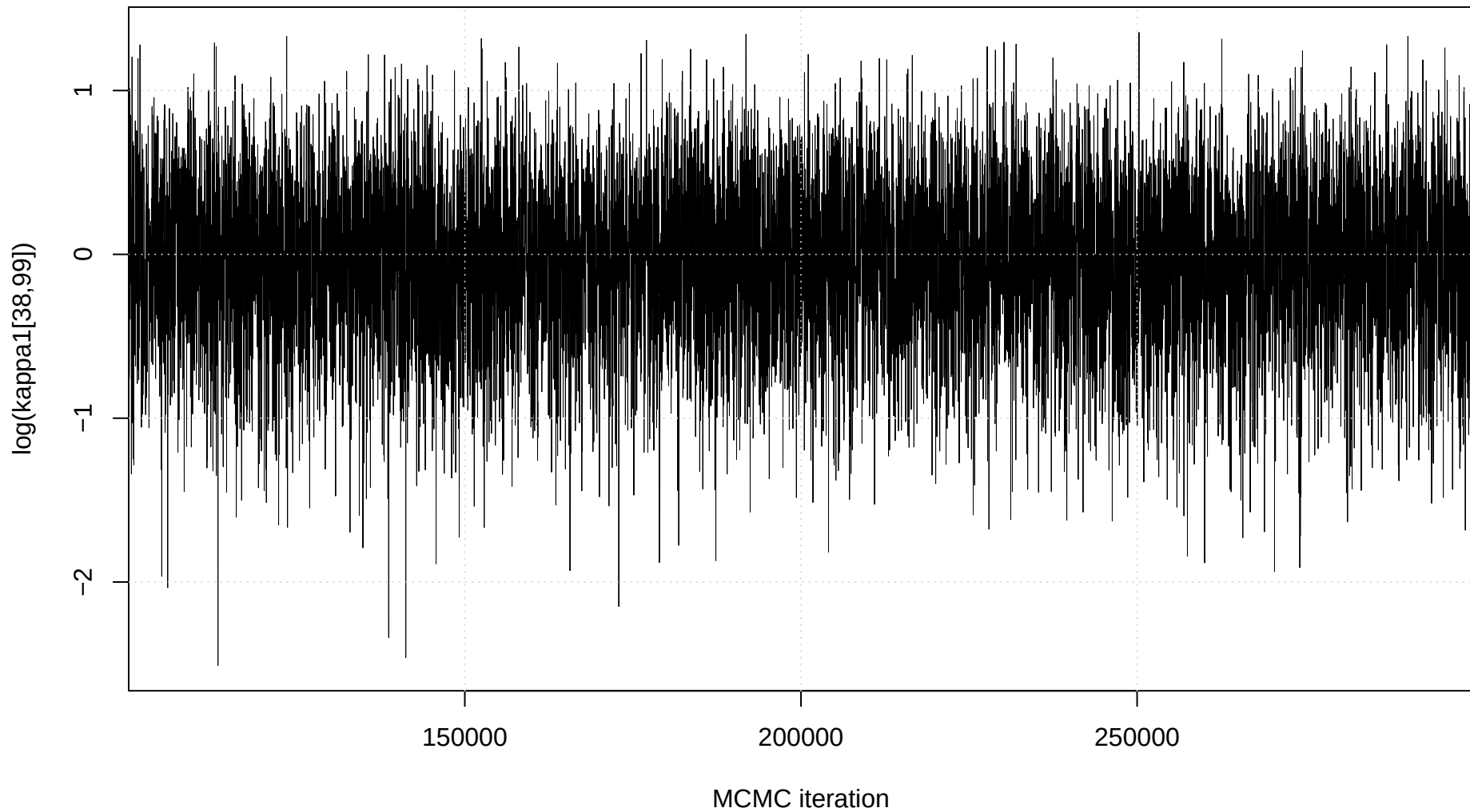
Trace plot: \log(\kappa_1[38,99])
