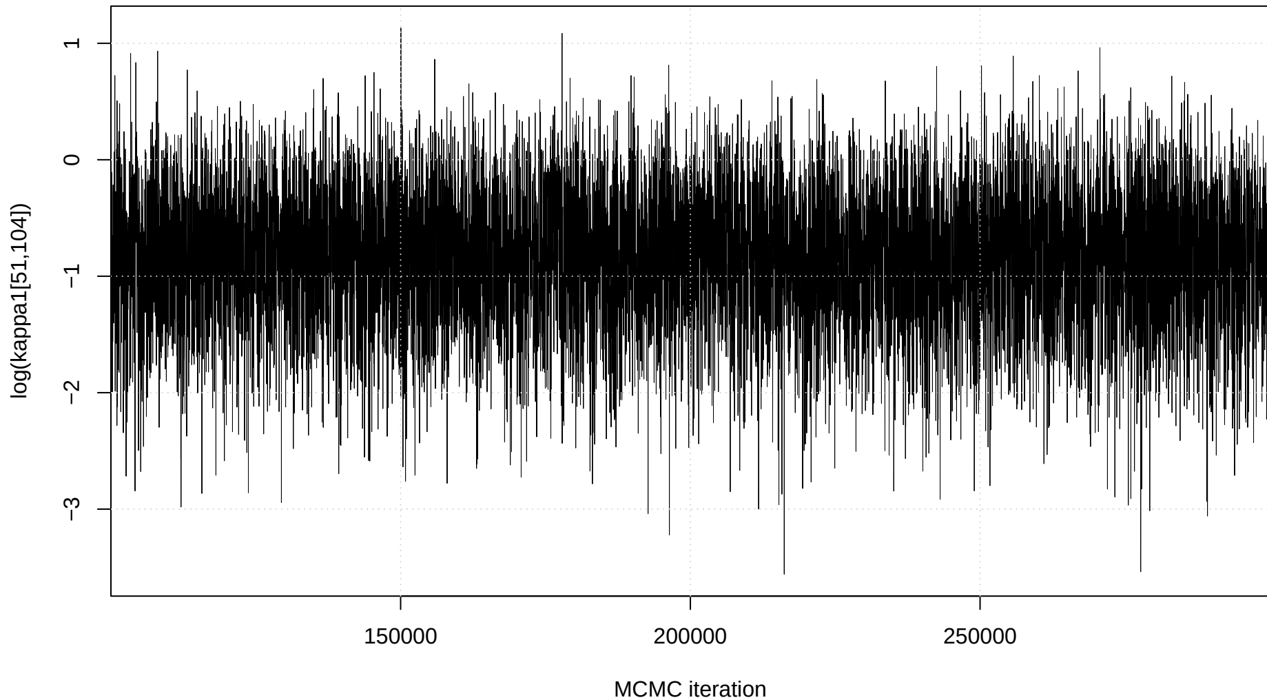
Trace plot: \log(\kappa_1[51,104])
