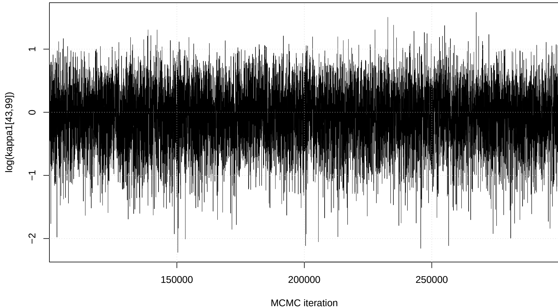
Trace plot: \log(\kappa_1[43,99])
