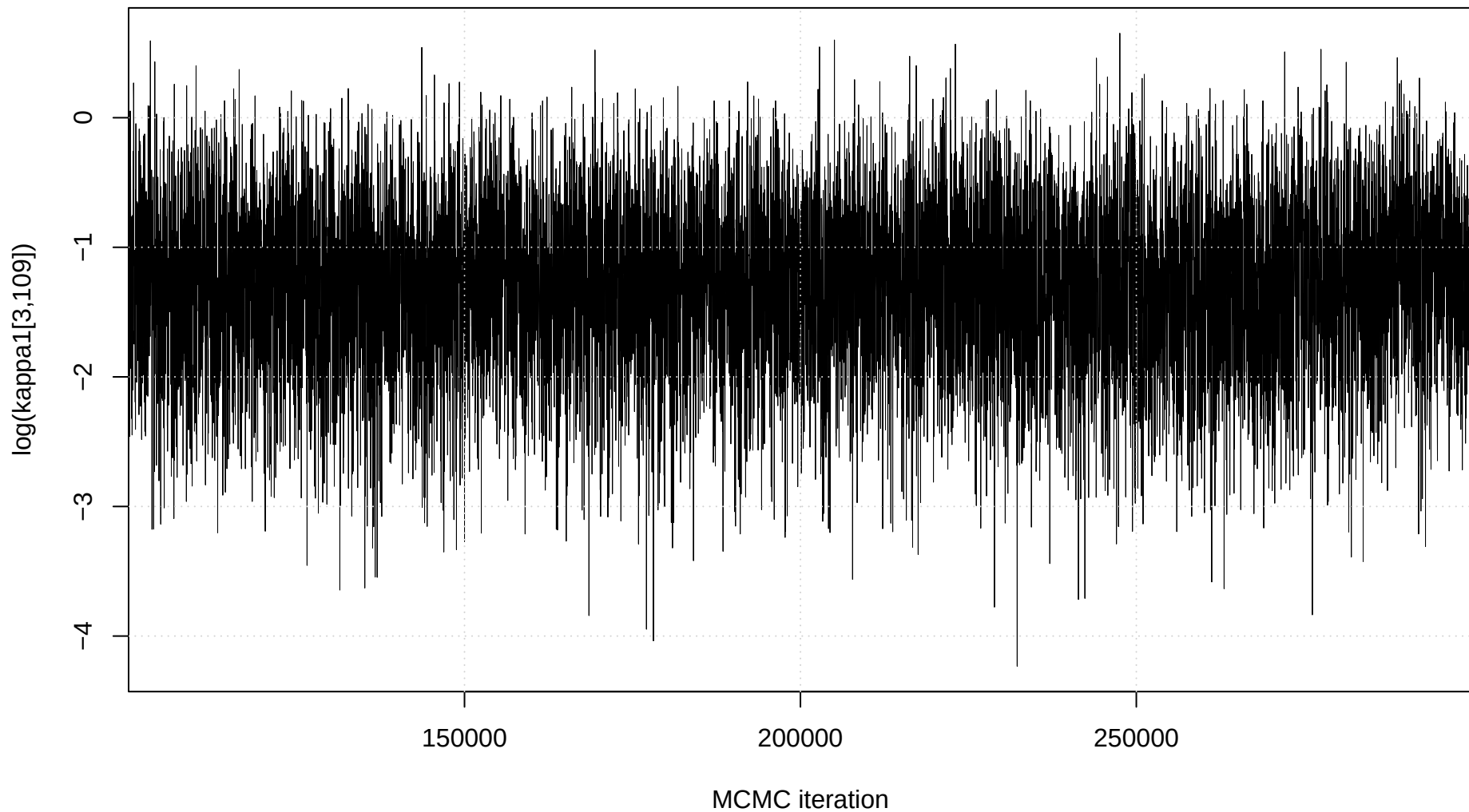
Trace plot: \log(\kappa_1[3,109])
