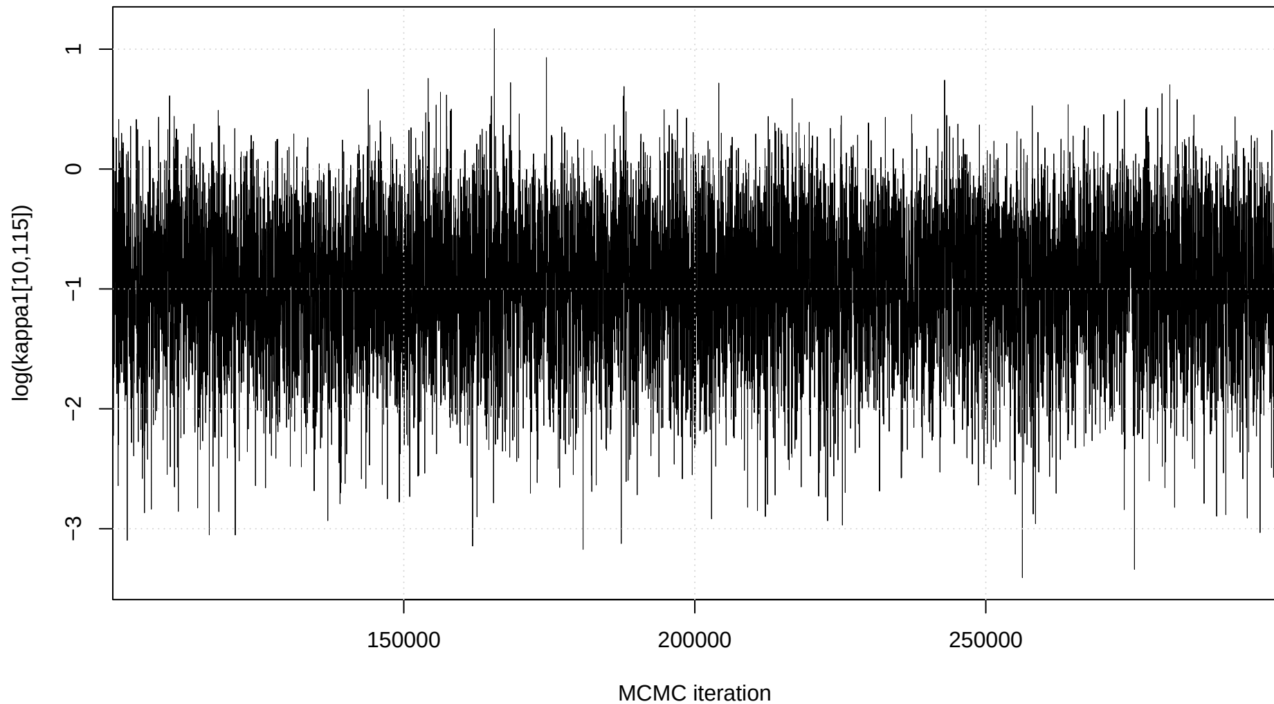
Trace plot: \log(\kappa_1[10,115])
