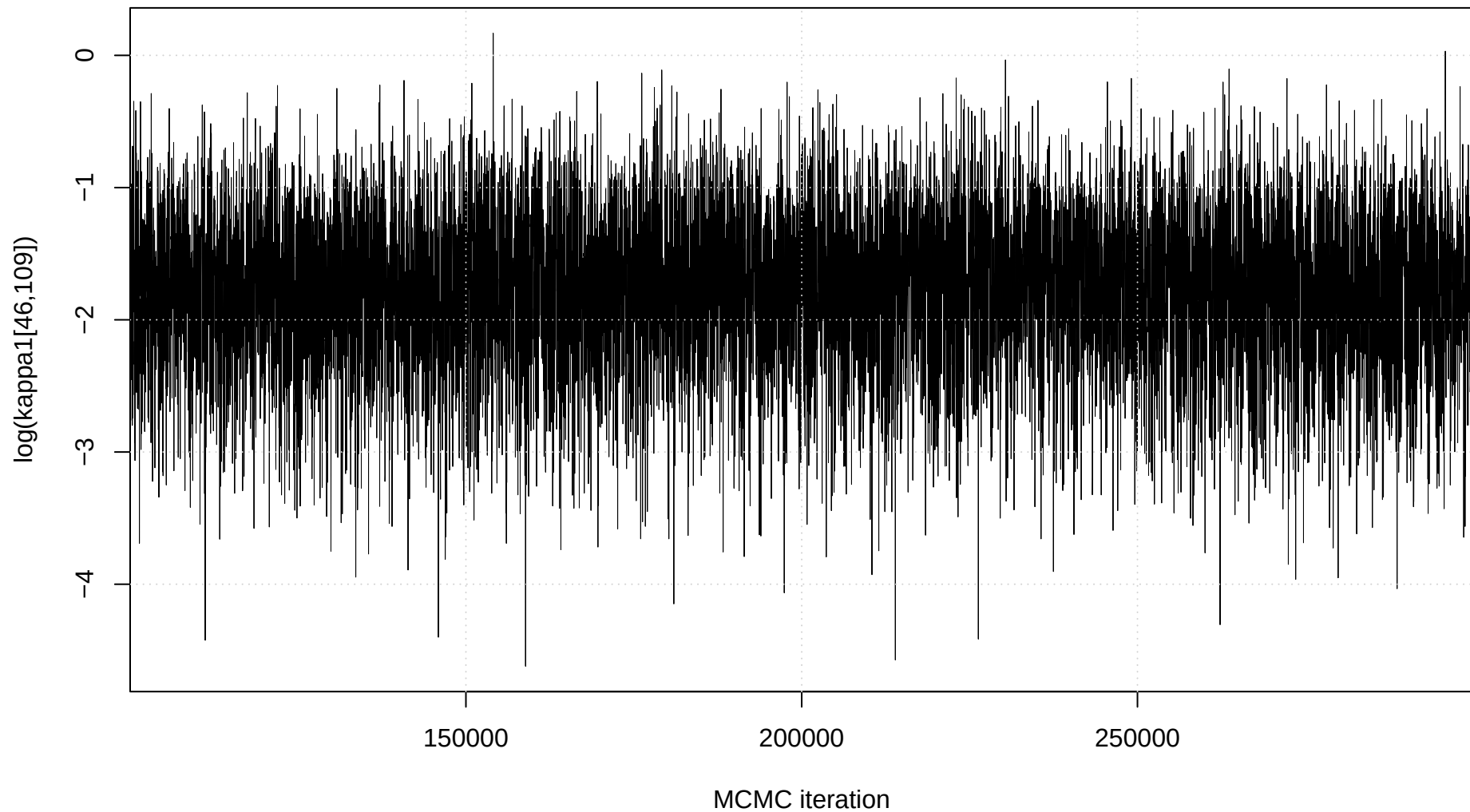
Trace plot: \log(\kappa_1[46,109])
