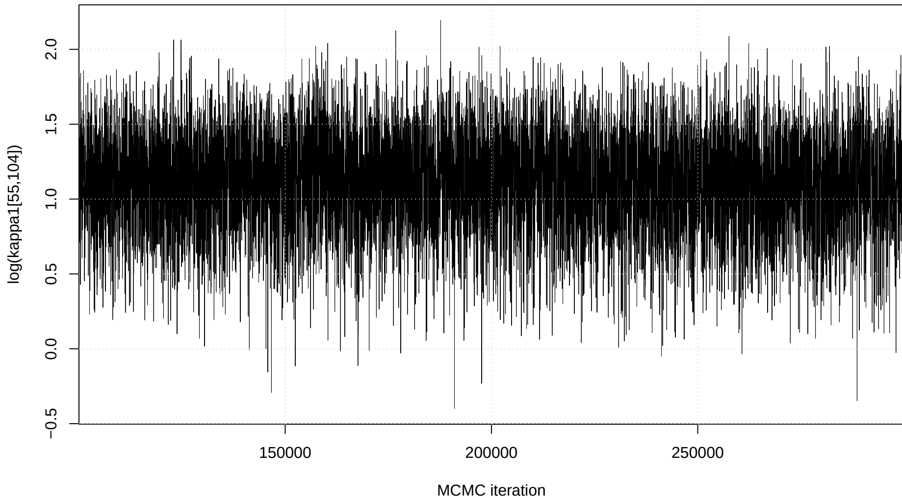
Trace plot: \log(\kappa_1[55,104])
