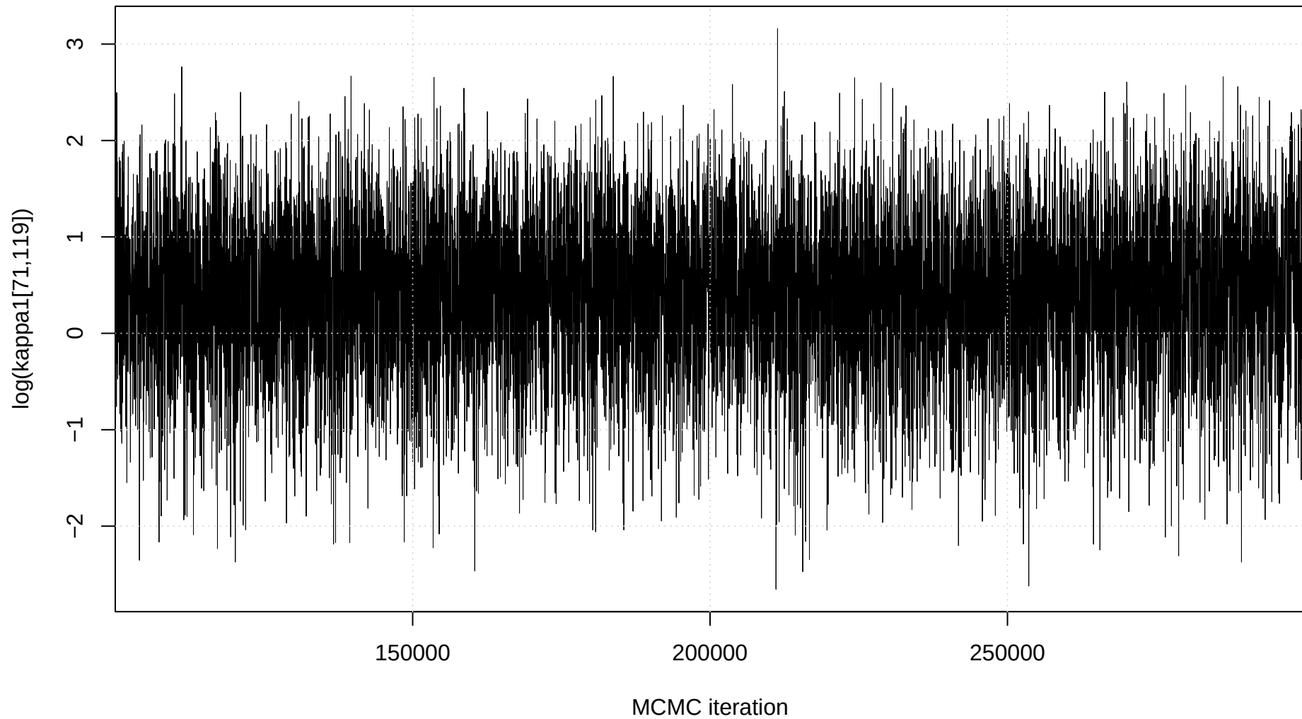
Trace plot: \log(\kappa_1[71,119])
