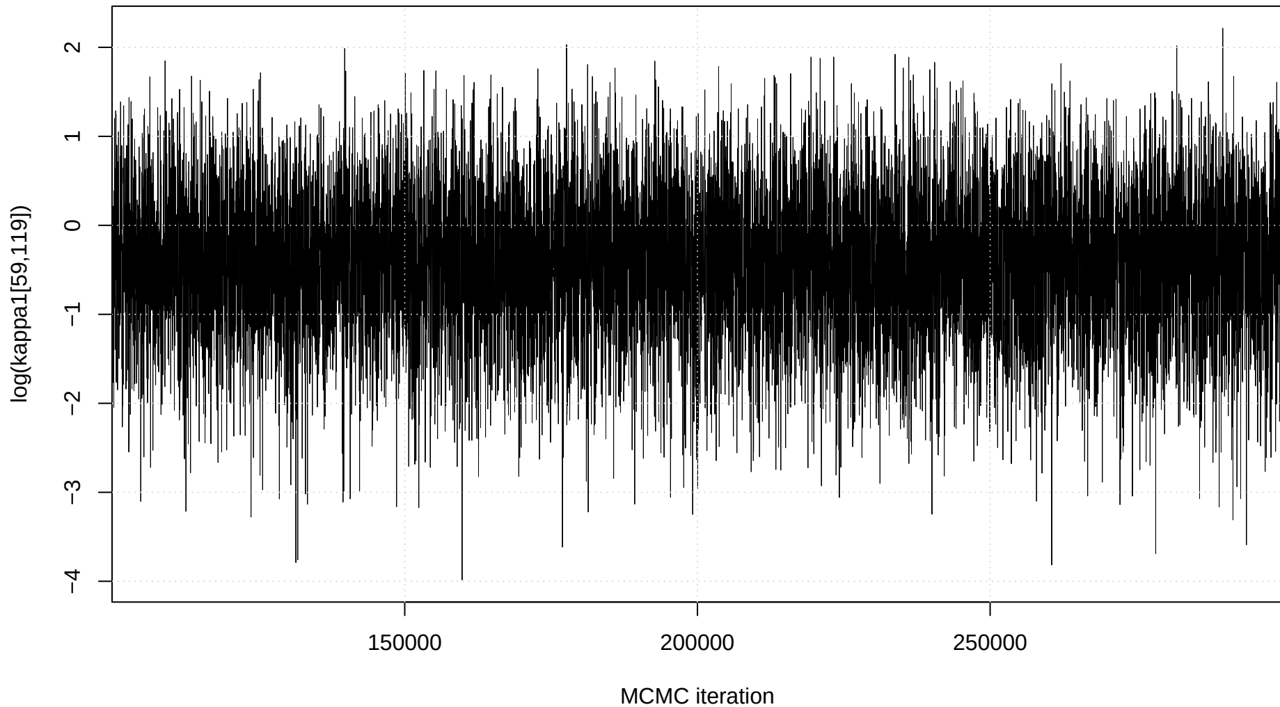
Trace plot: \log(\kappa_1[59,119])
