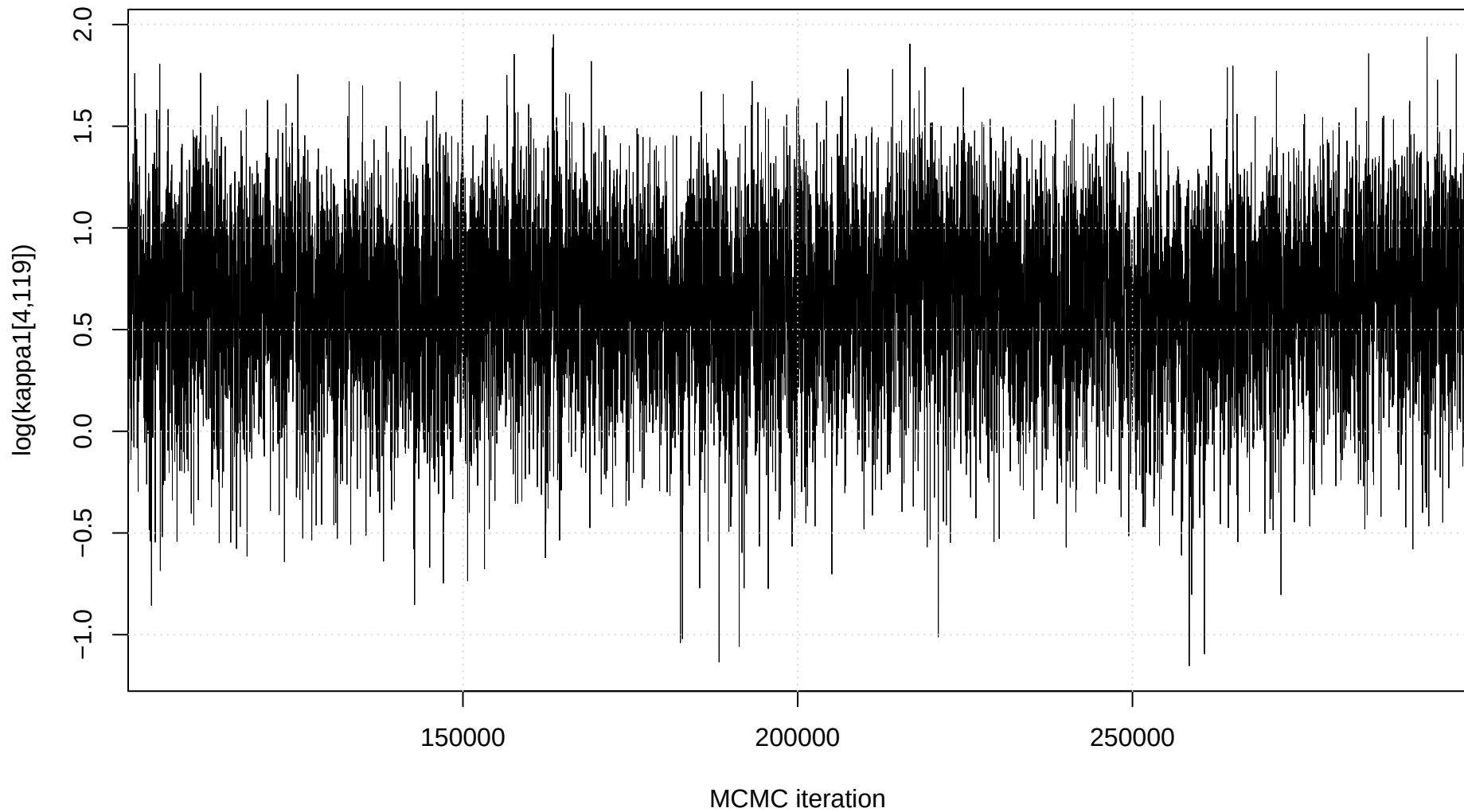
Trace plot: \log(\kappa_1[4,119])
