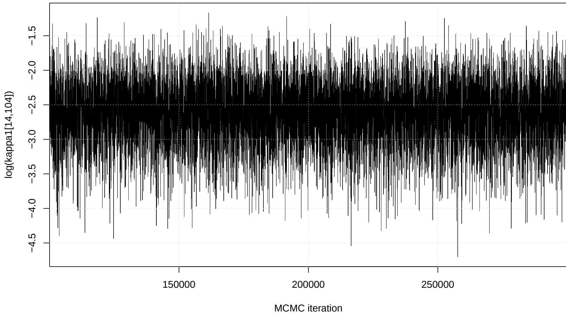
Trace plot: \log(\kappa_1[14,104])
