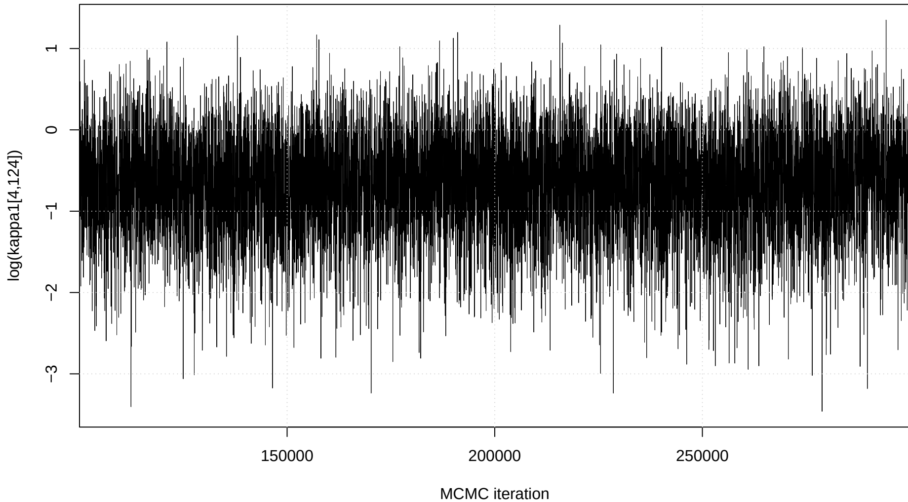
Trace plot: \log(\kappa_1[4,124])
