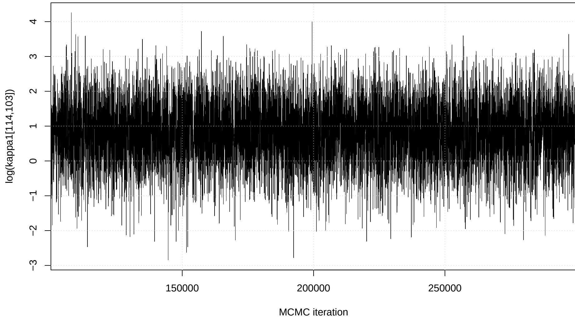
Trace plot: \log(\kappa_{114,103})
