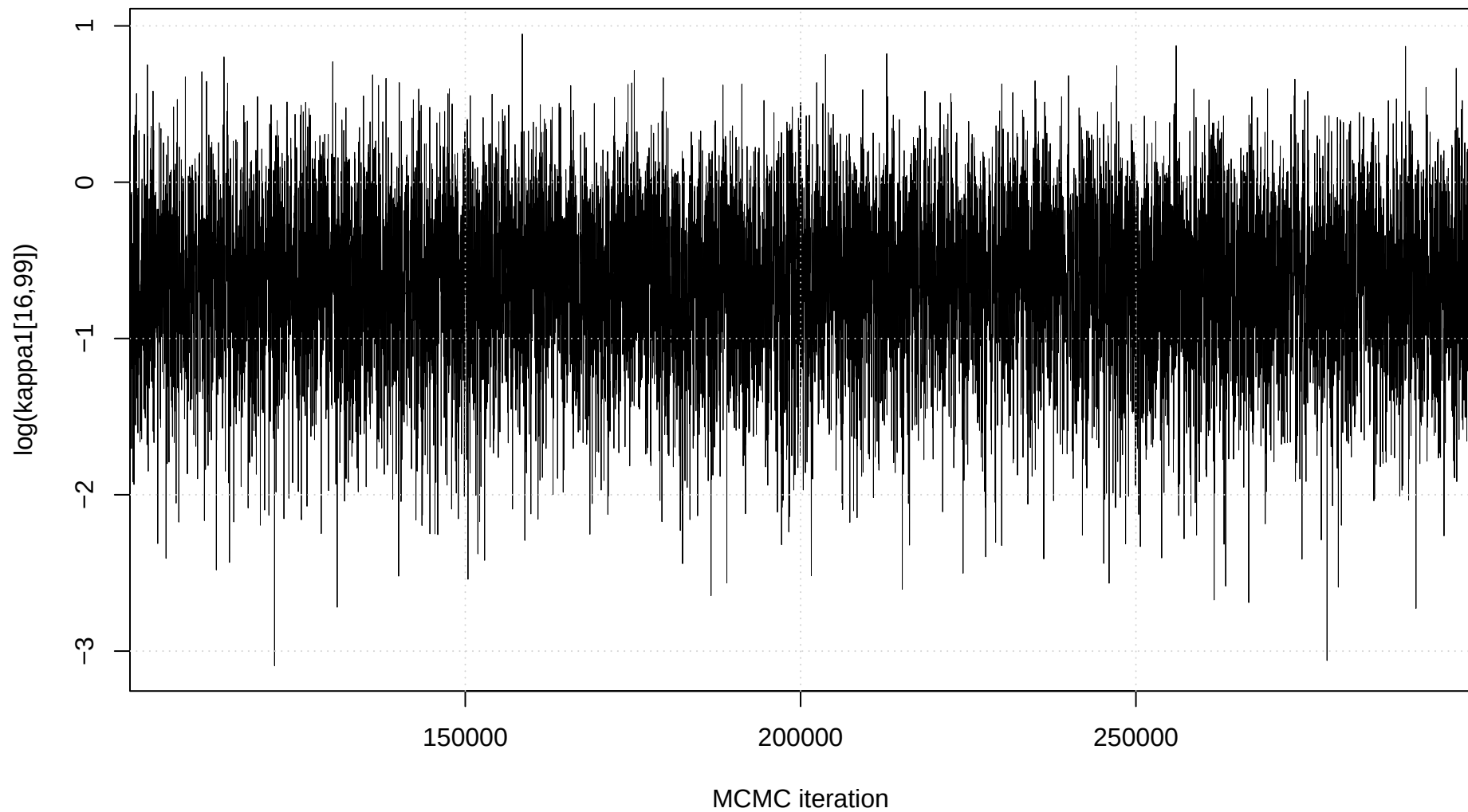
Trace plot: \log(\kappa_1[16,99])
