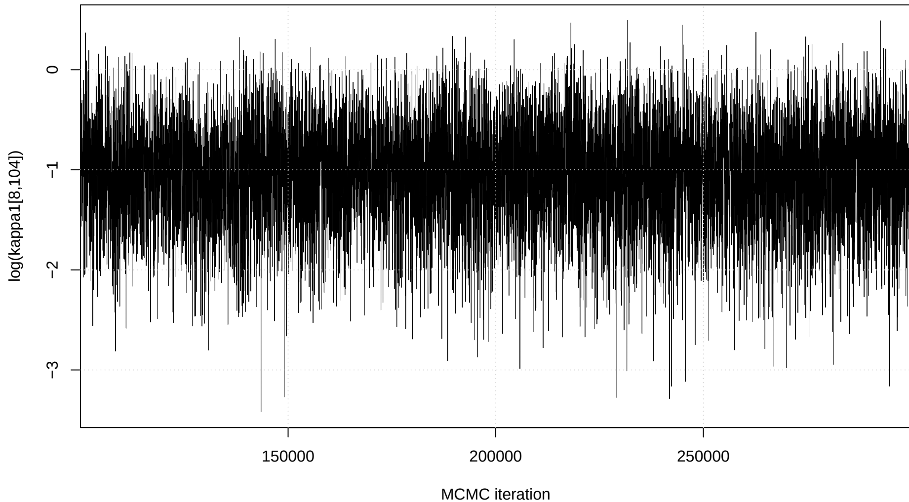
Trace plot: \log(\kappa_1[8,104])
