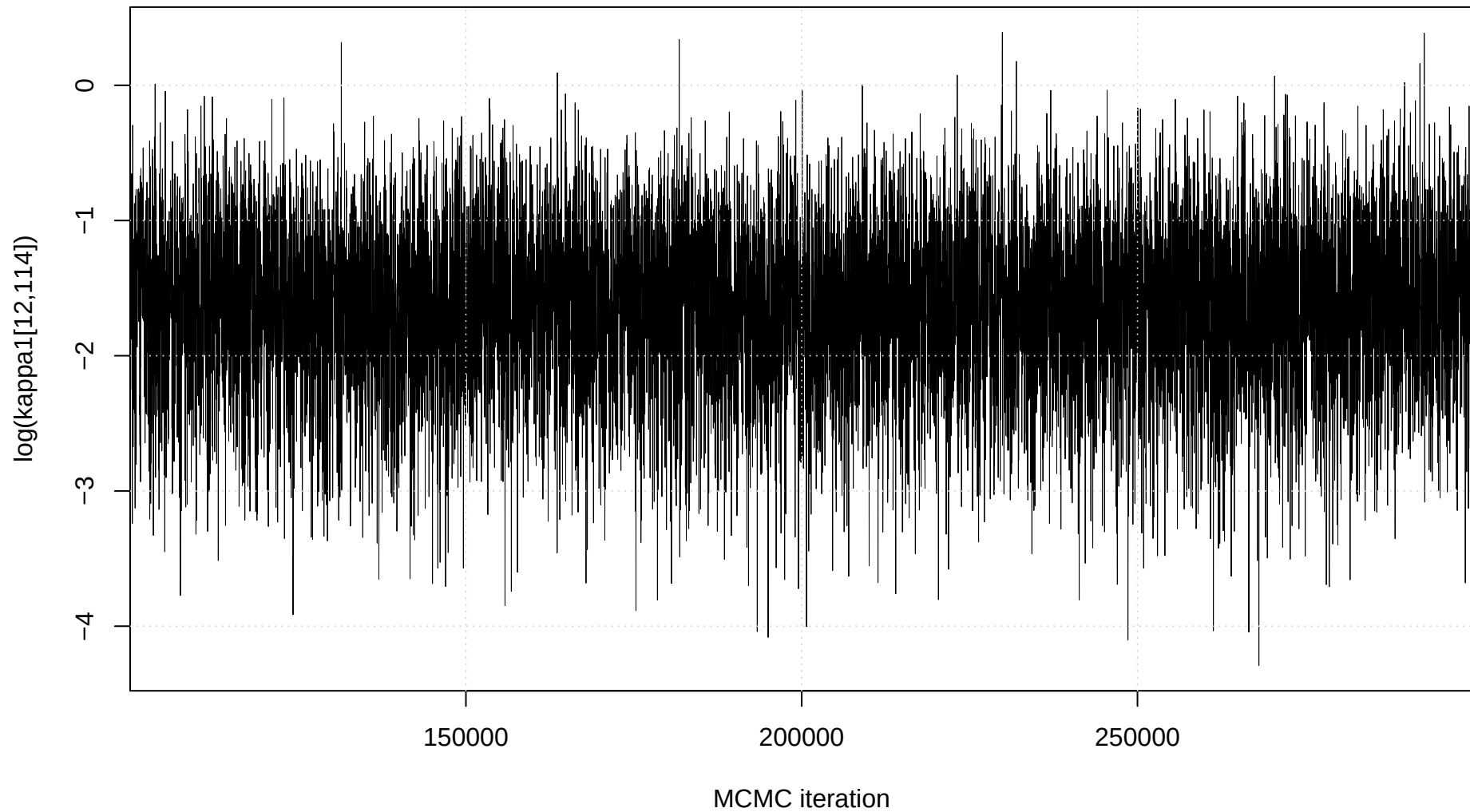
Trace plot: \log(\kappa_1[12,114])
