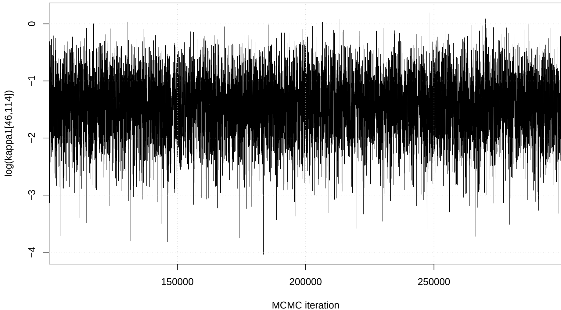
Trace plot: \log(\kappa_1[46,114])
