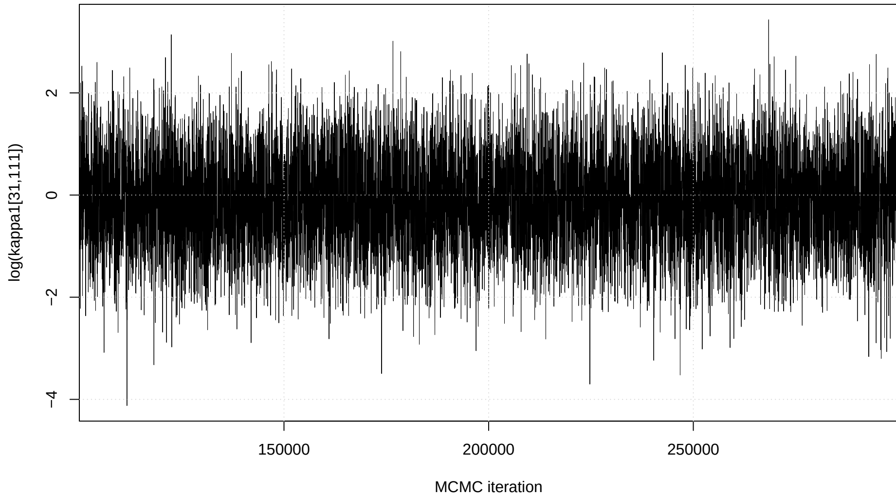
Trace plot: \log(\kappa_1[31,111])
