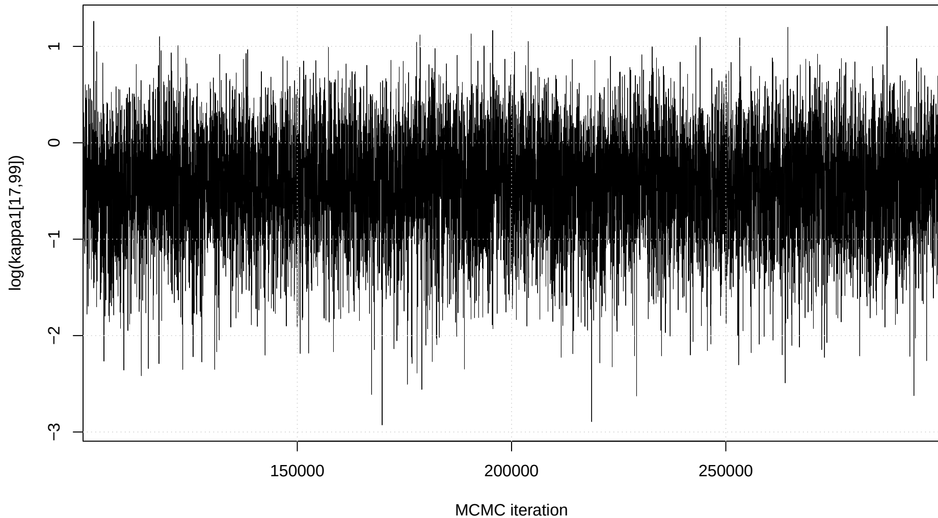
Trace plot: \log(\kappa_{1[17,99]})
