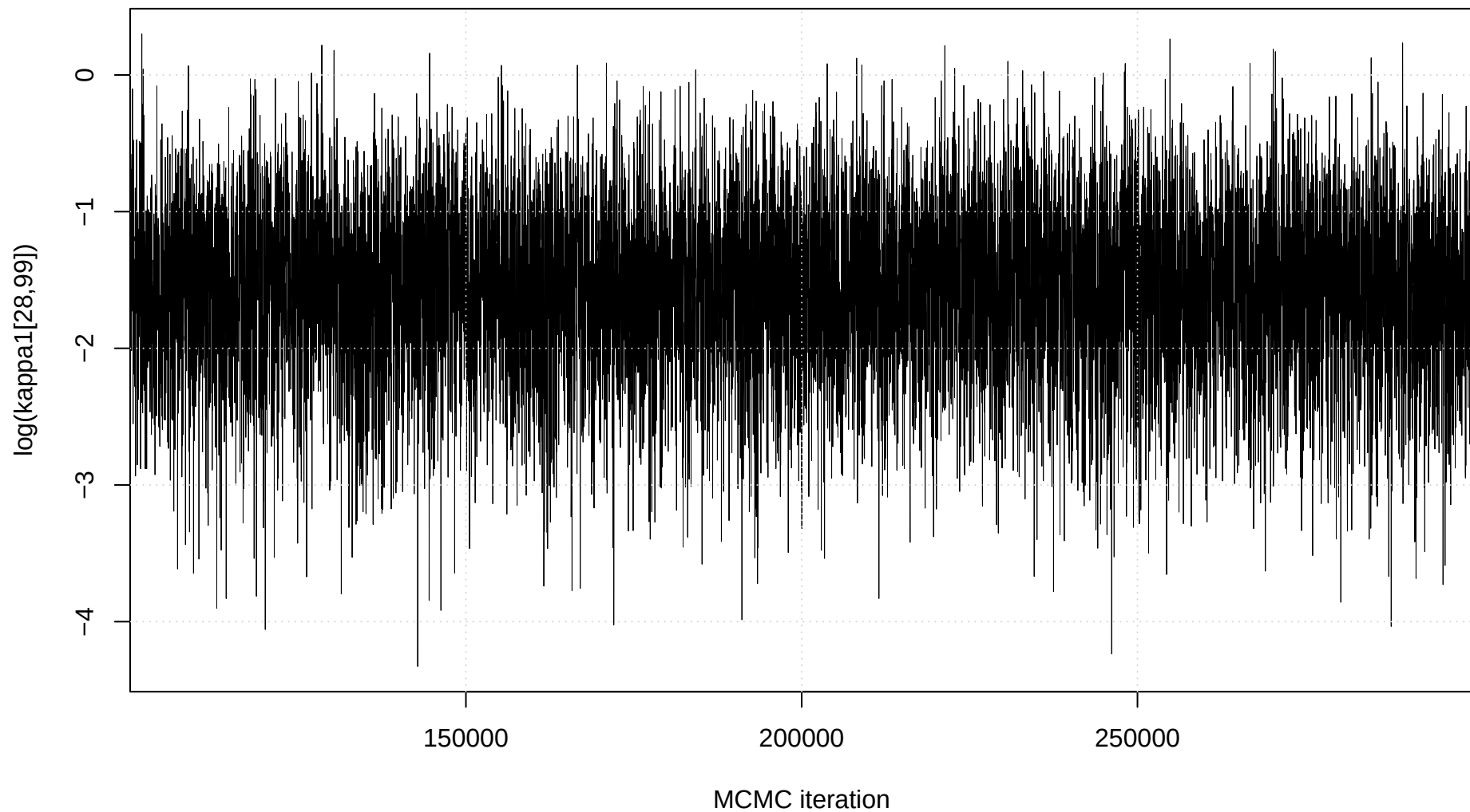
Trace plot: \log(\kappa_1[28,99])
