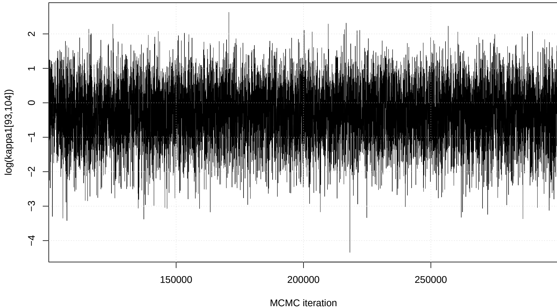
Trace plot: \log(\kappa_1[93,104])
