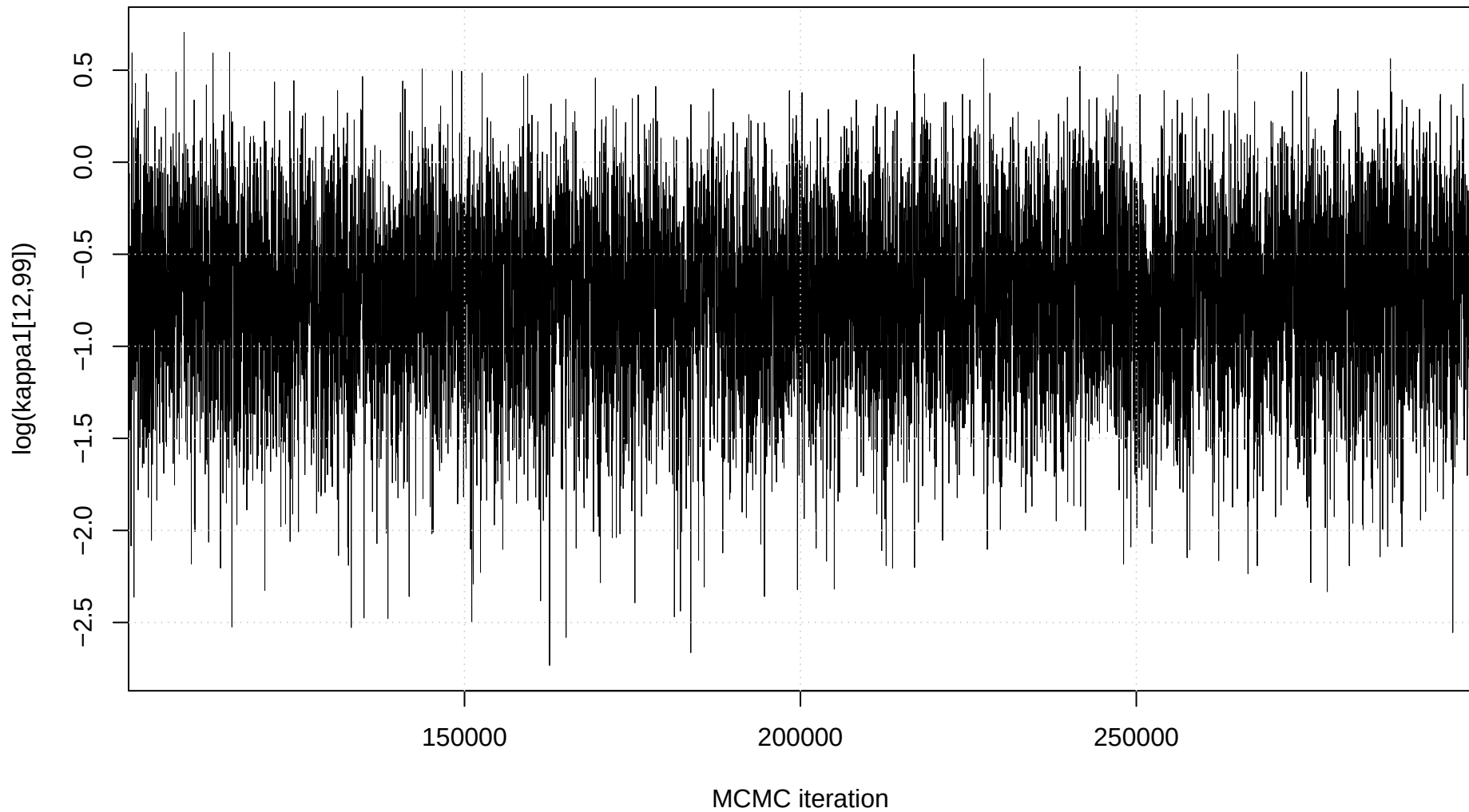
Trace plot: \log(\kappa_1[12,99])
