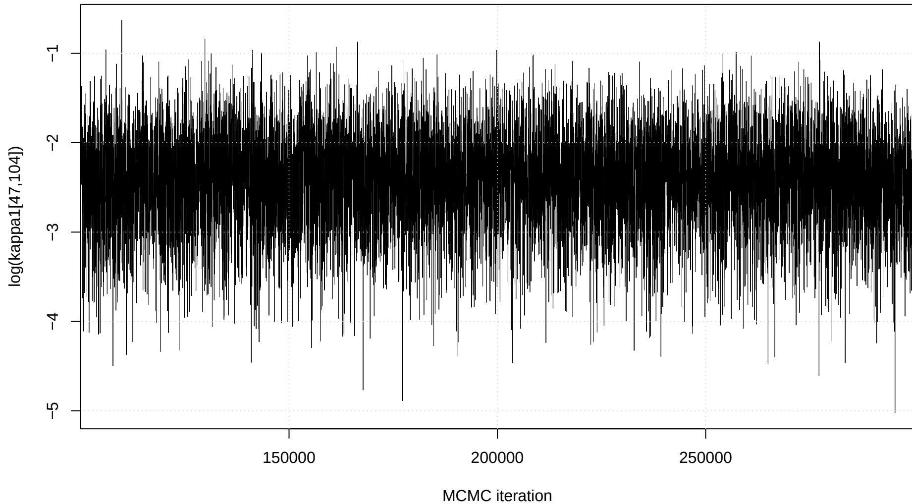
Trace plot: \log(\kappa_1[47,104])
