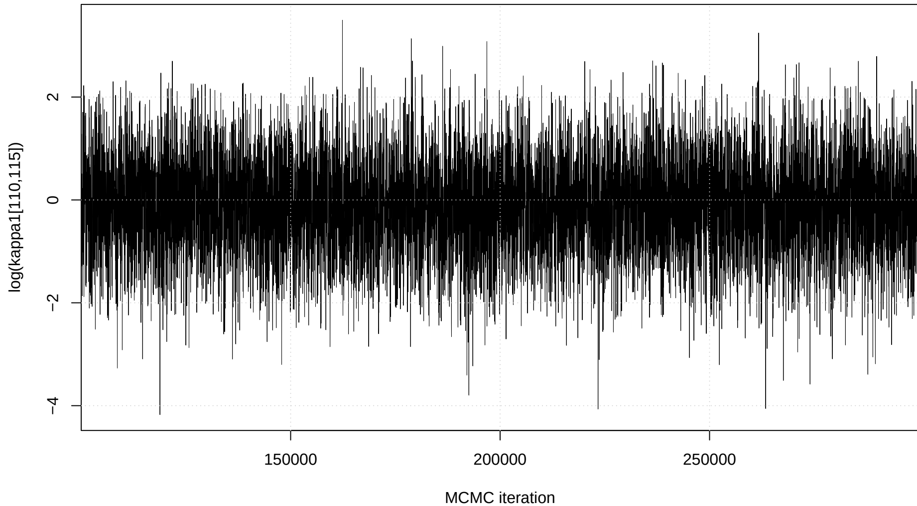
Trace plot: \log(\kappa_1[110,115])
