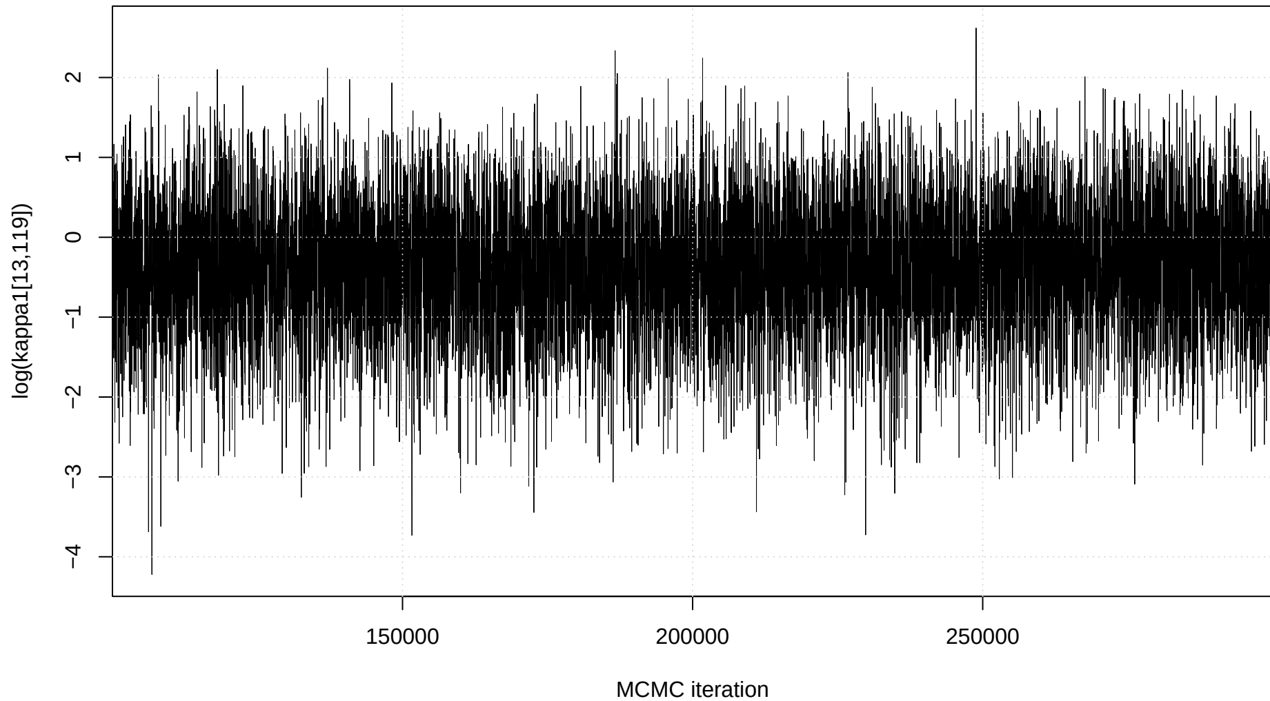
Trace plot: \log(\kappa_1[13,119])
