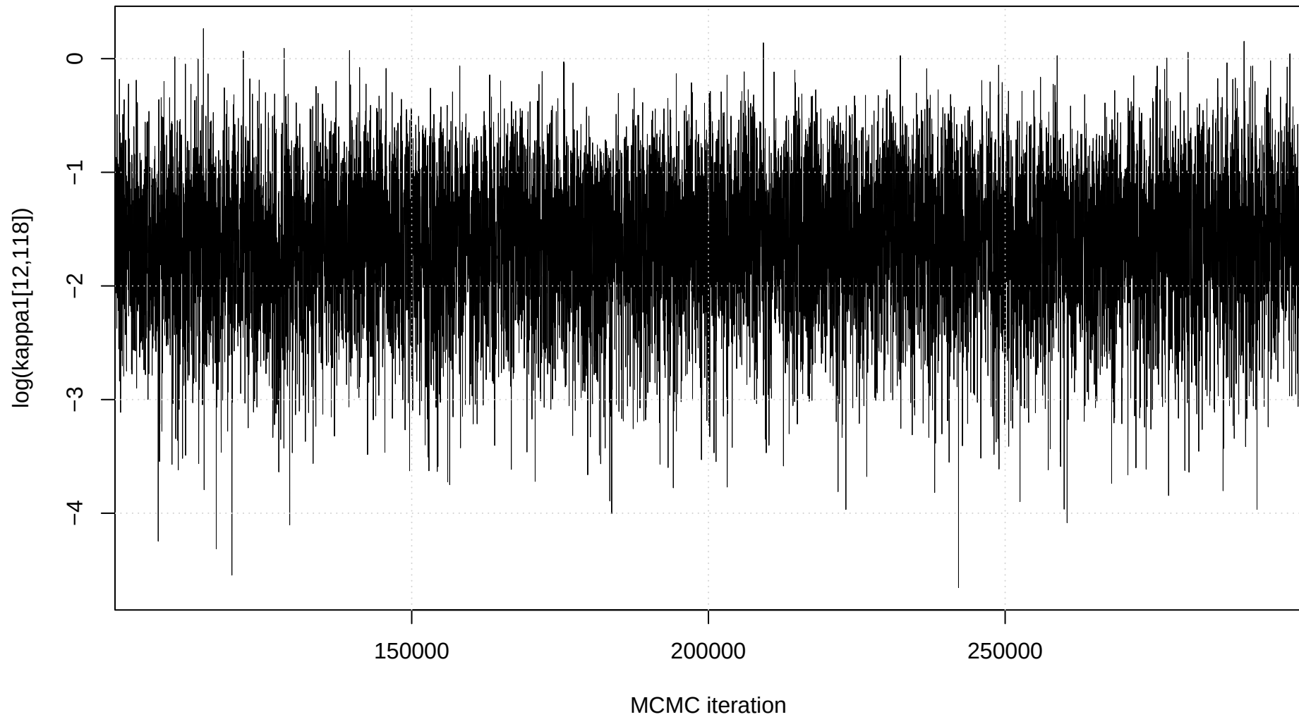
Trace plot: \log(\text{kappa1}[12,118])
