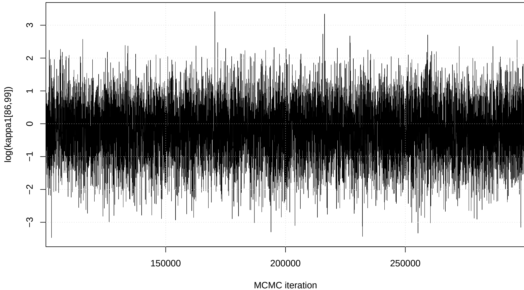
Trace plot: \log(\kappa_1[86,99])
