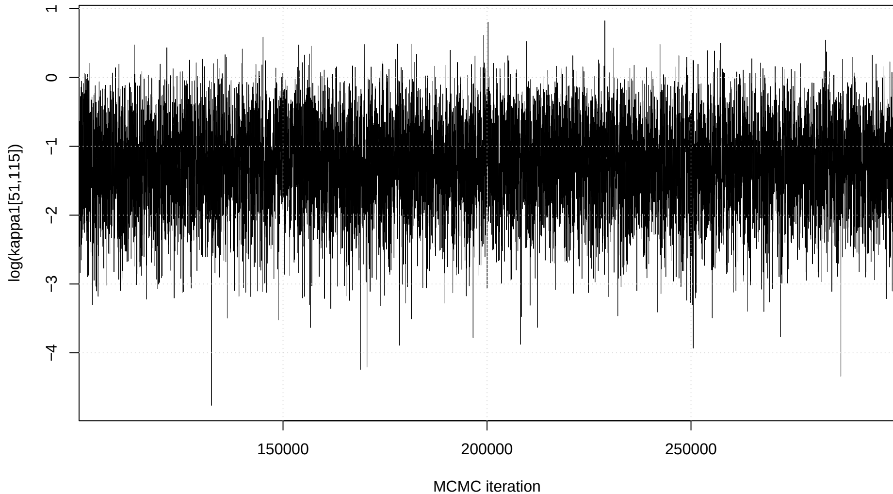
Trace plot: \log(\kappa_1[51,115])
