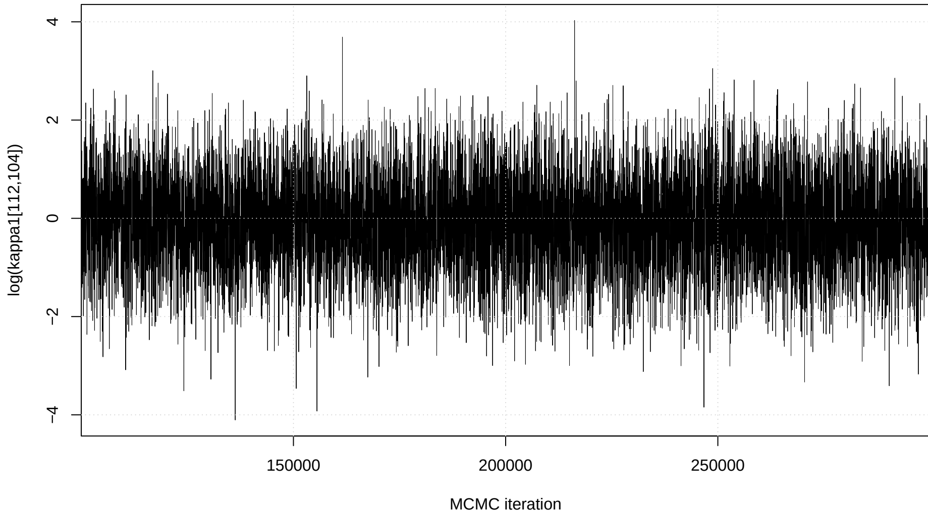
Trace plot: \log(\kappa_1[112,104])
