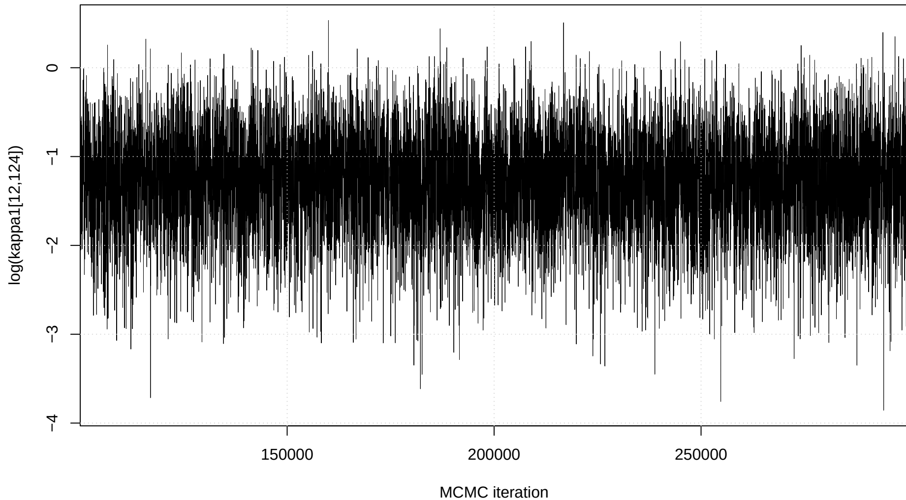
Trace plot: \log(\kappa_1[12,124])
