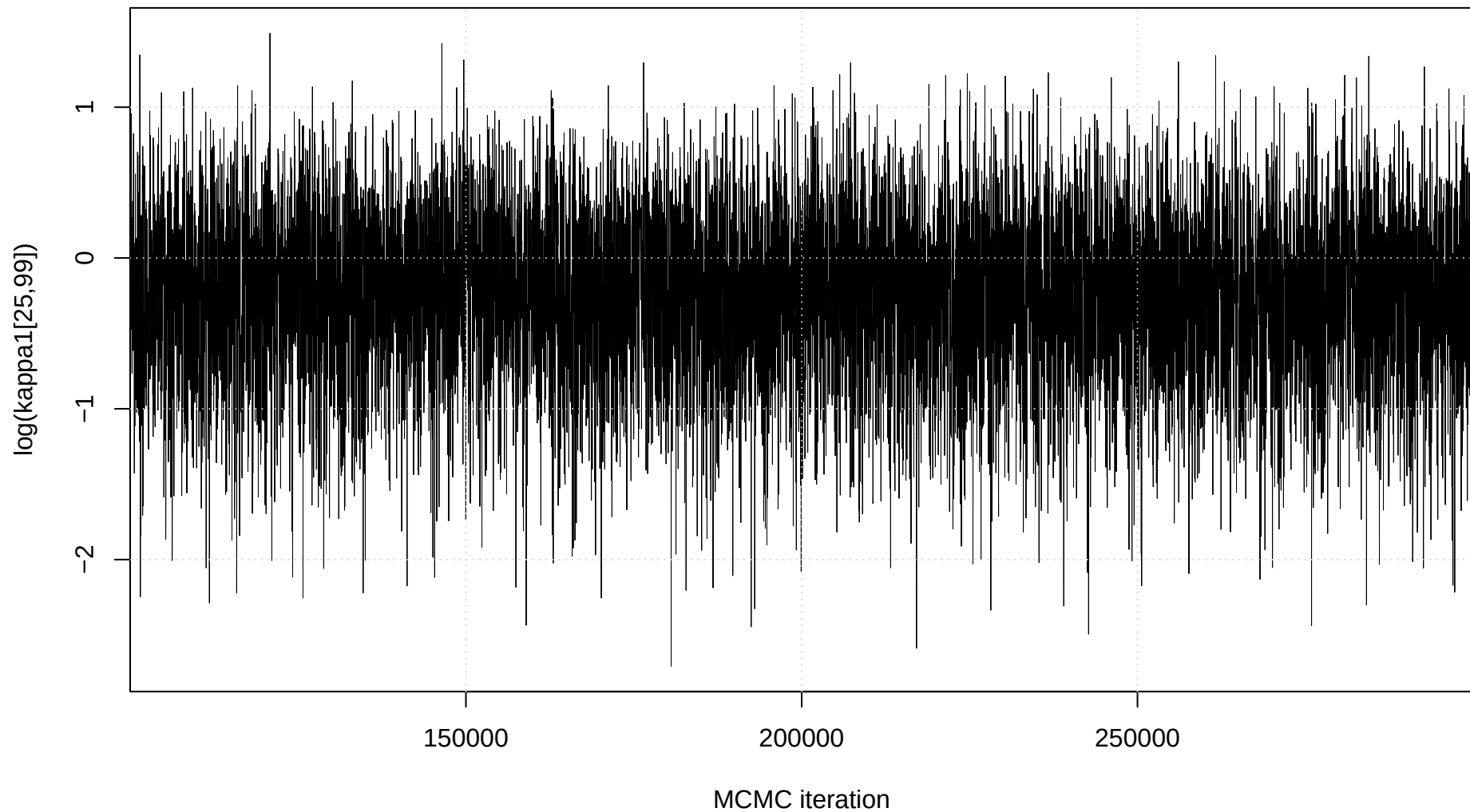
Trace plot: \log(\kappa_1[25,99])
