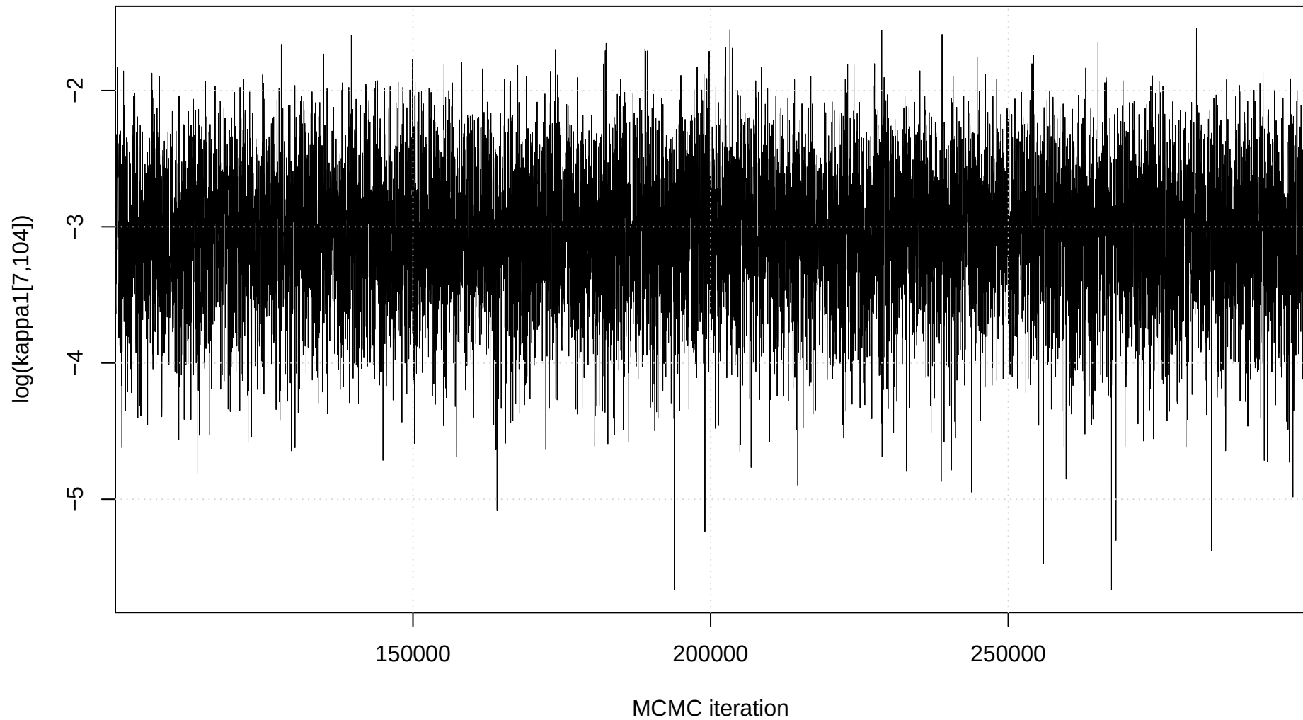
Trace plot: \log(\kappa_1[7,104])
