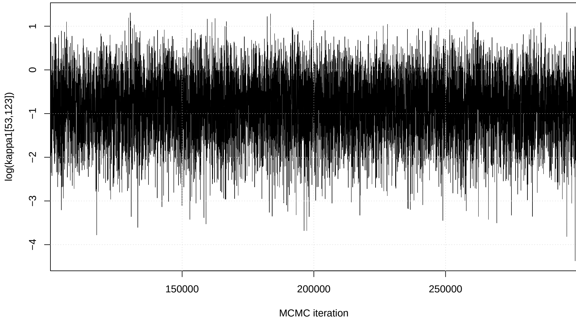
Trace plot: \log(\kappa_1[53,123])
