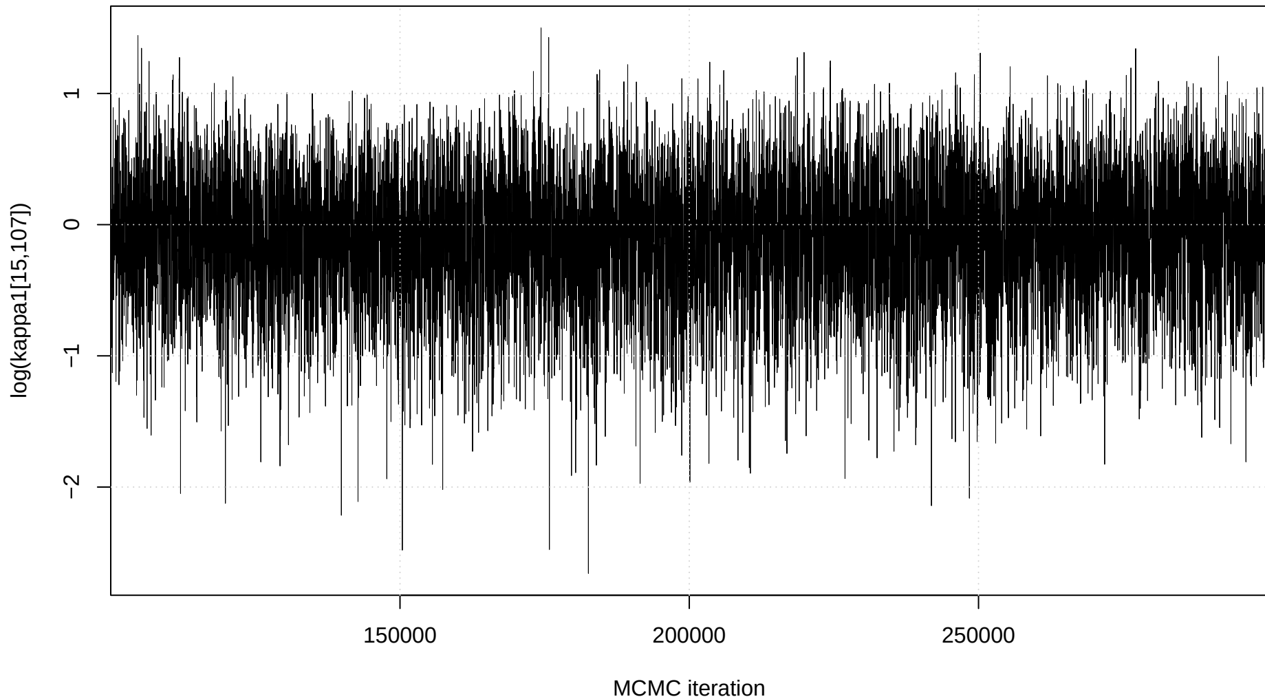
Trace plot: \log(\text{kappa1}[15,107])
