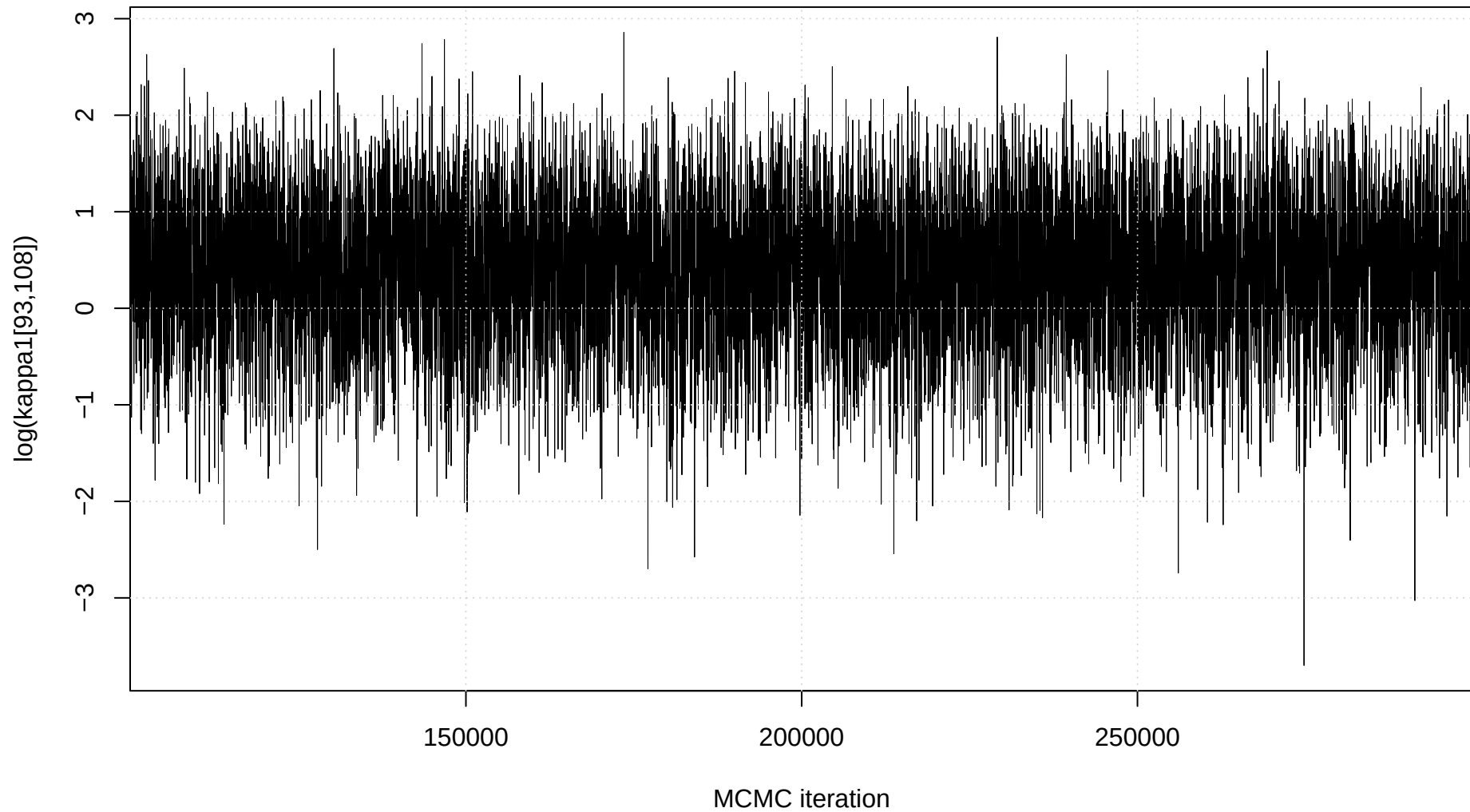
Trace plot: \log(\kappa_1[93,108])
