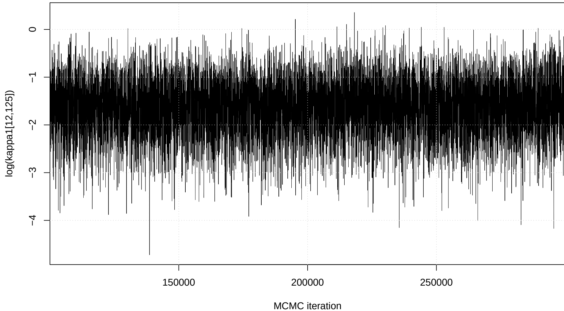
Trace plot: \log(\kappa_1[12,125])
