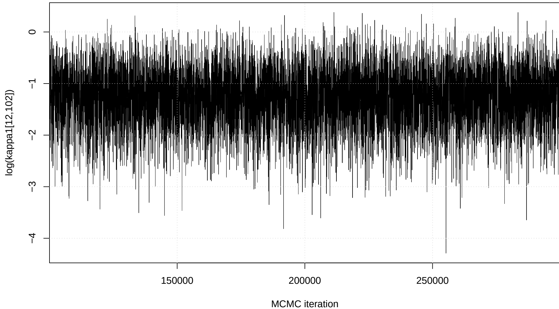
Trace plot: \log(\kappa_1[12,102])
