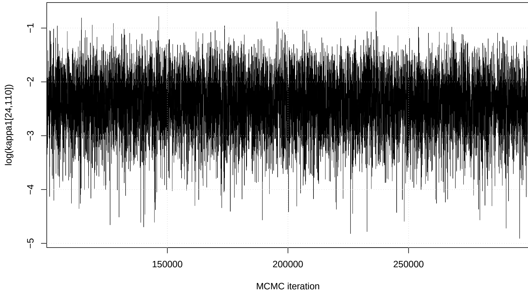
Trace plot: \log(\kappa_1[24,110])
