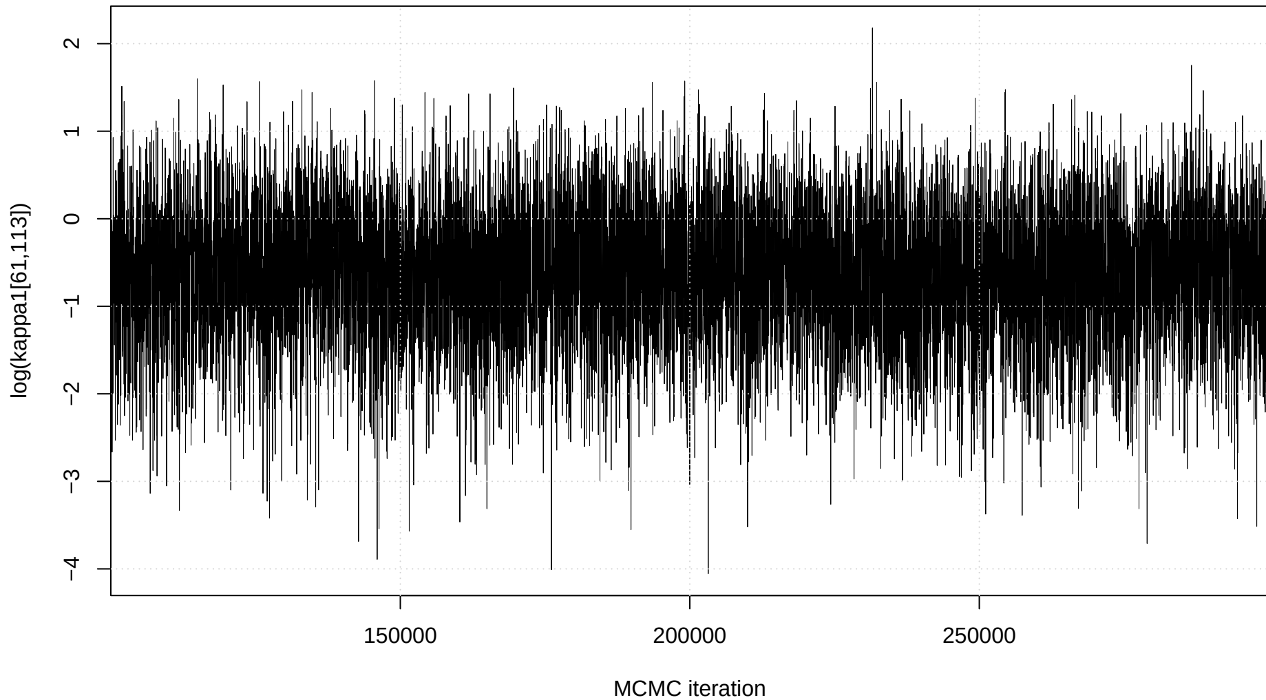
Trace plot: \log(\kappa_1[61,113])
