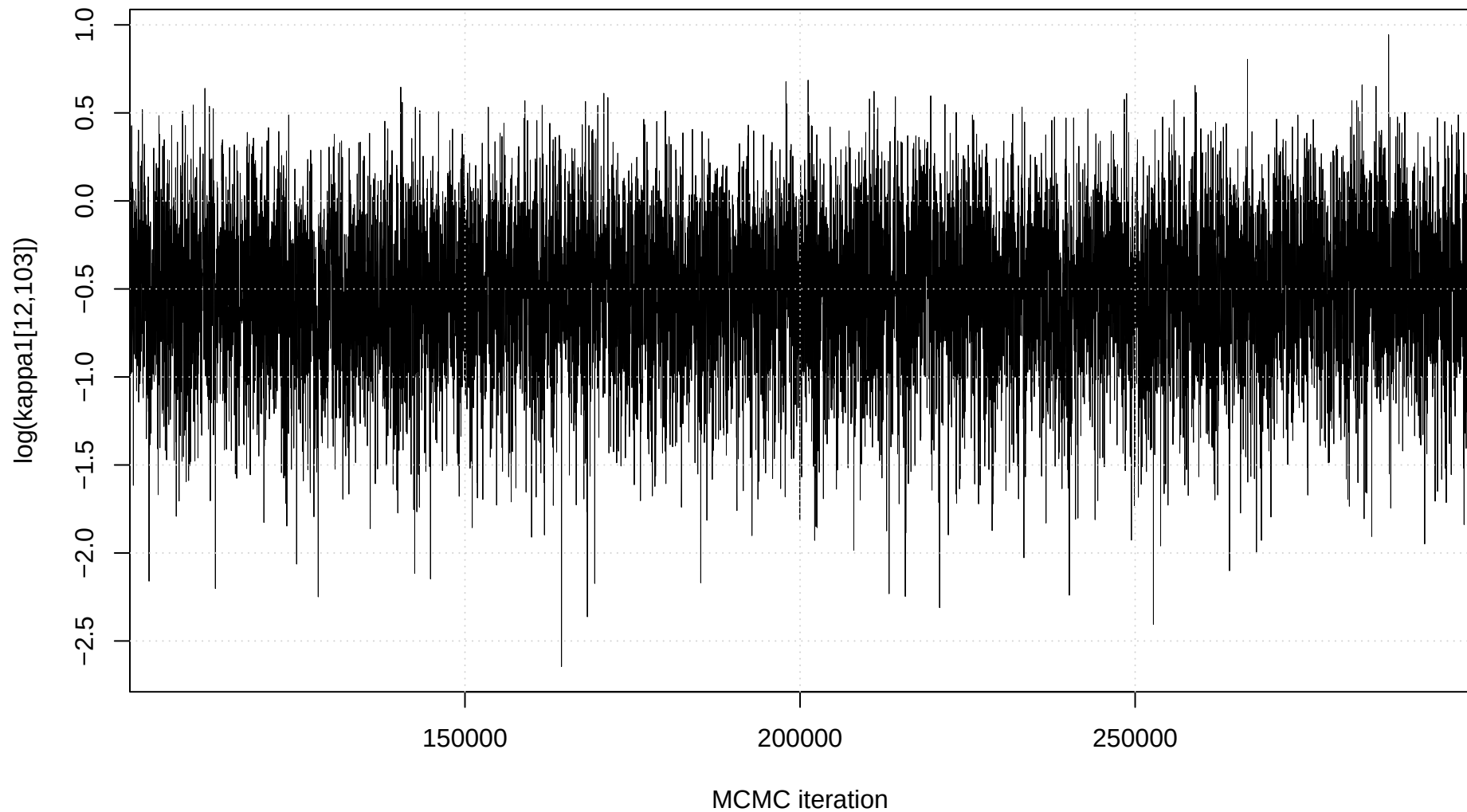
Trace plot: \log(\kappa_1[12,103])
