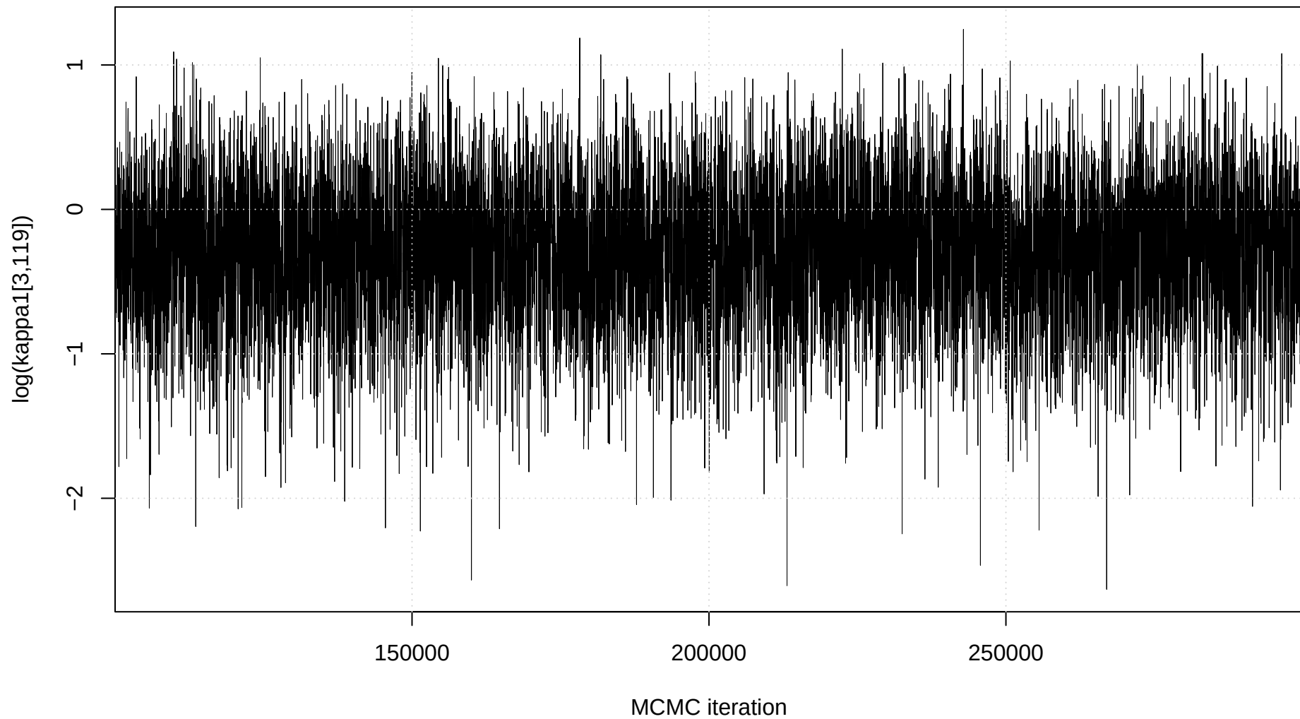
Trace plot: \log(\kappa_1[3,119])
