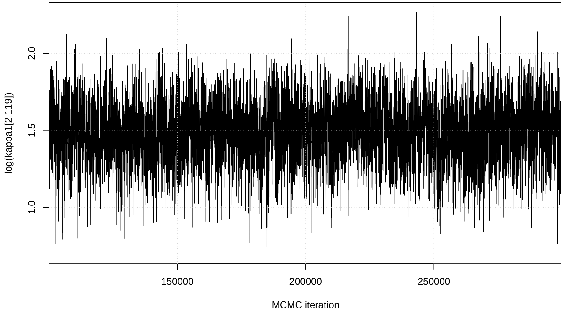
Trace plot: \log(\kappa_1[2,119])
