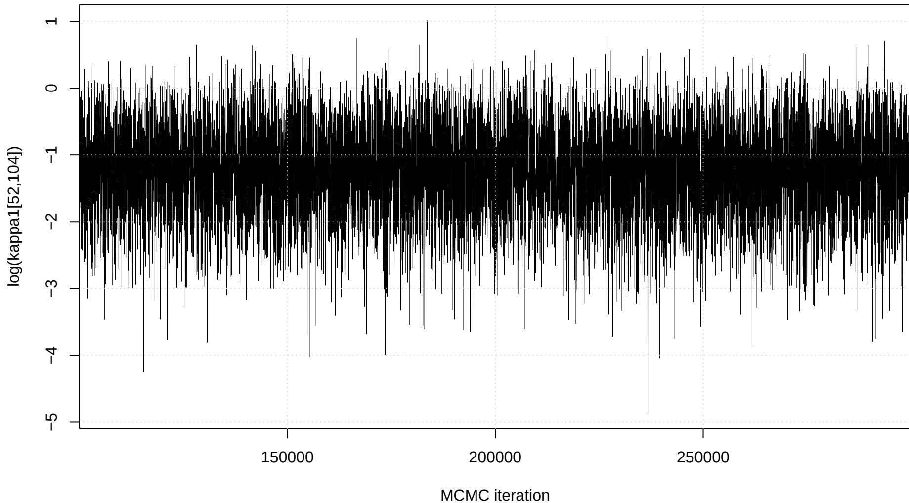
Trace plot: \log(\text{kappa1}[52,104])
