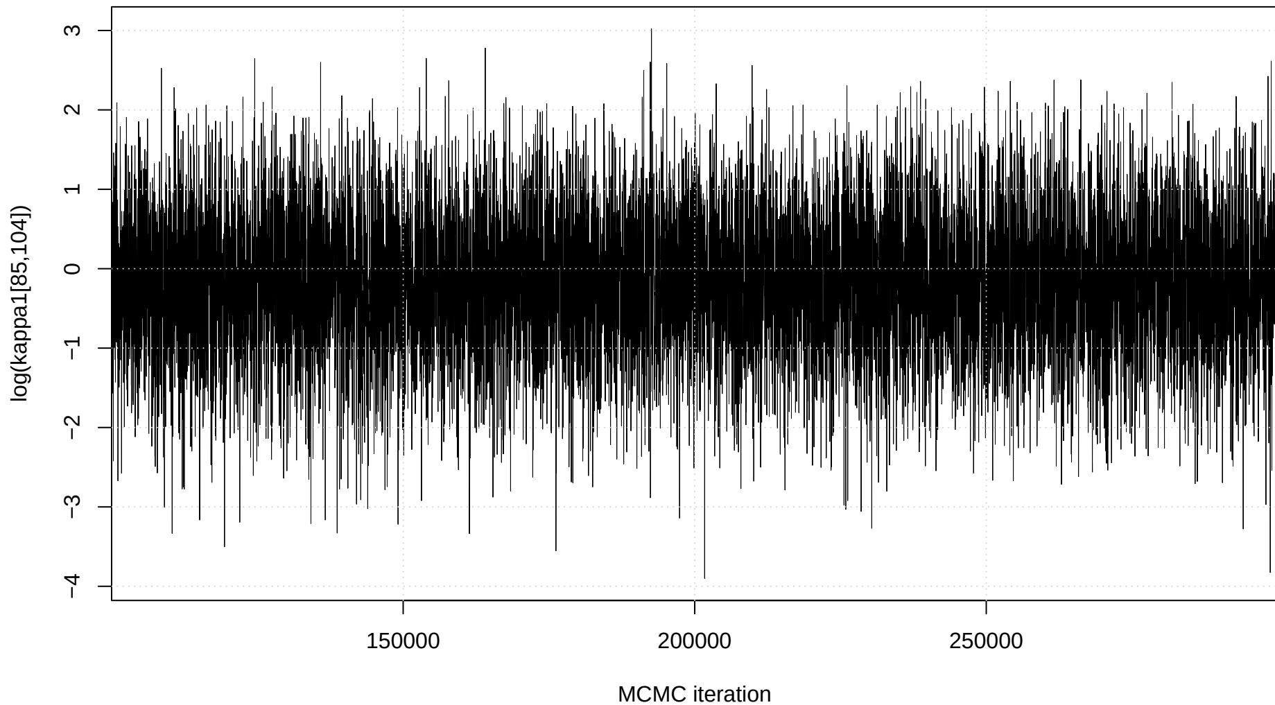
Trace plot: \log(\kappa_1[85,104])
