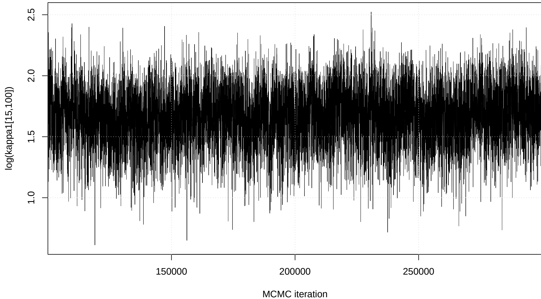
Trace plot: \log(\kappa_1[15,100])
