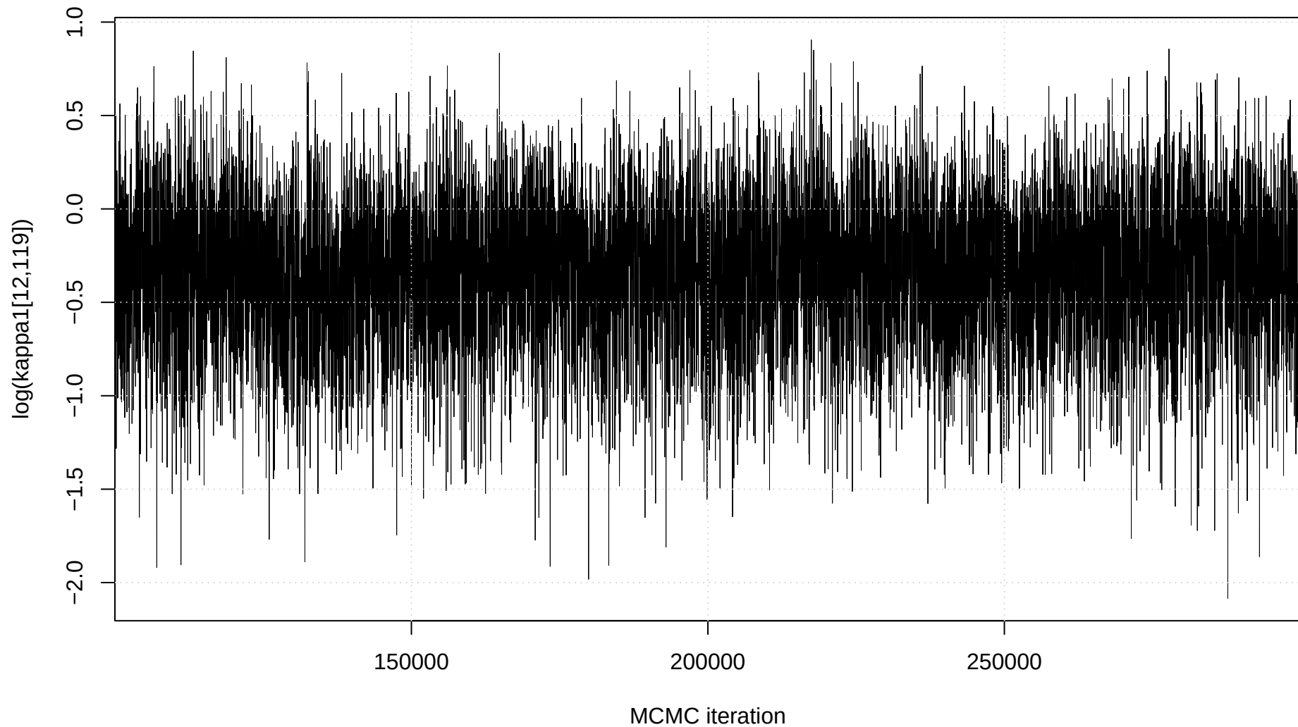
Trace plot: \log(\kappa_1[12,119])
