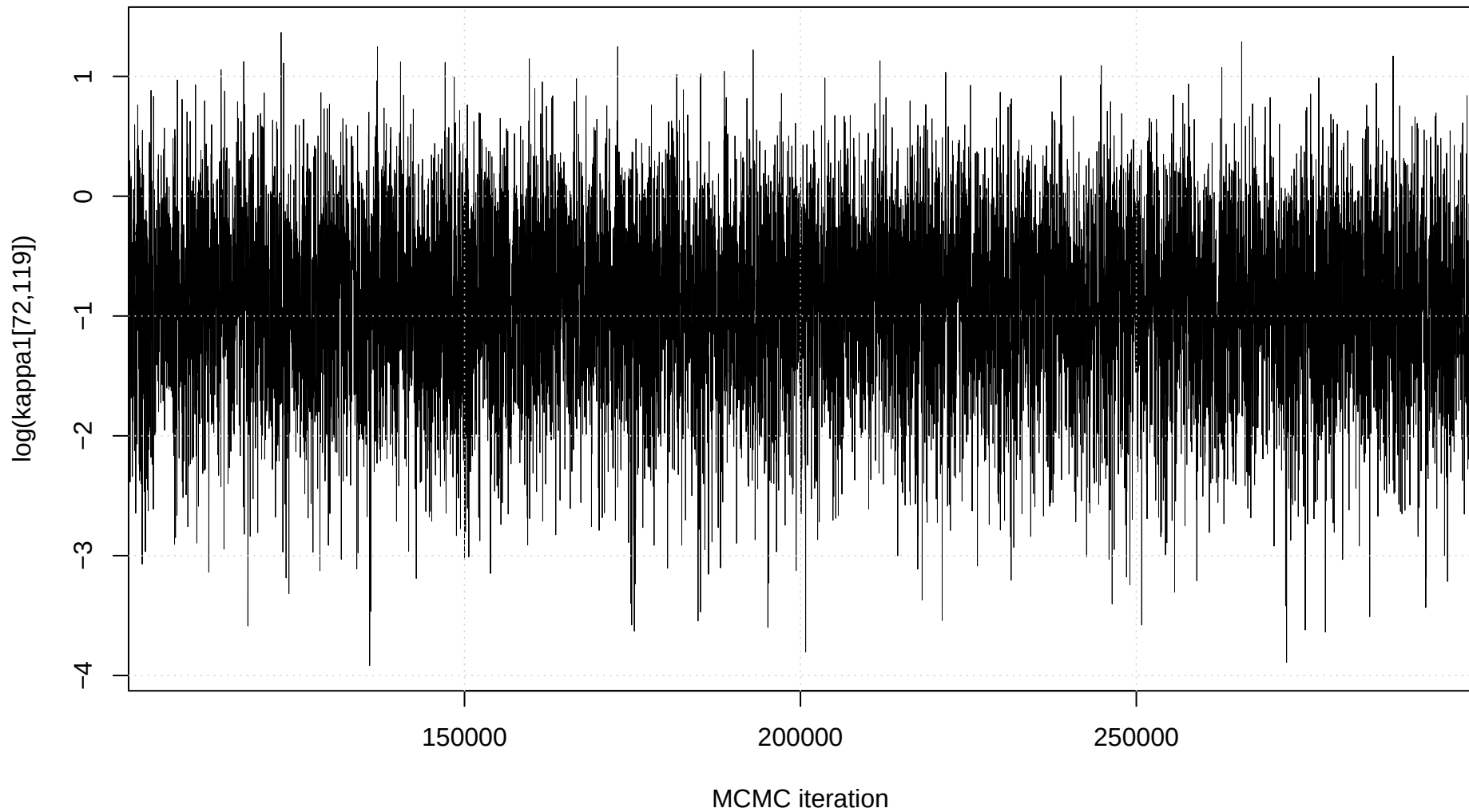
Trace plot: \log(\kappa_1[72,119])
