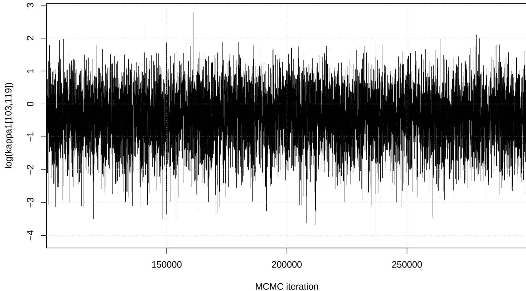
Trace plot: \log(\kappa_{1[103,119]})
