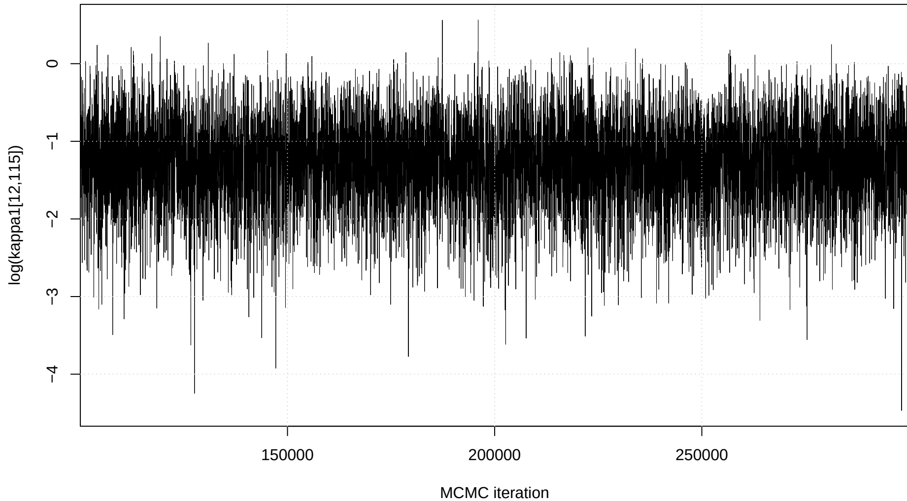
Trace plot: \log(\kappa_1[12,115])
