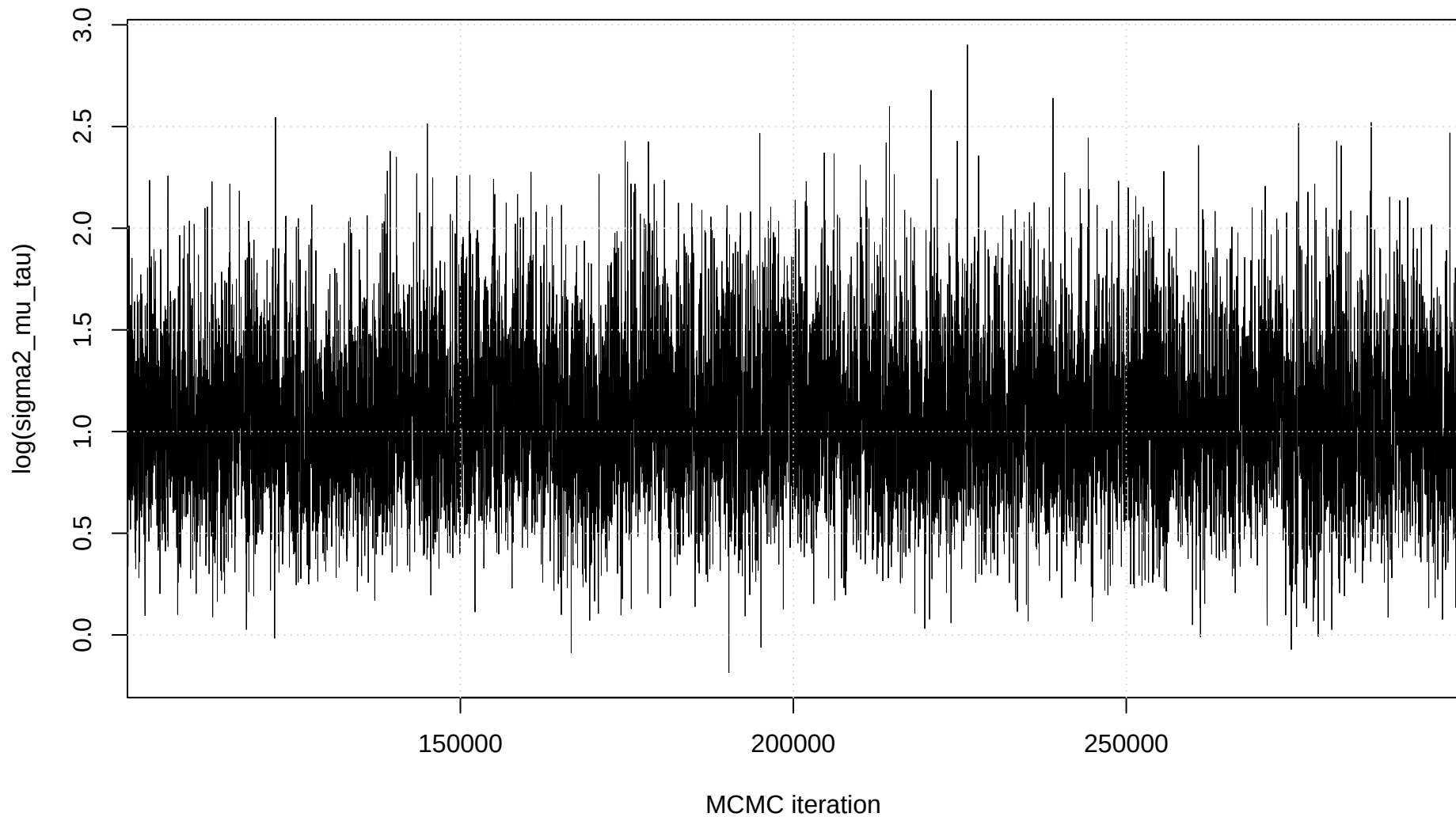
Trace plot: \log(\sigma^2_{\mu|\tau})
