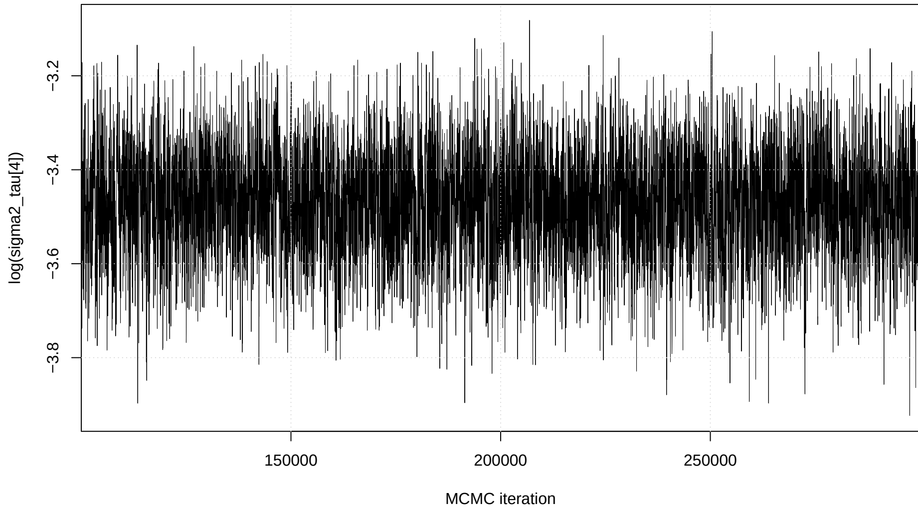
Trace plot: \log(\text{sigma2\_tau}[4])
