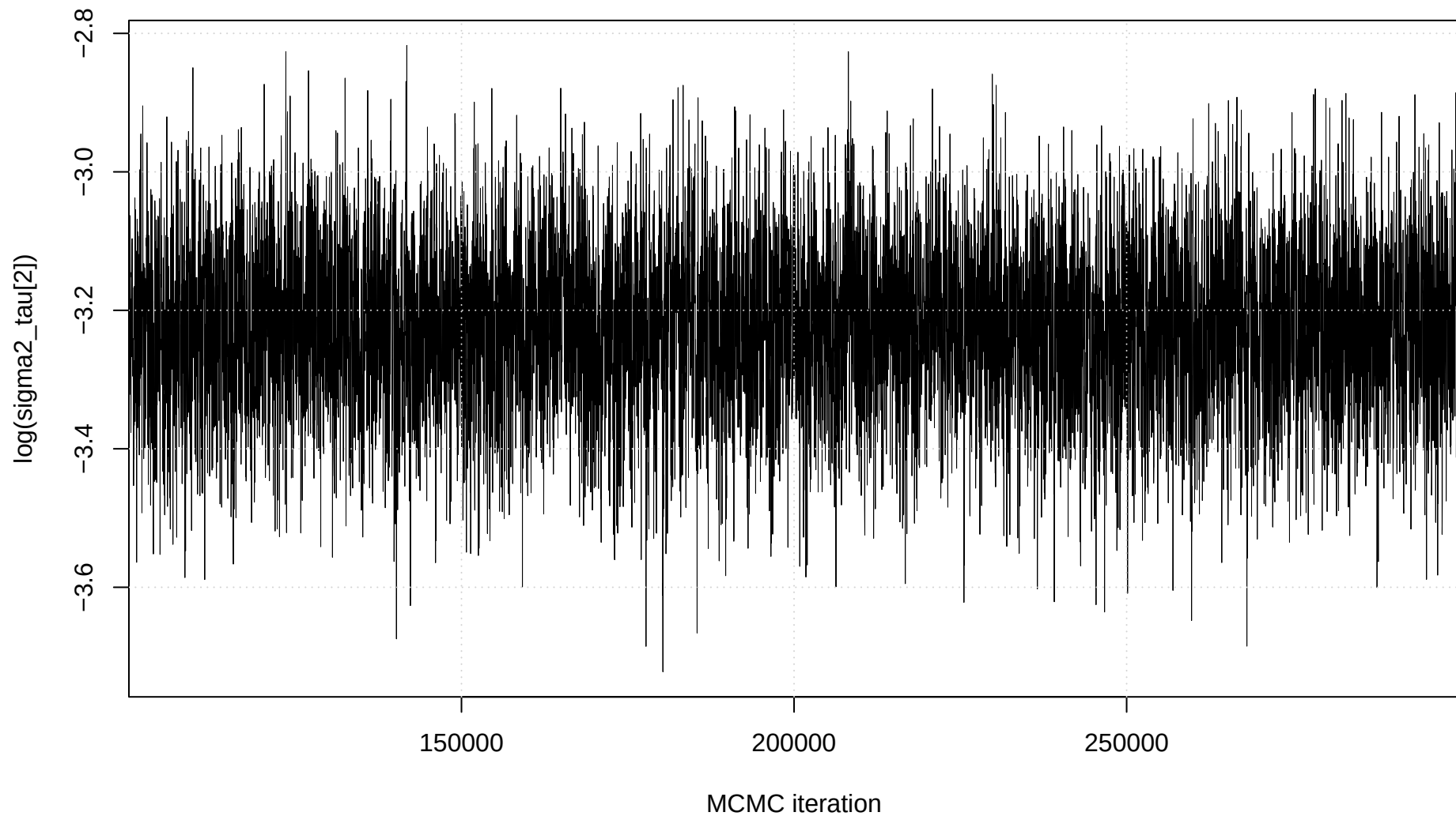
Trace plot: \log(\text{sigma2\_tau}[2])
