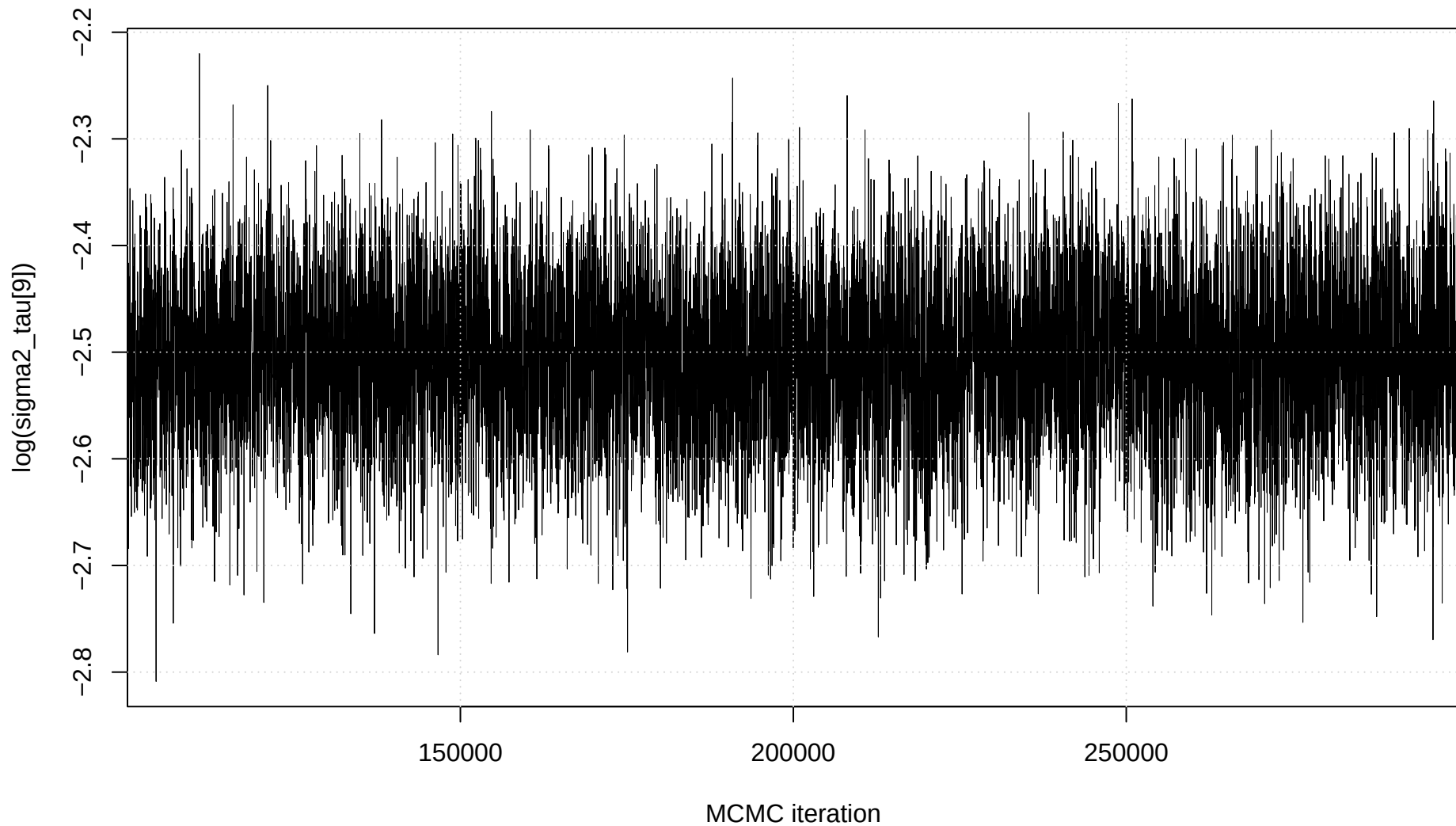
Trace plot: \log(\text{sigma2\_tau}[9])
