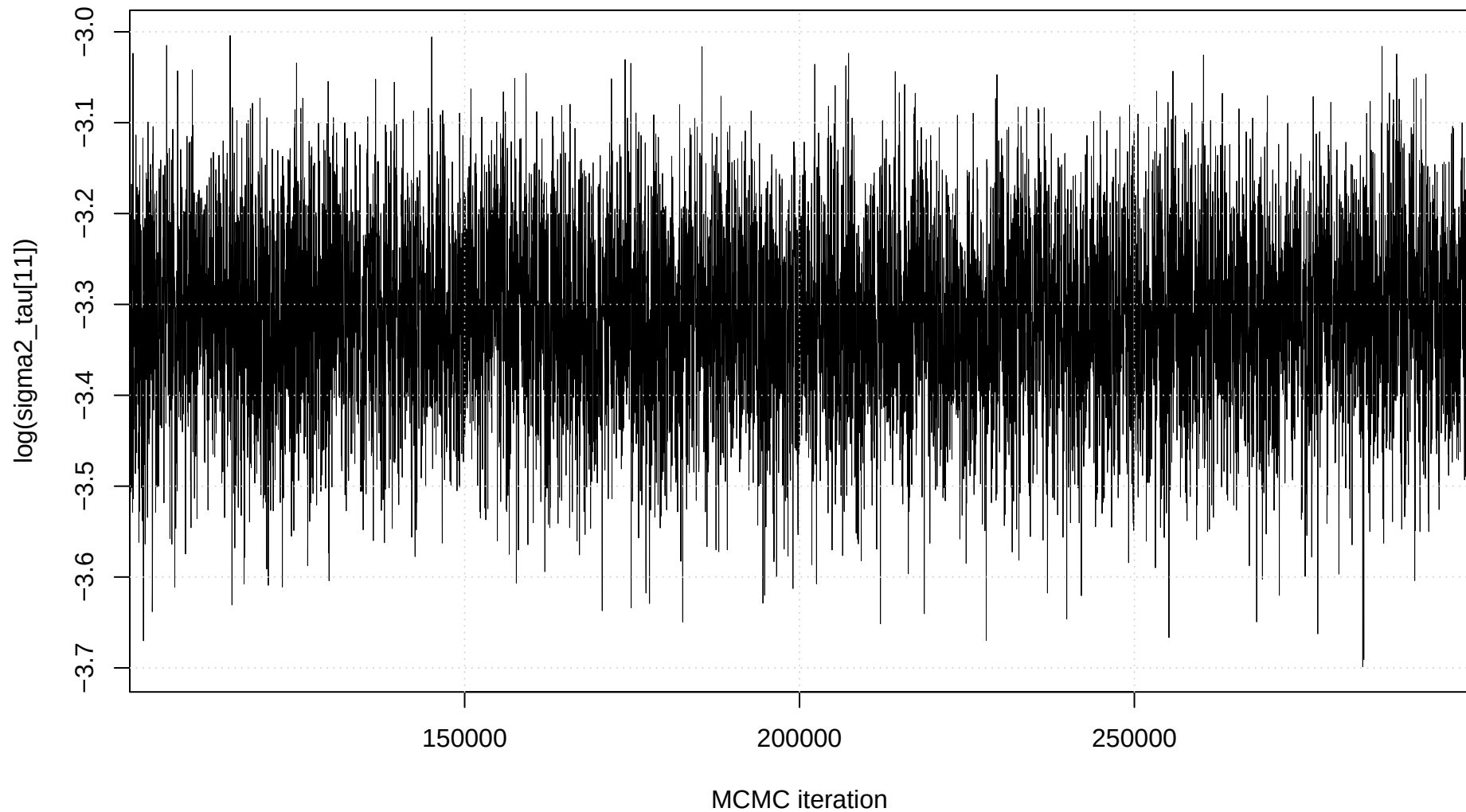
Trace plot: \log(\text{sigma2\_tau}[11])
