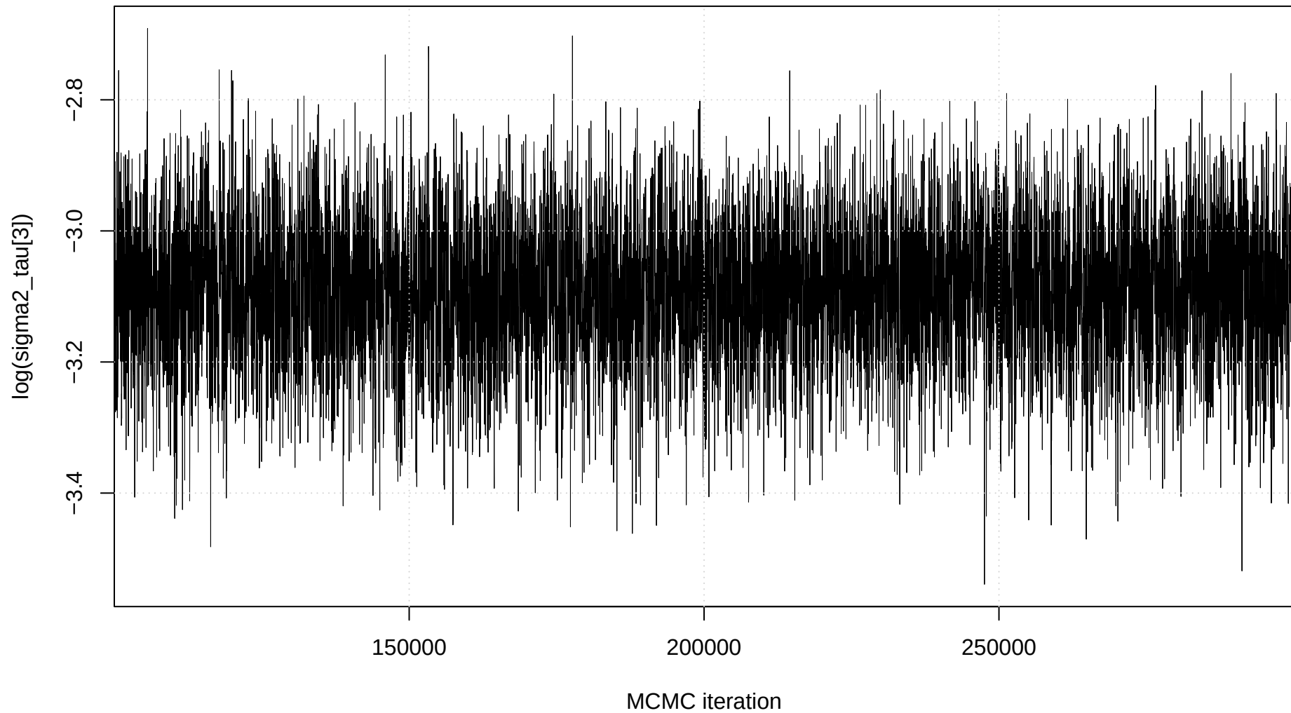
Trace plot: \log(\text{sigma2\_tau}[3])
