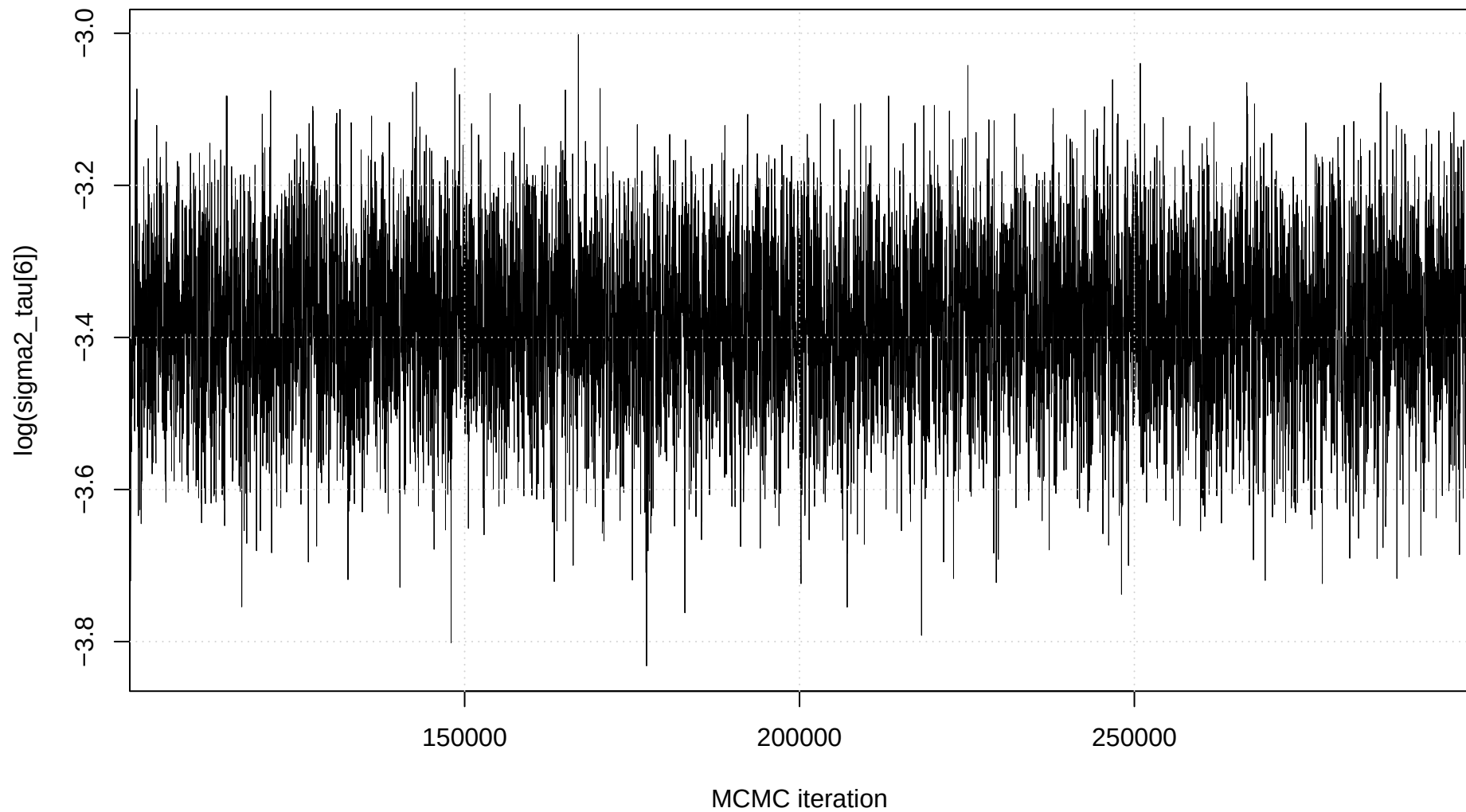
Trace plot: \log(\text{sigma2\_tau}[6])
