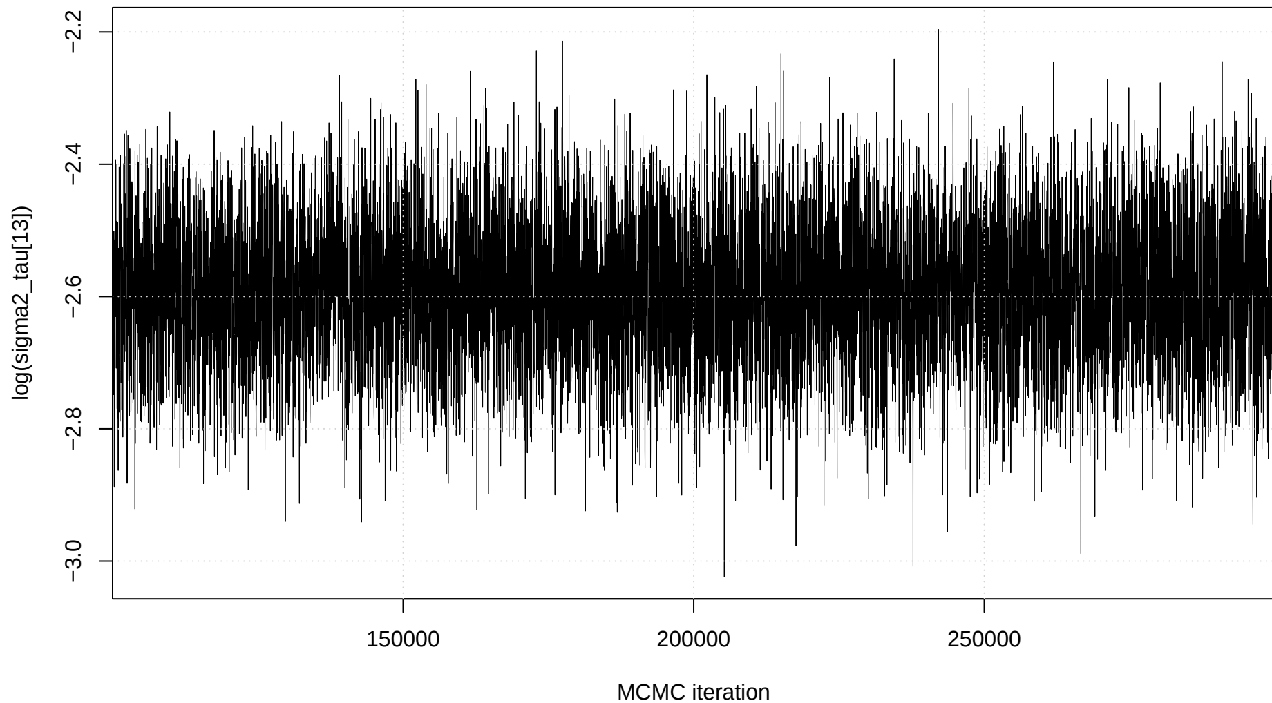
Trace plot: \log(\text{sigma2\_tau}[13])
