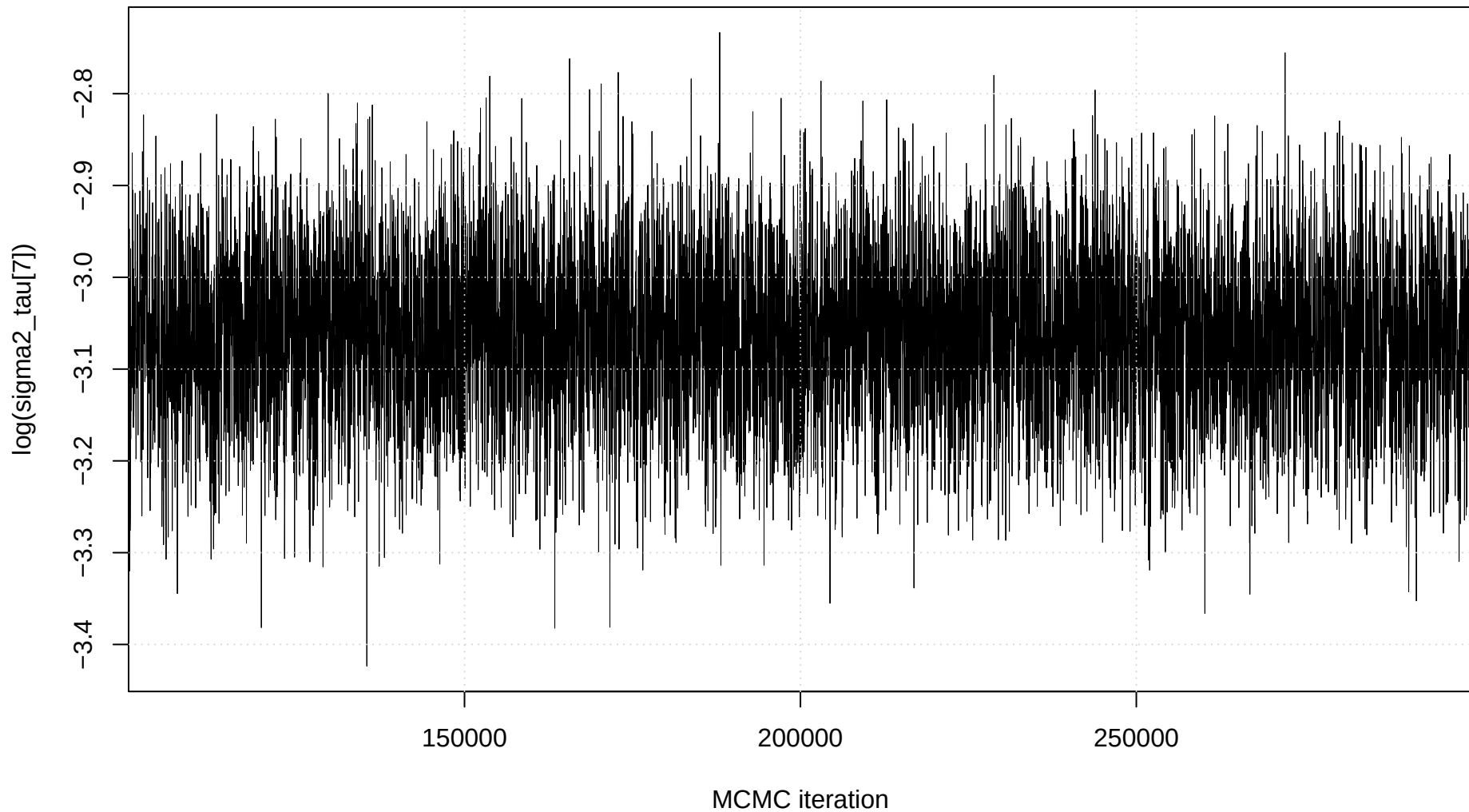
Trace plot: \log(\text{sigma2\_tau}[7])
