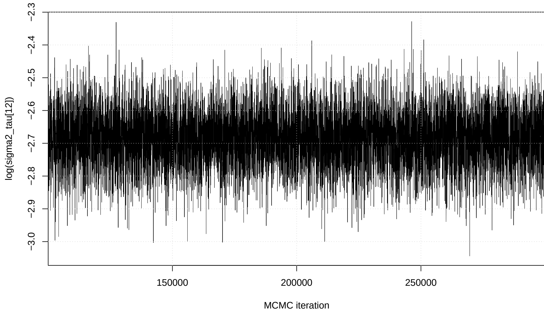
Trace plot: \log(\text{sigma2\_tau}[12])
