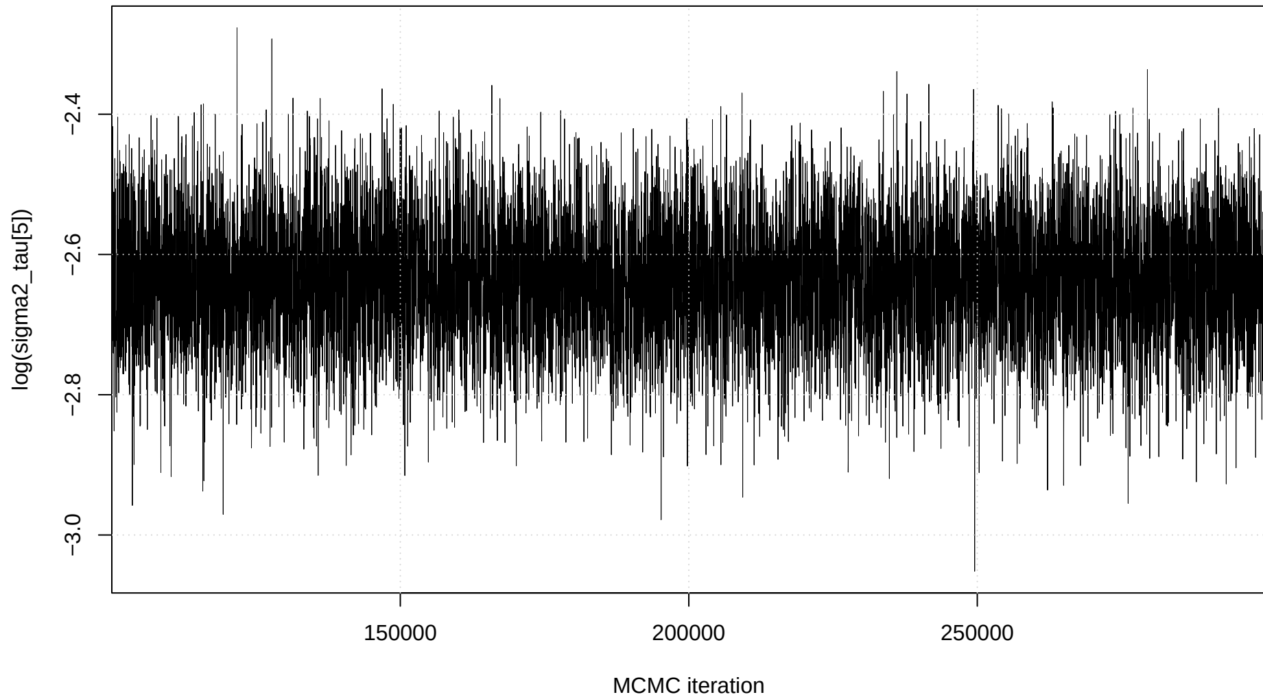
Trace plot: \log(\text{sigma2\_tau}[5])
