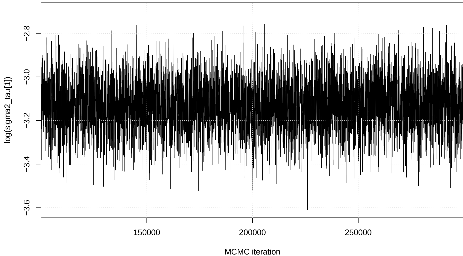
Trace plot: \log(\text{sigma2\_tau}[1])
