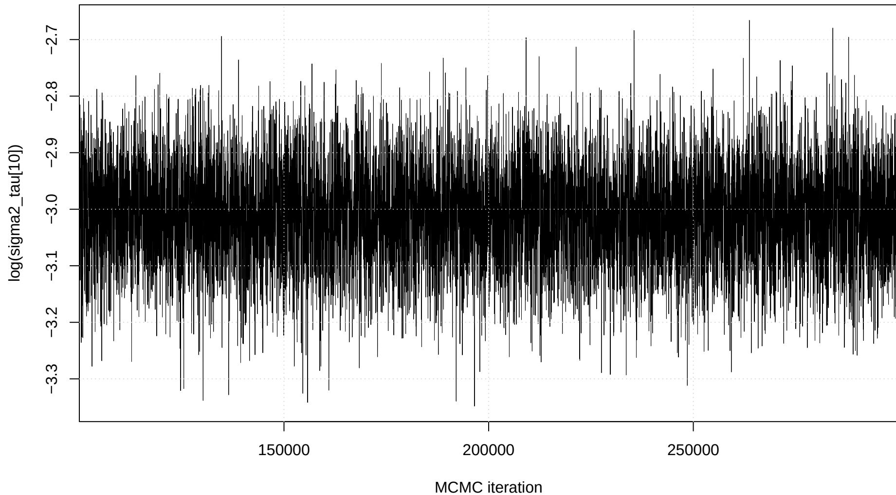
Trace plot: \log(\text{sigma2\_tau}[10])
