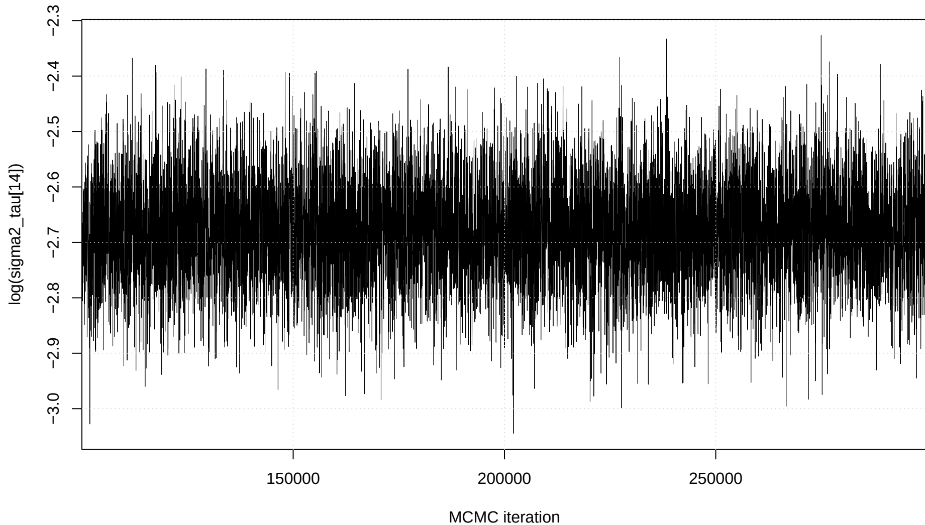
Trace plot: \log(\text{sigma2\_tau}[14])
