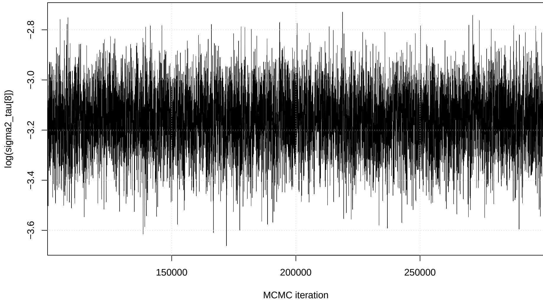
Trace plot: \log(\text{sigma2\_tau}[8])
