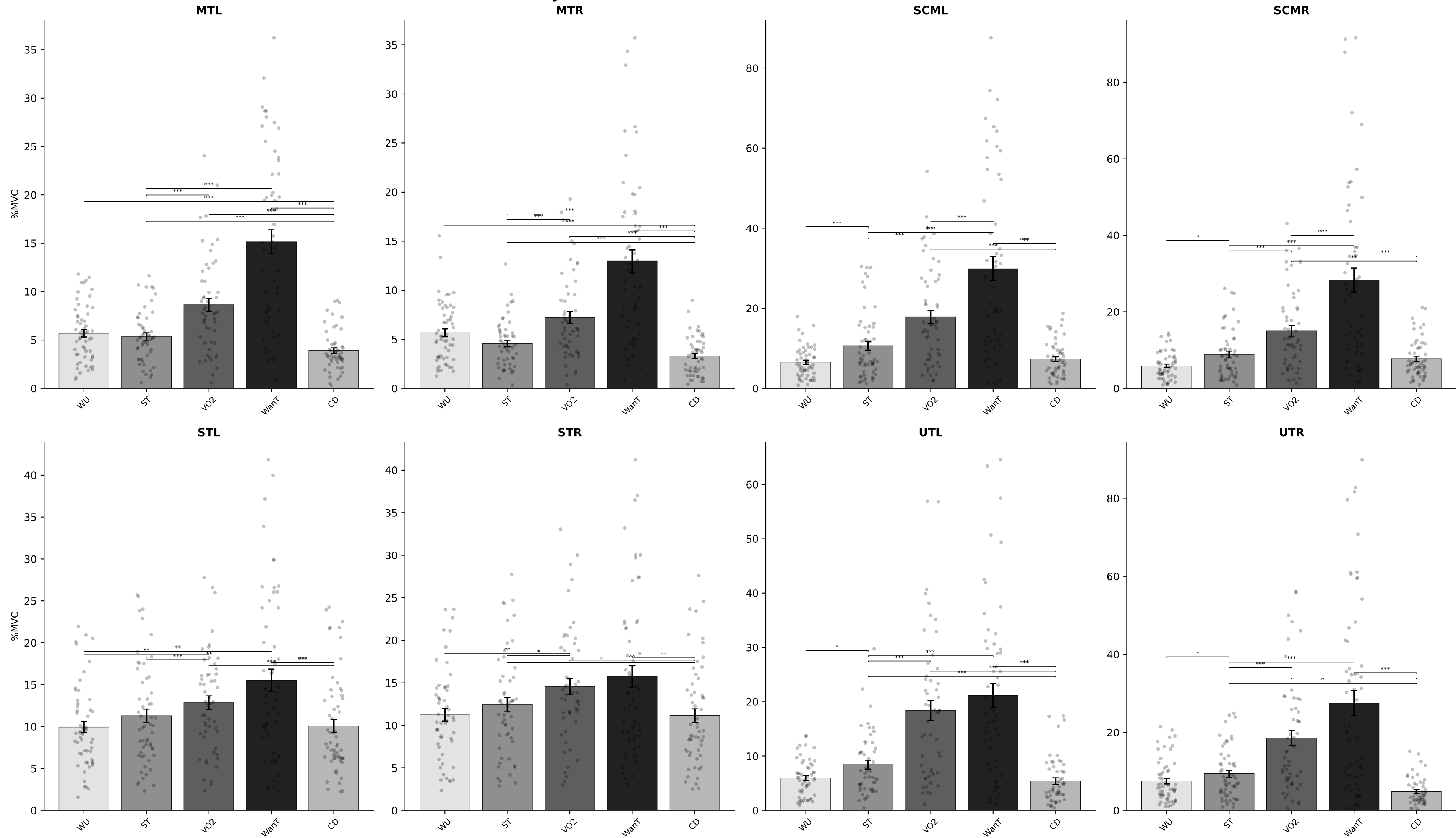
%MVC by Phase — All Muscles (RM ANOVA, outliers removed)
